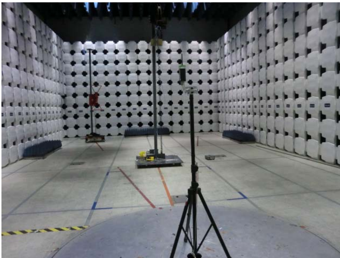
Scan from 1-18 GHz
