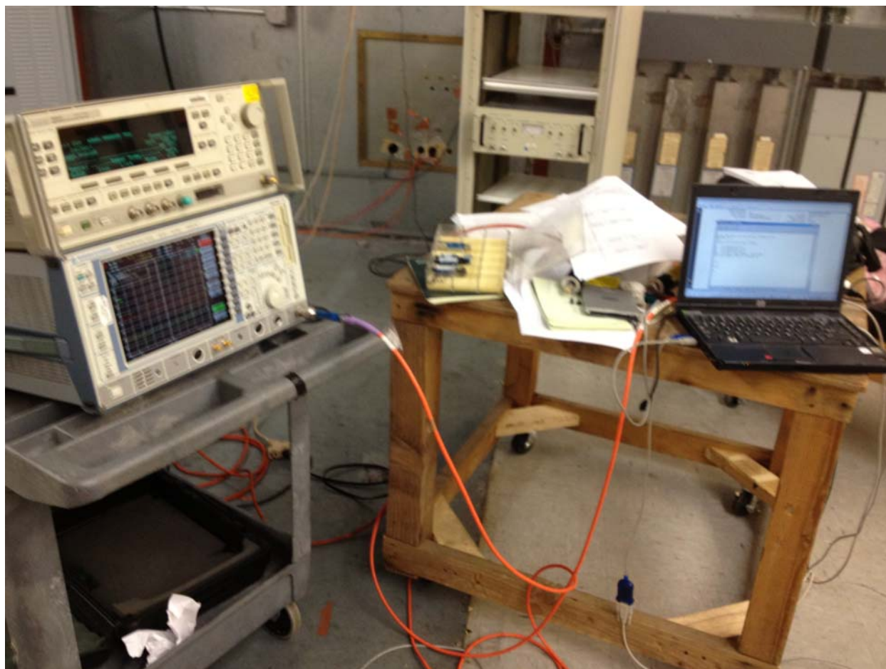
Antenna Port Conducted
