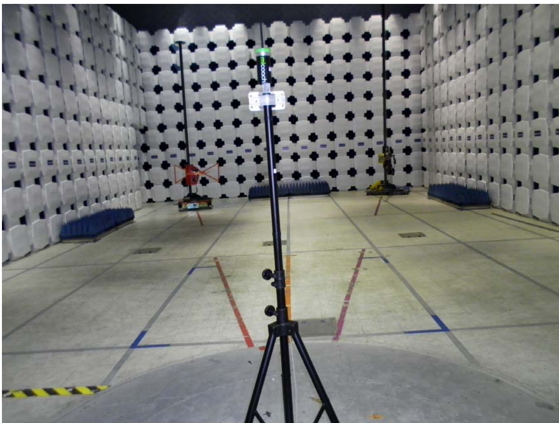
Scan from 30-1000MHz
