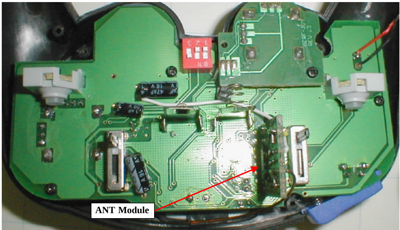
Controller Function PCB, Top
