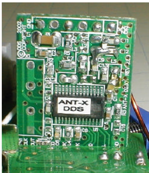
ANT Module In Place, Top View
