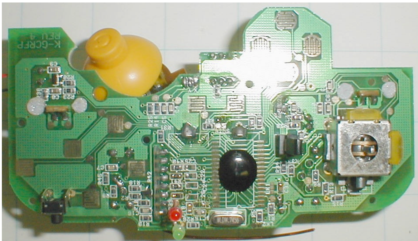
Controller Function PCB, Bottom
