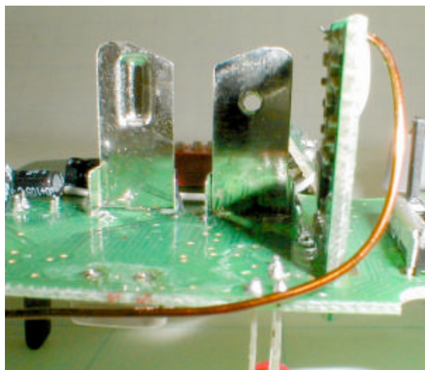
Antenna Detail
