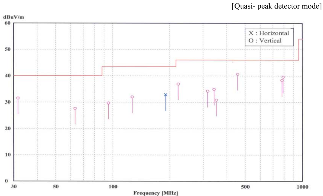
< Fig 6-1. Radiated emission result >
