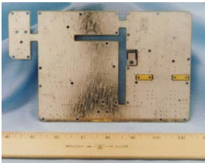
Figure 2: RF Assembly CCA, Solder Side
