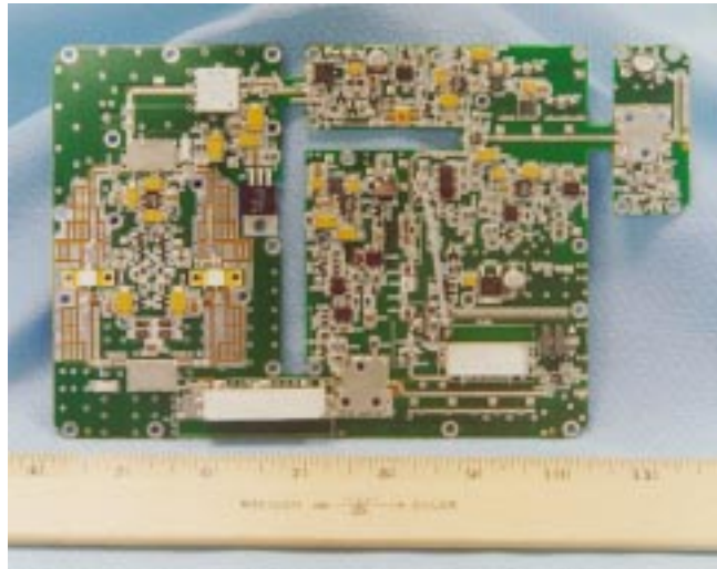
Figure 3: RF Assembly CCA, Component Side
