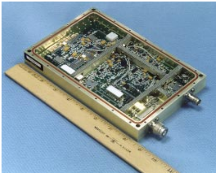
Figure 1: RF Assembly (LNA/PA) Cover Removed, Internal Chassis Assembly
