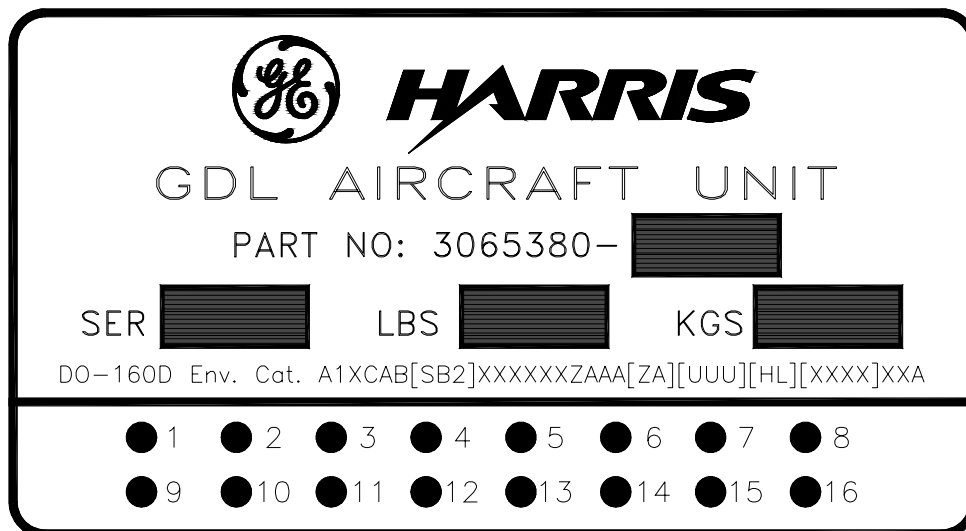
Figure 1.4: GDL Aircraft Unit Product Nameplate
