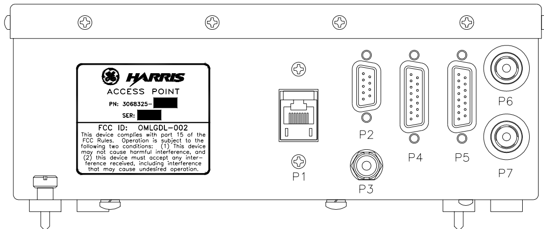
Figure 1.2: Access Point Compliance Label Mounting Location
