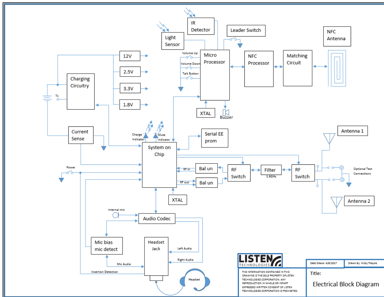
Figure 2. Electrical Block Diagram of Test Configuration
