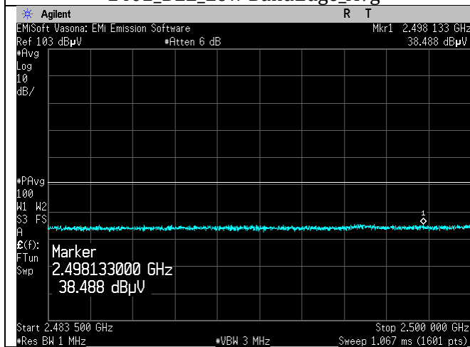
2480MHz_BLE_High BandEdge_Avg
