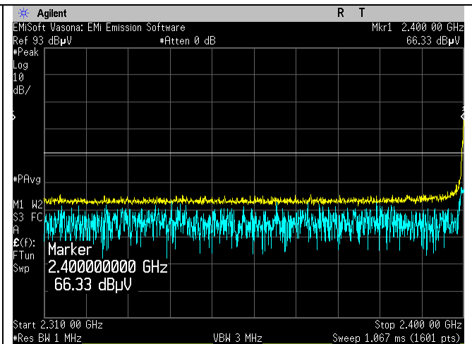
2402_BLE_Low BandEdge_Peak
