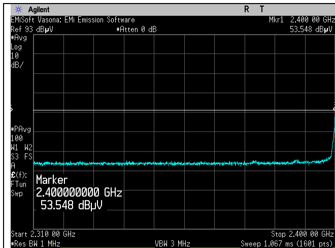
2402_BLE_Low BandEdge_Avg
