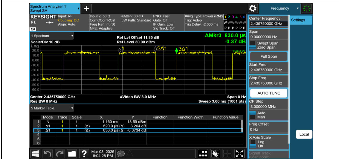
NTNV-11AX20MIMO-Ant2-2437-242Tone-RU61
