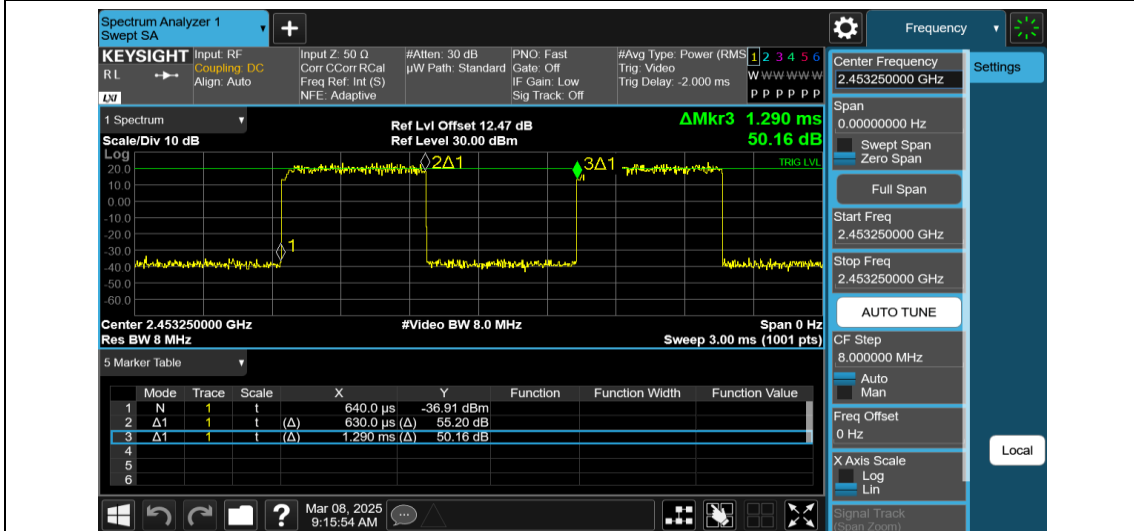
NTNV-11AX20MIMO-Ant1-2462-52Tone-RU37
