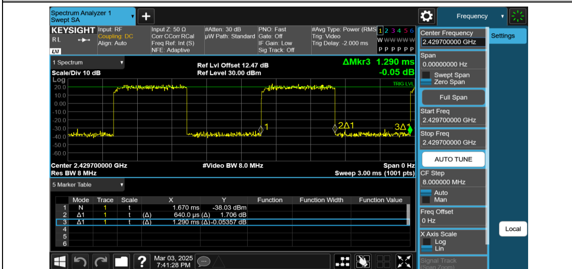
NTNV-11AX20MIMO-Ant1-2437-52Tone-RU37
