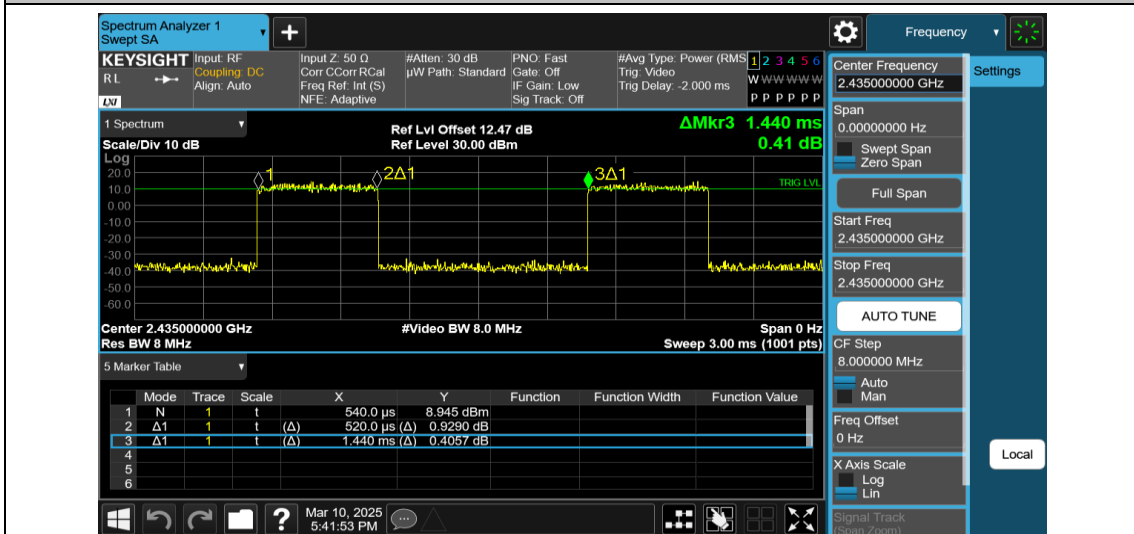
NTNV-11AX40MIMO-Ant1-2437-484Tone-RU65
