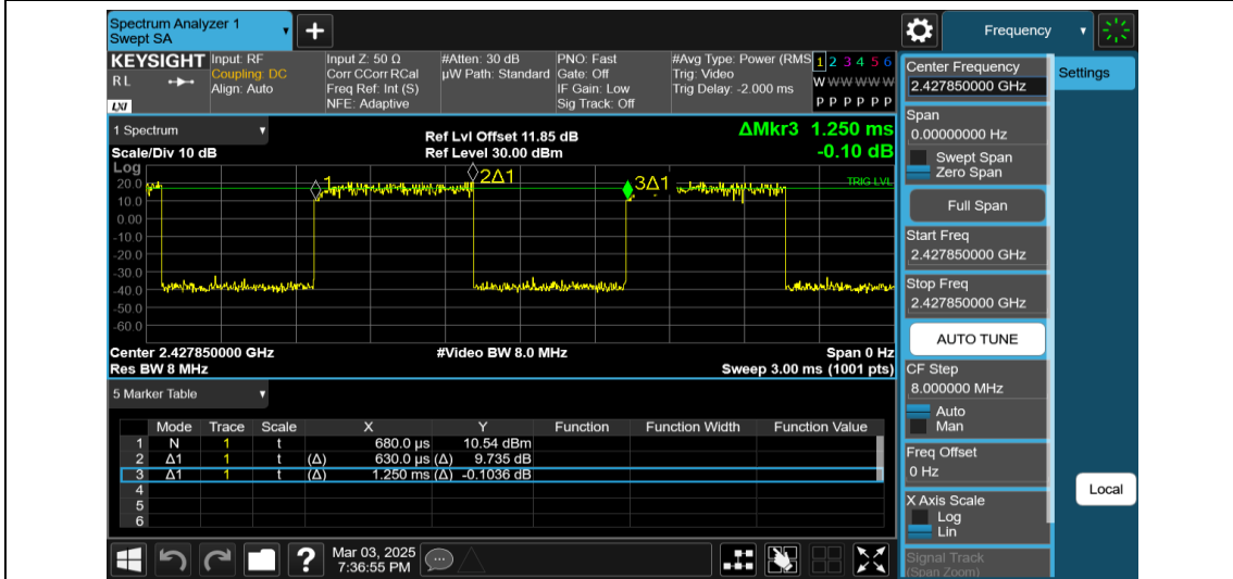
NTNV-11AX20MIMO-Ant2-2437-26Tone-RU0
