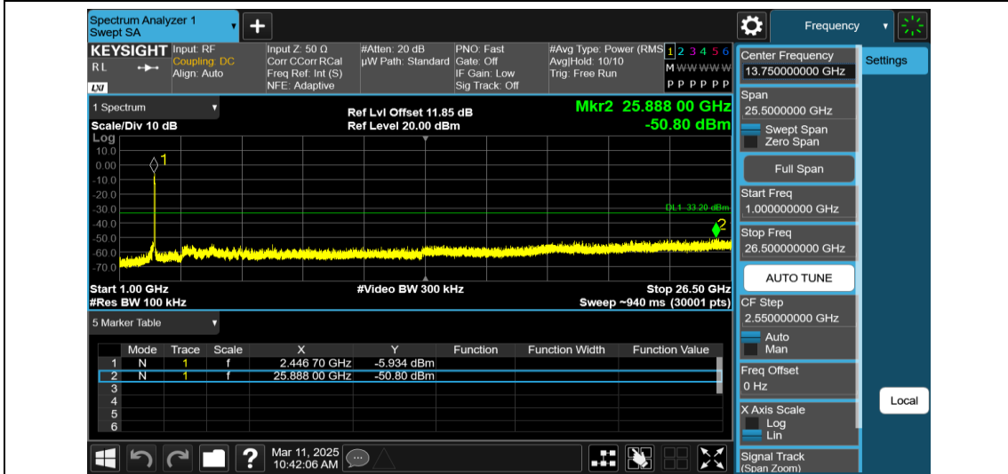
11AX40MIMO-Ant2-2452-484Tone-RU65-1000~26500-PASS
