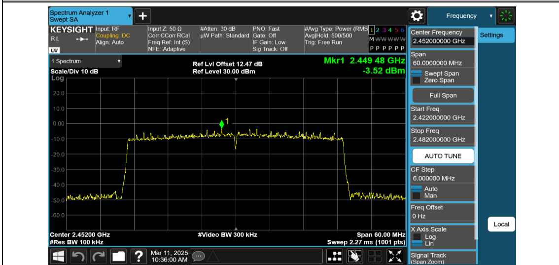
11AX40MIMO-Ant1-2452-484Tone-RU65-0~Reference-PASS
