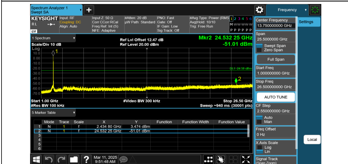
11AX40MIMO-Ant1-2452-26Tone-RU0-1000~26500-PASS
