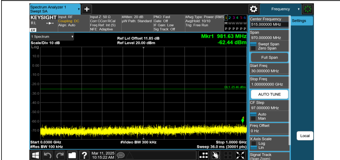
11AX40MIMO-Ant2-2452-52Tone-RU37-30~1000-PASS
