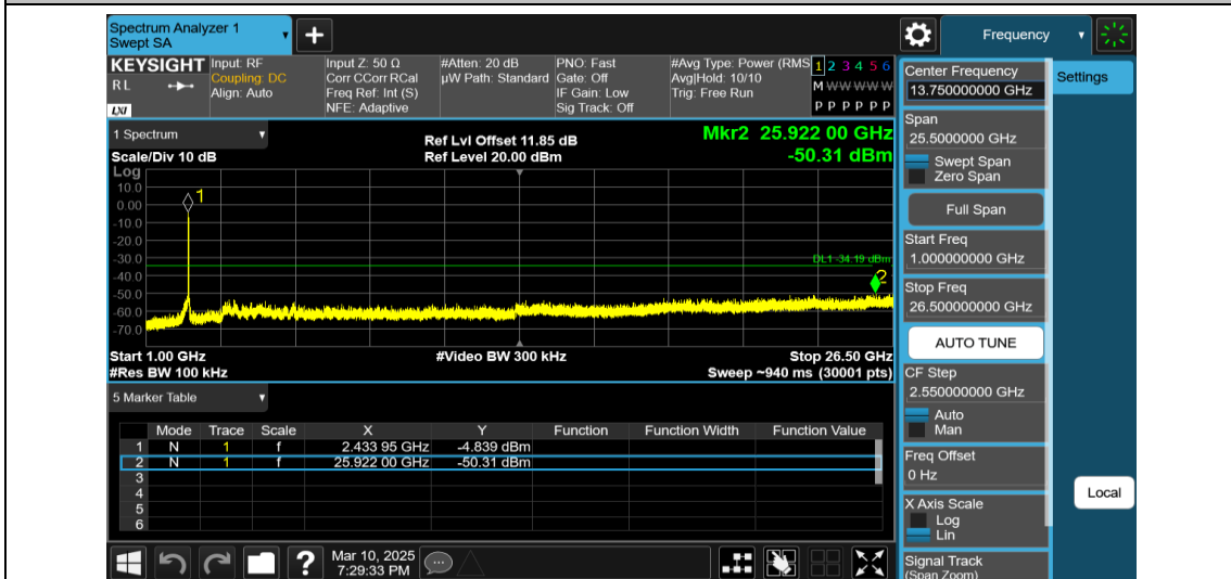
11AX40MIMO-Ant2-2437-484Tone-RU65-1000~26500-PASS
