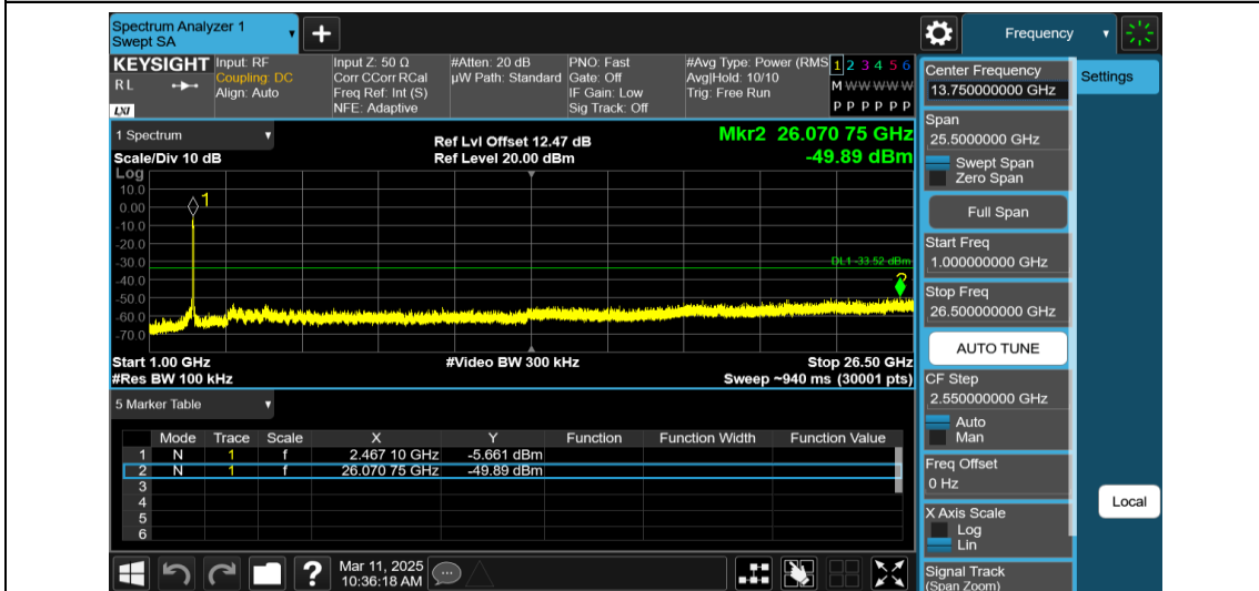
11AX40MIMO-Ant1-2452-484Tone-RU65-1000~26500-PASS
