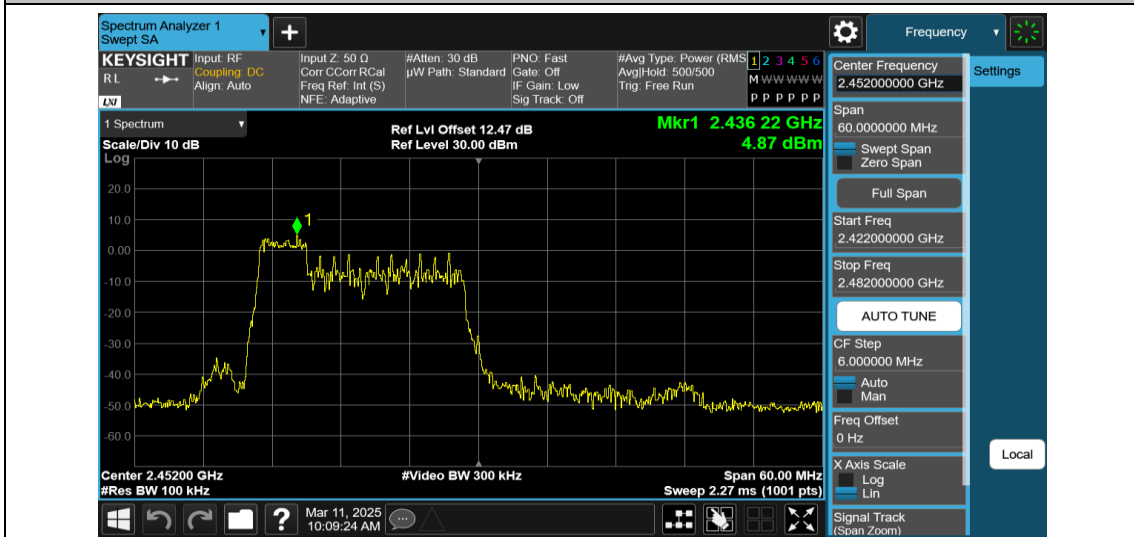
11AX40MIMO-Ant1-2452-52Tone-RU37-0~Reference-PASS
