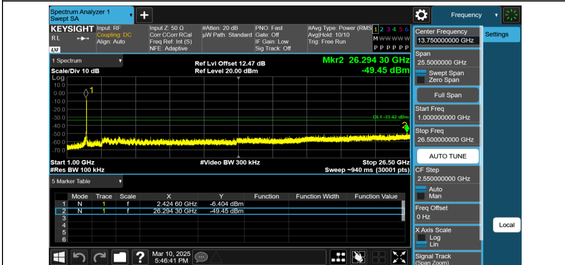
11AX40MIMO-Ant1-2437-484Tone-RU65-1000~26500-PASS
