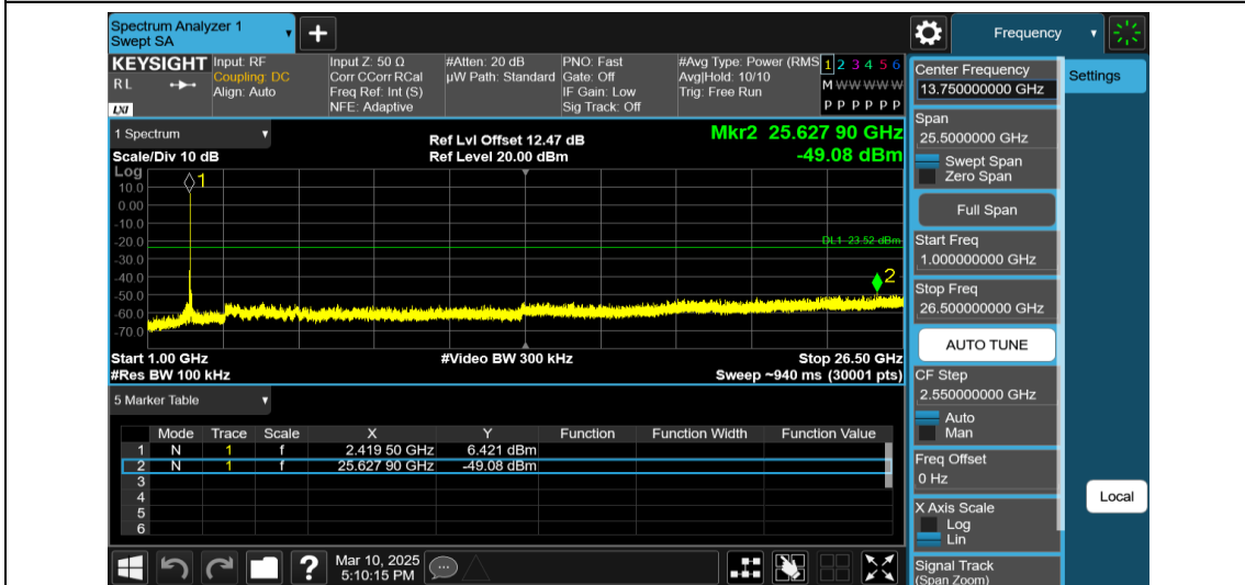
11AX40MIMO-Ant1-2437-26Tone-RU0-1000~26500-PASS
