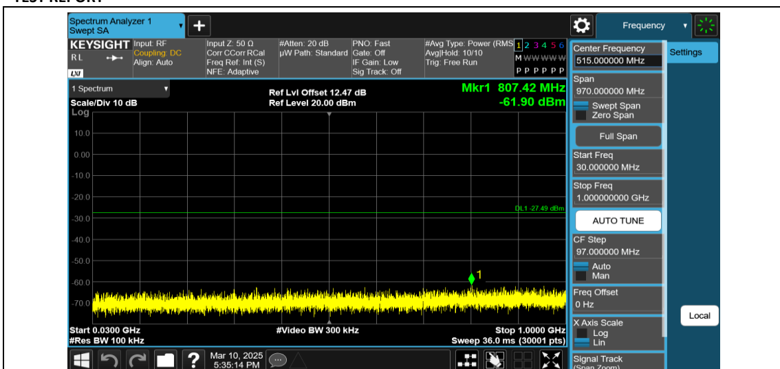
11AX40MIMO-Ant1-2437-106Tone-RU53-30~1000-PASS
