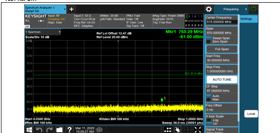
11AX40MIMO-Ant1-2452-52Tone-RU37-30~1000-PASS
