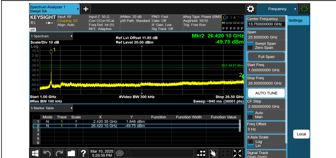
11AX40MIMO-Ant2-2437-52Tone-RU37-1000~26500-PASS
