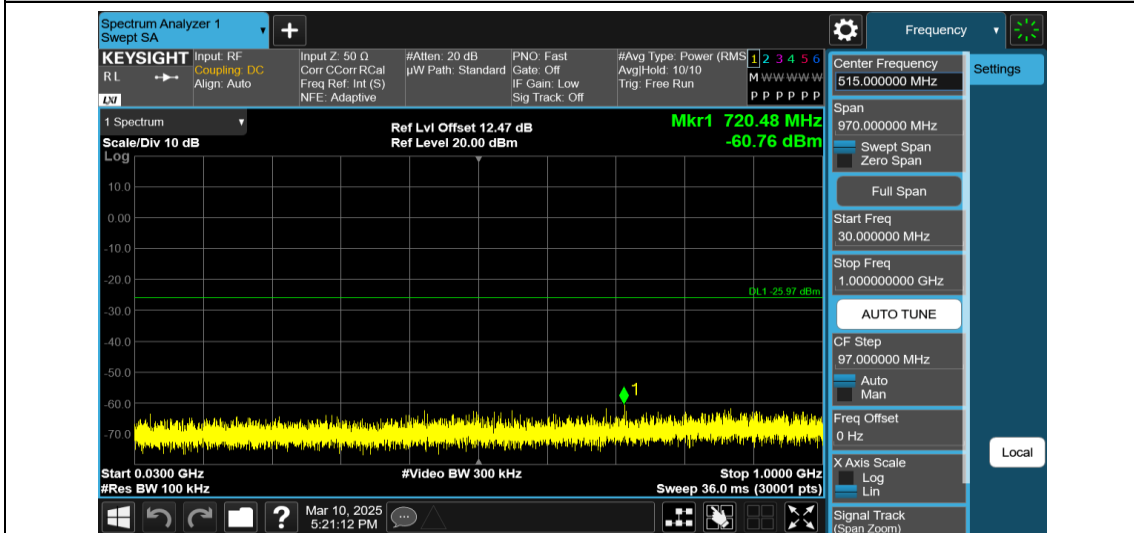
11AX40MIMO-Ant1-2437-52Tone-RU37-30~1000-PASS
