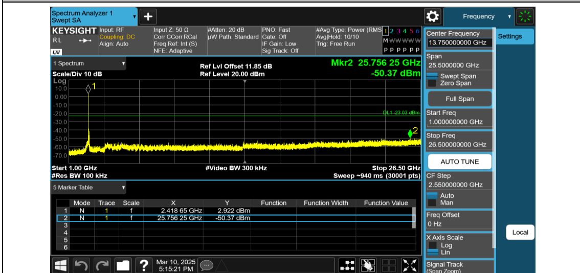
11AX40MIMO-Ant2-2437-26Tone-RU0-1000~26500-PASS
