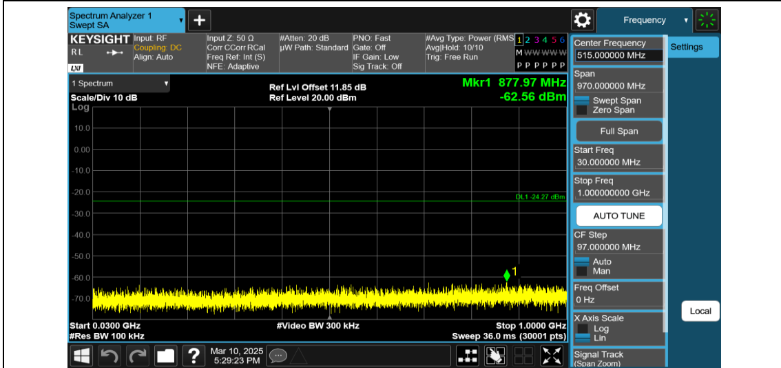
11AX40MIMO-Ant2-2437-52Tone-RU37-30~1000-PASS
