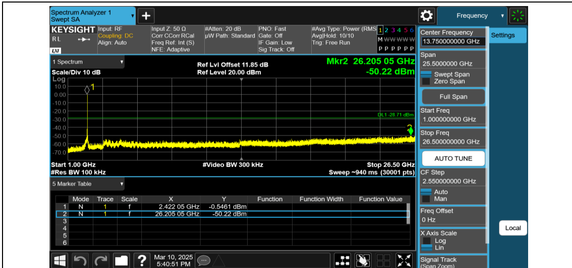
11AX40MIMO-Ant2-2437-106Tone-RU53-1000~26500-PASS
