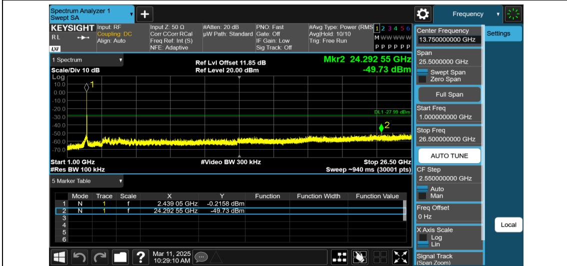
11AX40MIMO-Ant2-2452-106Tone-RU53-1000~26500-PASS
