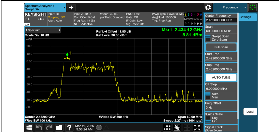
11AX40MIMO-Ant2-2452-26Tone-RU0-0~Reference-PASS
