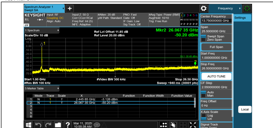
11AX40MIMO-Ant2-2452-242Tone-RU61-1000~26500-PASS
