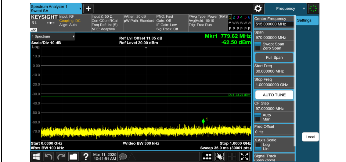
11AX40MIMO-Ant2-2452-484Tone-RU65-30~1000-PASS
