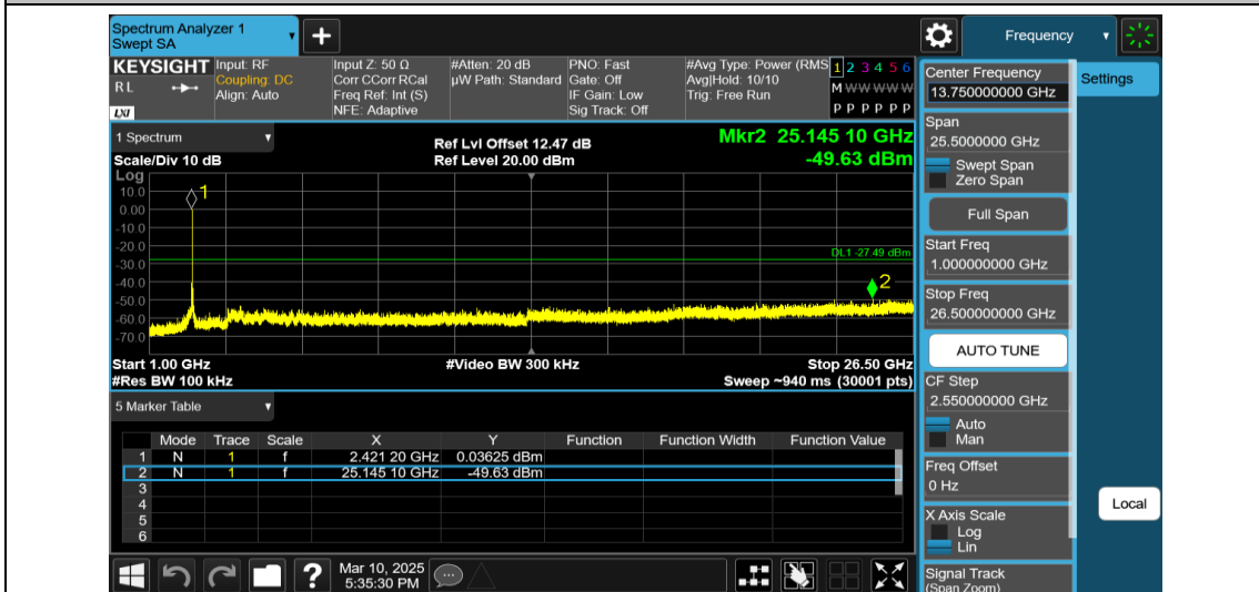
11AX40MIMO-Ant1-2437-106Tone-RU53-1000~26500-PASS
