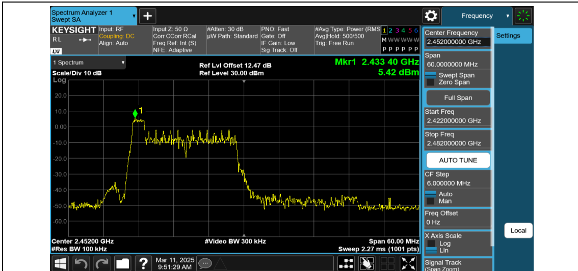
11AX40MIMO-Ant1-2452-26Tone-RU0-0~Reference-PASS
