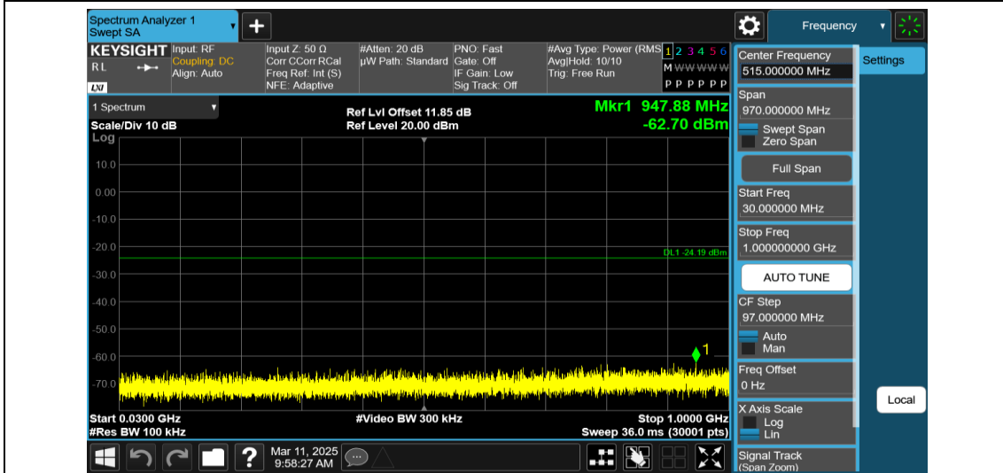
11AX40MIMO-Ant2-2452-26Tone-RU0-30~1000-PASS
