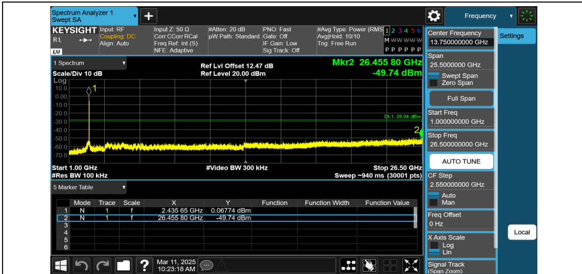
11AX40MIMO-Ant1-2452-106Tone-RU53-1000~26500-PASS
