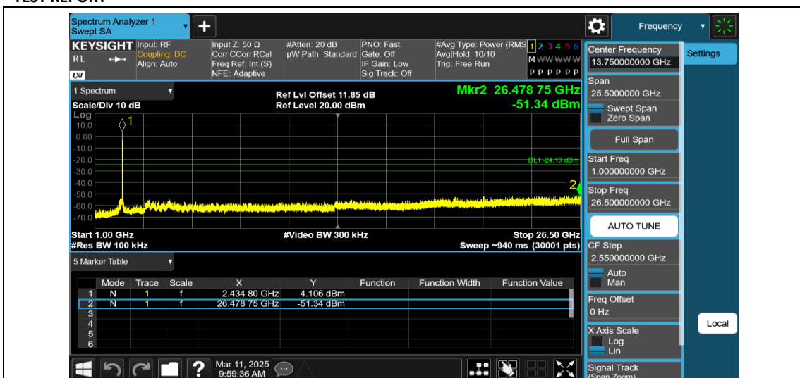
11AX40MIMO-Ant2-2452-26Tone-RU0-1000~26500-PASS
