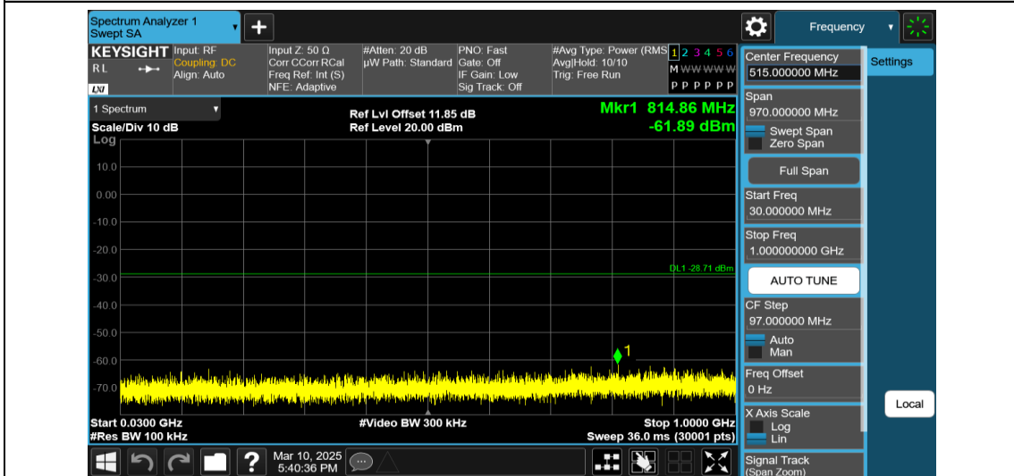
11AX40MIMO-Ant2-2437-106Tone-RU53-30~1000-PASS
