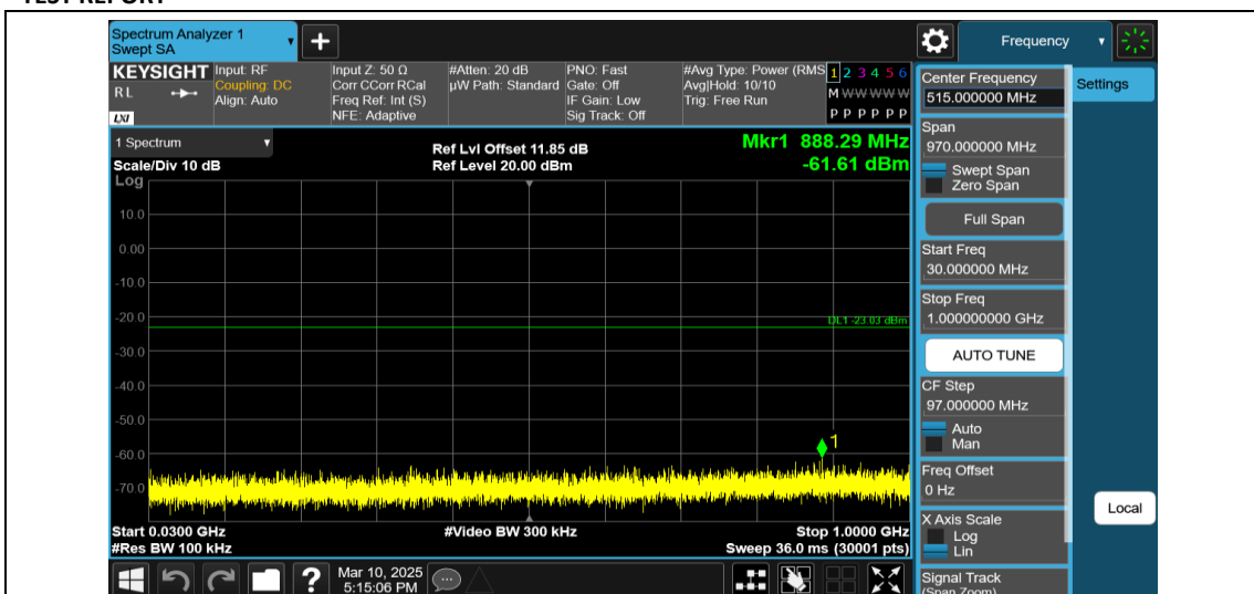
11AX40MIMO-Ant2-2437-26Tone-RU0-30~1000-PASS
