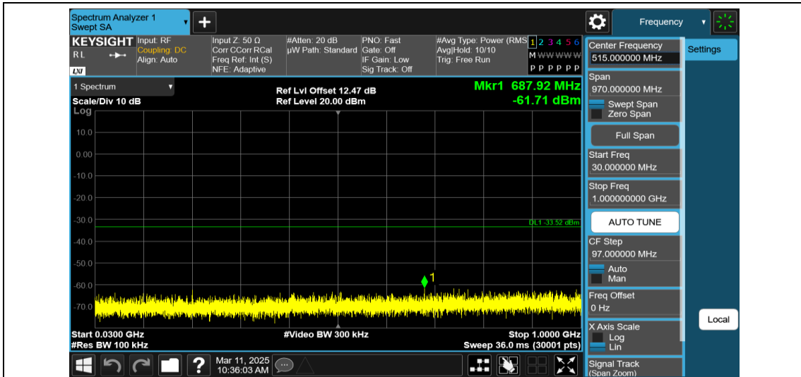
11AX40MIMO-Ant1-2452-484Tone-RU65-30~1000-PASS
