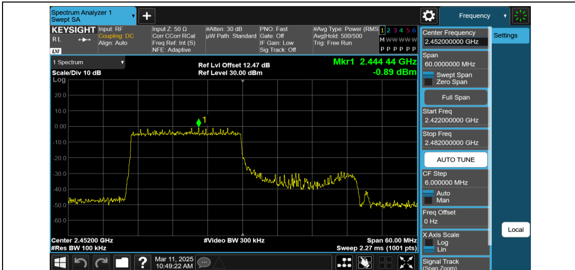
11AX40MIMO-Ant1-2452-242Tone-RU61-0~Reference-PASS
