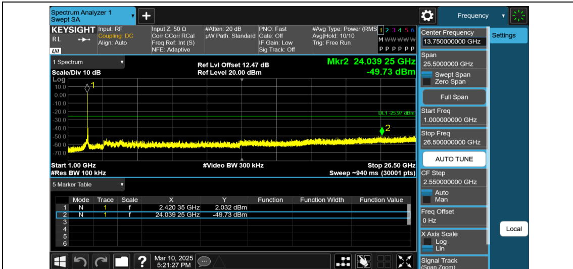
11AX40MIMO-Ant1-2437-52Tone-RU37-1000~26500-PASS
