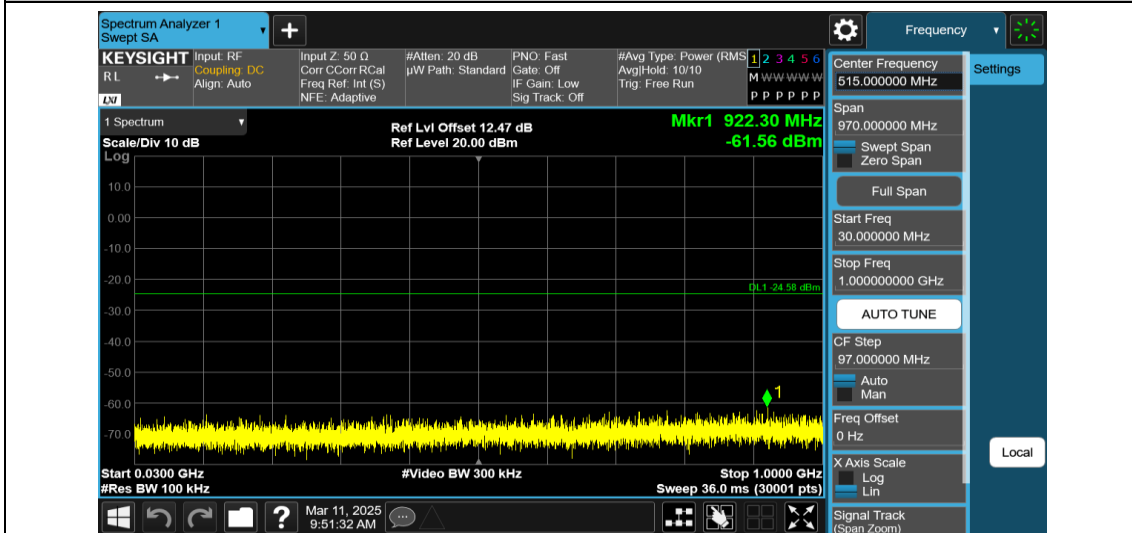
11AX40MIMO-Ant1-2452-26Tone-RU0-30~1000-PASS
