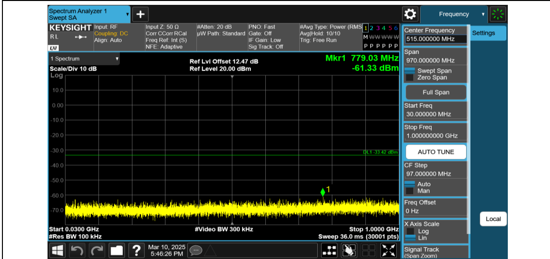
11AX40MIMO-Ant1-2437-484Tone-RU65-30~1000-PASS
