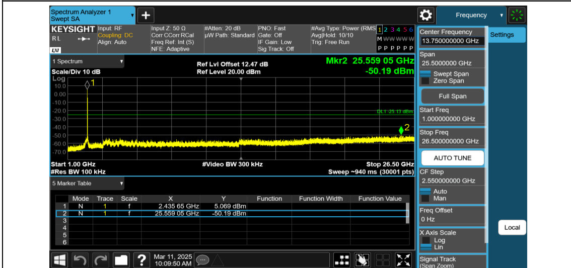
11AX40MIMO-Ant1-2452-52Tone-RU37-1000~26500-PASS
