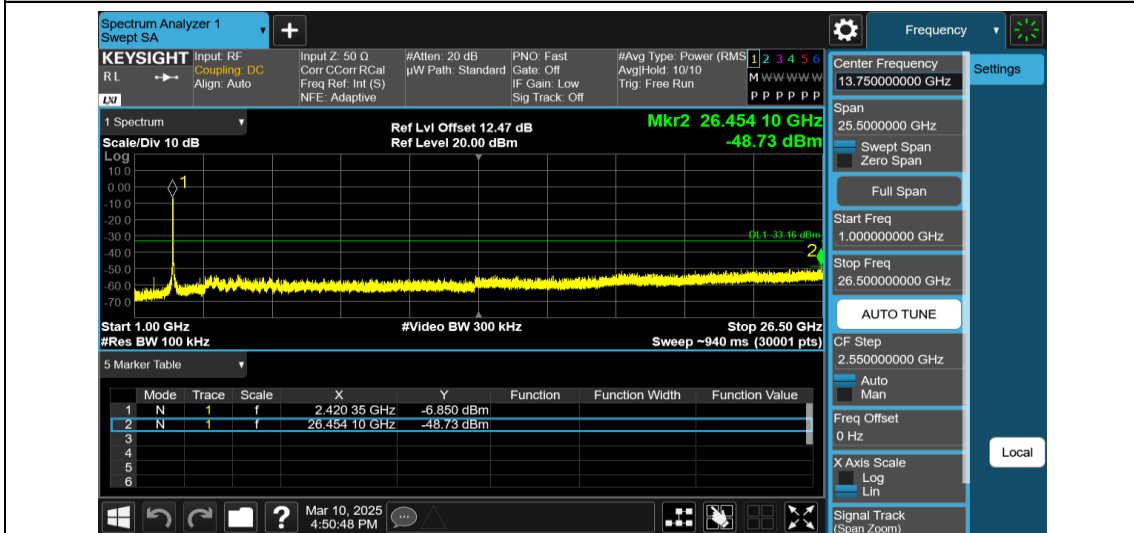
11AX40MIMO-Ant1-2422-484Tone-RU65-1000~26500-PASS
