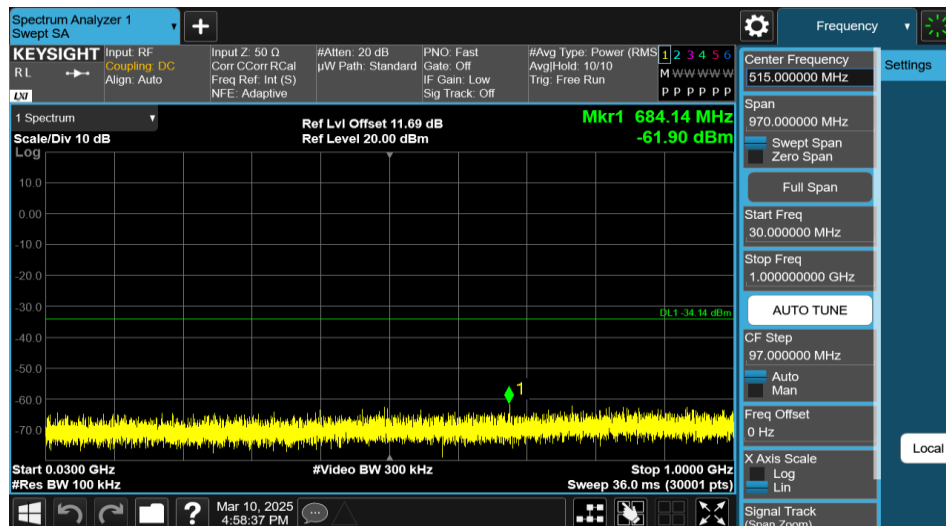
11AX40MIMO-Ant2-2422-484Tone-RU65-30~1000-PASS
