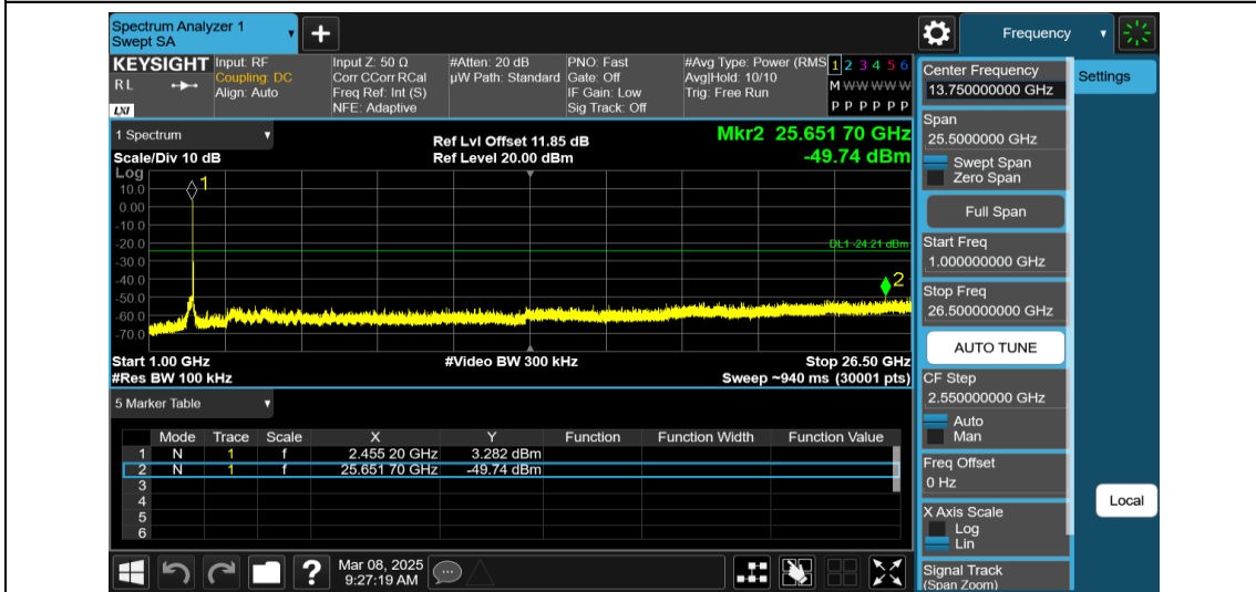
11AX20MIMO-Ant2-2462-52Tone-RU37-1000~26500-PASS
