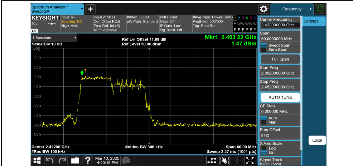
11AX40MIMO-Ant2-2422-106Tone-RU53-0~Reference-PASS
