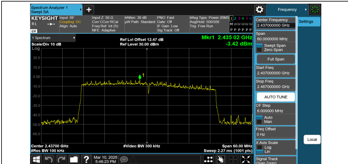
11AX40MIMO-Ant1-2437-484Tone-RU65-0~Reference-PASS
