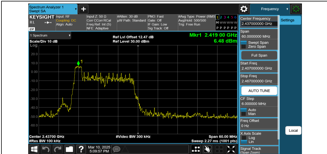
11AX40MIMO-Ant1-2437-26Tone-RU0-0~Reference-PASS
