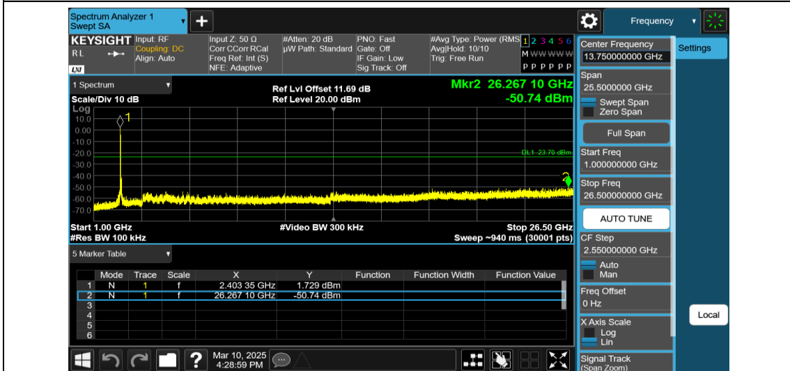
11AX40MIMO-Ant2-2422-52Tone-RU37-1000~26500-PASS
