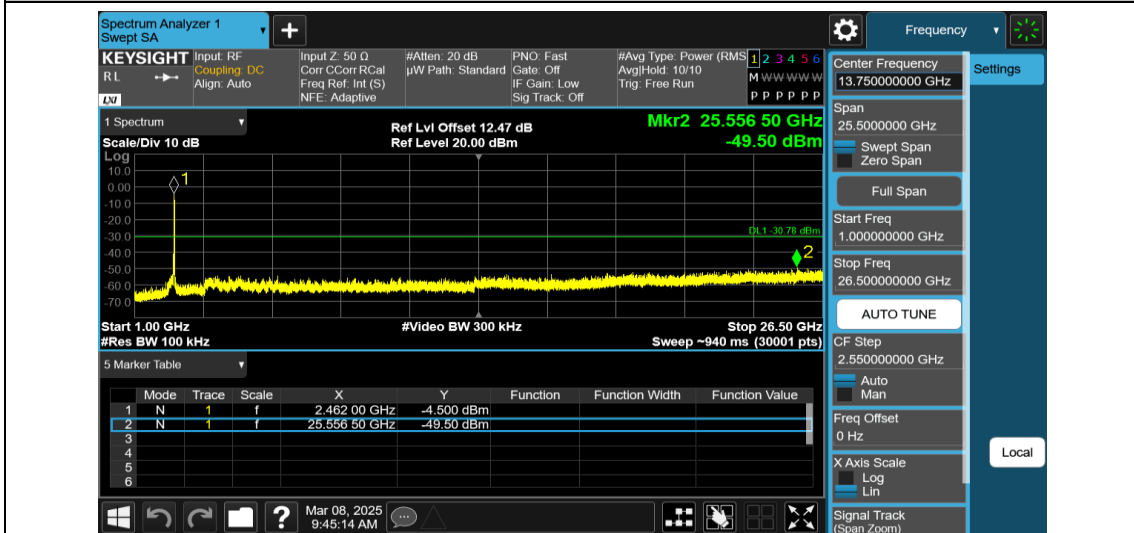
11AX20MIMO-Ant1-2462-242Tone-RU61-1000~26500-PASS
