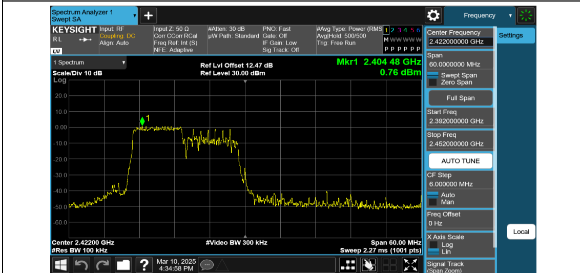
11AX40MIMO-Ant1-2422-106Tone-RU53-0~Reference-PASS
