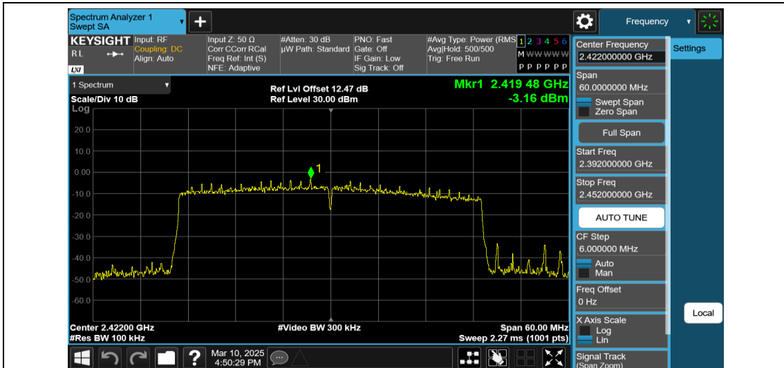
11AX40MIMO-Ant1-2422-484Tone-RU65-0~Reference-PASS
