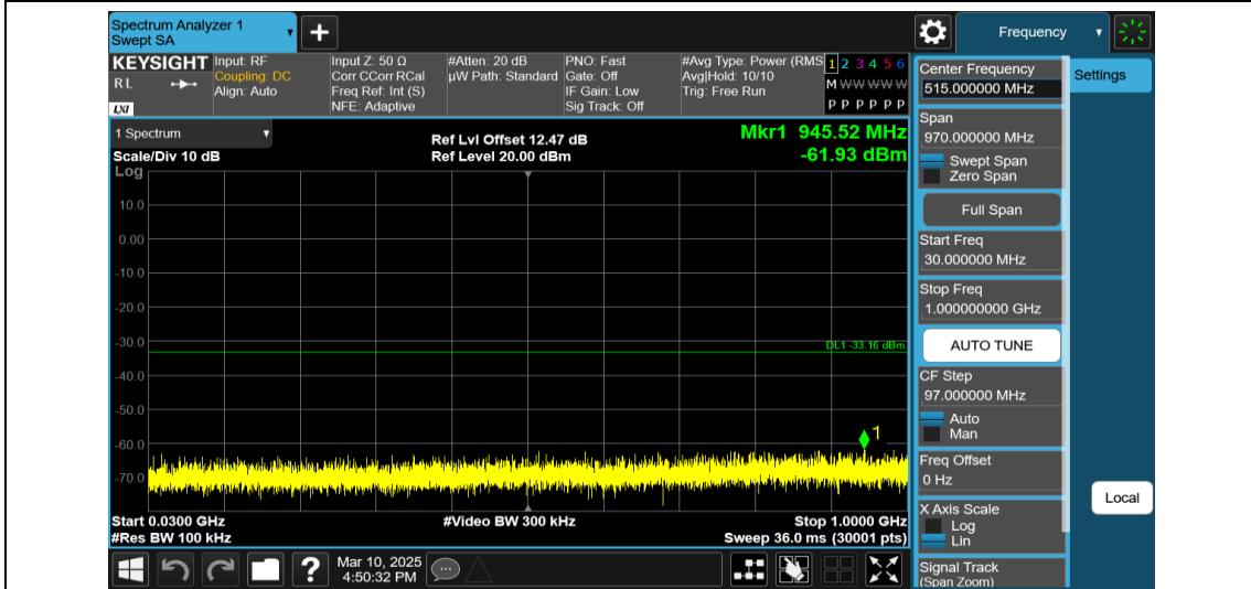
11AX40MIMO-Ant1-2422-484Tone-RU65-30~1000-PASS
