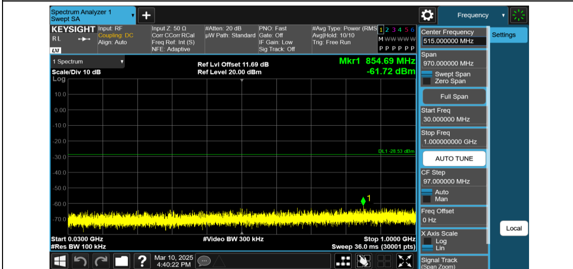
11AX40MIMO-Ant2-2422-106Tone-RU53-30~1000-PASS
