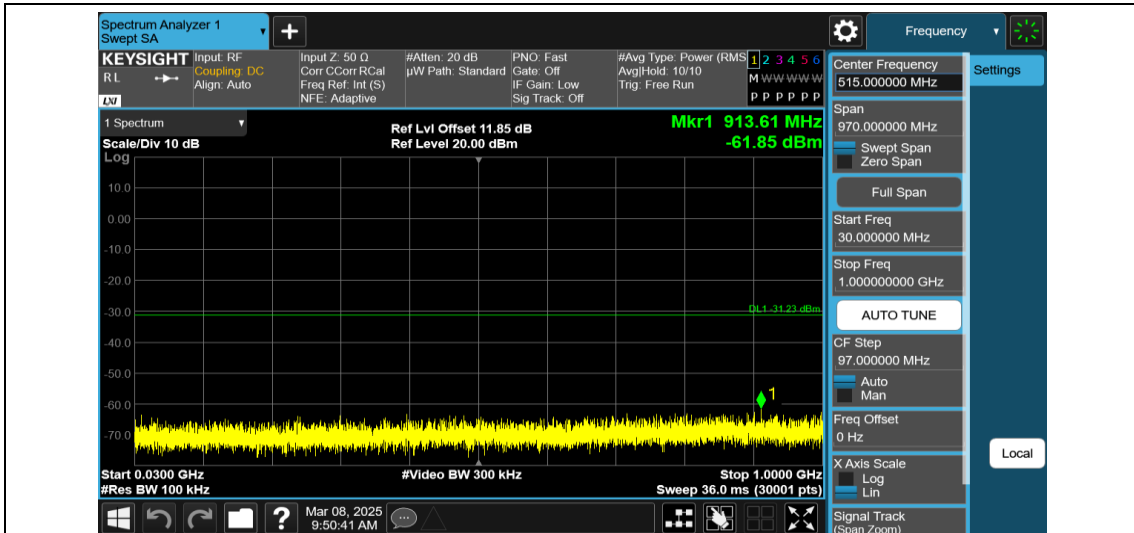
11AX20MIMO-Ant2-2462-242Tone-RU61-30~1000-PASS
