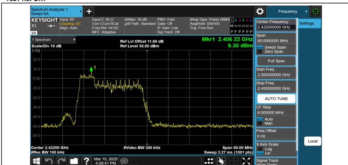
11AX40MIMO-Ant2-2422-52Tone-RU37-0~Reference-PASS
