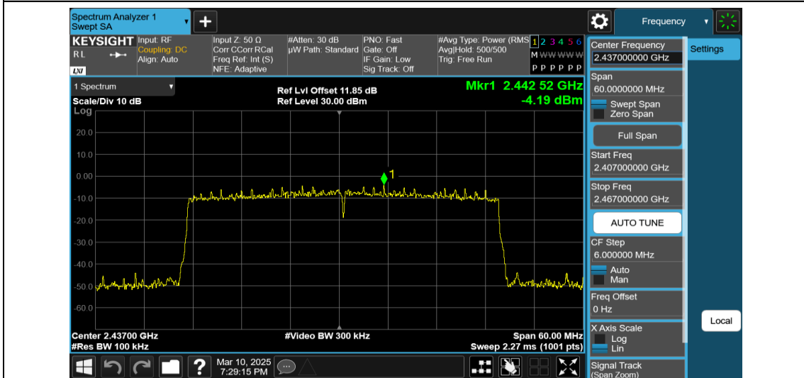
11AX40MIMO-Ant2-2437-484Tone-RU65-0~Reference-PASS
