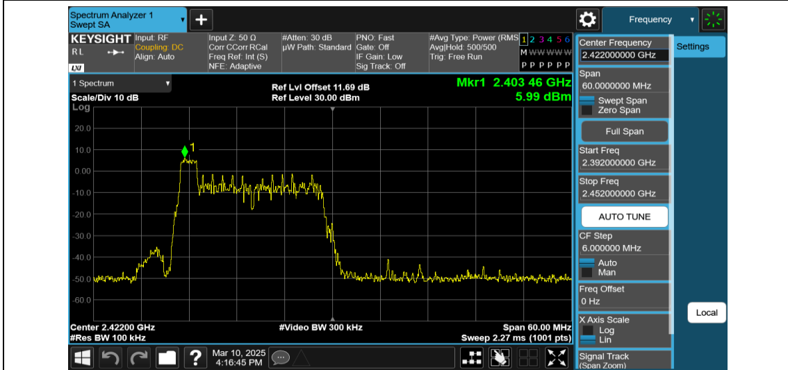
11AX40MIMO-Ant2-2422-26Tone-RU0-0~Reference-PASS
