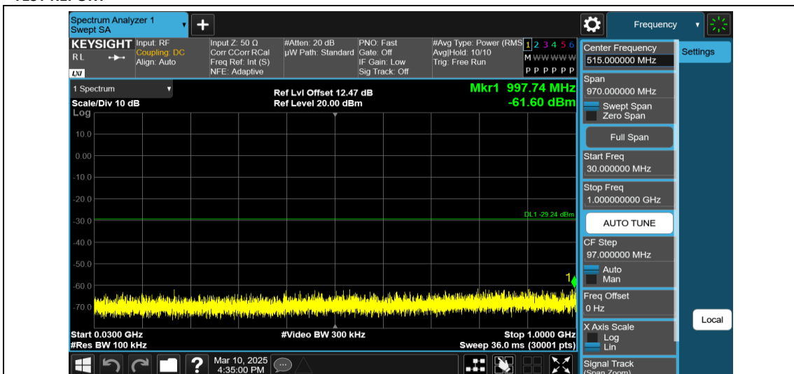
11AX40MIMO-Ant1-2422-106Tone-RU53-30~1000-PASS
