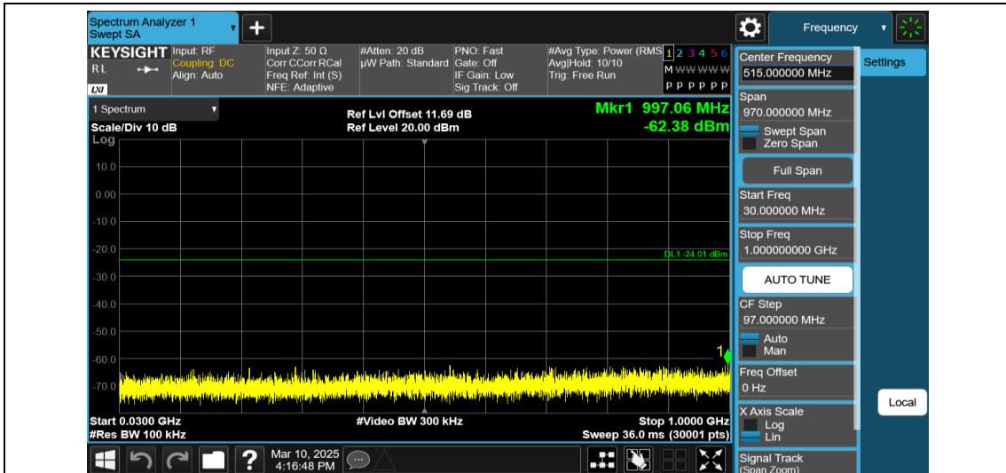
11AX40MIMO-Ant2-2422-26Tone-RU0-30~1000-PASS
