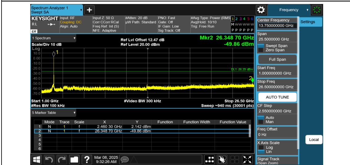
11AX20MIMO-Ant1-2462-106Tone-RU53-1000~26500-PASS
