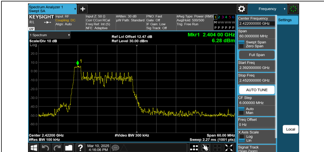
11AX40MIMO-Ant1-2422-26Tone-RU0-0~Reference-PASS
