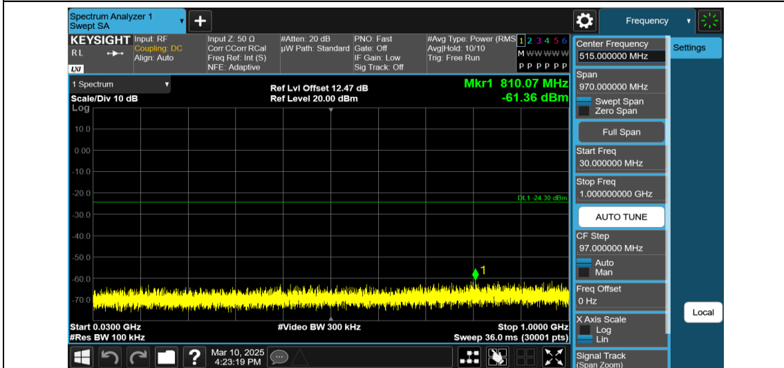
11AX40MIMO-Ant1-2422-52Tone-RU37-30~1000-PASS
