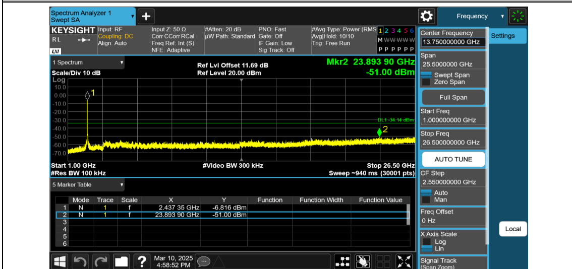
11AX40MIMO-Ant2-2422-484Tone-RU65-1000~26500-PASS
