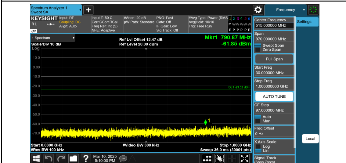
11AX40MIMO-Ant1-2437-26Tone-RU0-30~1000-PASS
