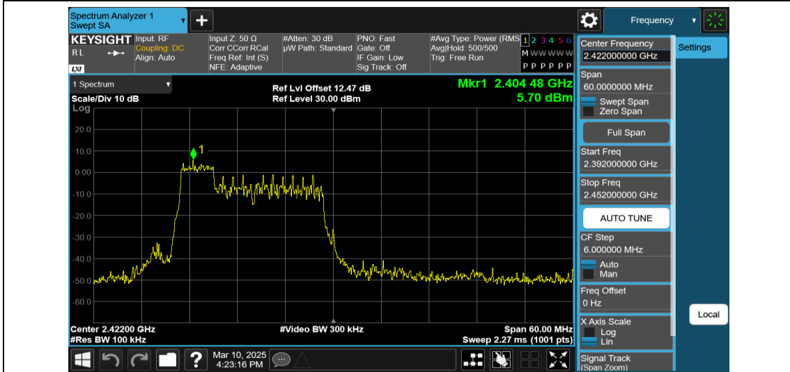
11AX40MIMO-Ant1-2422-52Tone-RU37-0~Reference-PASS
