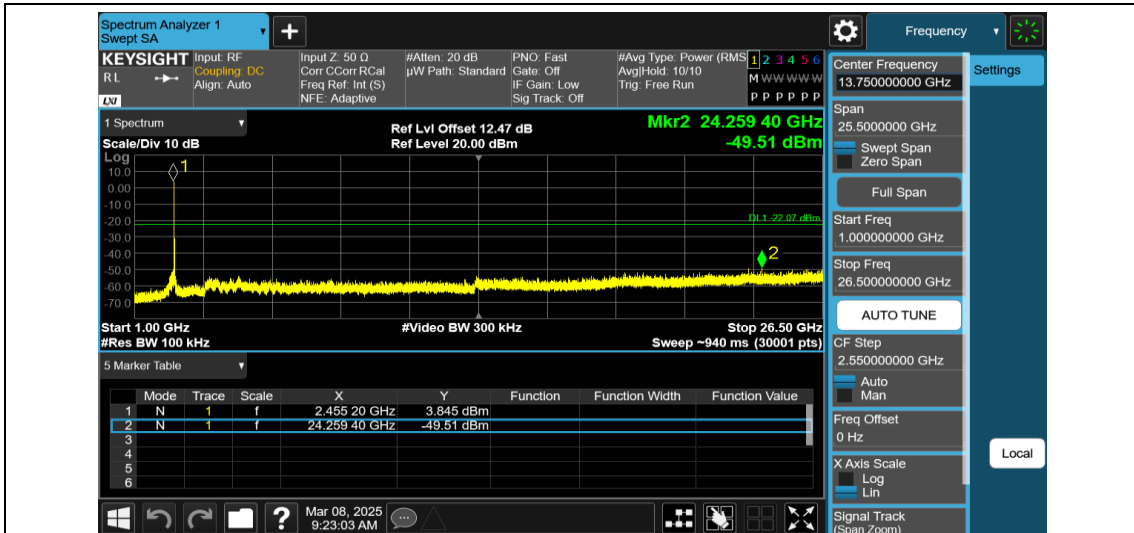
11AX20MIMO-Ant1-2462-52Tone-RU37-1000~26500-PASS
