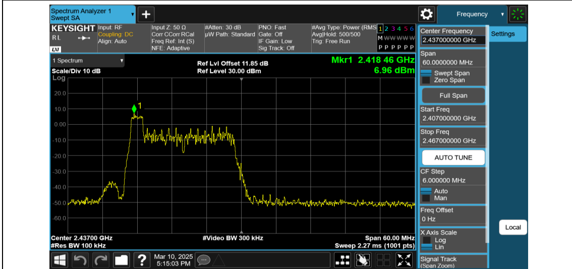
11AX40MIMO-Ant2-2437-26Tone-RU0-0~Reference-PASS
