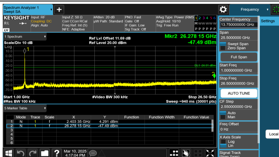
11AX40MIMO-Ant2-2422-26Tone-RU0-1000~26500-PASS
