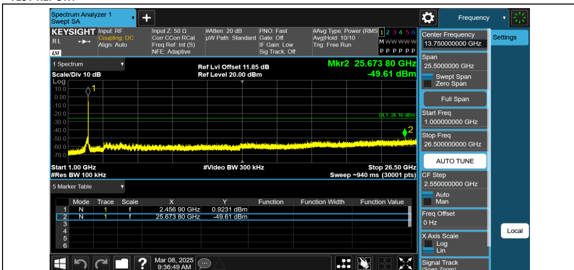
11AX20MIMO-Ant2-2462-106Tone-RU53-1000~26500-PASS
