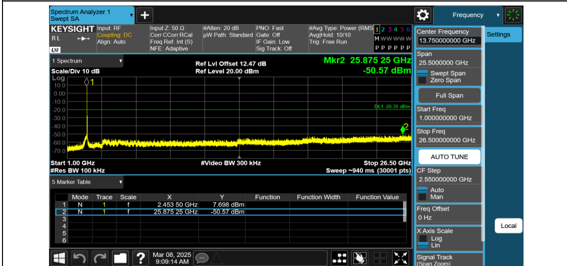
11AX20MIMO-Ant1-2462-26Tone-RU0-1000~26500-PASS
