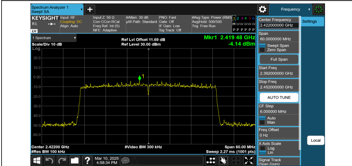
11AX40MIMO-Ant2-2422-484Tone-RU65-0~Reference-PASS
