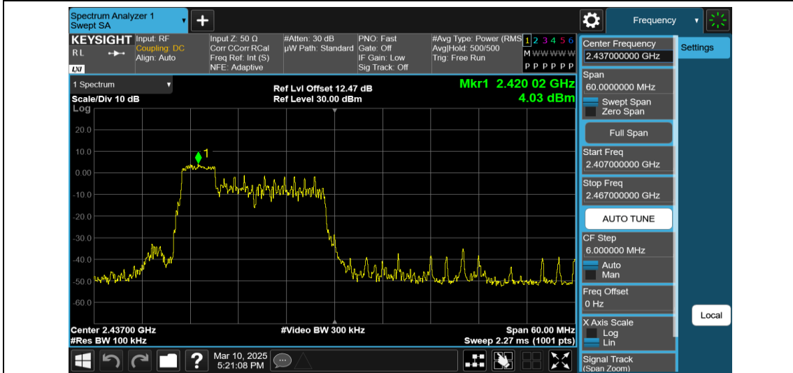
11AX40MIMO-Ant1-2437-52Tone-RU37-0~Reference-PASS
