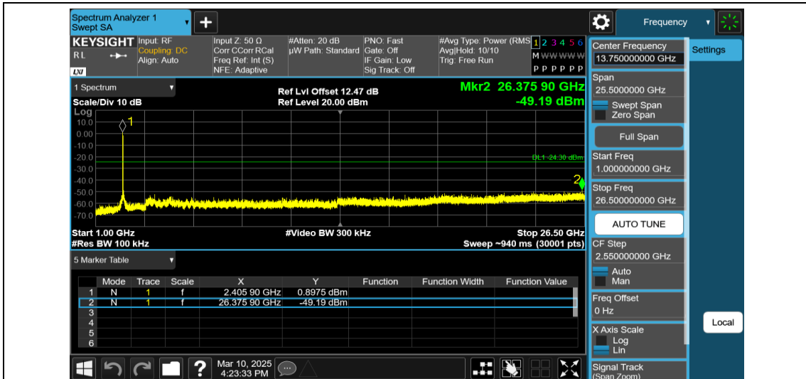
11AX40MIMO-Ant1-2422-52Tone-RU37-1000~26500-PASS
