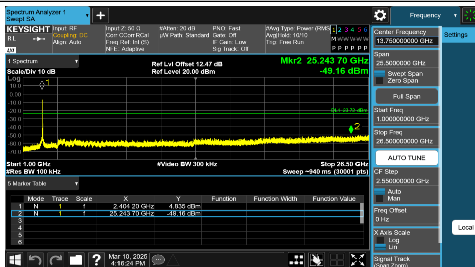
11AX40MIMO-Ant1-2422-26Tone-RU0-1000~26500-PASS
