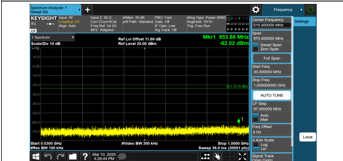
11AX40MIMO-Ant2-2422-52Tone-RU37-30~1000-PASS
