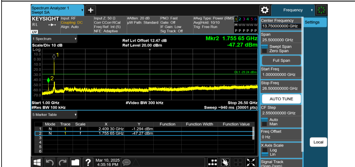
11AX40MIMO-Ant1-2422-106Tone-RU53-1000~26500-PASS
