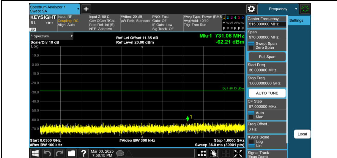
11AX20MIMO-Ant2-2437-106Tone-RU53-30~1000-PASS
