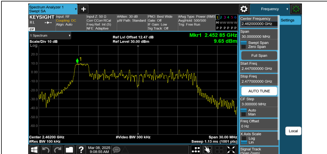
11AX20MIMO-Ant1-2462-26Tone-RU0-0~Reference-PASS
