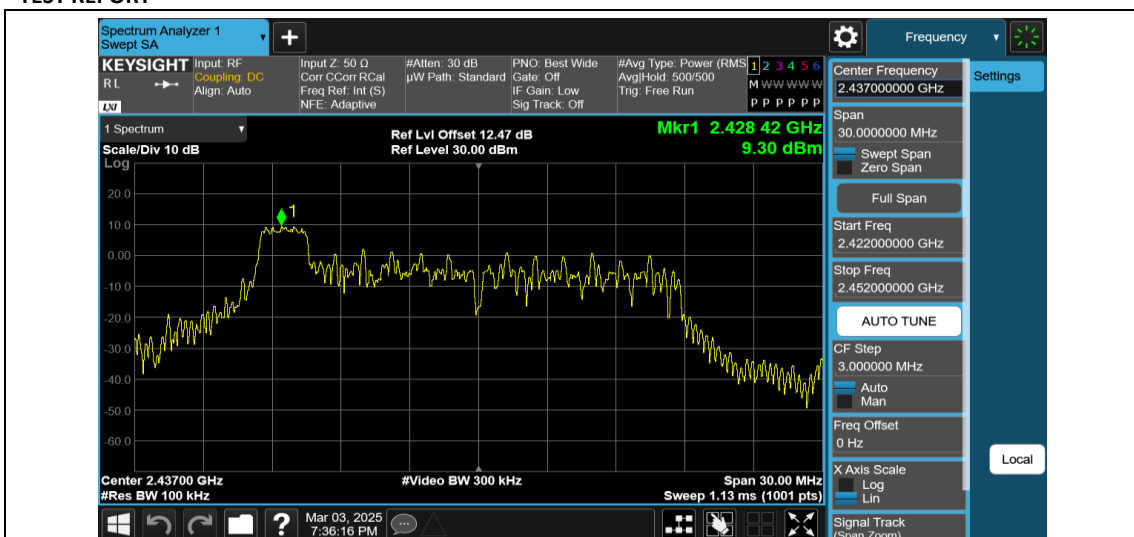
11AX20MIMO-Ant1-2437-26Tone-RU0-0~Reference-PASS
