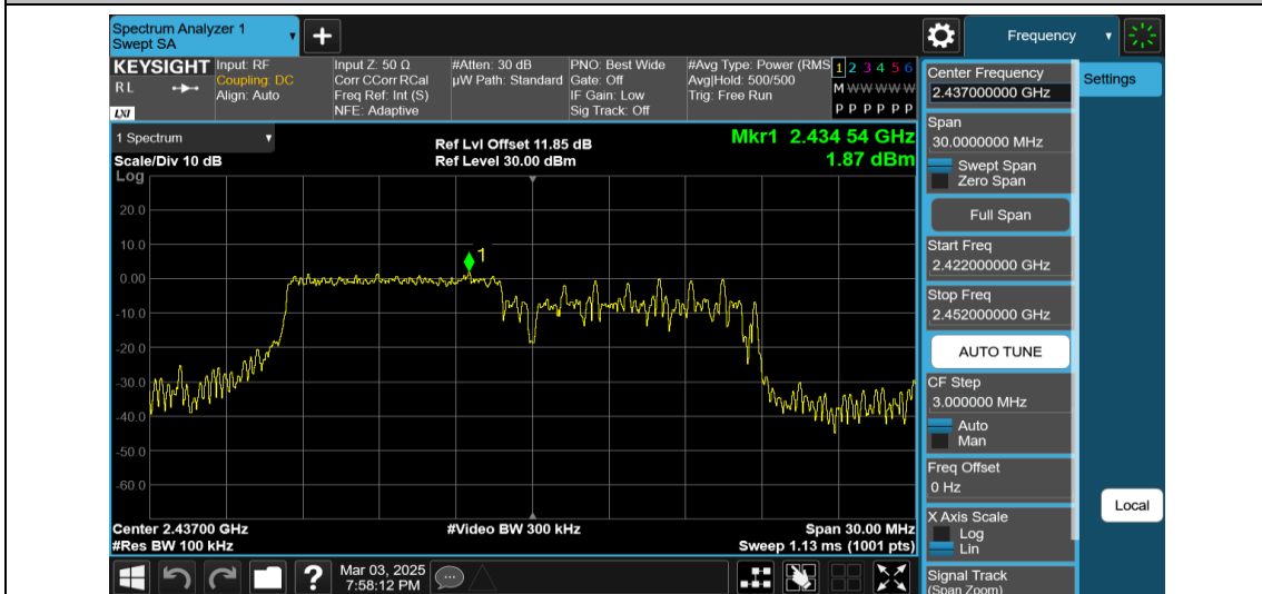
11AX20MIMO-Ant2-2437-106Tone-RU53-0~Reference-PASS
