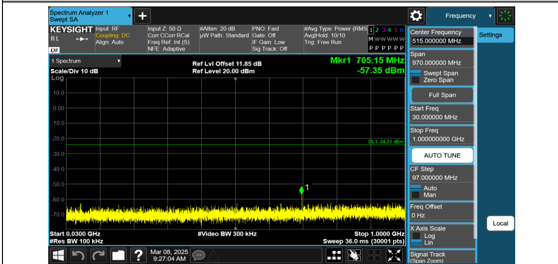
11AX20MIMO-Ant2-2462-52Tone-RU37-30~1000-PASS
