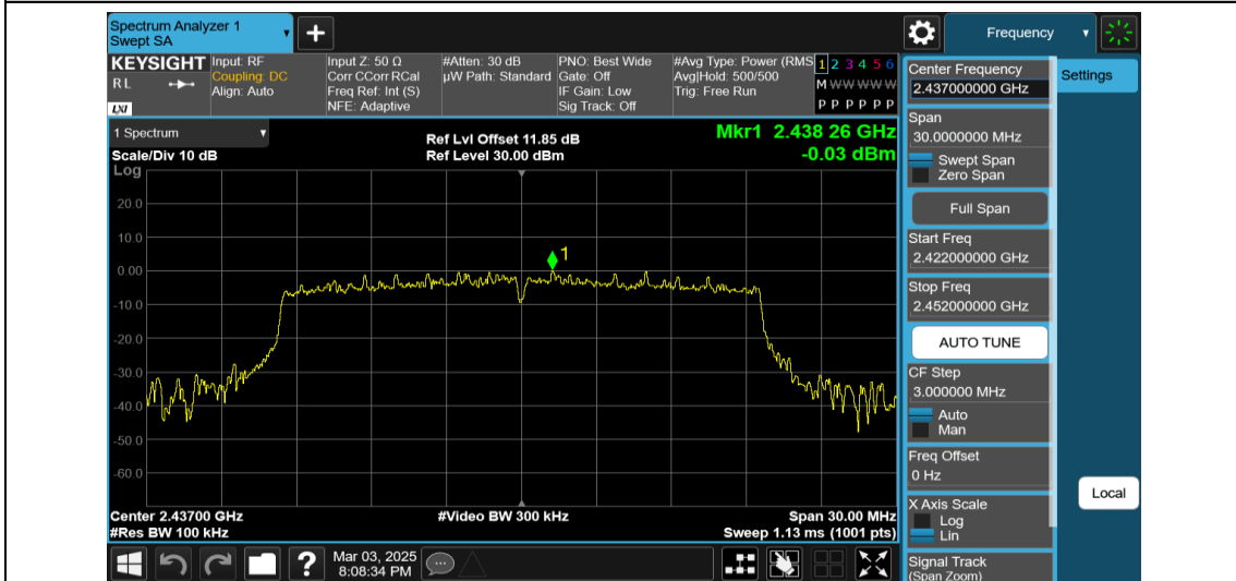
11AX20MIMO-Ant2-2437-242Tone-RU61-0~Reference-PASS
