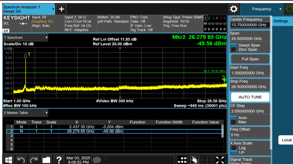
11AX20MIMO-Ant2-2437-242Tone-RU61-1000~26500-PASS
