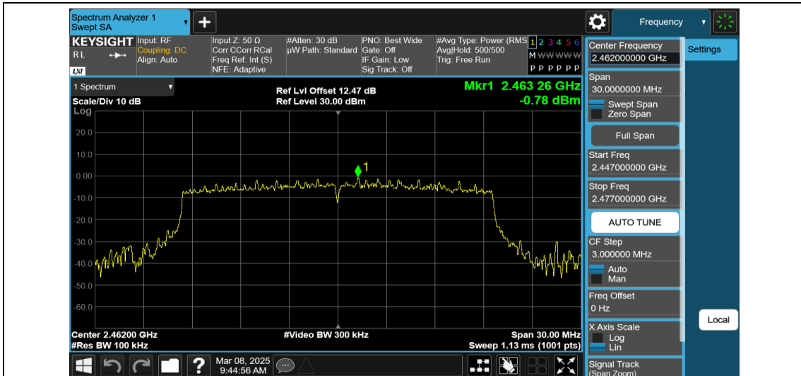
11AX20MIMO-Ant1-2462-242Tone-RU61-0~Reference-PASS
