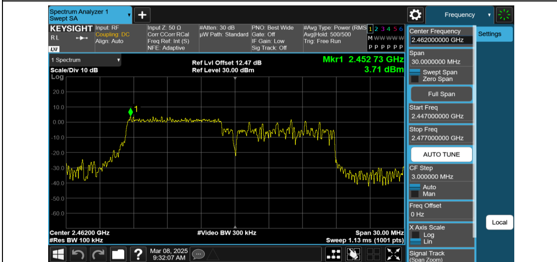
11AX20MIMO-Ant1-2462-106Tone-RU53-0~Reference-PASS
