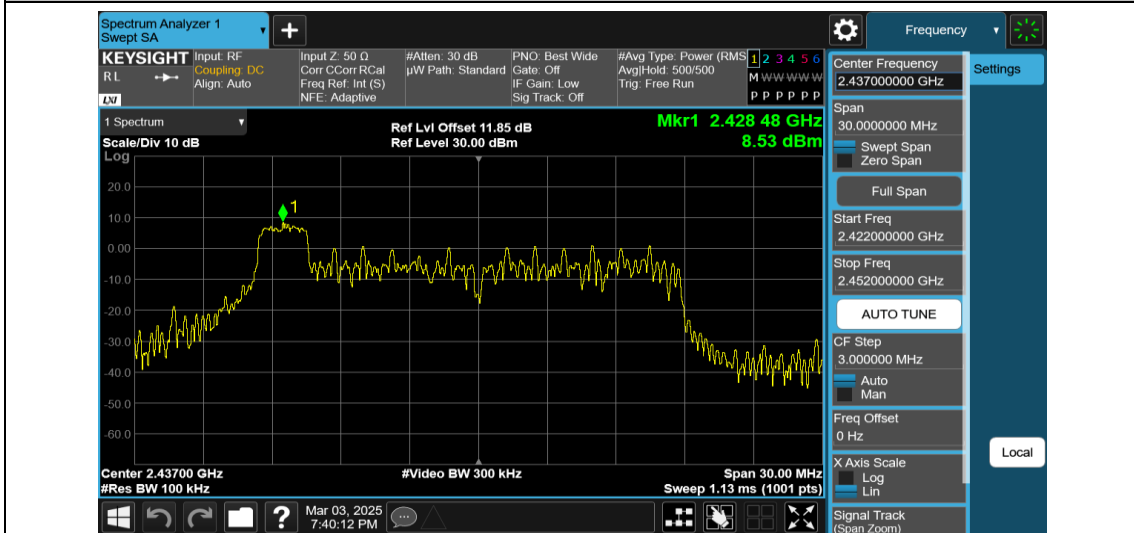
11AX20MIMO-Ant2-2437-26Tone-RU0-0~Reference-PASS
