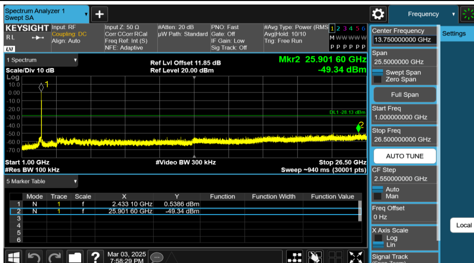
11AX20MIMO-Ant2-2437-106Tone-RU53-1000~26500-PASS
