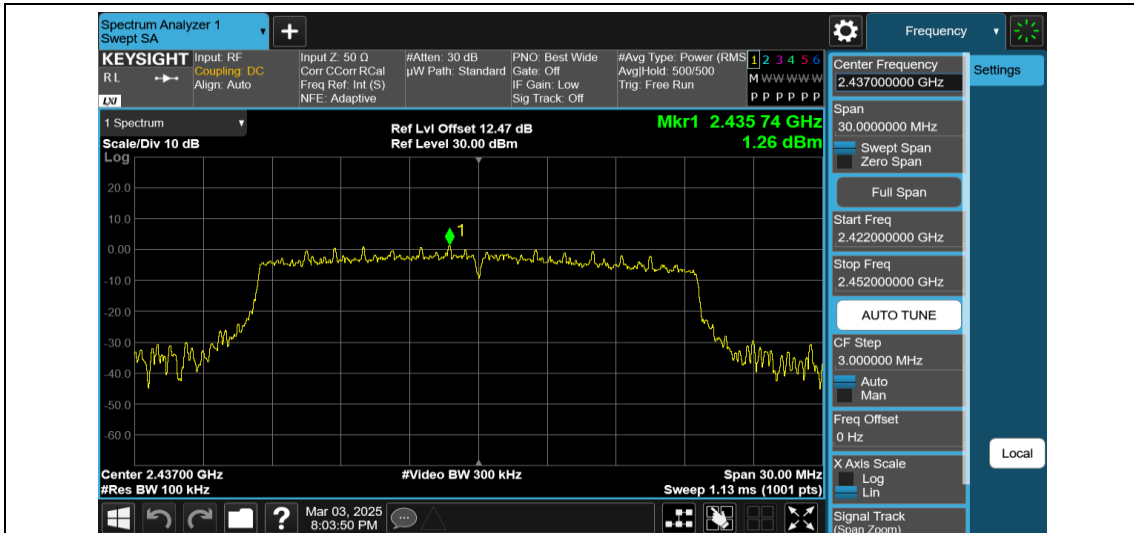
11AX20MIMO-Ant1-2437-242Tone-RU61-0~Reference-PASS
