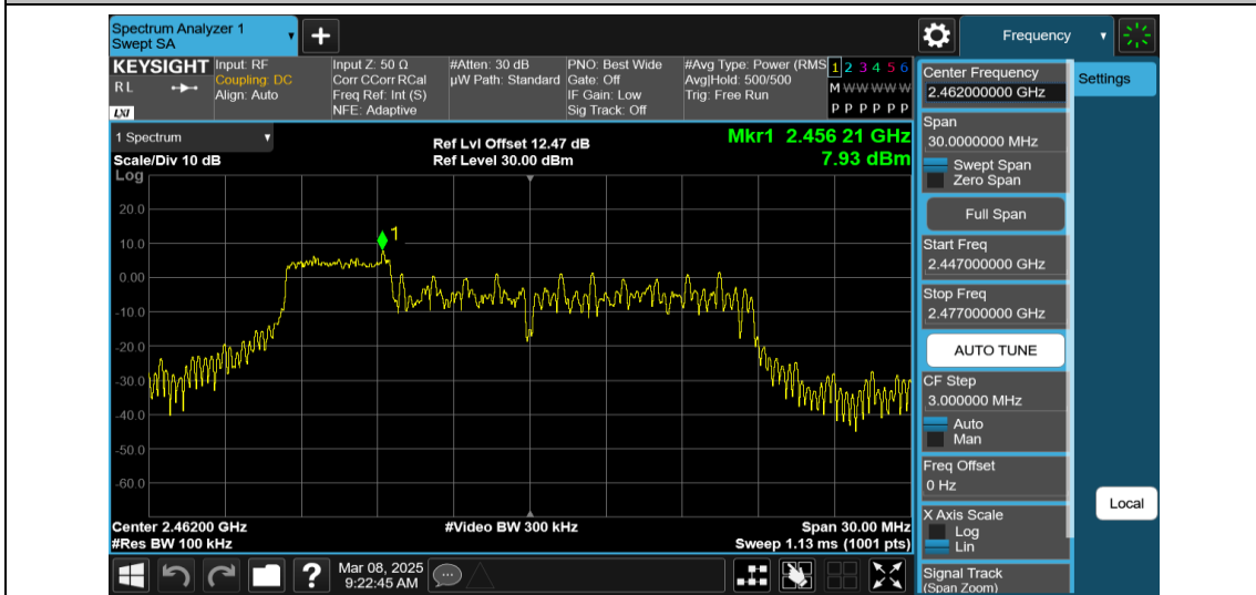
11AX20MIMO-Ant1-2462-52Tone-RU37-0~Reference-PASS
