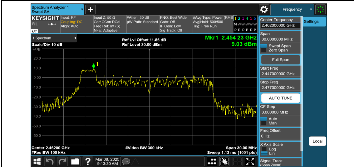
11AX20MIMO-Ant2-2462-26Tone-RU0-0~Reference-PASS
