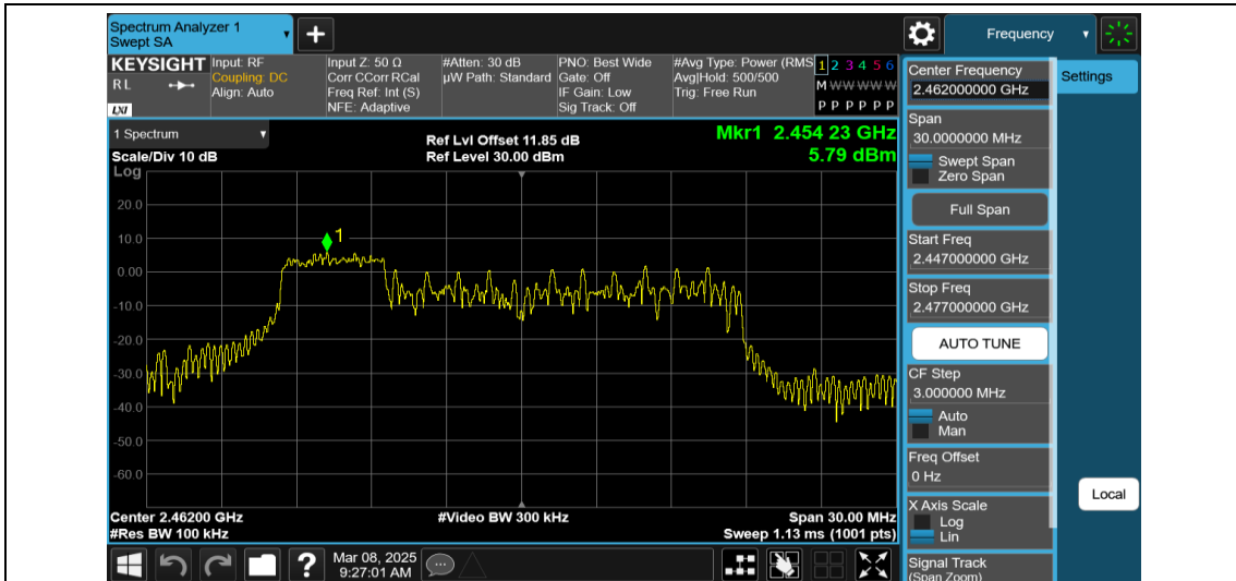
11AX20MIMO-Ant2-2462-52Tone-RU37-0~Reference-PASS
