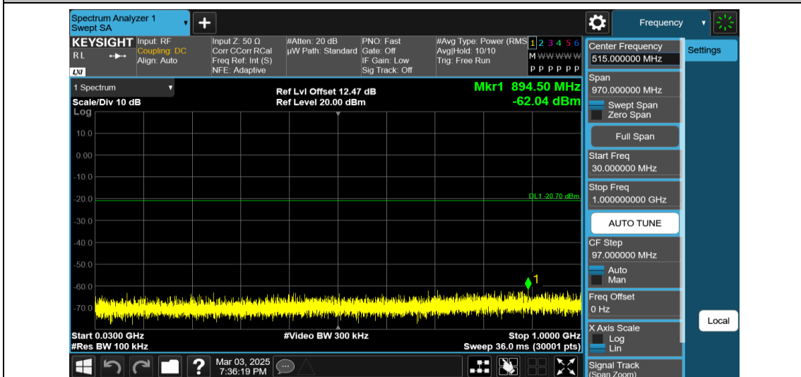
11AX20MIMO-Ant1-2437-26Tone-RU0-30~1000-PASS
