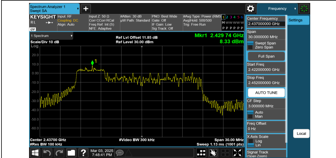
11AX20MIMO-Ant2-2437-52Tone-RU37-0~Reference-PASS
