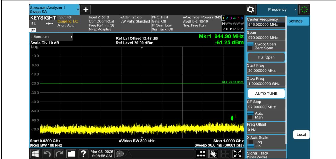
11AX20MIMO-Ant1-2462-26Tone-RU0-30~1000-PASS
