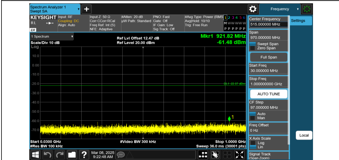
11AX20MIMO-Ant1-2462-52Tone-RU37-30~1000-PASS
