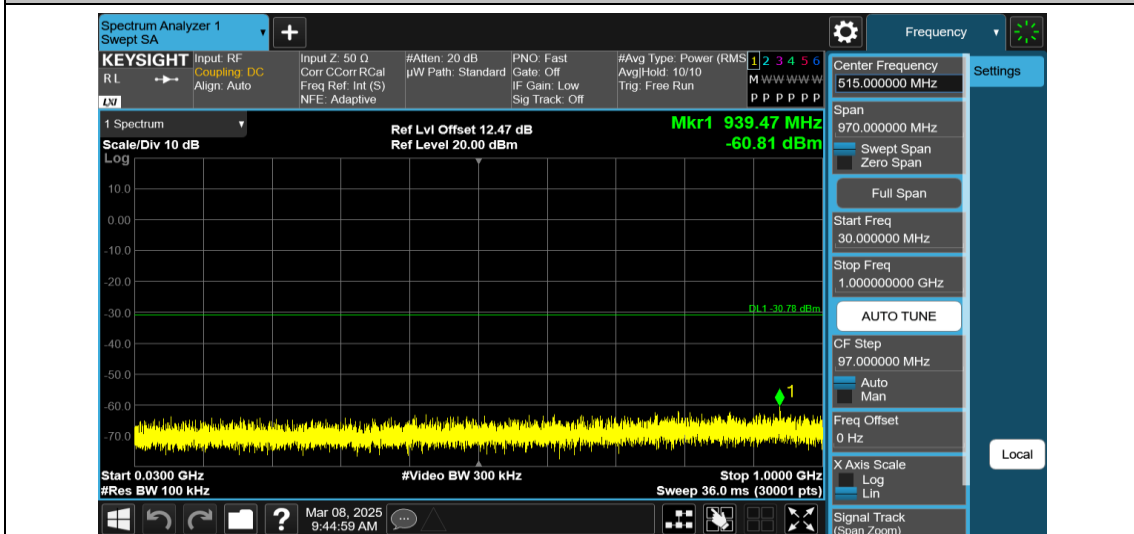
11AX20MIMO-Ant1-2462-242Tone-RU61-30~1000-PASS
