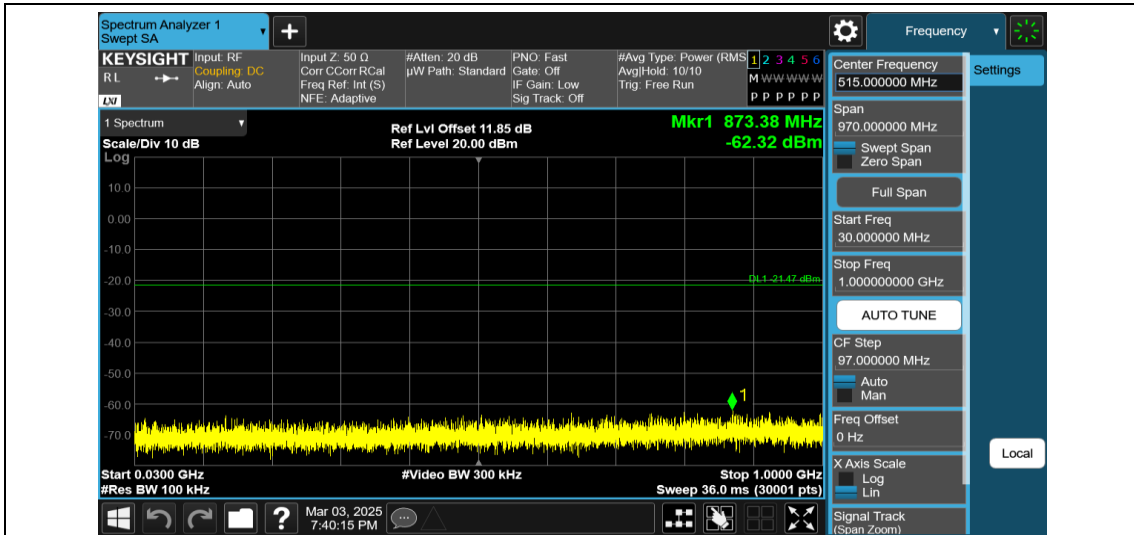
11AX20MIMO-Ant2-2437-26Tone-RU0-30~1000-PASS
