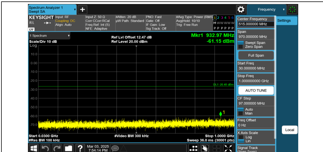
11AX20MIMO-Ant1-2437-106Tone-RU53-30~1000-PASS
