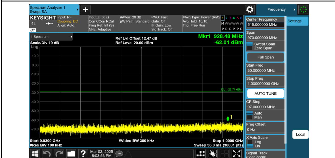
11AX20MIMO-Ant1-2437-242Tone-RU61-30~1000-PASS
