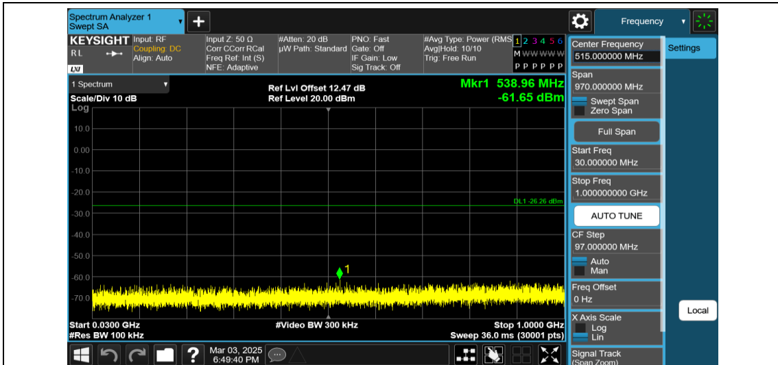
11AX20MIMO-Ant1-2412-242Tone-RU61-30~1000-PASS
