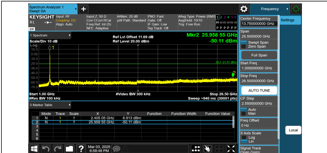
11AX20MIMO-Ant2-2412-52Tone-RU37-1000~26500-PASS
