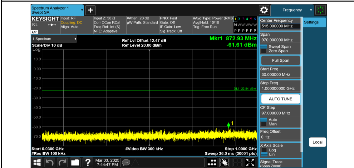
11AX20MIMO-Ant1-2437-52Tone-RU37-30~1000-PASS
