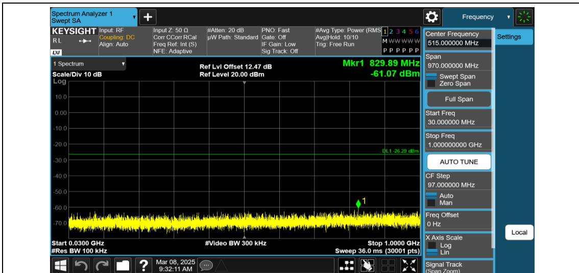
11AX20MIMO-Ant1-2462-106Tone-RU53-30~1000-PASS
