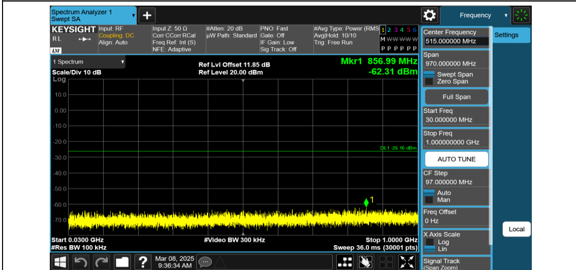
11AX20MIMO-Ant2-2462-106Tone-RU53-30~1000-PASS
