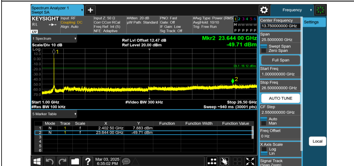
11AX20MIMO-Ant1-2412-26Tone-RU0-1000~26500-PASS
