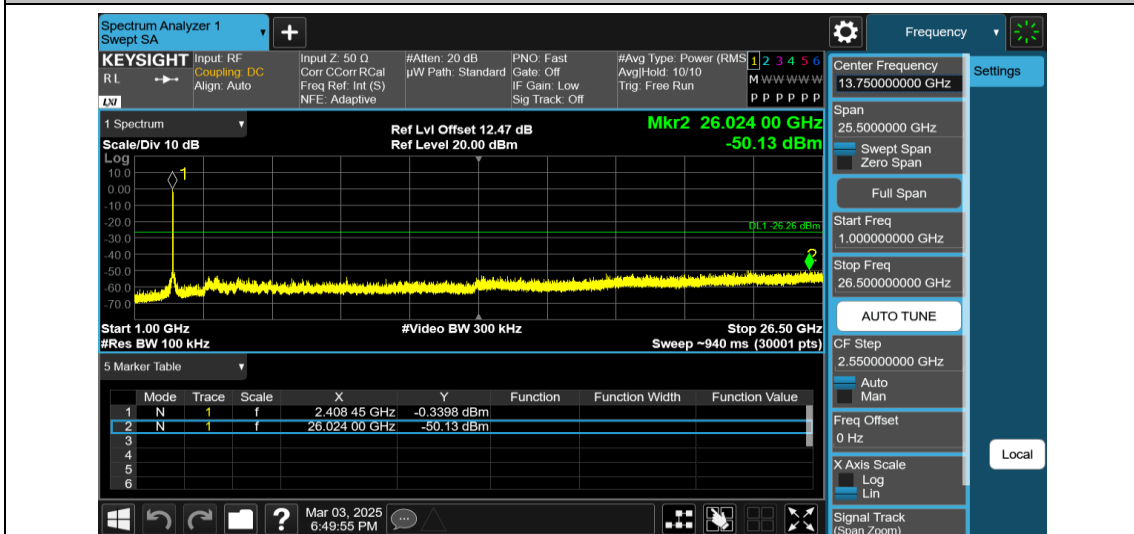
11AX20MIMO-Ant1-2412-242Tone-RU61-1000~26500-PASS
