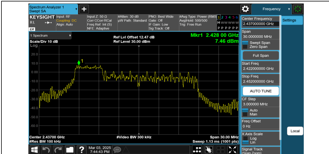
11AX20MIMO-Ant1-2437-52Tone-RU37-0~Reference-PASS
