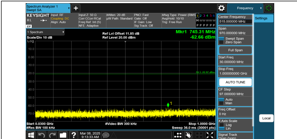
11AX20MIMO-Ant2-2462-26Tone-RU0-30~1000-PASS
