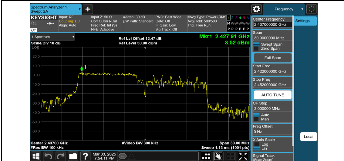
11AX20MIMO-Ant1-2437-106Tone-RU53-0~Reference-PASS
