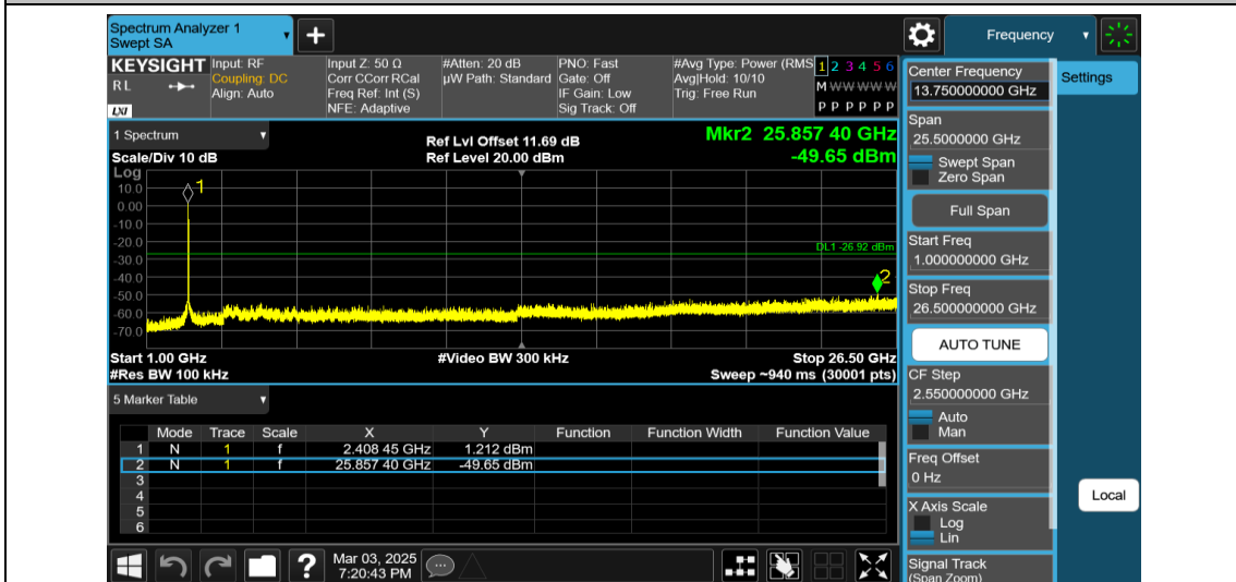
11AX20MIMO-Ant2-2412-106Tone-RU53-1000~26500-PASS
