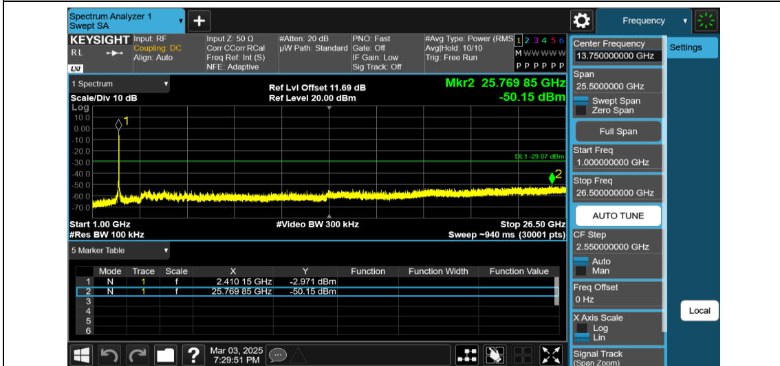
11AX20MIMO-Ant2-2412-242Tone-RU61-1000~26500-PASS
