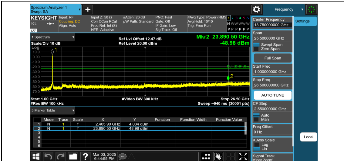
11AX20MIMO-Ant1-2412-106Tone-RU53-1000~26500-PASS
