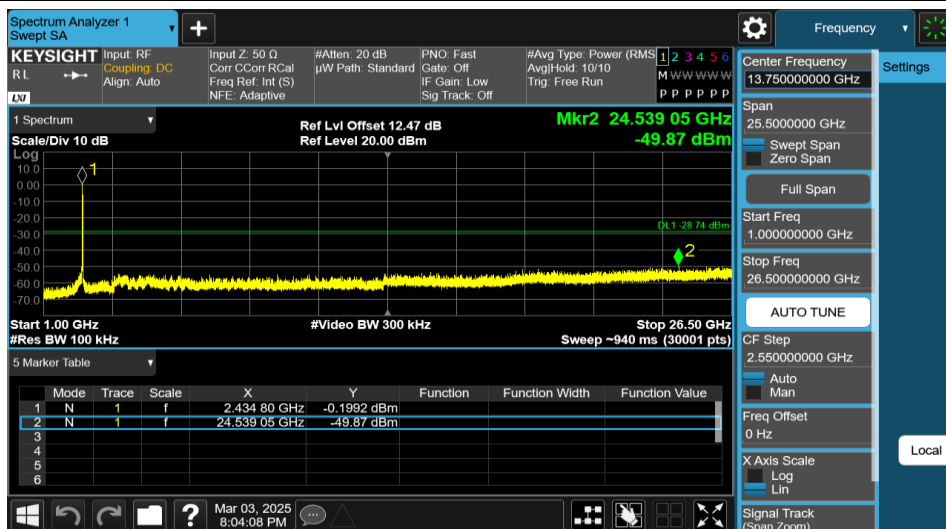
11AX20MIMO-Ant1-2437-242Tone-RU61-1000~26500-PASS
