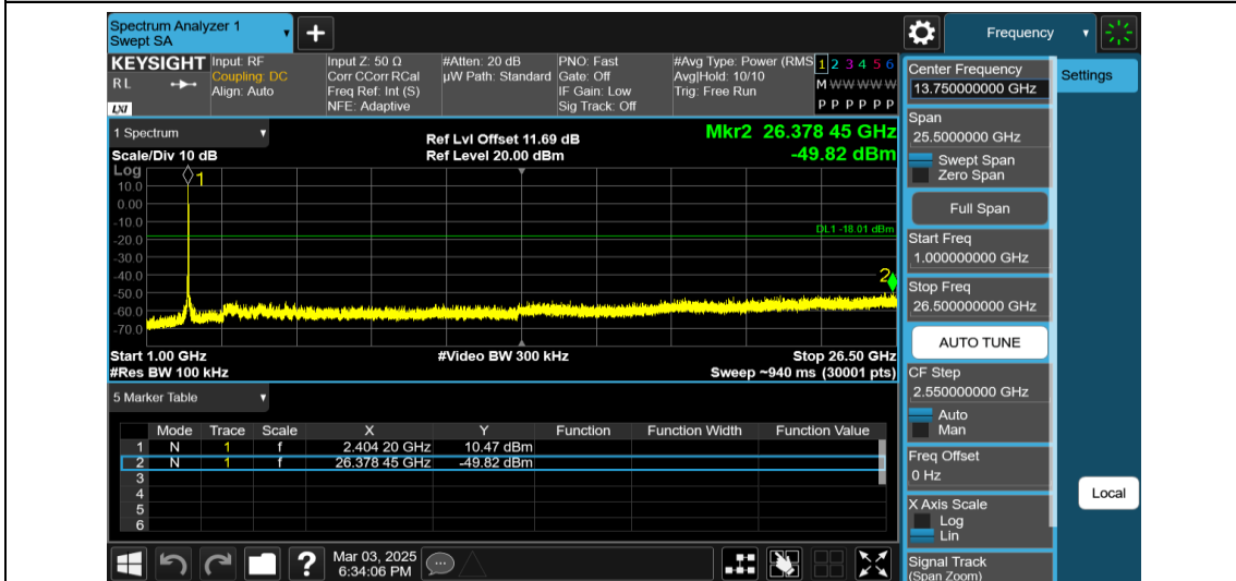
11AX20MIMO-Ant2-2412-26Tone-RU0-1000~26500-PASS
