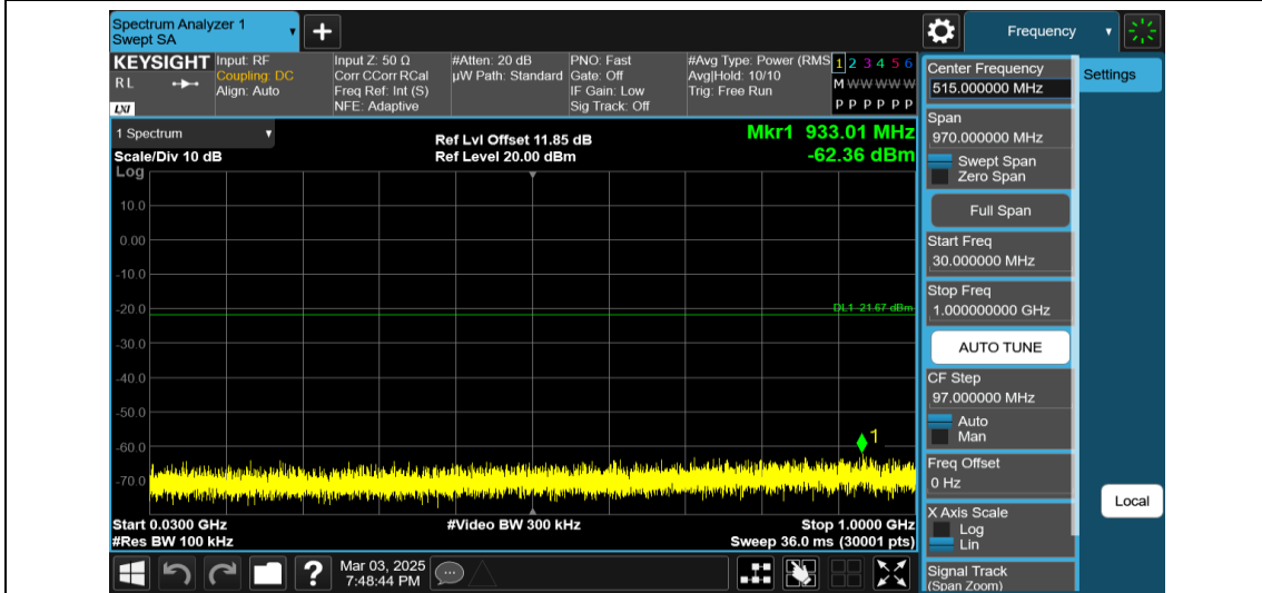
11AX20MIMO-Ant2-2437-52Tone-RU37-30~1000-PASS
