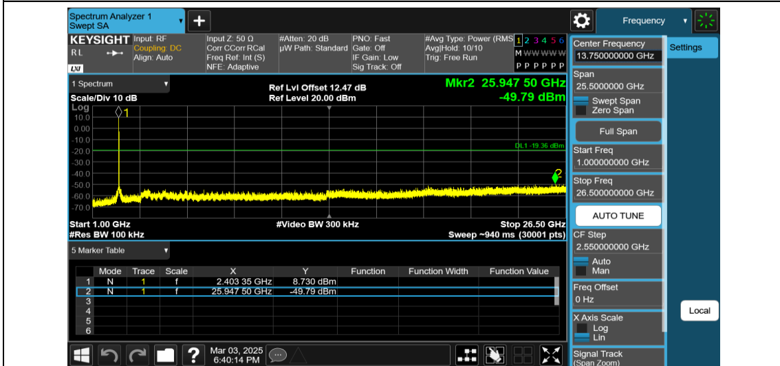
11AX20MIMO-Ant1-2412-52Tone-RU37-1000~26500-PASS
