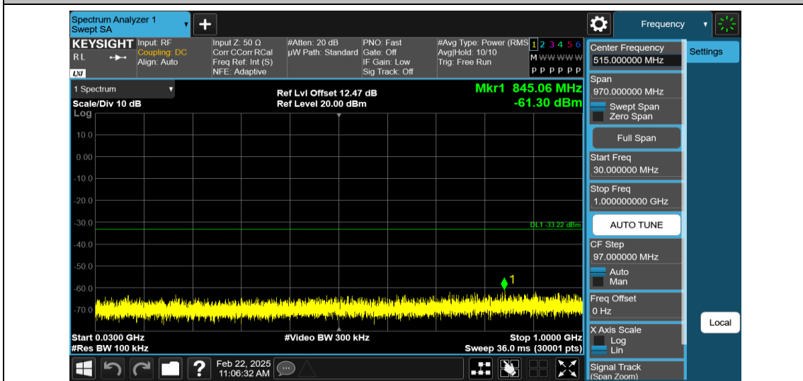
11AX40MIMO-Ant1-2437-30~1000-PASS
