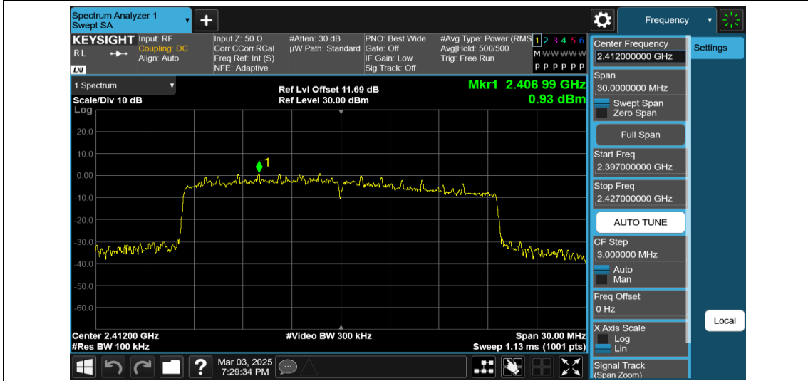
11AX20MIMO-Ant2-2412-242Tone-RU61-0~Reference-PASS
