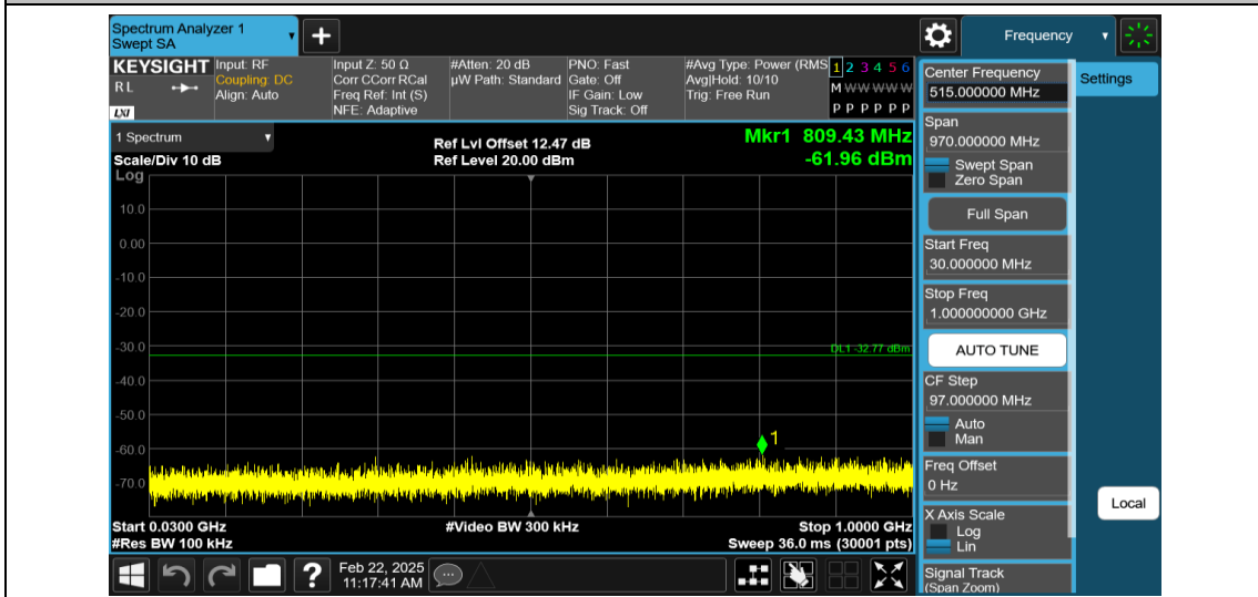
11AX40MIMO-Ant1-2452-30~1000-PASS
