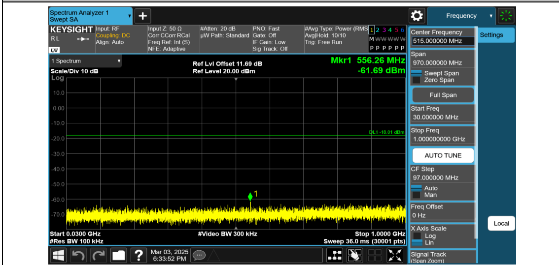
11AX20MIMO-Ant2-2412-26Tone-RU0-30~1000-PASS
