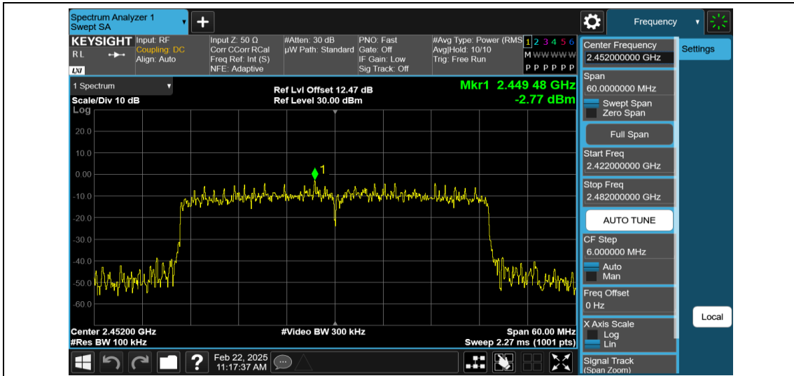
11AX40MIMO-Ant1-2452-0~Reference-PASS
