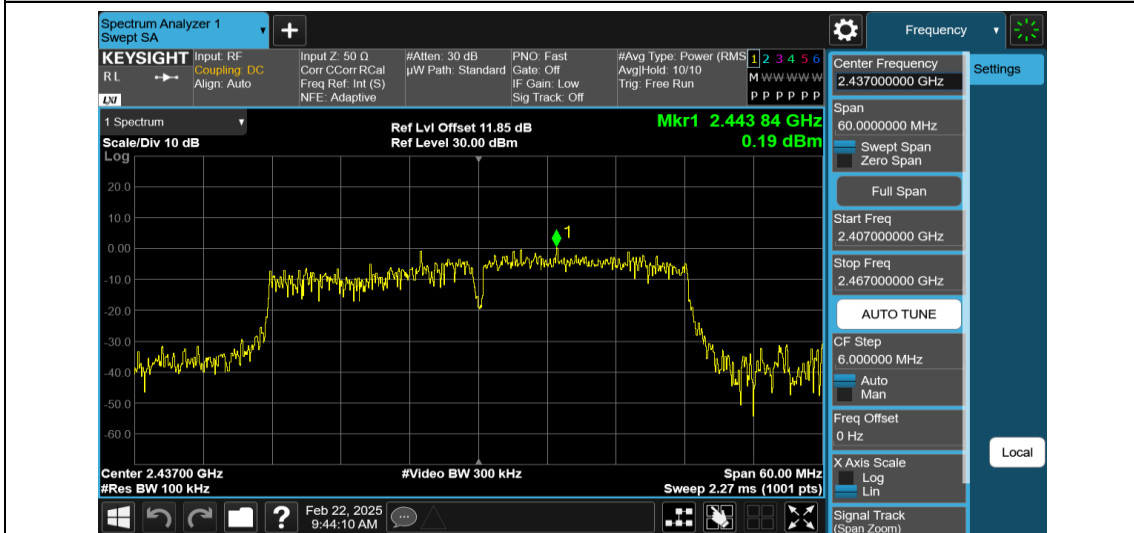
11N40MIMO-Ant2-2437-0~Reference-PASS
