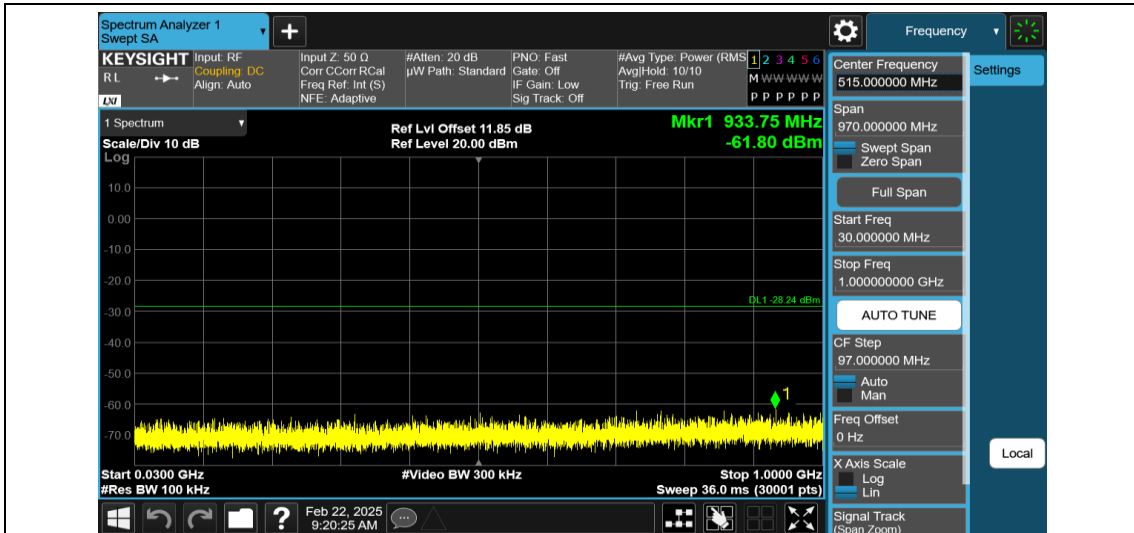
11N20MIMO-Ant2-2462-30~1000-PASS
