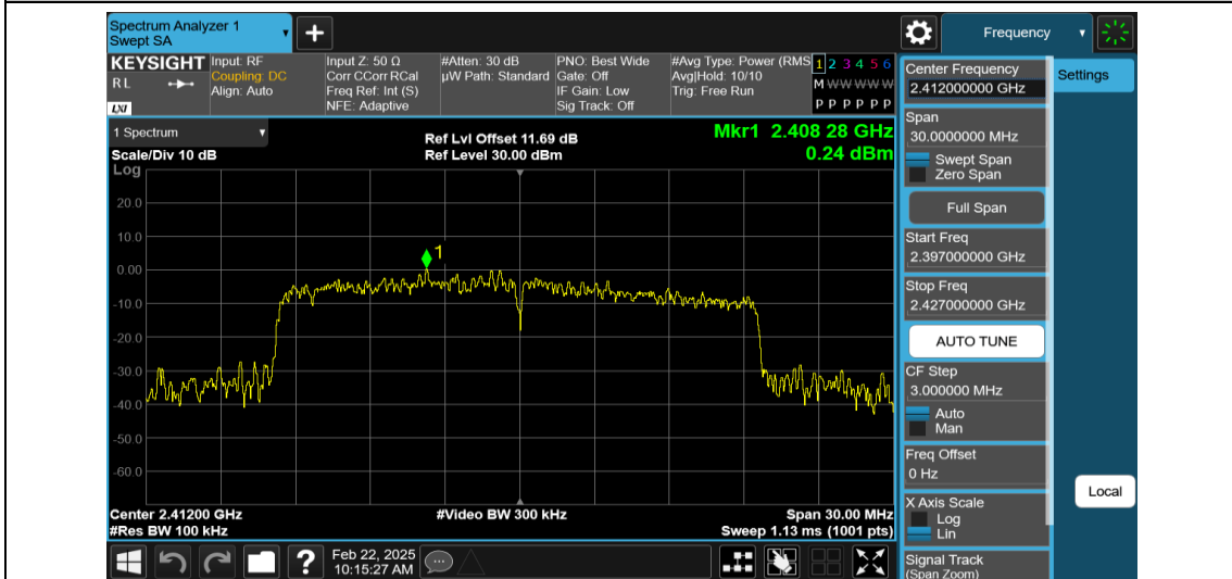
11AX20MIMO-Ant2-2412-0~Reference-PASS
