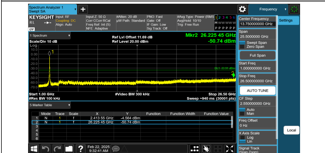
11N40MIMO-Ant2-2422-1000~26500-PASS
