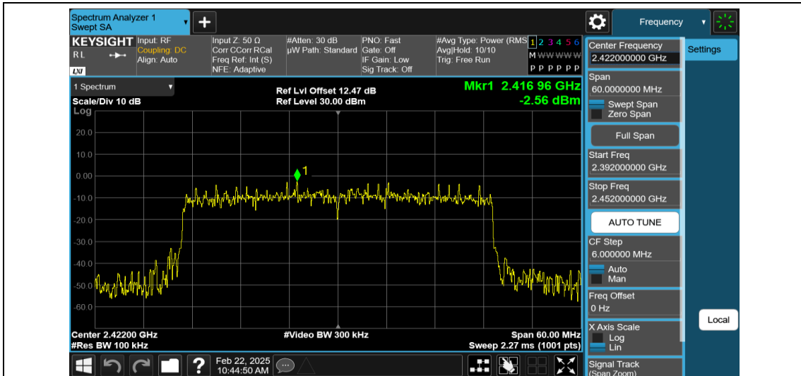
11AX40MIMO-Ant1-2422-0~Reference-PASS
