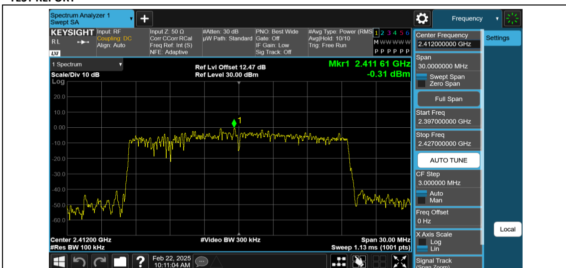
11AX20MIMO-Ant1-2412-0~Reference-PASS
