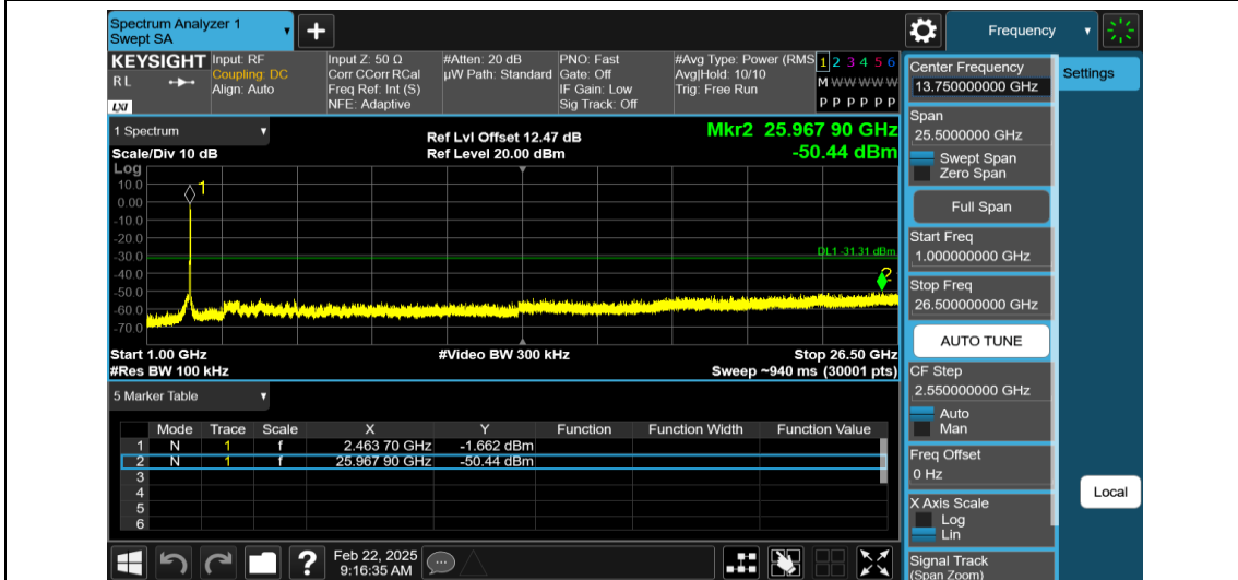
11N20MIMO-Ant1-2462-1000~26500-PASS
