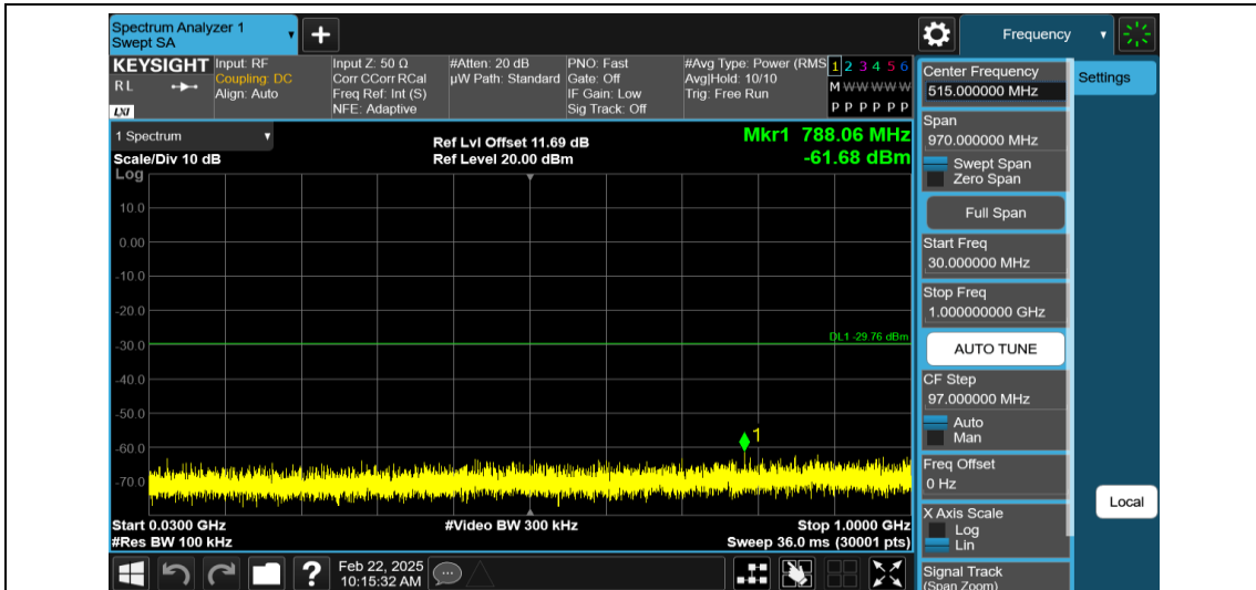
11AX20MIMO-Ant2-2412-30~1000-PASS
