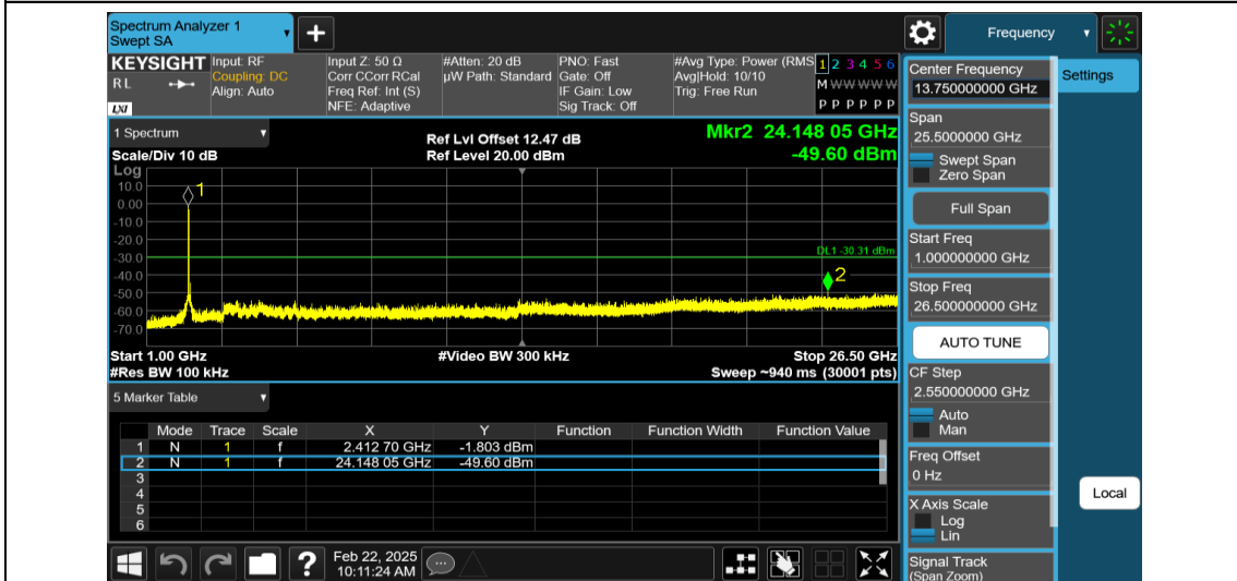
11AX20MIMO-Ant1-2412-1000~26500-PASS
