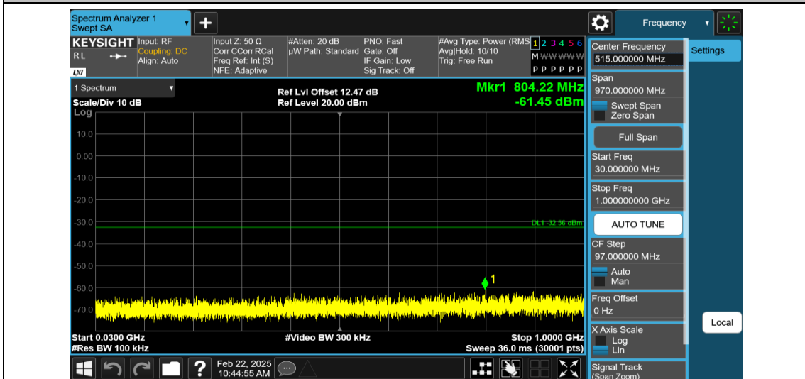
11AX40MIMO-Ant1-2422-30~1000-PASS
