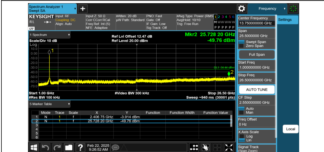
11N40MIMO-Ant1-2422-1000~26500-PASS
