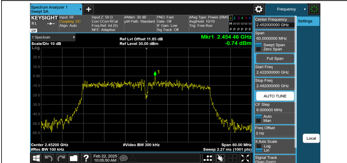
11N40MIMO-Ant2-2452-0~Reference-PASS
