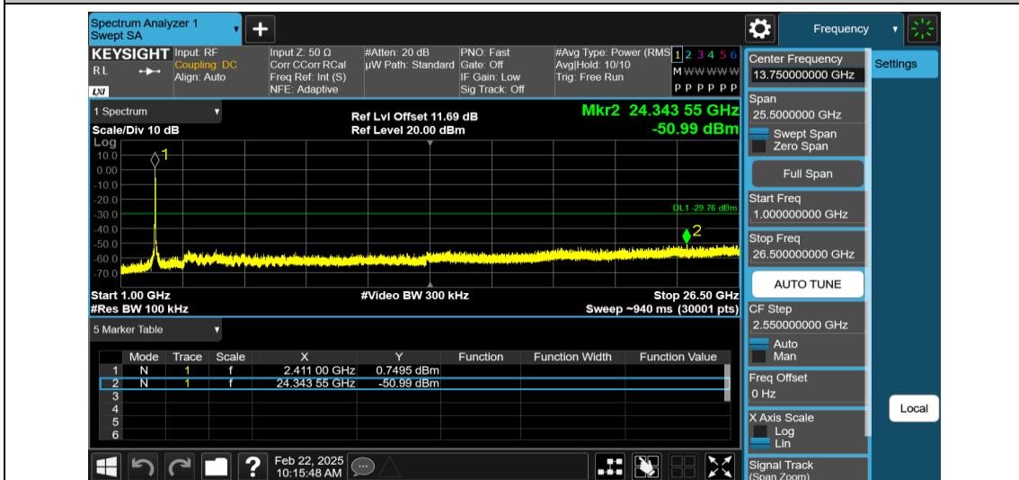
11AX20MIMO-Ant2-2412-1000~26500-PASS
