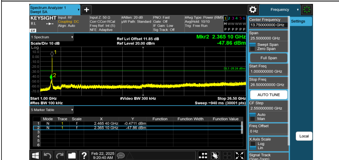
11N20MIMO-Ant2-2462-1000~26500-PASS
