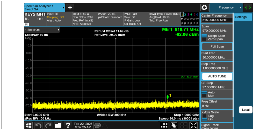
11N40MIMO-Ant2-2422-30~1000-PASS
