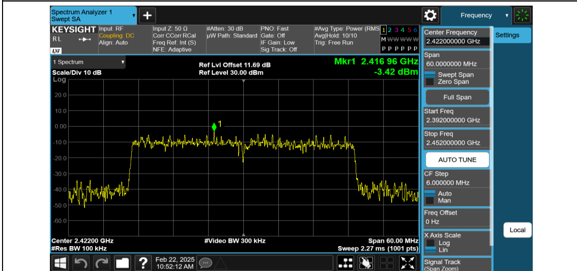
11AX40MIMO-Ant2-2422-0~Reference-PASS
