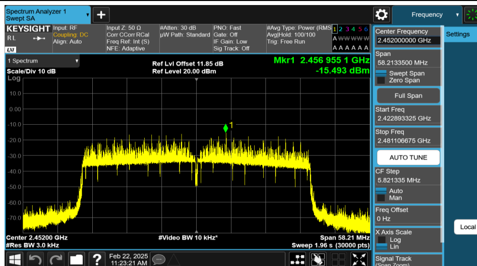
11AX40MIMO-Ant2-2452-PASS
