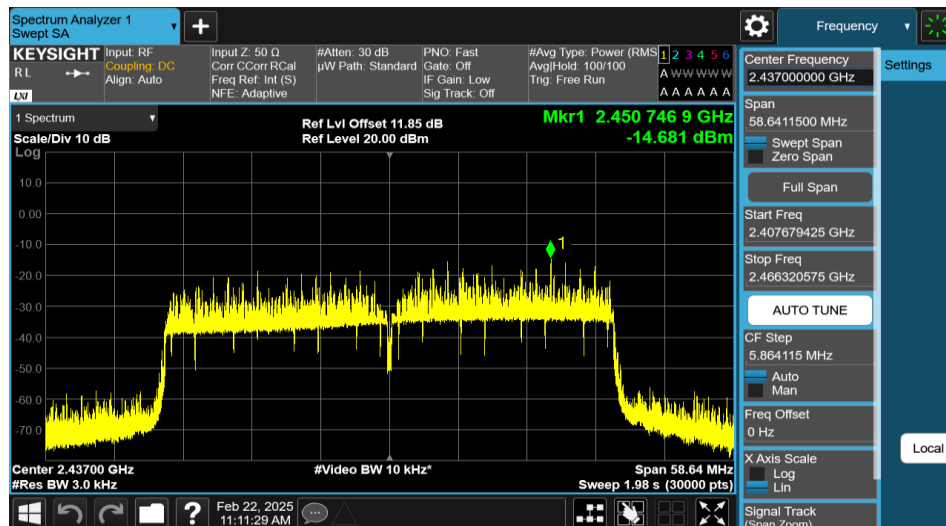
11AX40MIMO-Ant2-2437-PASS
