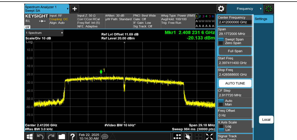
11AX20MIMO-Ant2-2412-PASS
