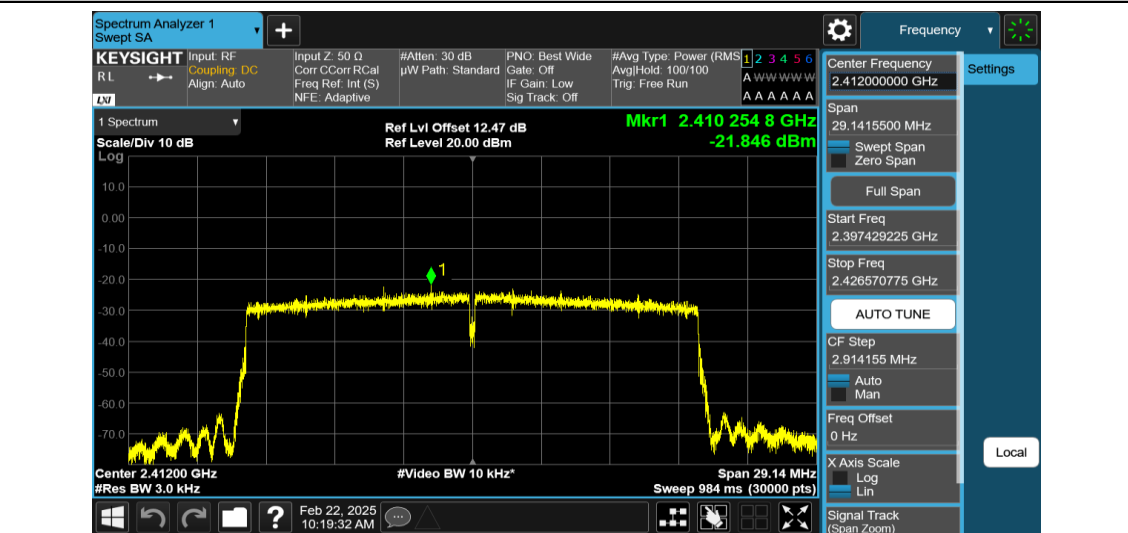
11AX20MIMO-Ant1-2412-PASS
