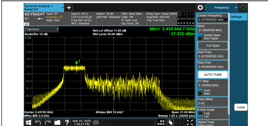
11AX20MIMO-Ant2-2437-52Tone-RU37-PASS
