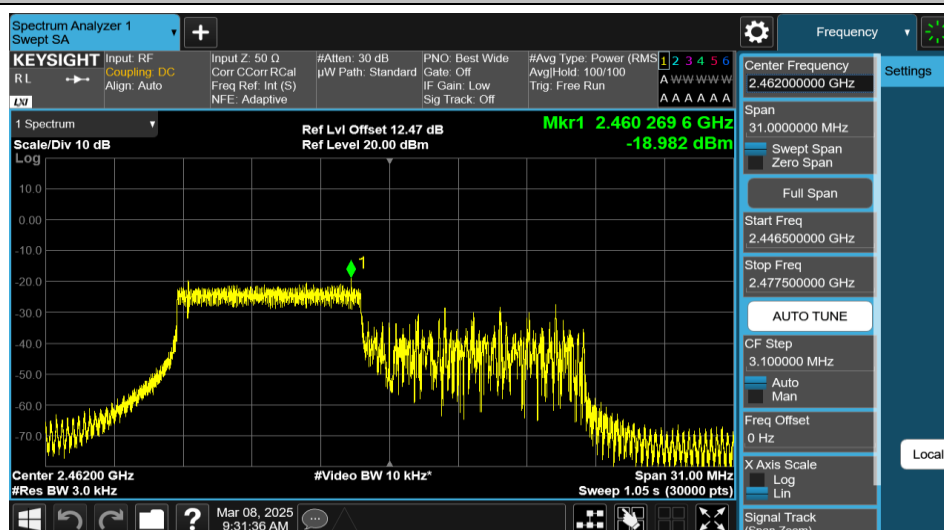
11AX20MIMO-Ant1-2462-106Tone-RU53-PASS
