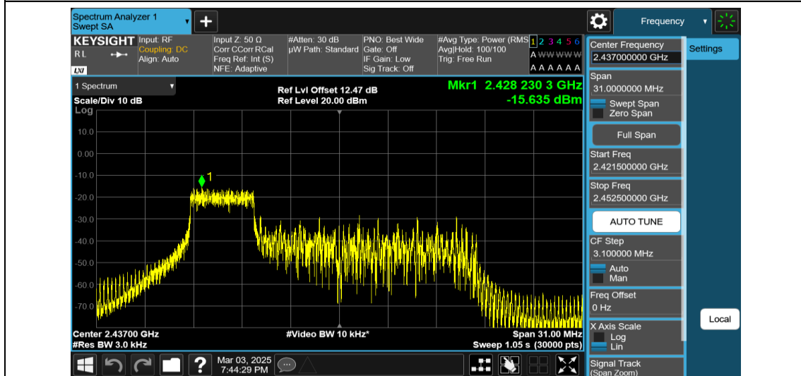
11AX20MIMO-Ant1-2437-52Tone-RU37-PASS
