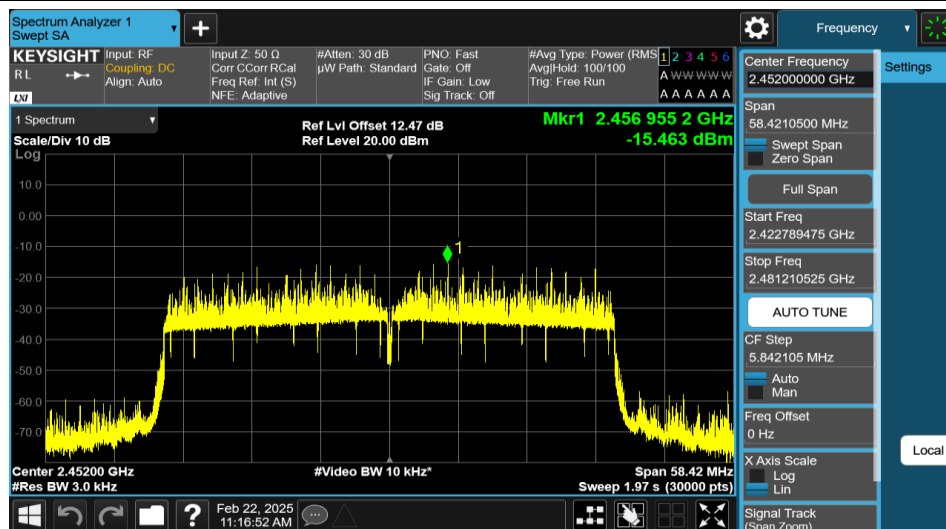
11AX40MIMO-Ant1-2452-PASS
