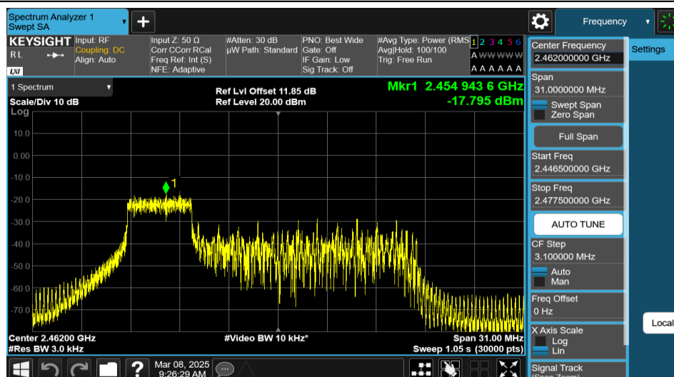
11AX20MIMO-Ant2-2462-52Tone-RU37-PASS
