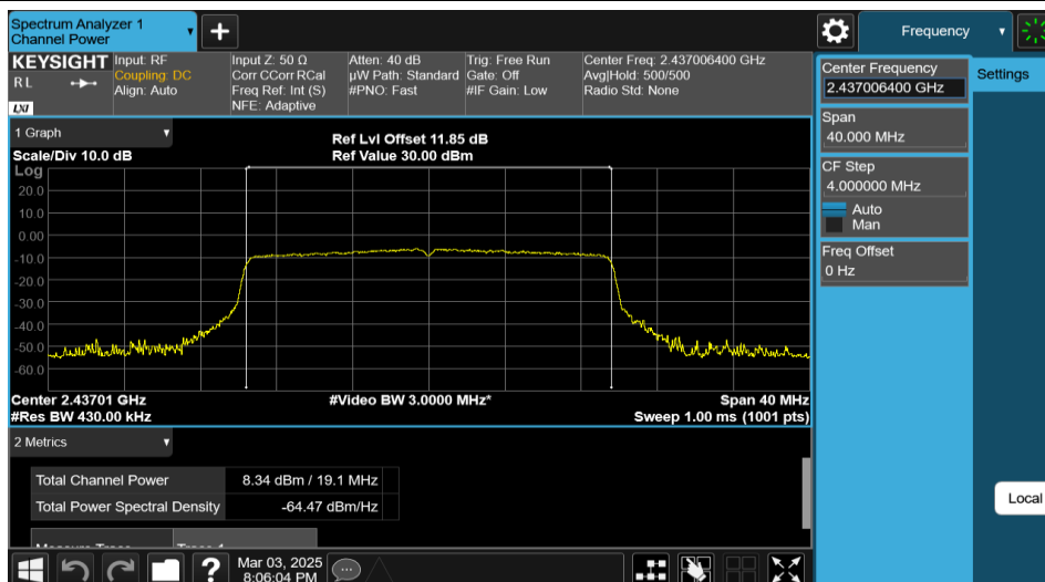
11AX20MIMO-Ant2-2437-242Tone-RU61-PASS
