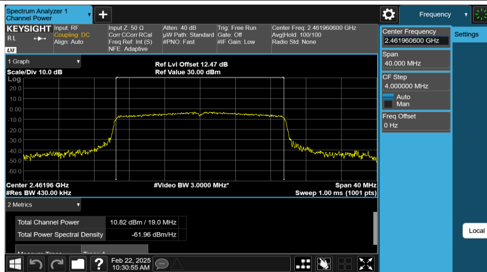
11AX20MIMO-Ant1-2462-PASS
