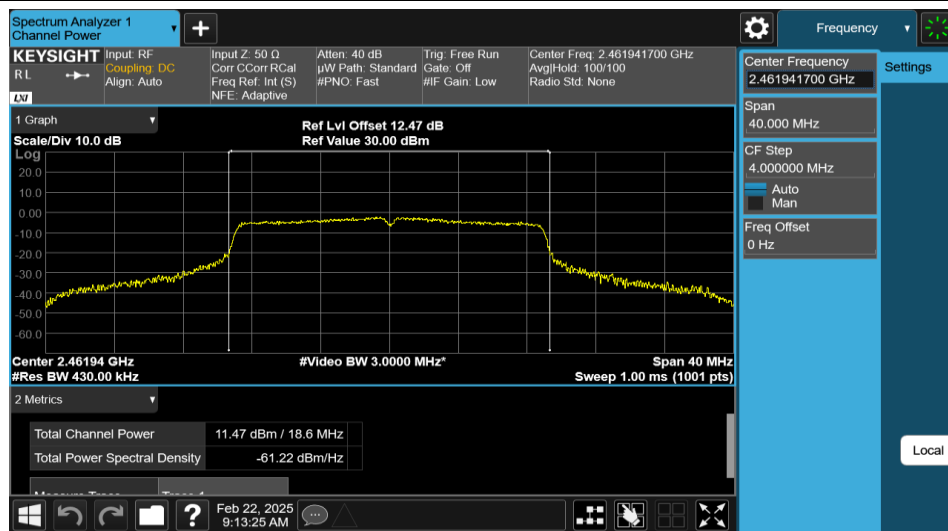
11N20MIMO-Ant1-2462-PASS
