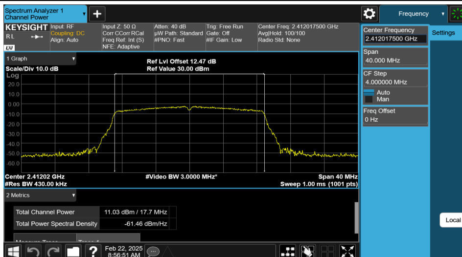
11N20MIMO-Ant1-2412-PASS
