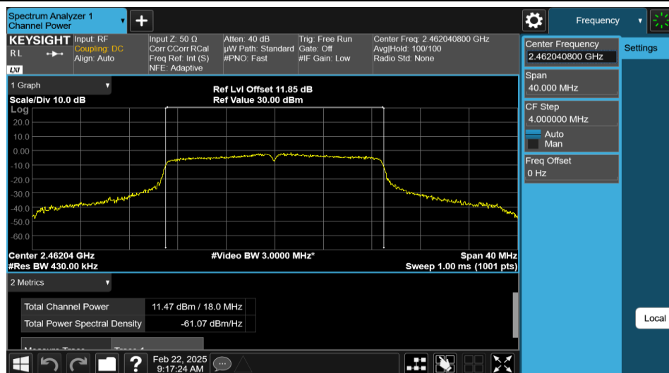
11N20MIMO-Ant2-2462-PASS
