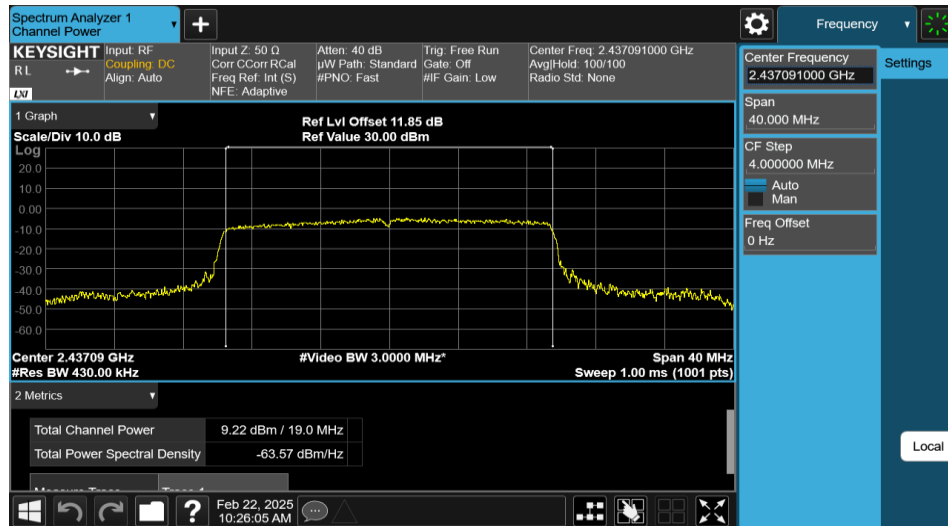
11AX20MIMO-Ant2-2437-PASS
