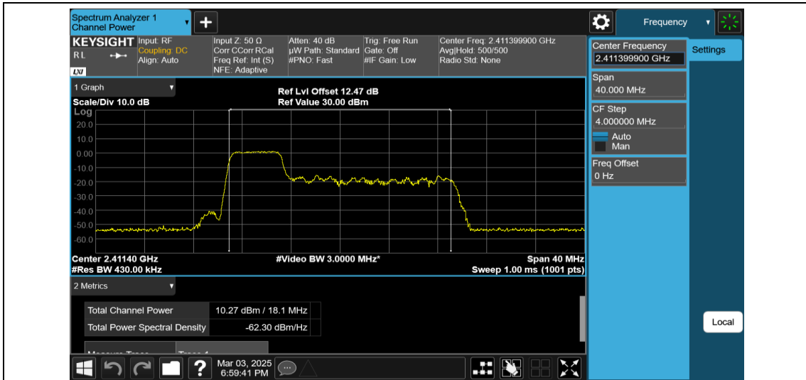
11AX20MIMO-Ant1-2412-52Tone-RU37-PASS
