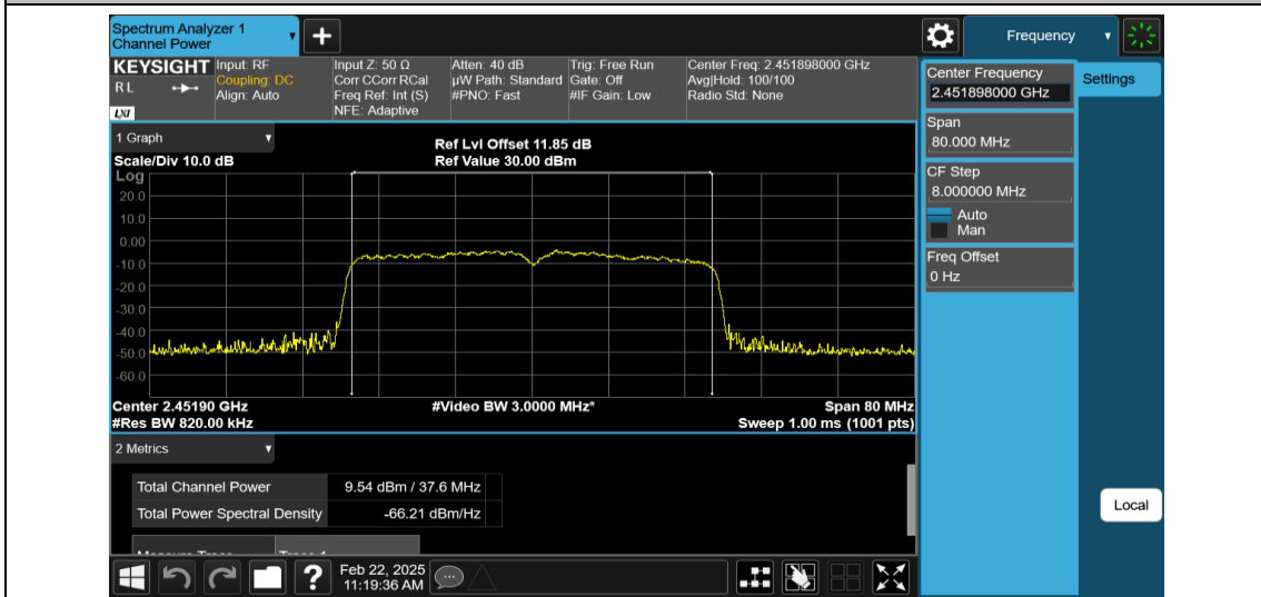
11AX40MIMO-Ant2-2452-PASS
