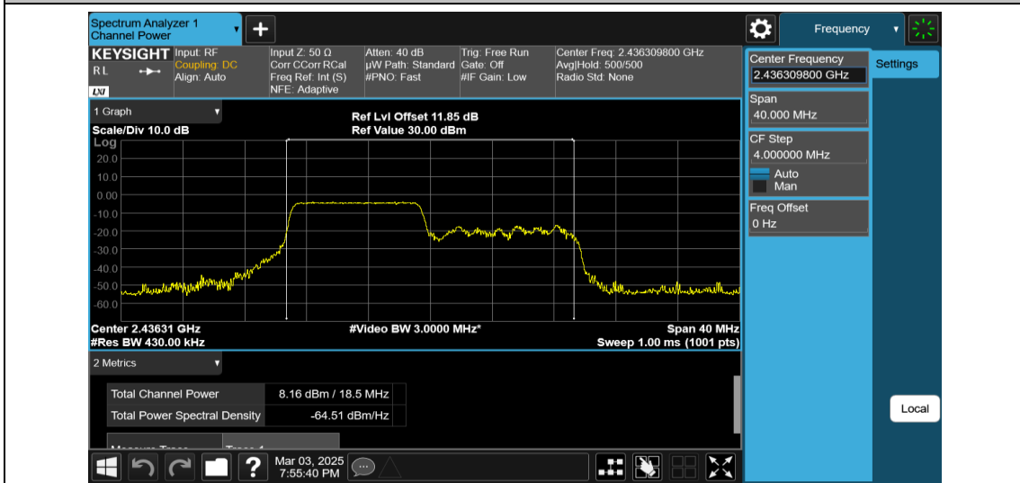
11AX20MIMO-Ant2-2437-106Tone-RU53-PASS
