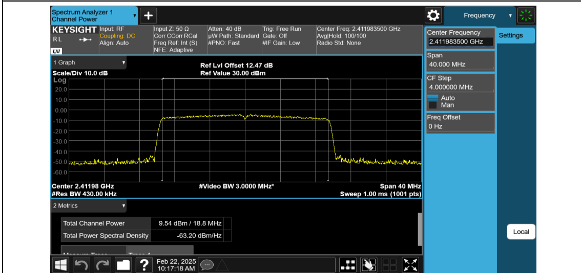
11AX20MIMO-Ant1-2412-PASS
