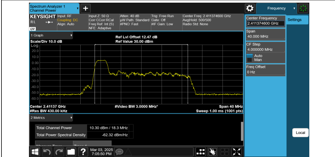
11AX20MIMO-Ant1-2412-26Tone-RU0-PASS
