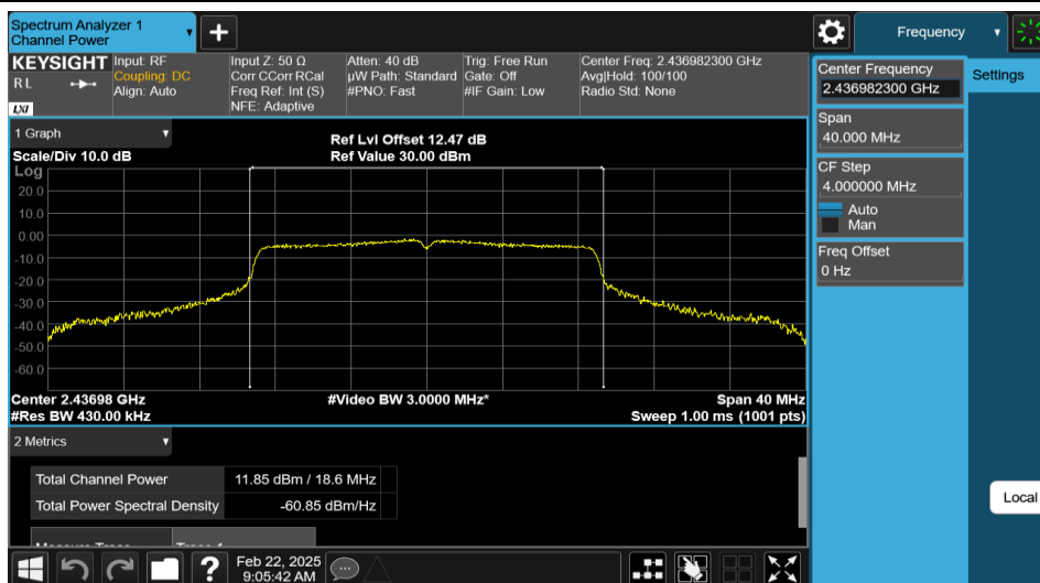
11N20MIMO-Ant1-2437-PASS
