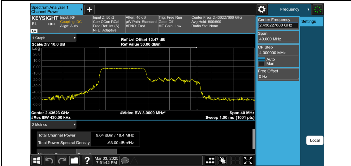
11AX20MIMO-Ant1-2437-106Tone-RU53-PASS
