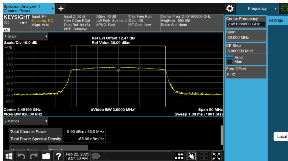
11N40MIMO-Ant1-2452-PASS
