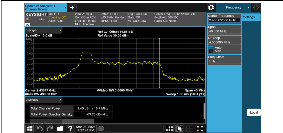
11AX20MIMO-Ant2-2437-26Tone-RU0-PASS
