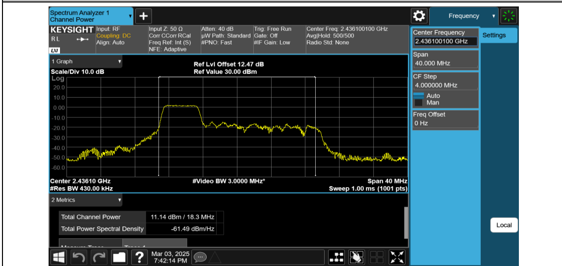
11AX20MIMO-Ant1-2437-52Tone-RU37-PASS
