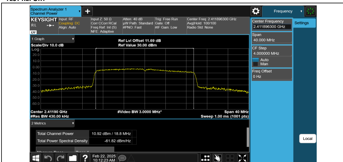
11AX20MIMO-Ant2-2412-PASS
