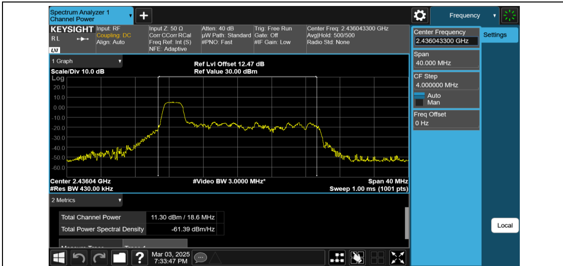
11AX20MIMO-Ant1-2437-26Tone-RU0-PASS
