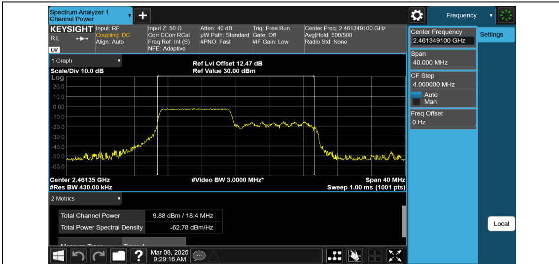
11AX20MIMO-Ant1-2462-106Tone-RU53-PASS
