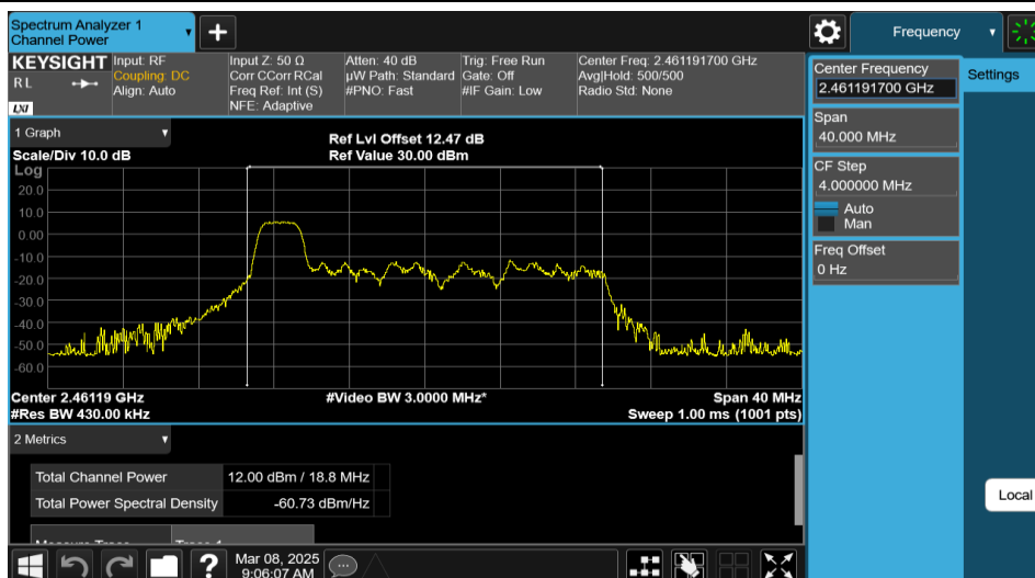
11AX20MIMO-Ant1-2462-26Tone-RU0-PASS
