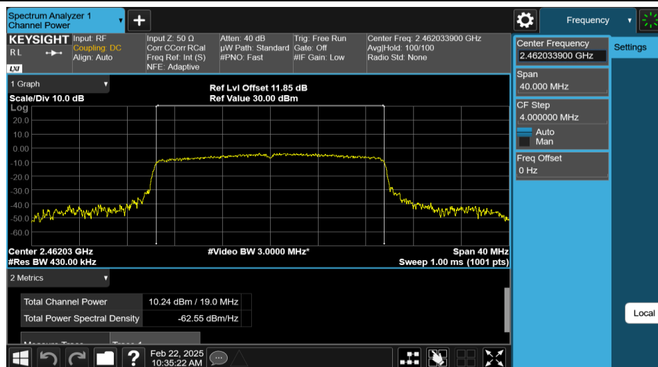
11AX20MIMO-Ant2-2462-PASS
