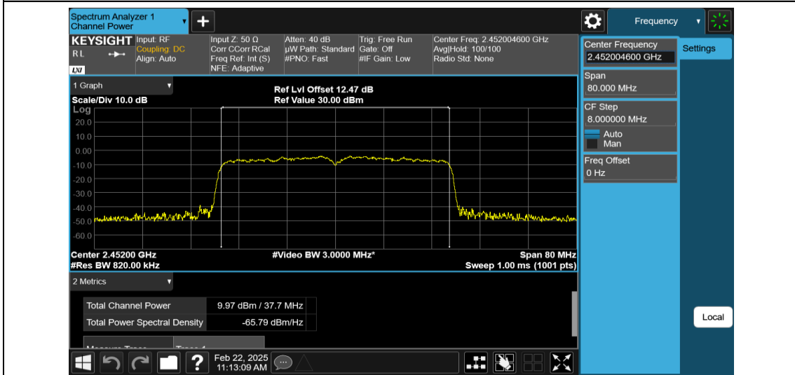
11AX40MIMO-Ant1-2452-PASS
