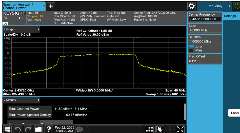
11N20MIMO-Ant2-2437-PASS
