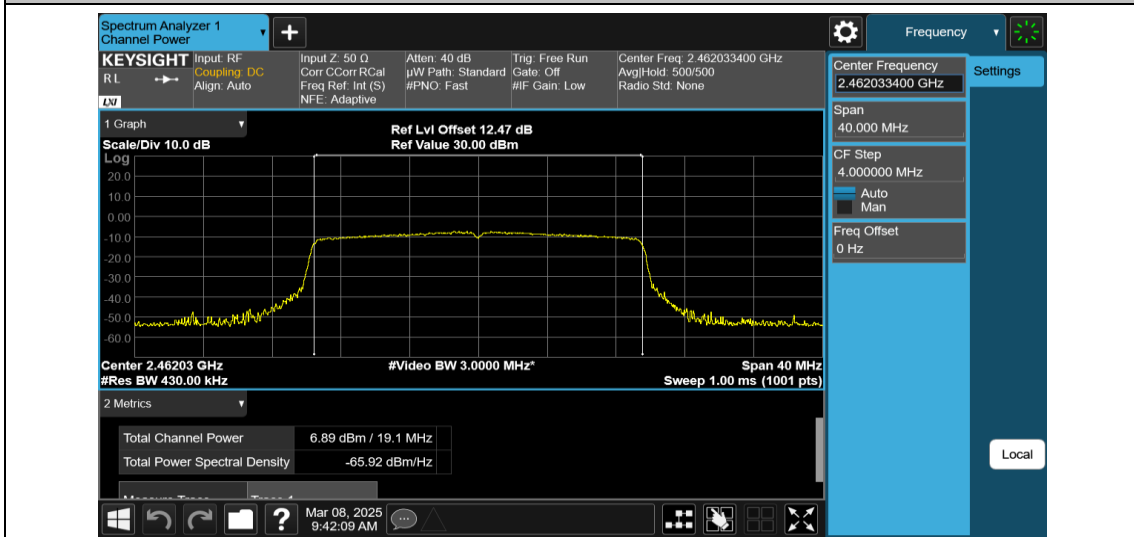
11AX20MIMO-Ant1-2462-242Tone-RU61-PASS
