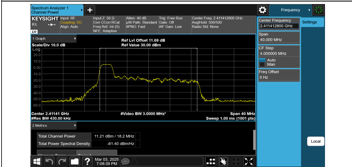
11AX20MIMO-Ant2-2412-26Tone-RU0-PASS
