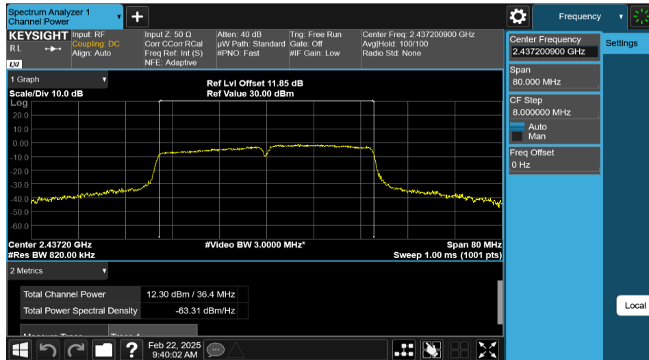
11N40MIMO-Ant2-2437-PASS
