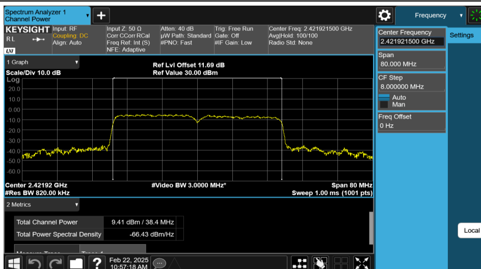
11AX40MIMO-Ant2-2422-PASS
