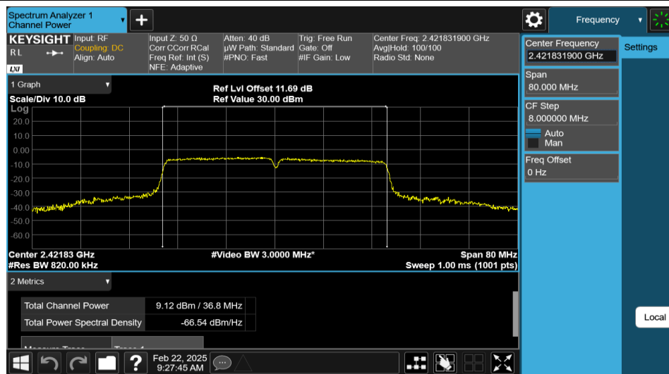
11N40MIMO-Ant2-2422-PASS
