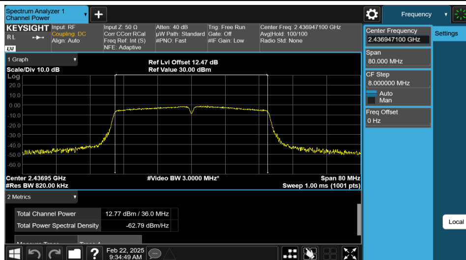
11N40MIMO-Ant1-2437-PASS
