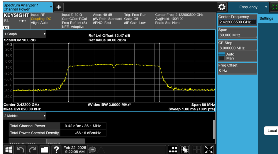
11N40MIMO-Ant1-2422-PASS
