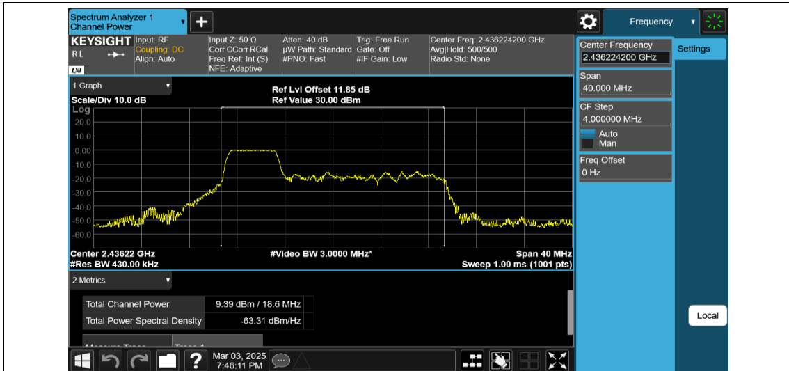
11AX20MIMO-Ant2-2437-52Tone-RU37-PASS
