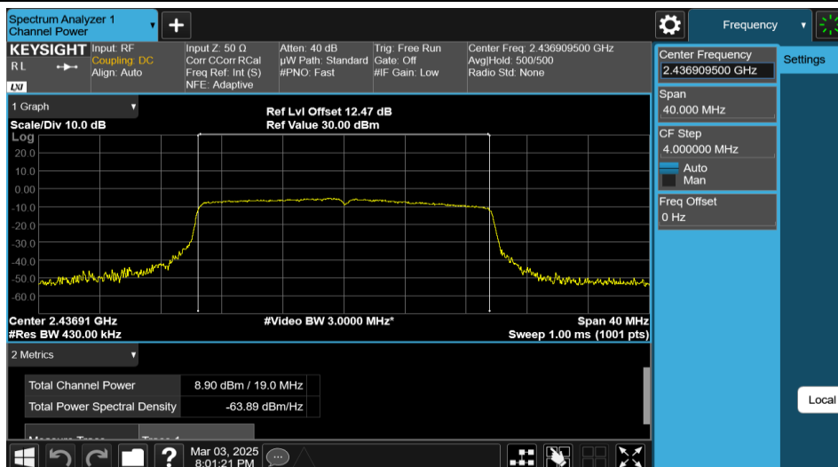
11AX20MIMO-Ant1-2437-242Tone-RU61-PASS
