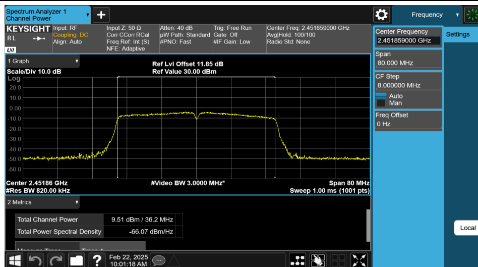
11N40MIMO-Ant2-2452-PASS
