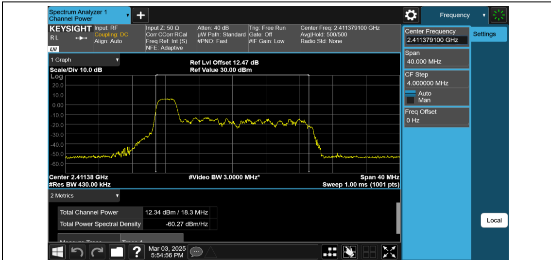
11AX20SISO-Ant1-2412-26Tone-RU0-PASS
