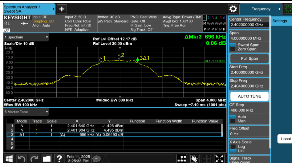
BLE_1M-Ant1-2402-PASS
