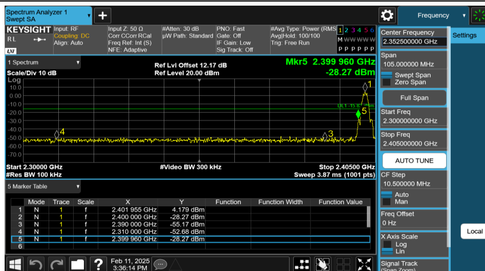
BLE_2M-Ant1-2402-PASS
