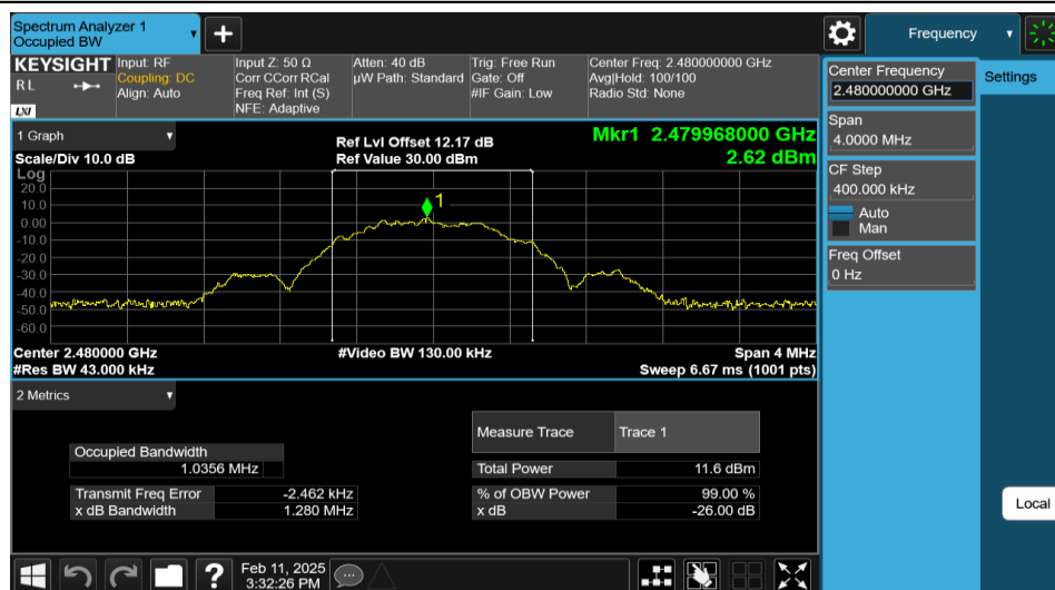
BLE_1M-Ant1-2480
