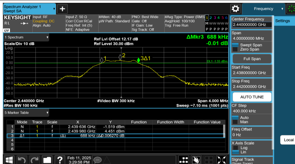
BLE_1M-Ant1-2440-PASS
