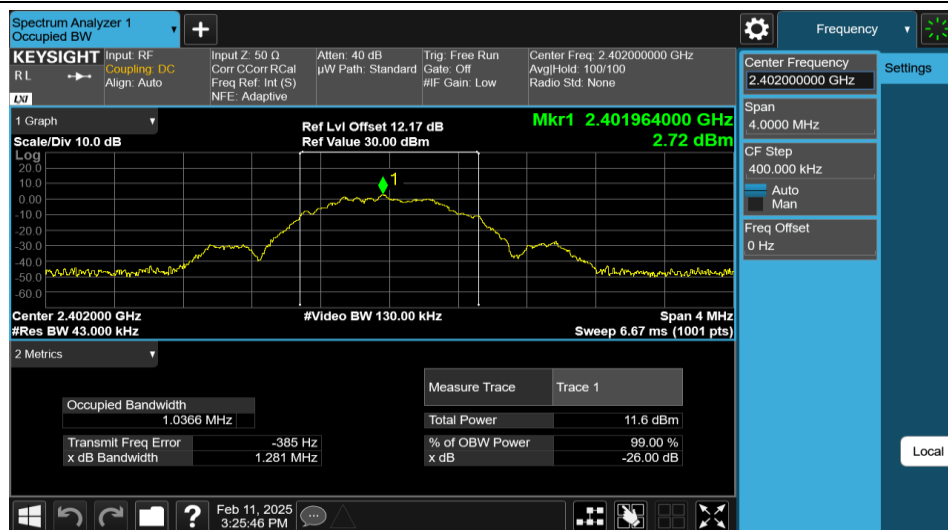
BLE_1M-Ant1-2402
