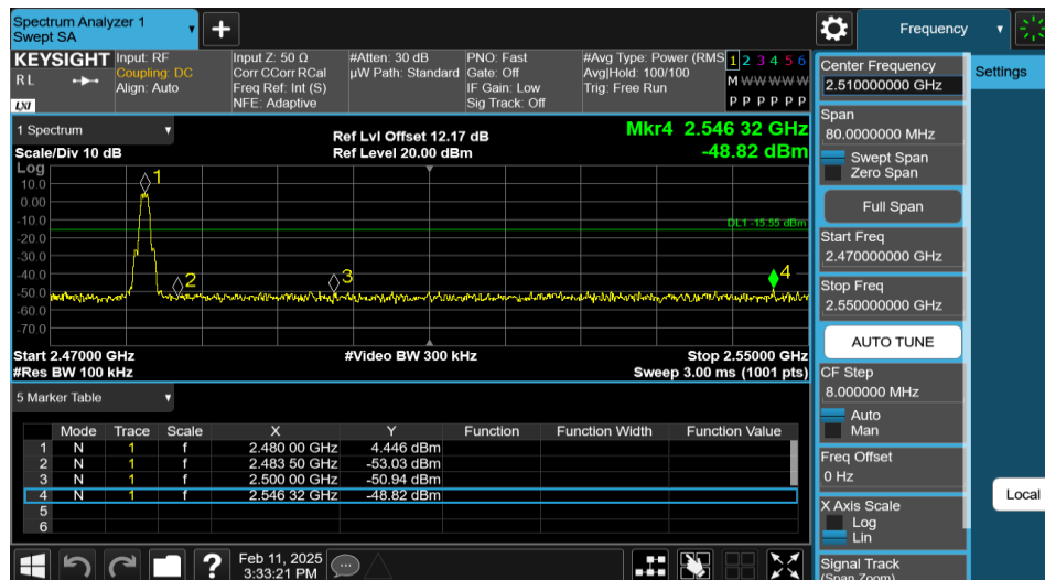
BLE_1M-Ant1-2480-PASS
