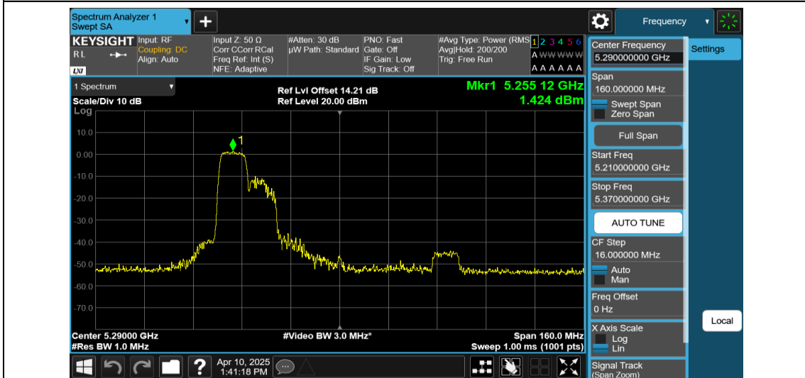
11AX80MIMO-Ant2-5290-106Tone-RU53-PASS
