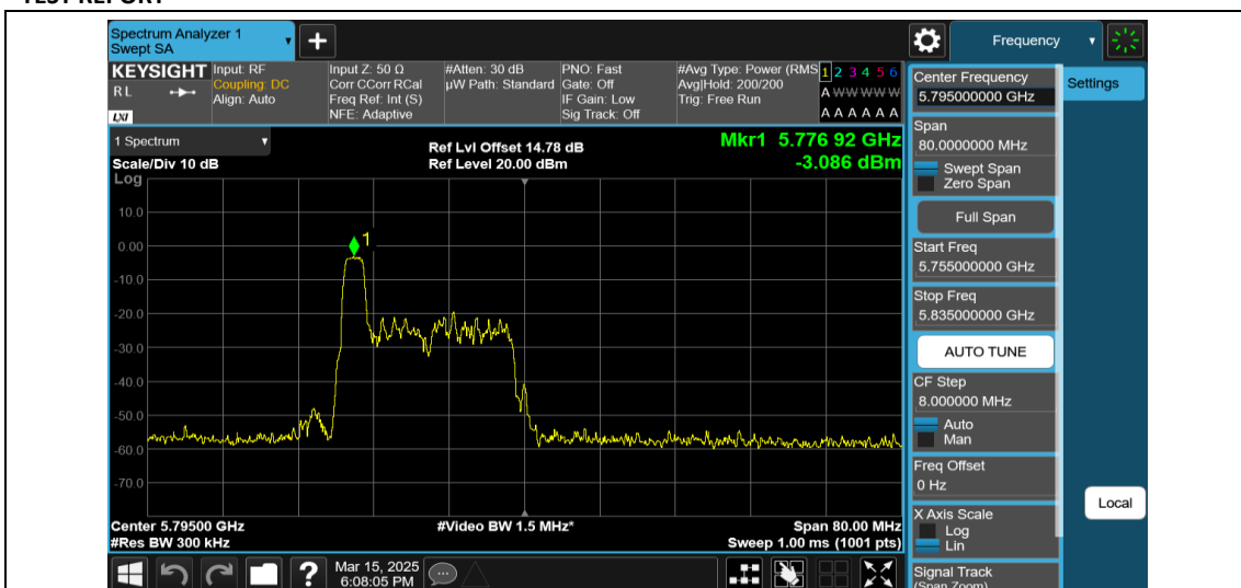
11AX40MIMO-Ant1-5795-26Tone-RU0-PASS
