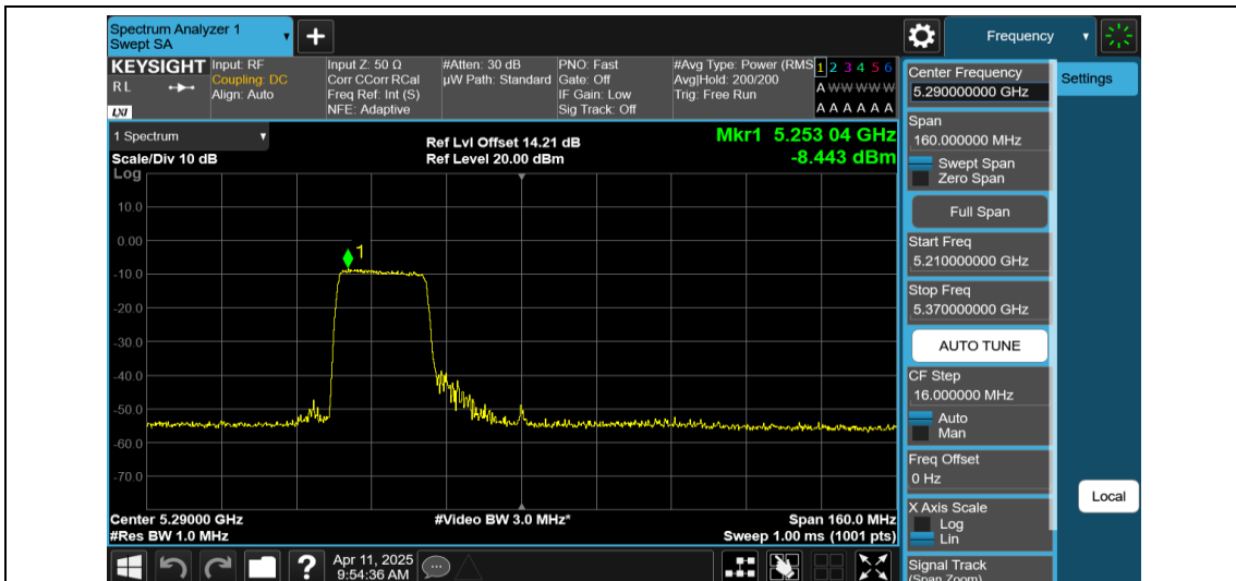
11AX80MIMO-Ant2-5290-242Tone-RU61-PASS
