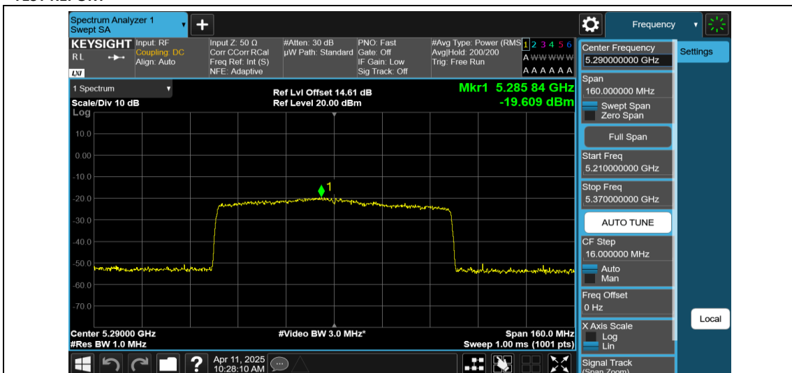
11AX80MIMO-Ant1-5290-996Tone-RU67-PASS
