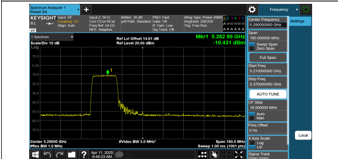
11AX80MIMO-Ant1-5290-242Tone-RU61-PASS
