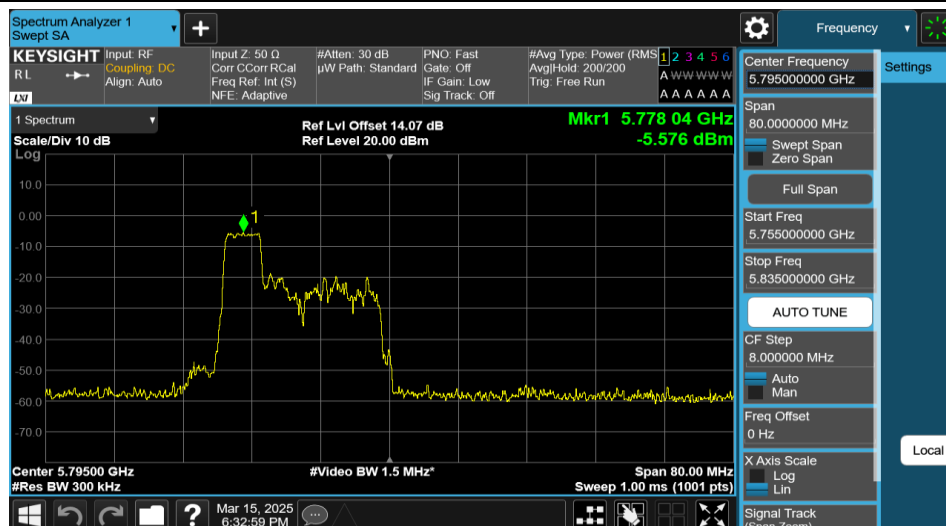
11AX40MIMO-Ant2-5795-52Tone-RU37-PASS
