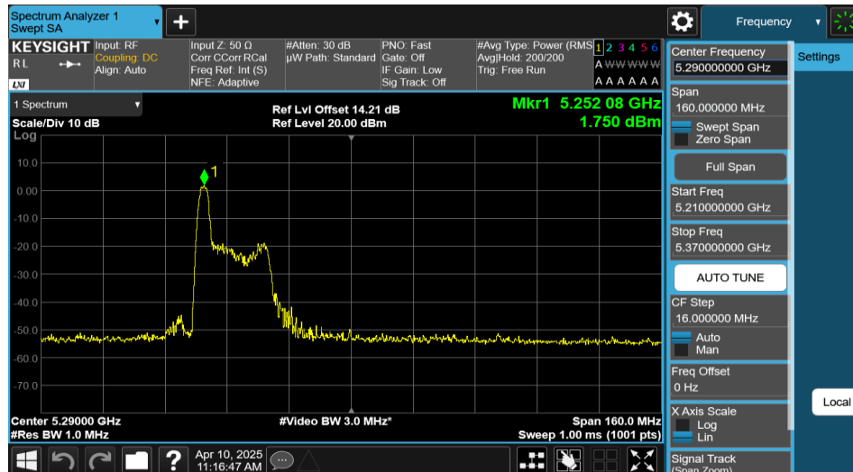
11AX80MIMO-Ant2-5290-26Tone-RU0-PASS
