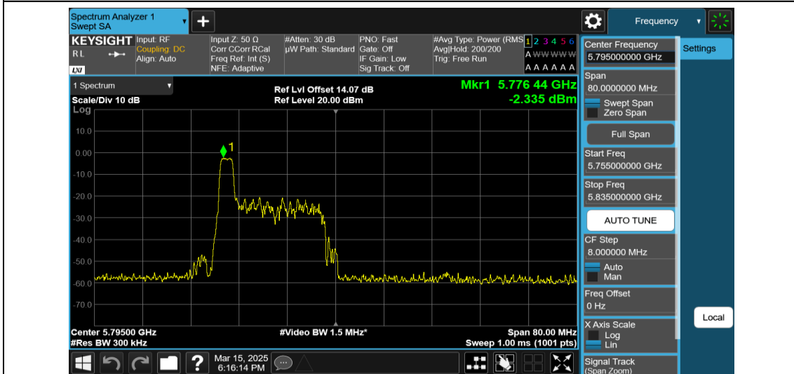
11AX40MIMO-Ant2-5795-26Tone-RU0-PASS
