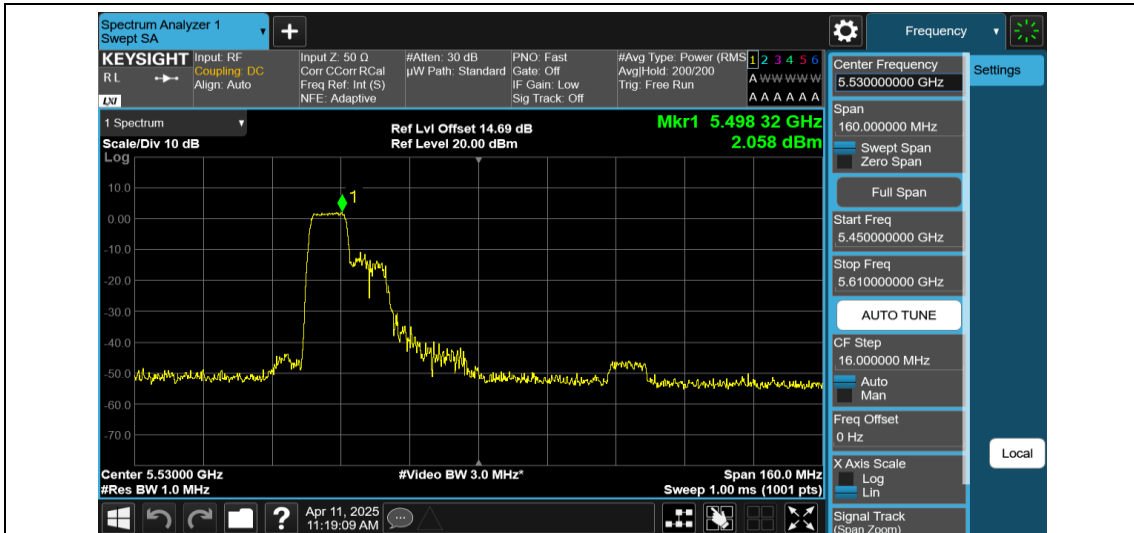
11AX80MIMO-Ant1-5530-106Tone-RU53-PASS
