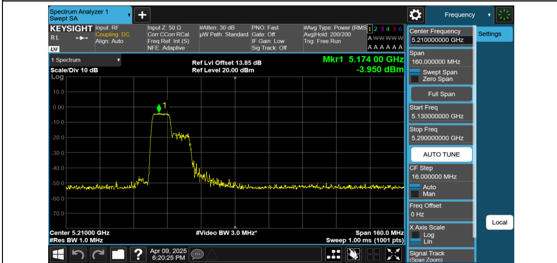
11AX80MIMO-Ant2-5210-106Tone-RU53-PASS
