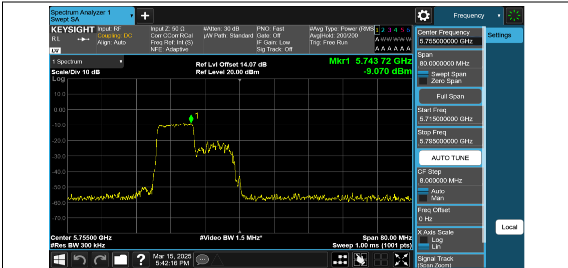
11AX40MIMO-Ant2-5755-106Tone-RU53-PASS
