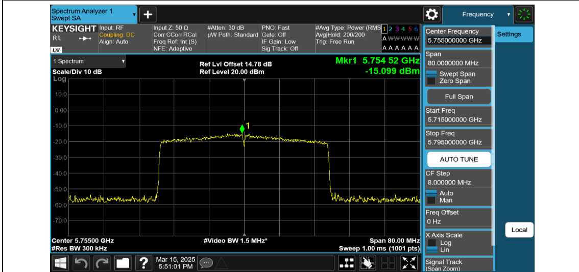
11AX40MIMO-Ant1-5755-484Tone-RU65-PASS
