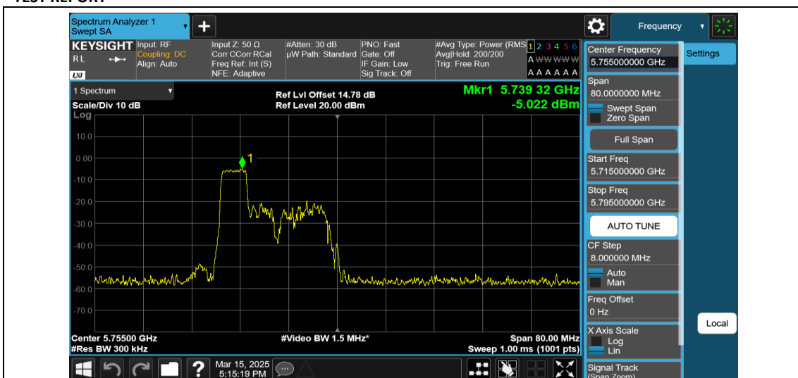
11AX40MIMO-Ant1-5755-52Tone-RU37-PASS
