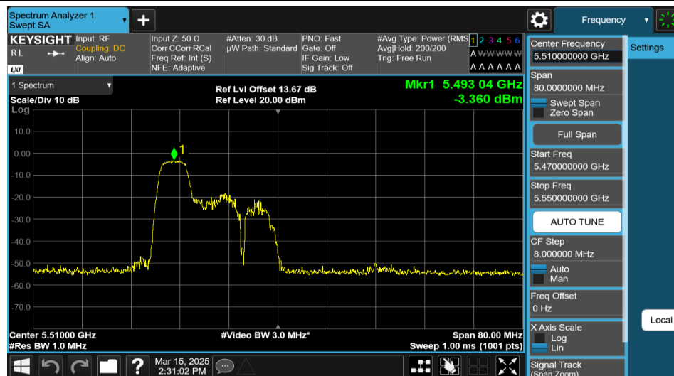
11AX40MIMO-Ant2-5510-52Tone-RU37-PASS
