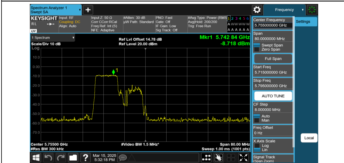
11AX40MIMO-Ant1-5755-106Tone-RU53-PASS
