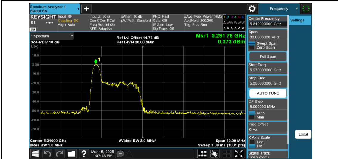
11AX40MIMO-Ant1-5310-26Tone-RU0-PASS
