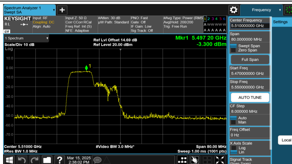
11AX40MIMO-Ant1-5510-106Tone-RU53-PASS
