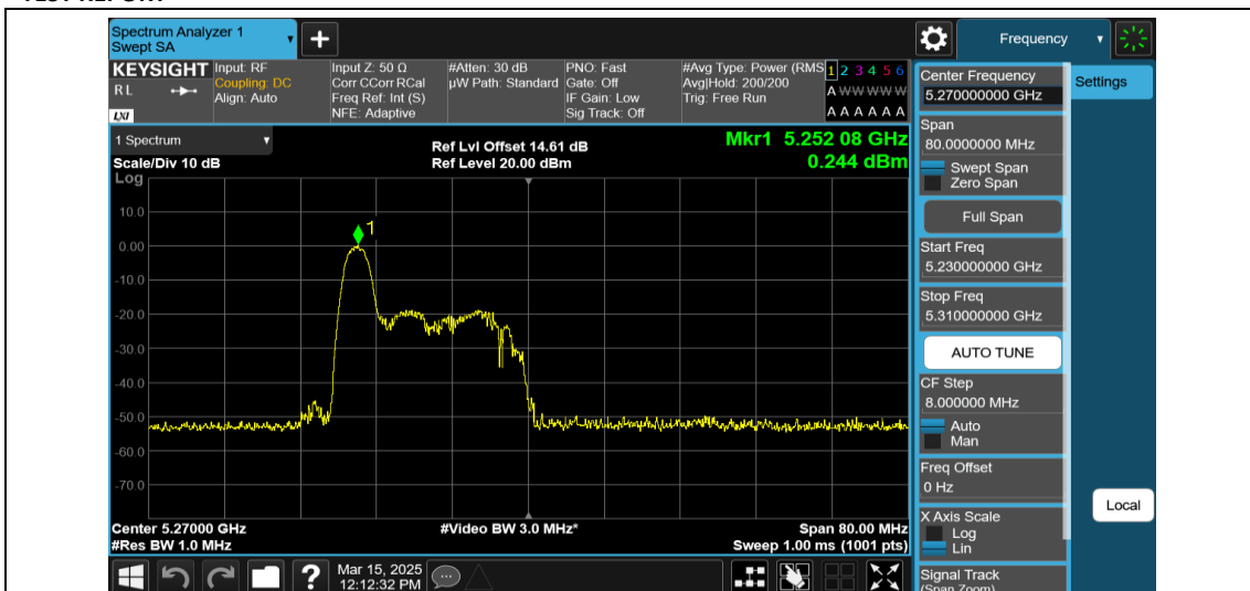
11AX40MIMO-Ant1-5270-26Tone-RU0-PASS
