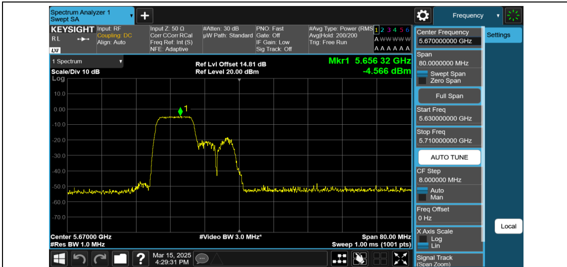
11AX40MIMO-Ant1-5670-106Tone-RU53-PASS
