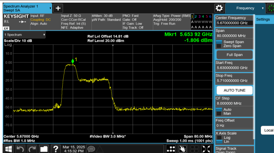
11AX40MIMO-Ant1-5670-52Tone-RU37-PASS
