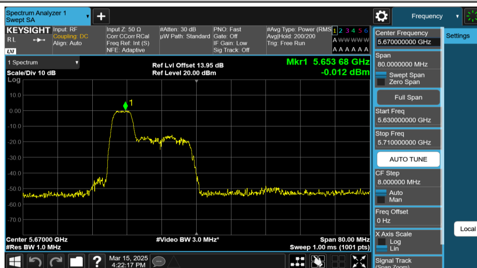
11AX40MIMO-Ant2-5670-52Tone-RU37-PASS
