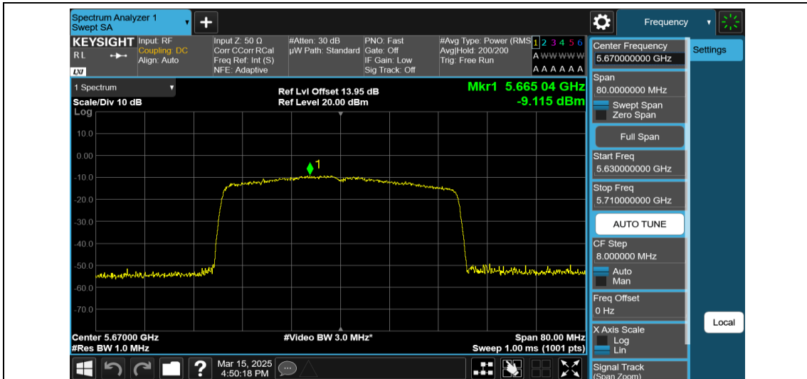
11AX40MIMO-Ant2-5670-484Tone-RU65-PASS
