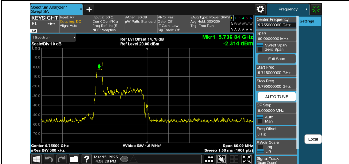
11AX40MIMO-Ant1-5755-26Tone-RU0-PASS
