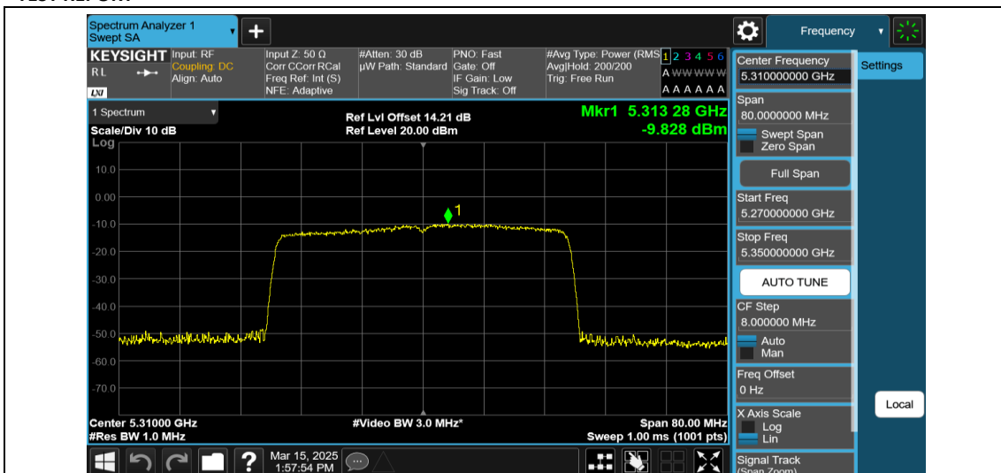
11AX40MIMO-Ant2-5310-484Tone-RU65-PASS
