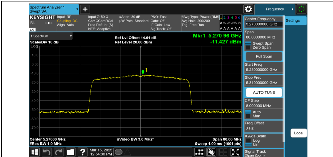
11AX40MIMO-Ant1-5270-484Tone-RU65-PASS
