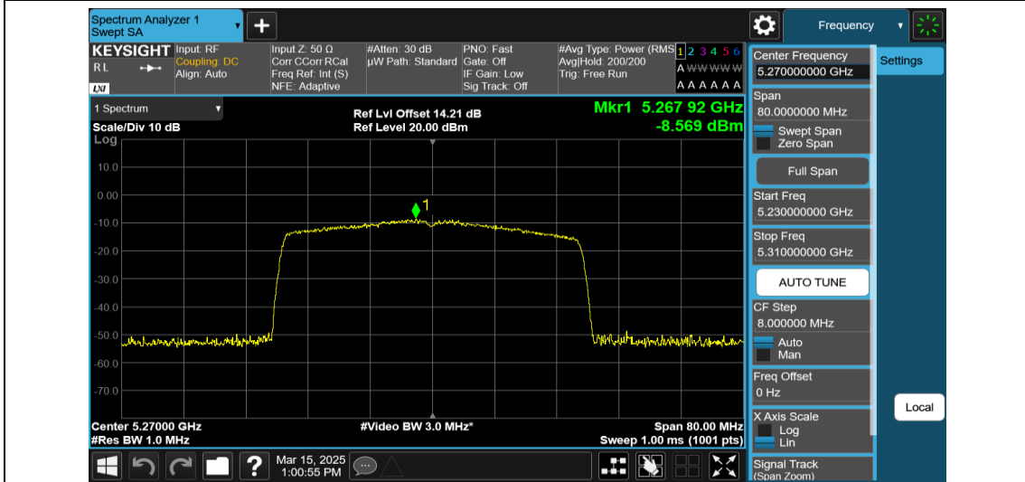
11AX40MIMO-Ant2-5270-484Tone-RU65-PASS
