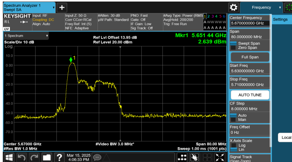
11AX40MIMO-Ant2-5670-26Tone-RU0-PASS
