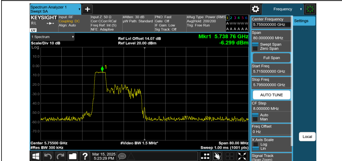
11AX40MIMO-Ant2-5755-52Tone-RU37-PASS
