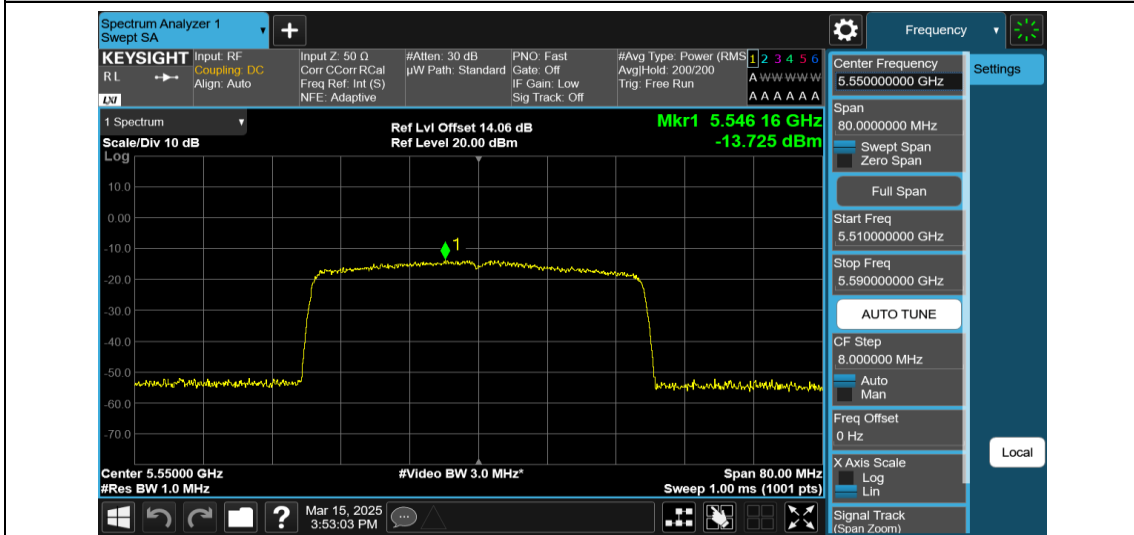
11AX40MIMO-Ant2-5550-484Tone-RU65-PASS
