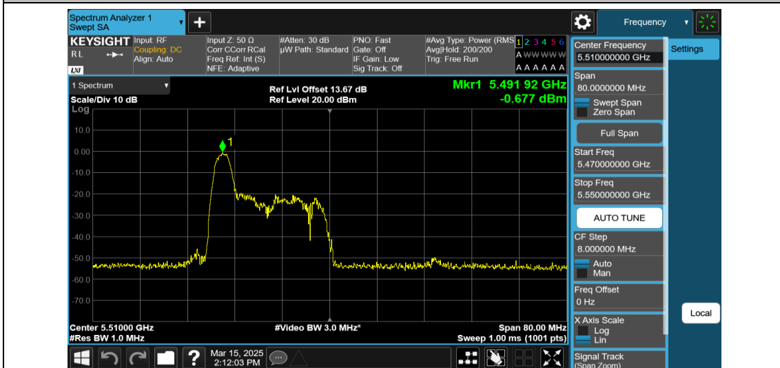
11AX40MIMO-Ant2-5510-26Tone-RU0-PASS
