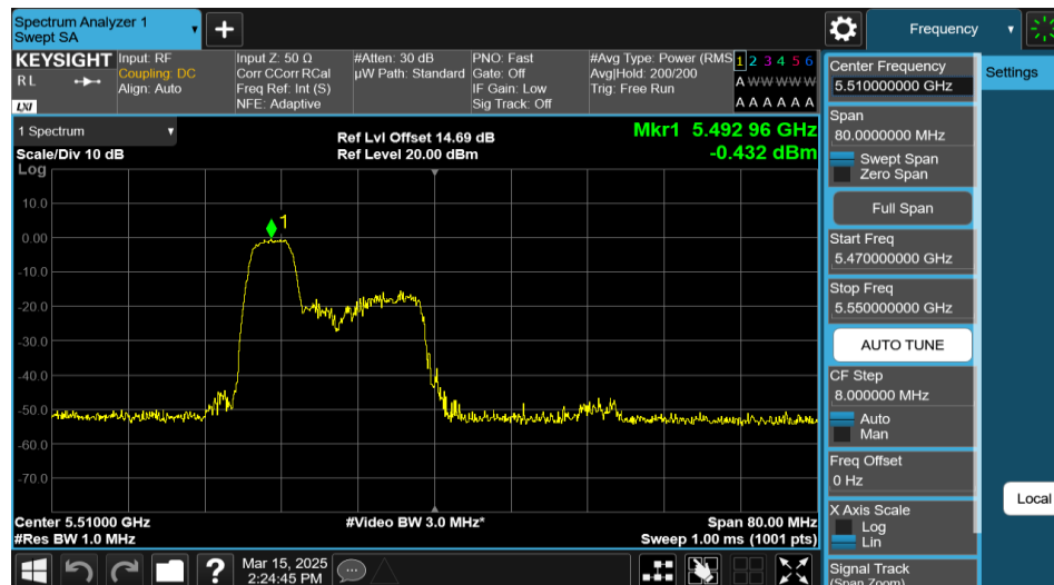
11AX40MIMO-Ant1-5510-52Tone-RU37-PASS
