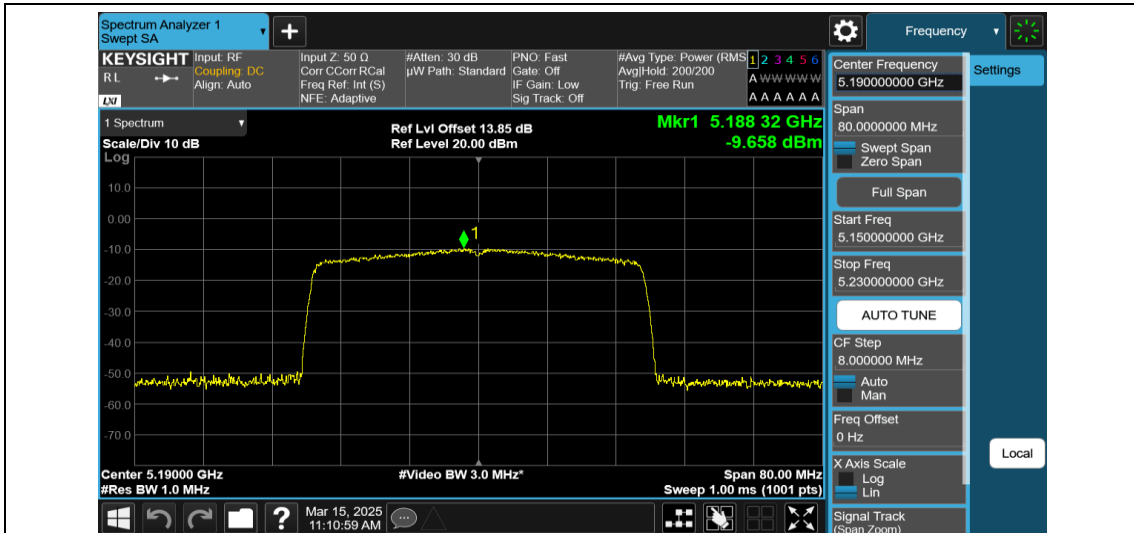
11AX40MIMO-Ant2-5190-484Tone-RU65-PASS
