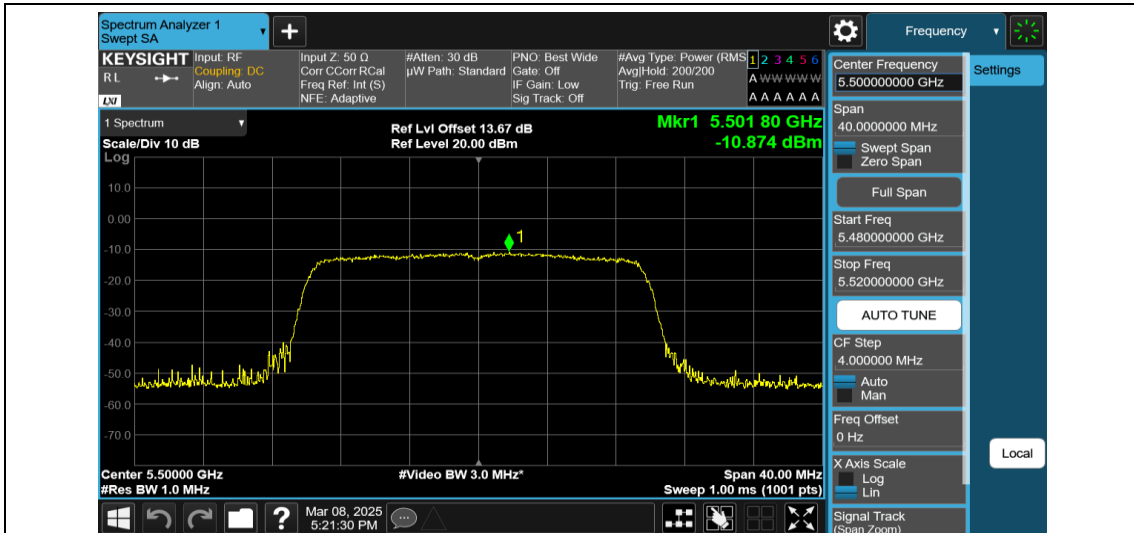
11AX20MIMO-Ant2-5500-242Tone-RU61-PASS
