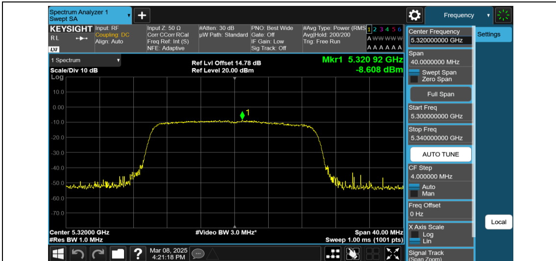
11AX20MIMO-Ant1-5320-242Tone-RU61-PASS
