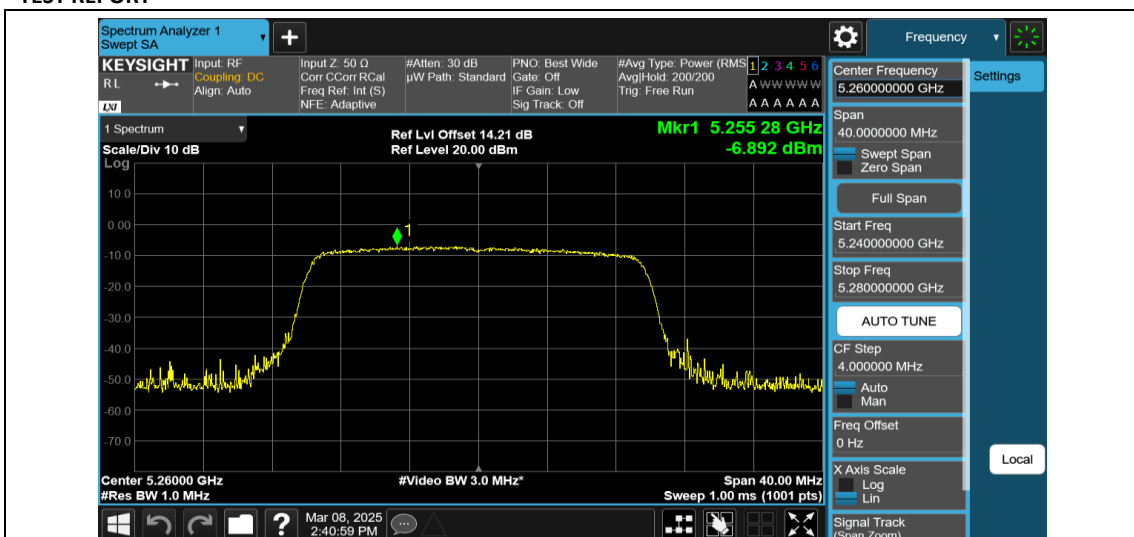
11AX20MIMO-Ant2-5260-242Tone-RU61-PASS
