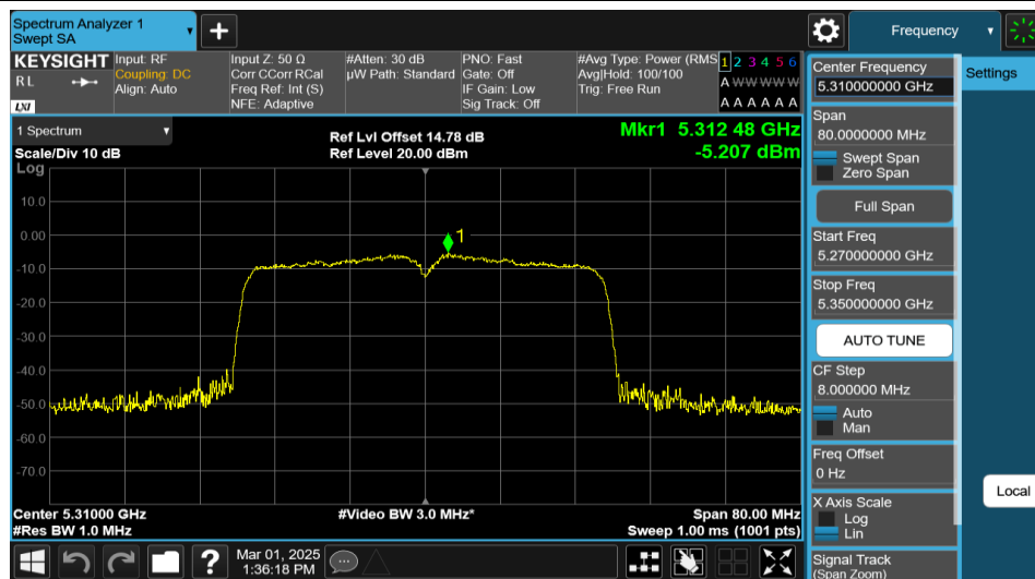
11AX40MIMO-Ant1-5310-PASS
