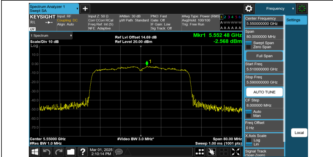
11AX40MIMO-Ant1-5550-PASS
