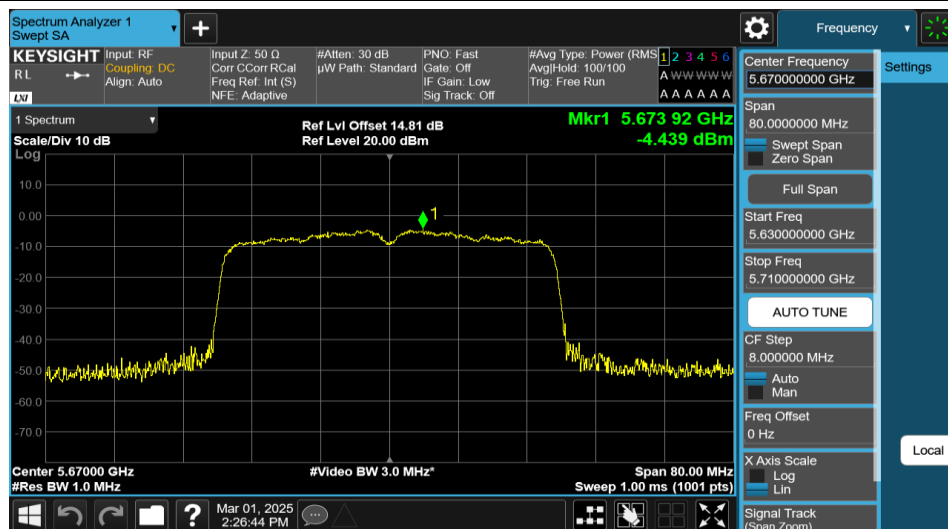
11AX40MIMO-Ant1-5670-PASS
