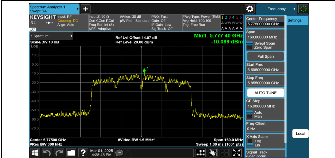
11AX80MIMO-Ant2-5775-PASS
