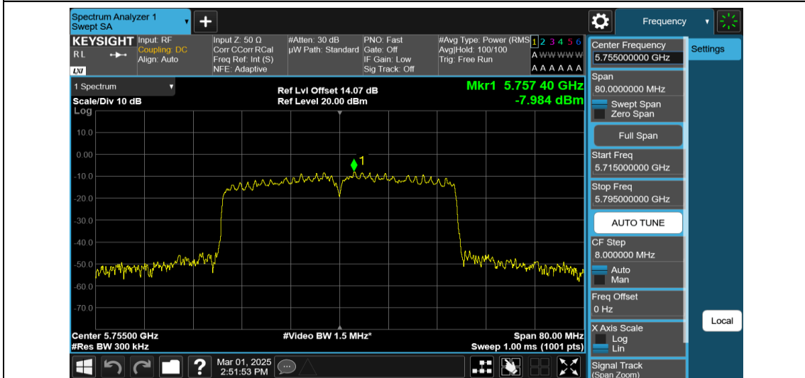
11AX40MIMO-Ant2-5755-PASS
