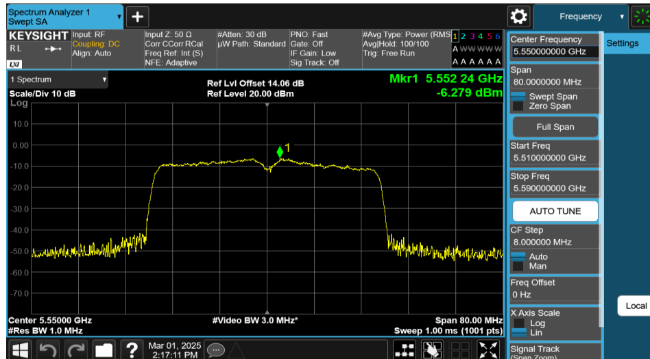
11AX40MIMO-Ant2-5550-PASS
