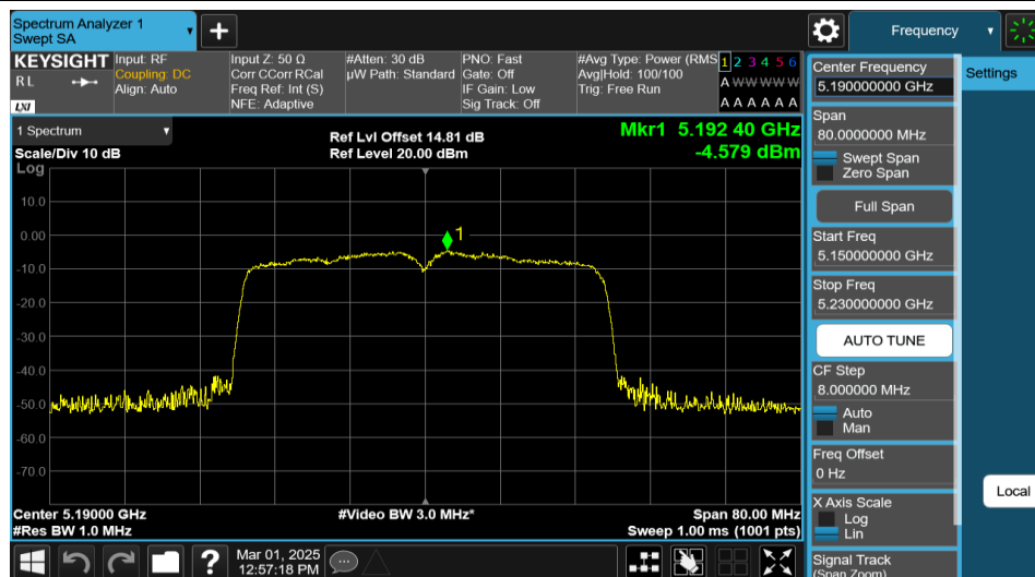
11AX40MIMO-Ant1-5190-PASS
