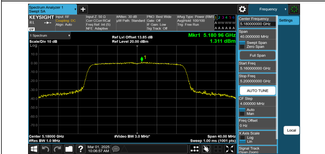
11AX20MIMO-Ant2-5180-PASS
