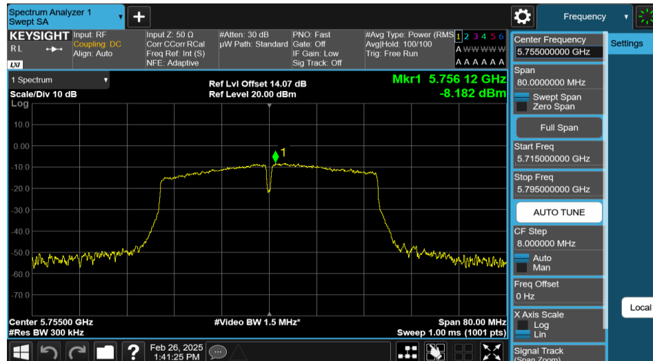
11AC40MIMO-Ant2-5755-PASS
