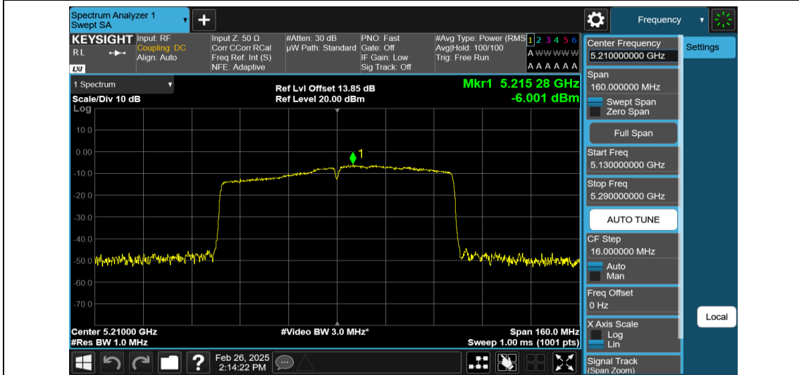
11AC80MIMO-Ant2-5210-PASS
