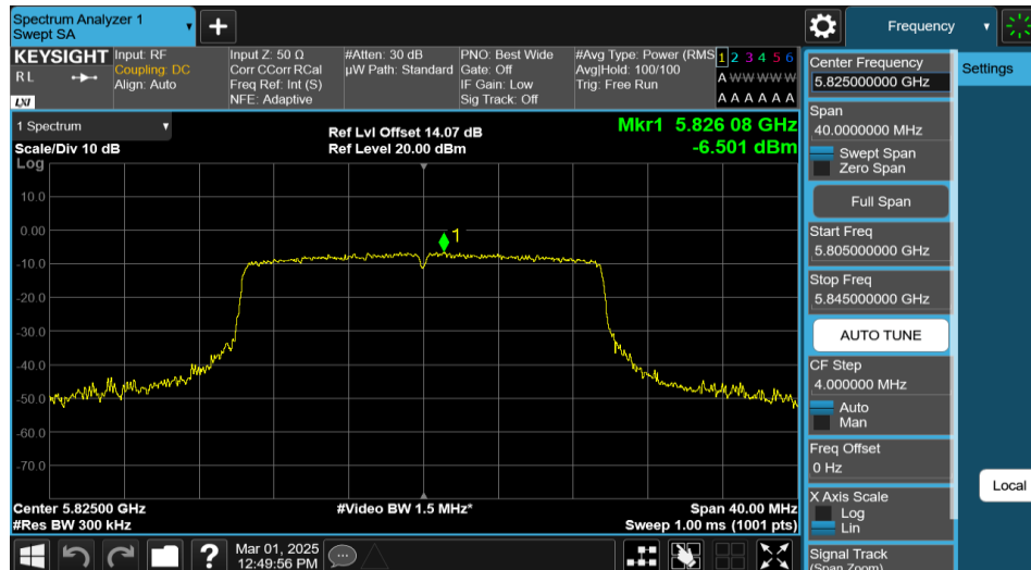
11AX20MIMO-Ant2-5825-PASS
