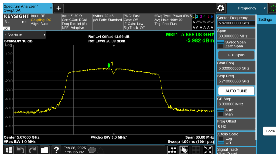
11AC40MIMO-Ant2-5670-PASS
