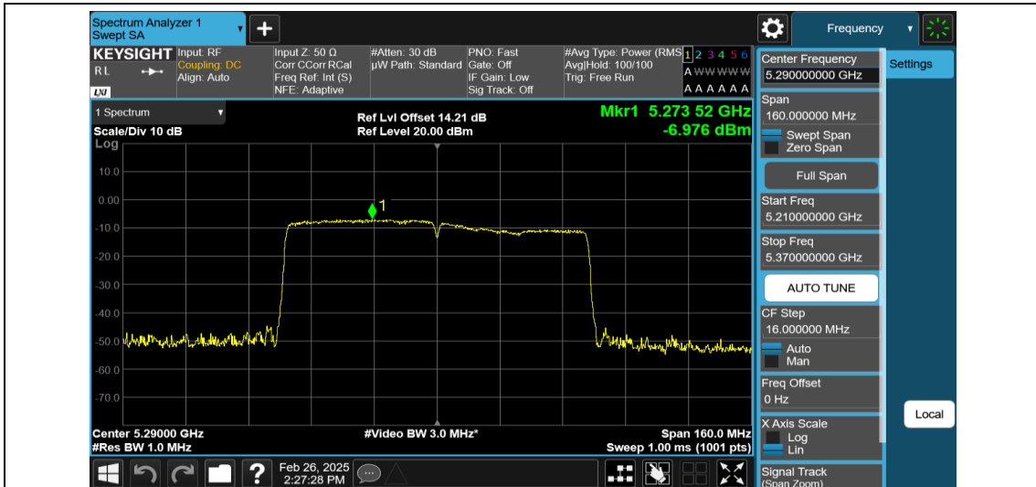
11AC80MIMO-Ant2-5290-PASS
