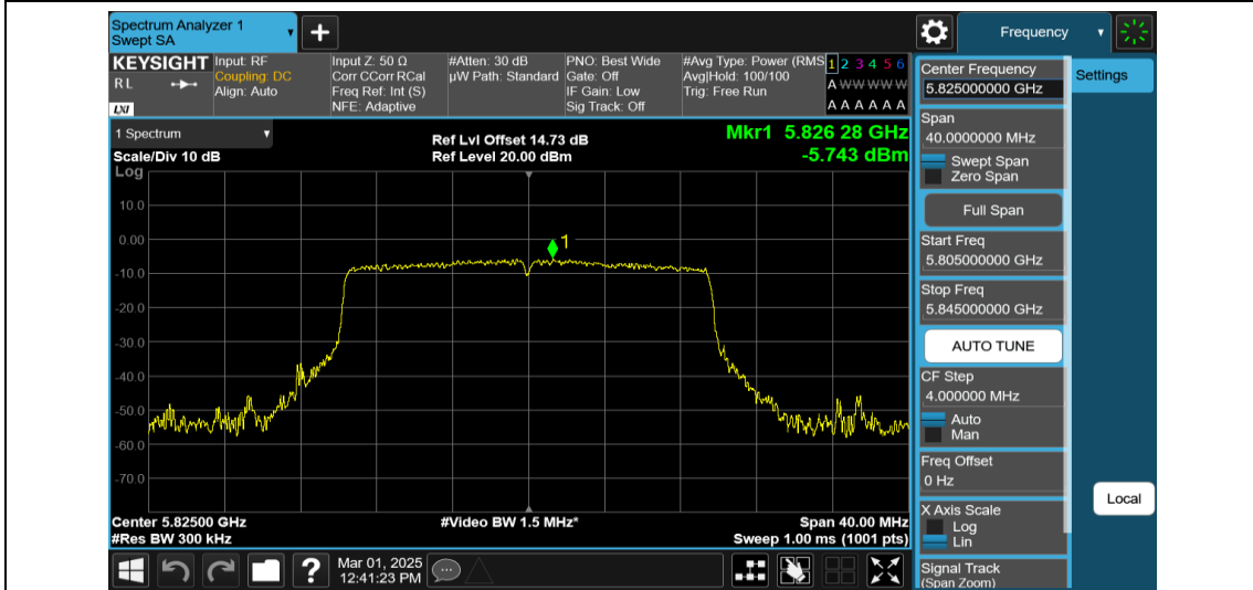
11AX20MIMO-Ant1-5825-PASS
