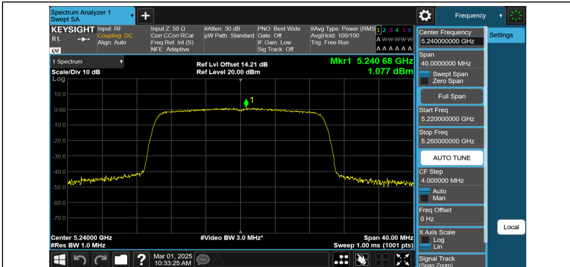
11AX20MIMO-Ant2-5240-PASS
