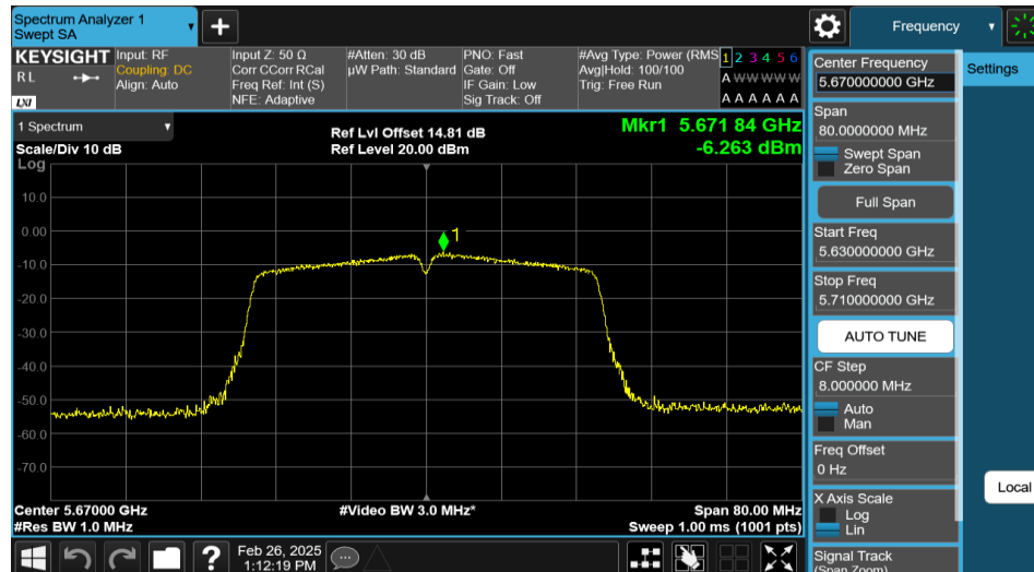
11AC40MIMO-Ant1-5670-PASS
