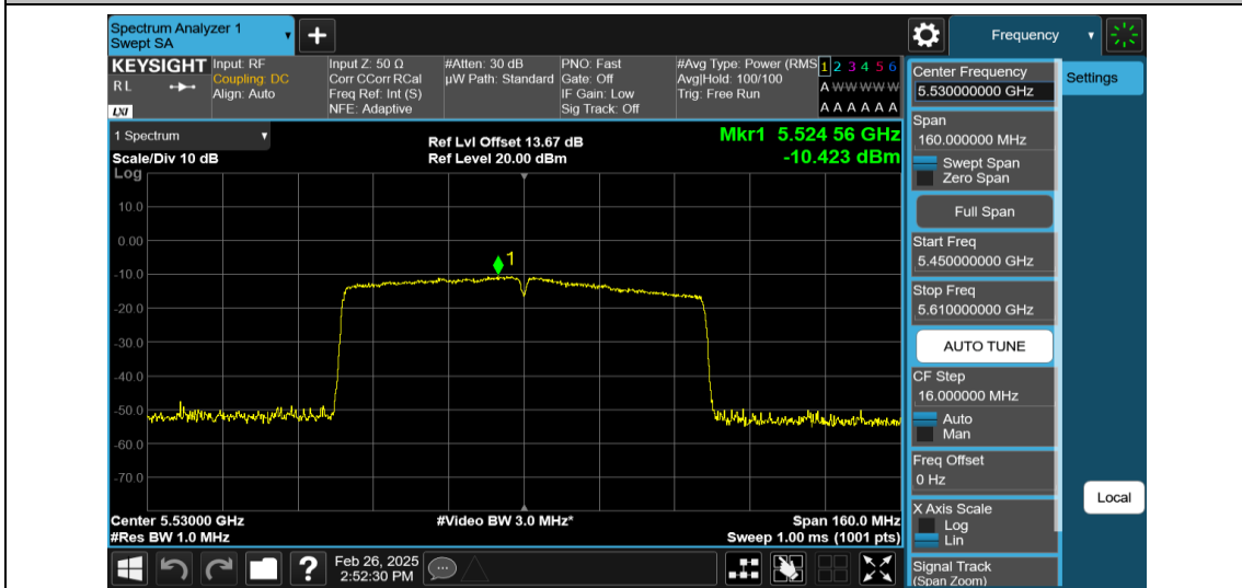
11AC80MIMO-Ant2-5530-PASS
