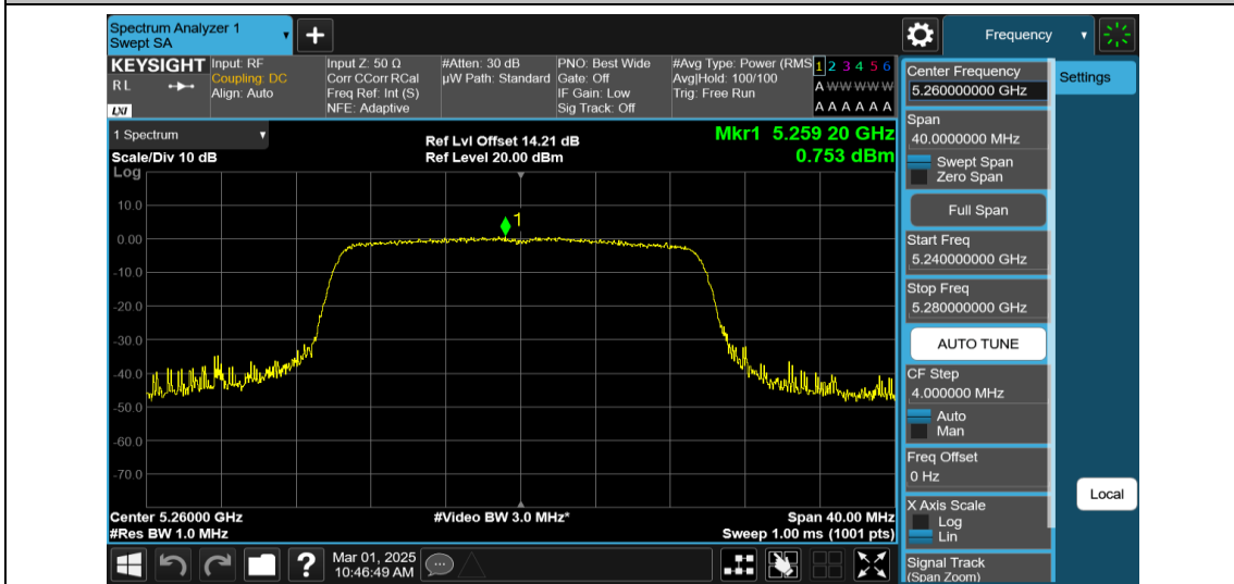
11AX20MIMO-Ant2-5260-PASS
