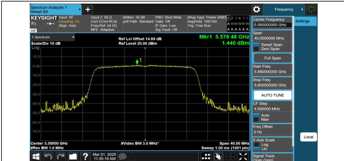
11AX20MIMO-Ant1-5580-PASS
