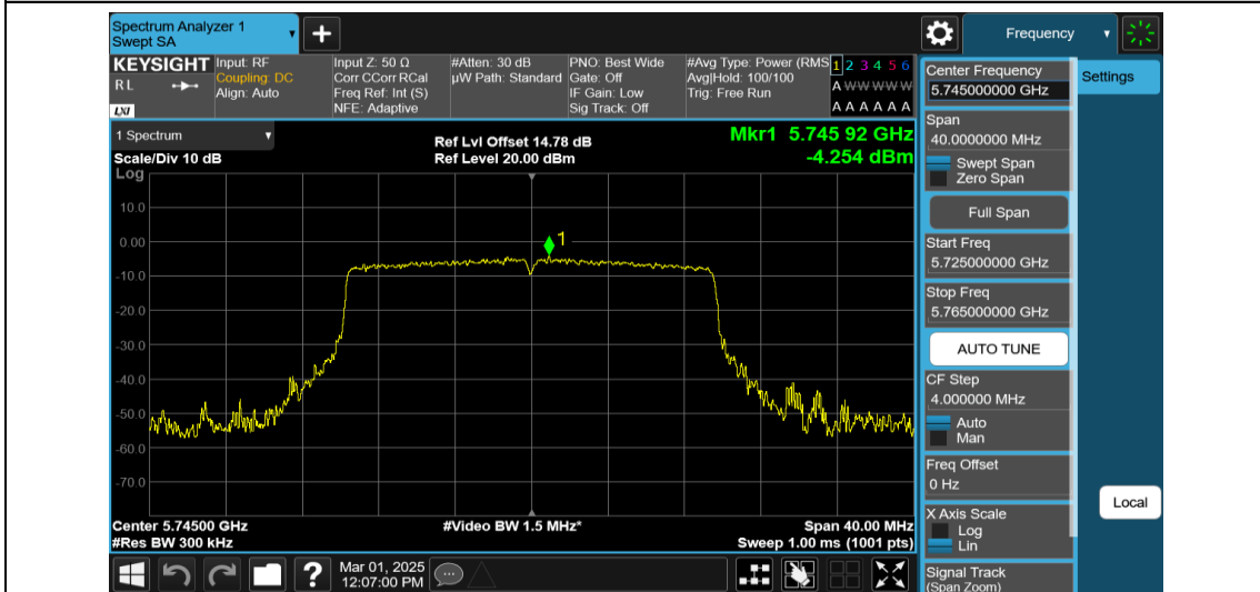
11AX20MIMO-Ant2-5745-PASS
