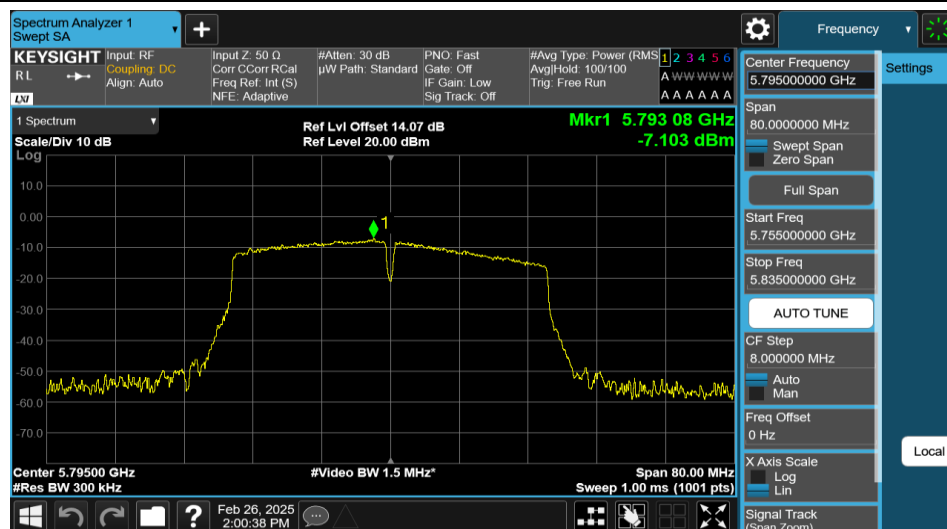
11AC40MIMO-Ant2-5795-PASS
