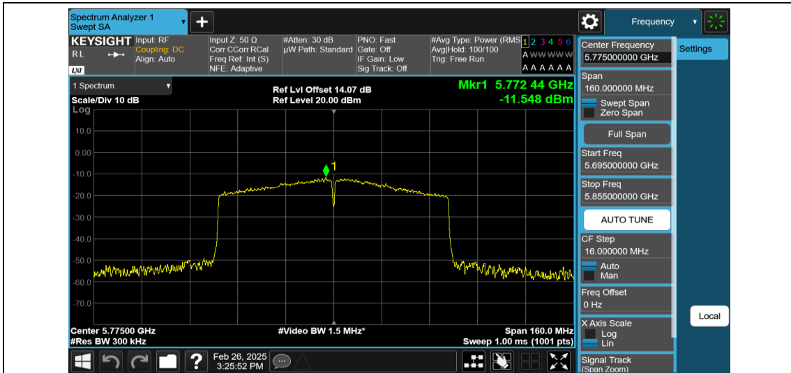
11AC80MIMO-Ant2-5775-PASS
