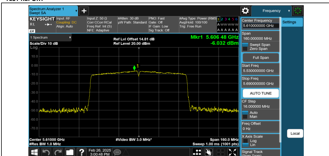
11AC80MIMO-Ant1-5610-PASS
