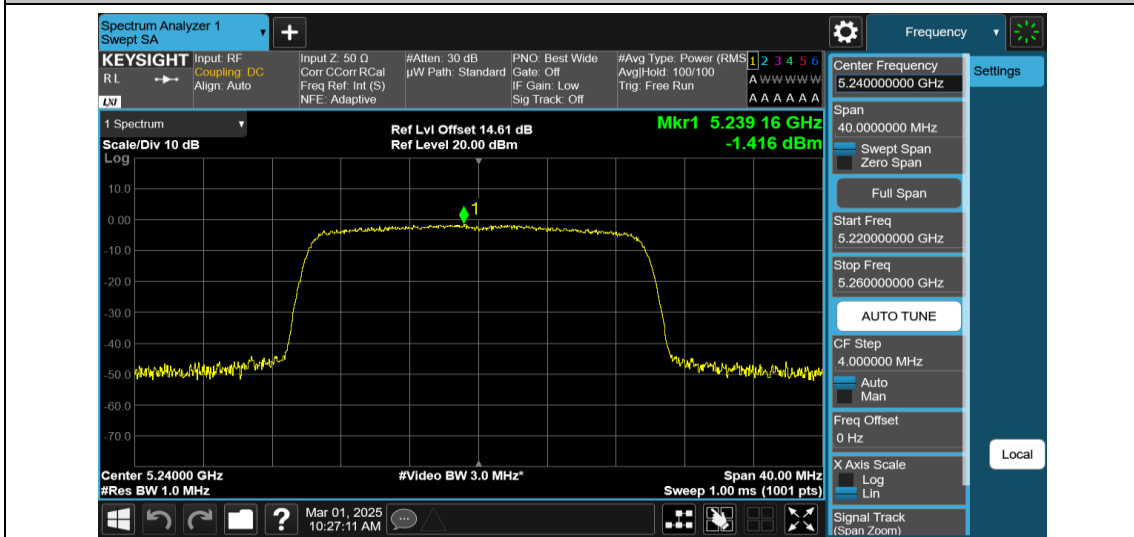
11AX20MIMO-Ant1-5240-PASS
