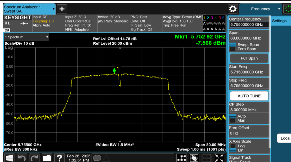
11AC40MIMO-Ant1-5755-PASS
