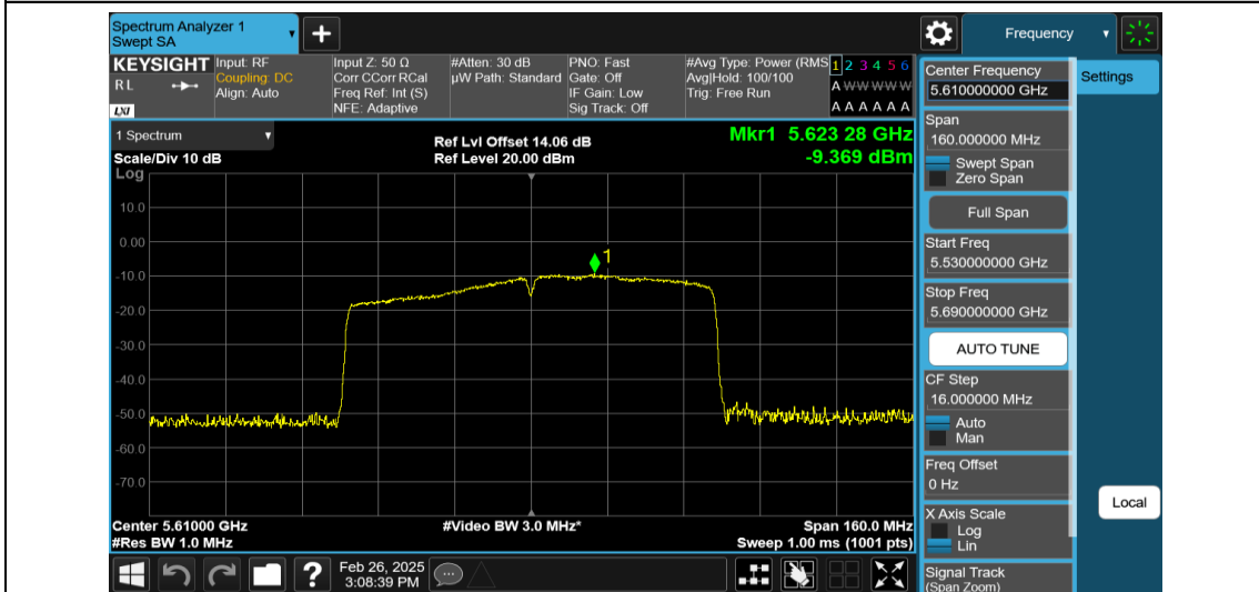
11AC80MIMO-Ant2-5610-PASS
