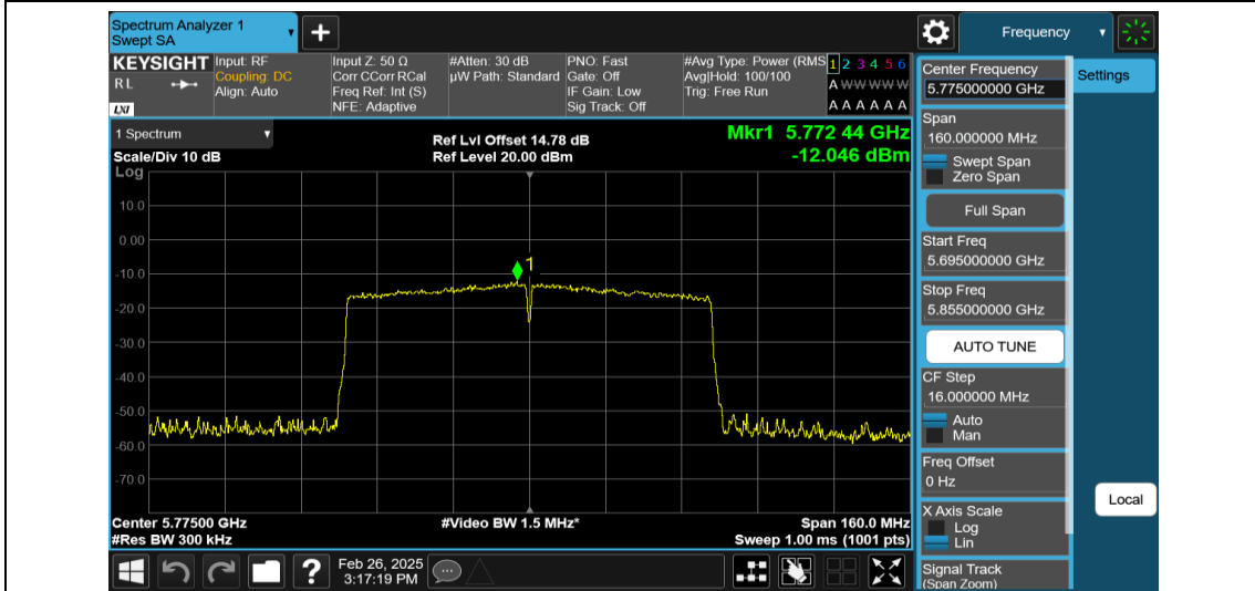
11AC80MIMO-Ant1-5775-PASS
