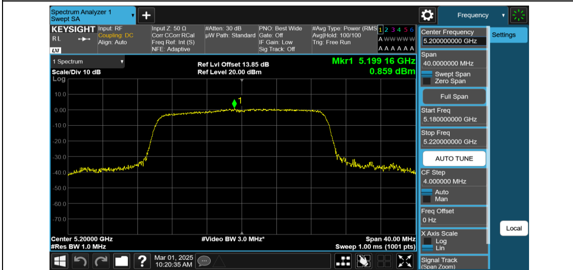
11AX20MIMO-Ant2-5200-PASS
