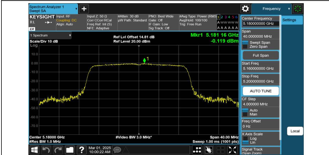
11AX20MIMO-Ant1-5180-PASS
