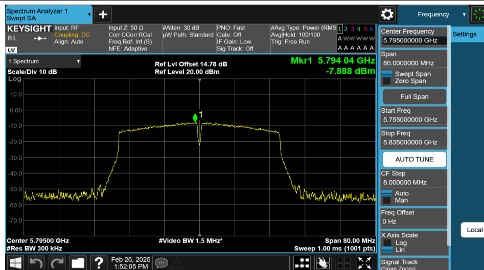
11AC40MIMO-Ant1-5795-PASS
