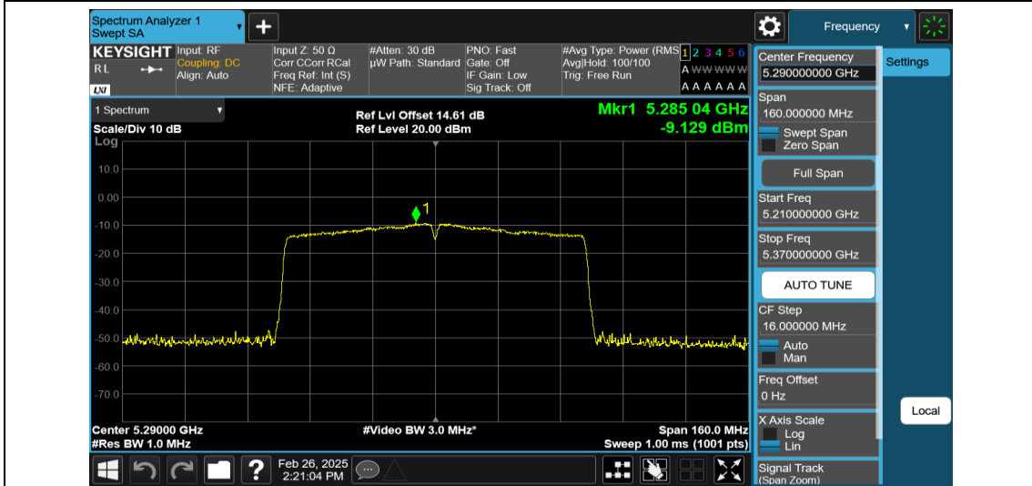
11AC80MIMO-Ant1-5290-PASS
