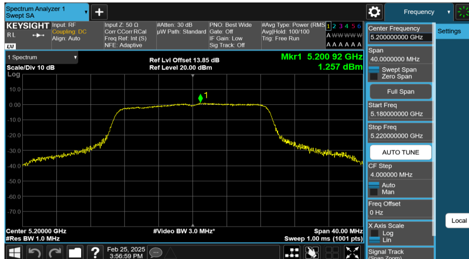
11AC20MIMO-Ant2-5200-PASS
