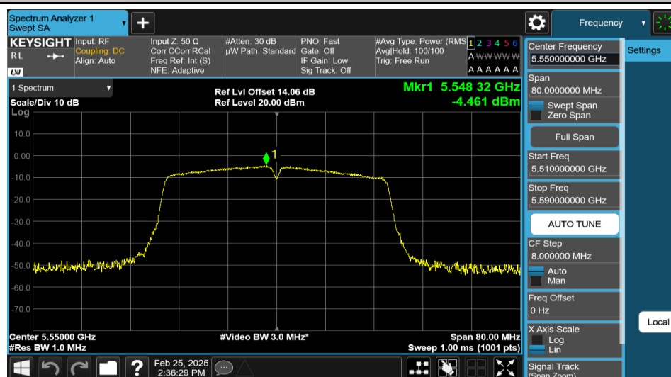
11N40MIMO-Ant2-5550-PASS
