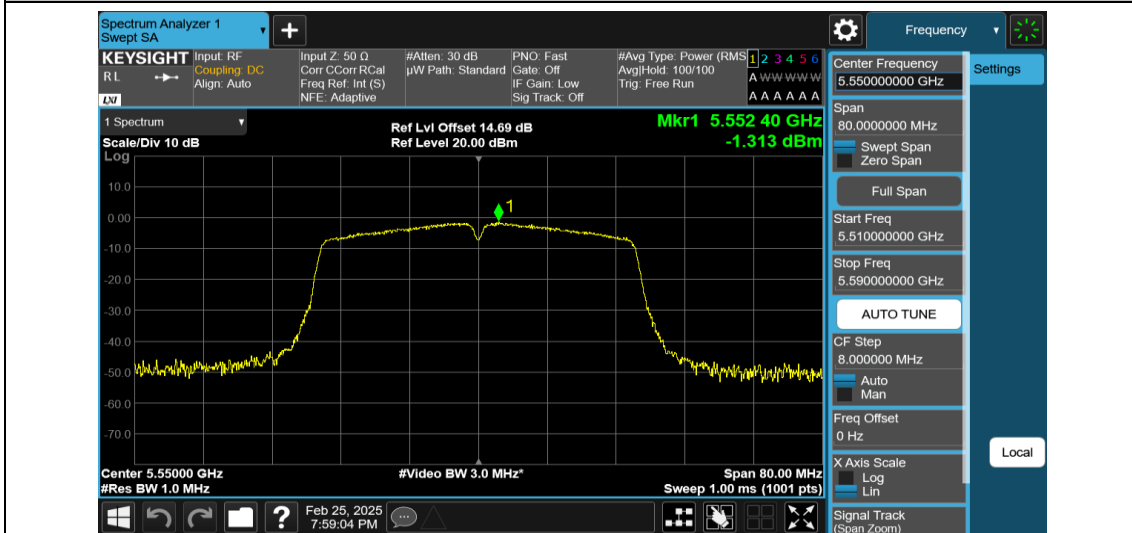
11AC40MIMO-Ant1-5550-PASS
