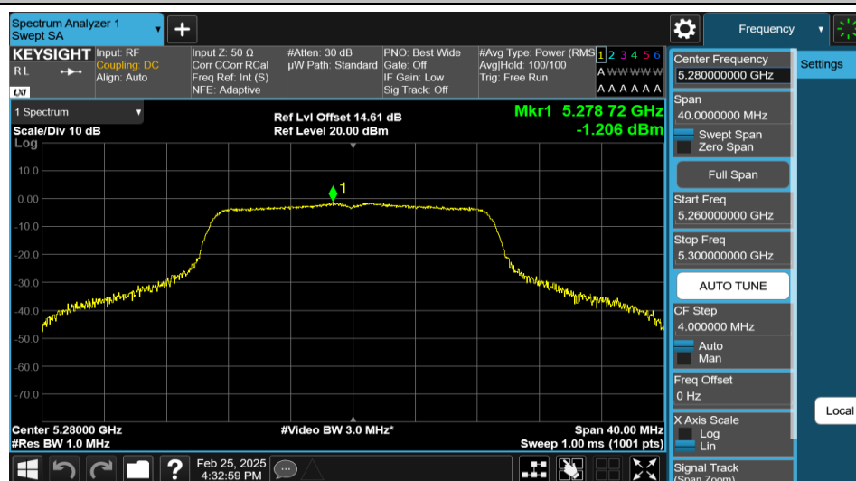
11AC20MIMO-Ant1-5280-PASS
