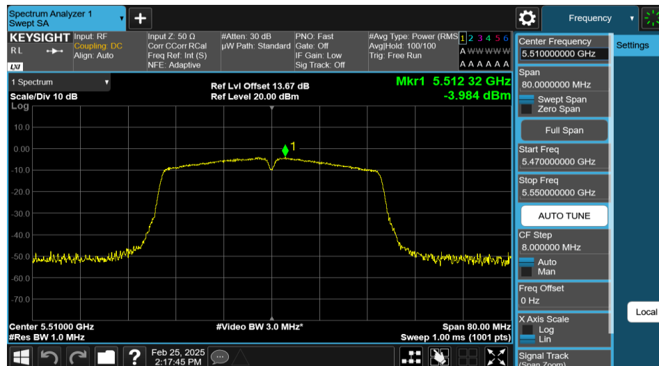
11N40MIMO-Ant2-5510-PASS
