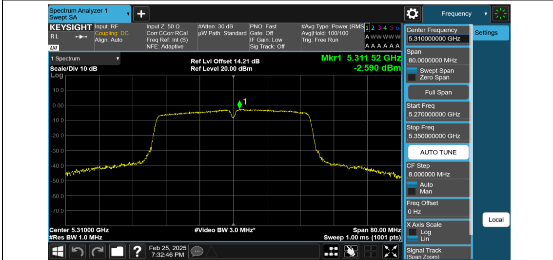
11AC40MIMO-Ant2-5310-PASS
