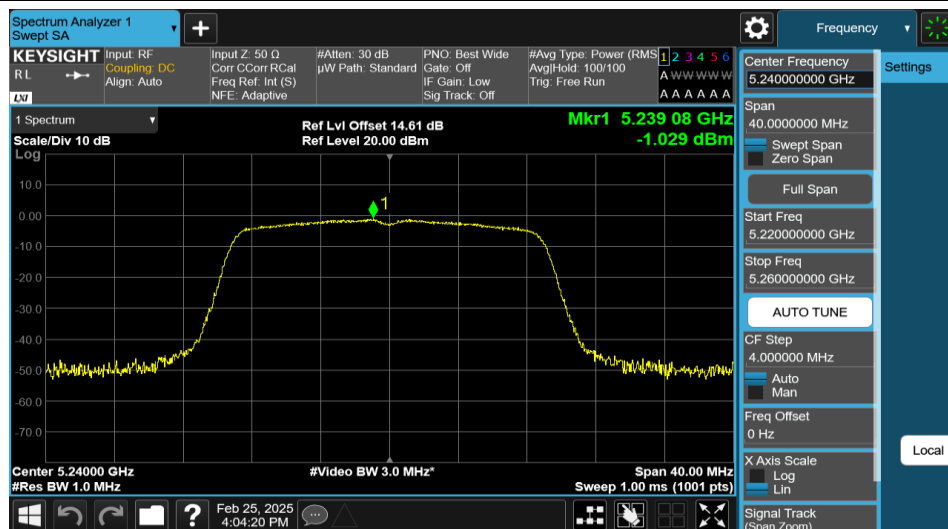
11AC20MIMO-Ant1-5240-PASS
