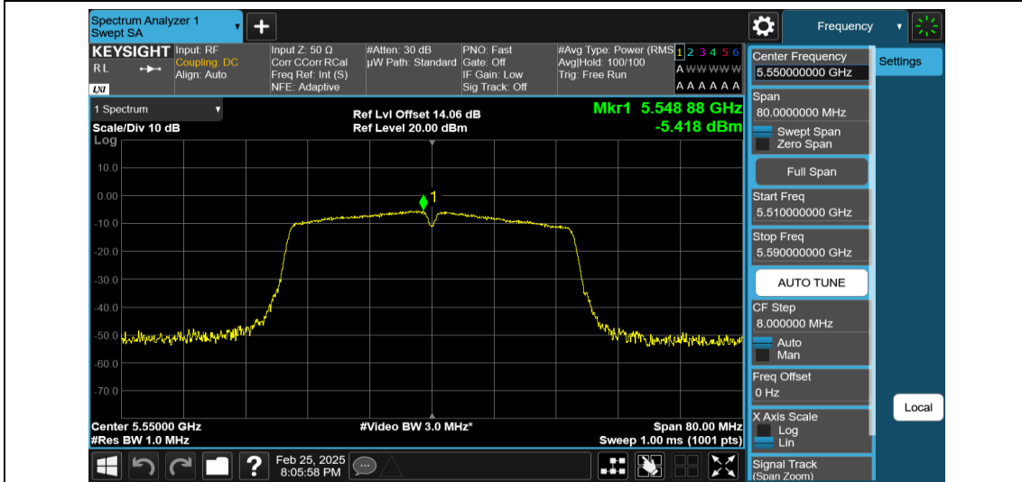
11AC40MIMO-Ant2-5550-PASS
