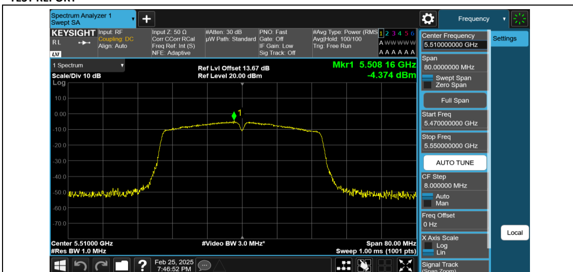
11AC40MIMO-Ant2-5510-PASS
