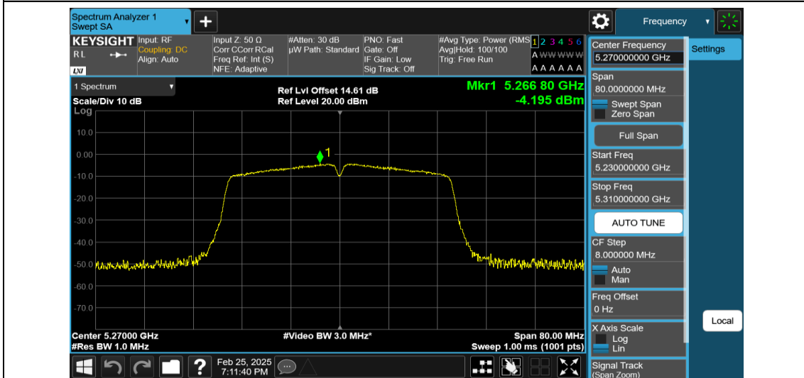
11AC40MIMO-Ant1-5270-PASS
