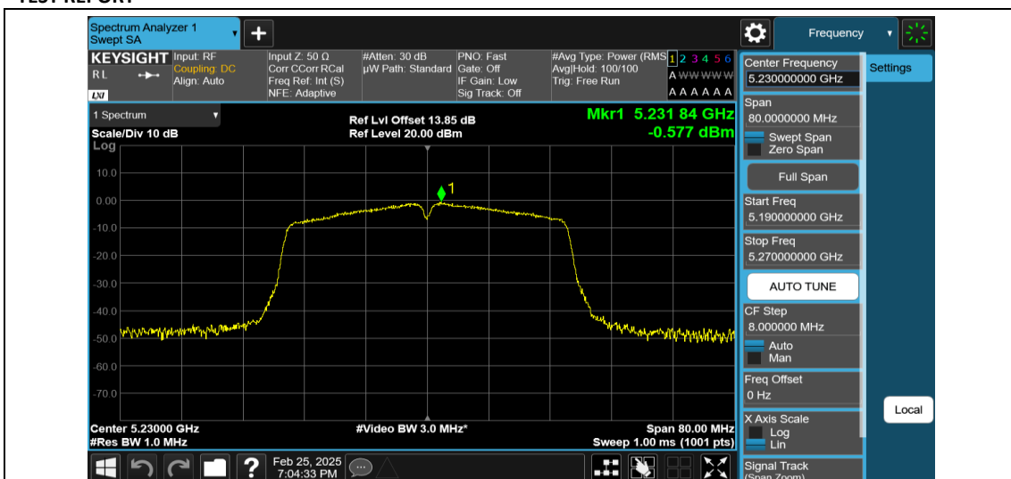
11AC40MIMO-Ant2-5230-PASS
