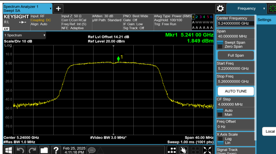
11AC20MIMO-Ant2-5240-PASS
