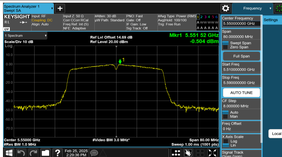
11N40MIMO-Ant1-5550-PASS
