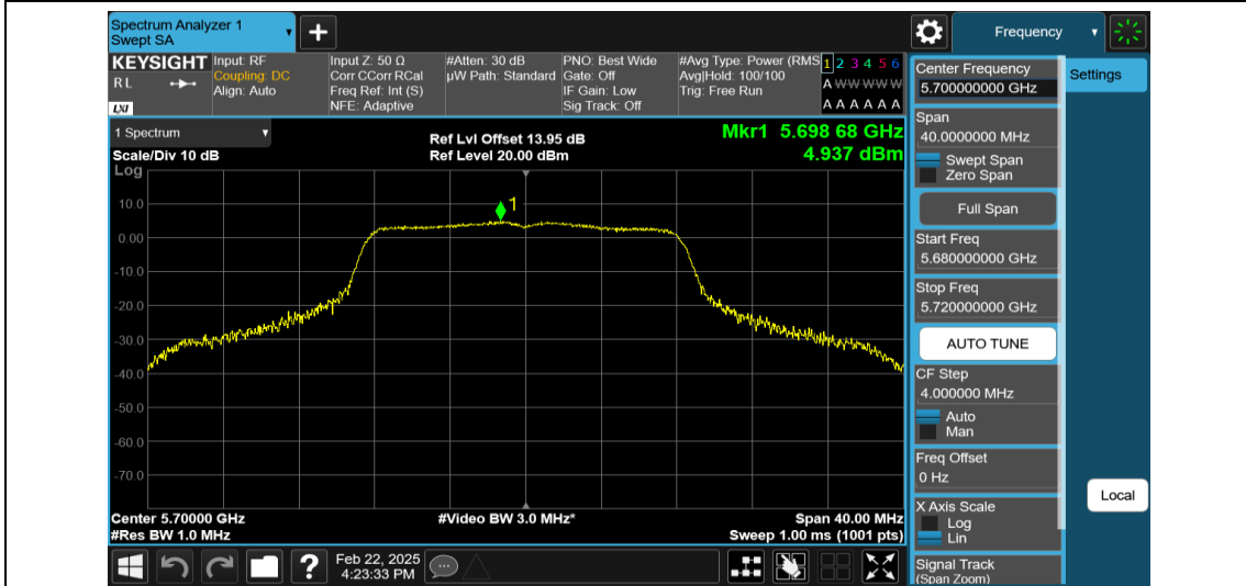
11A-Ant2-5700-PASS
