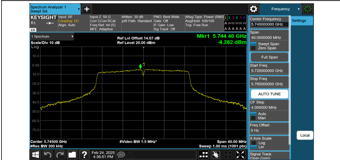
11N20MIMO-Ant2-5745-PASS
