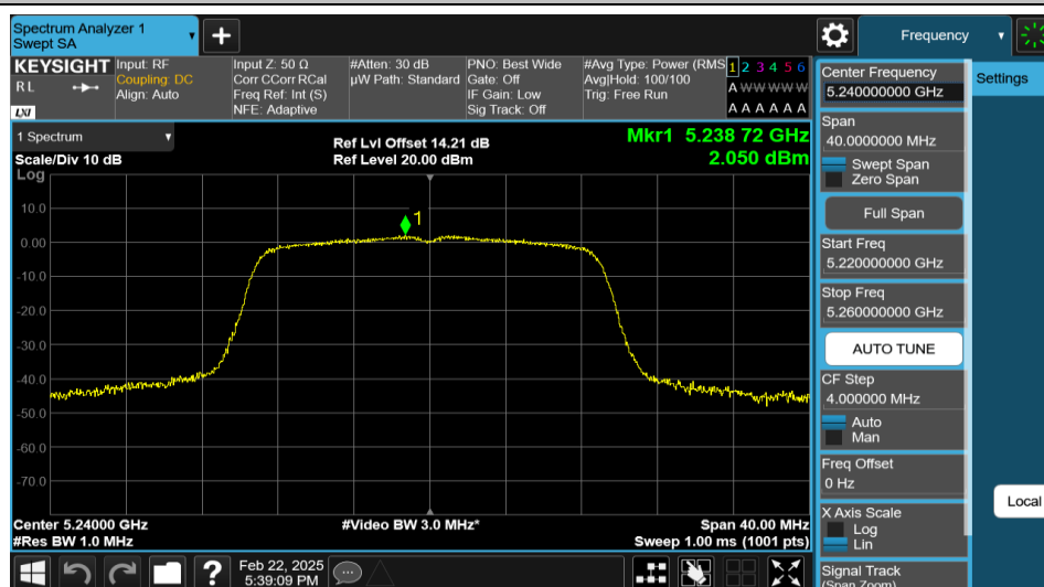
11N20MIMO-Ant2-5240-PASS
