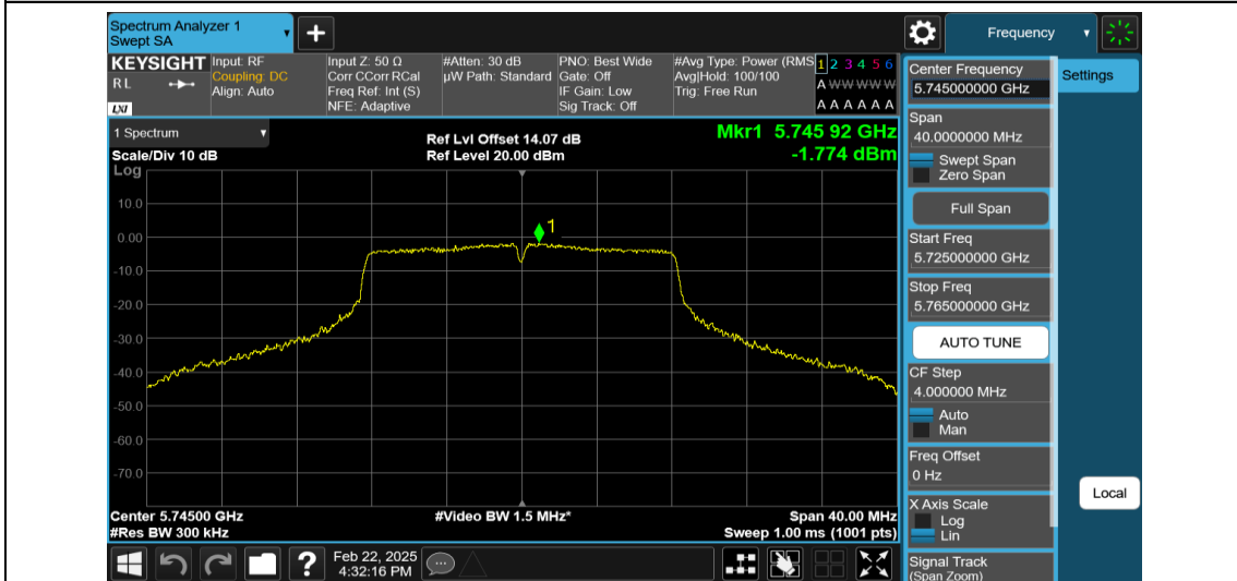
11A-Ant2-5745-PASS
