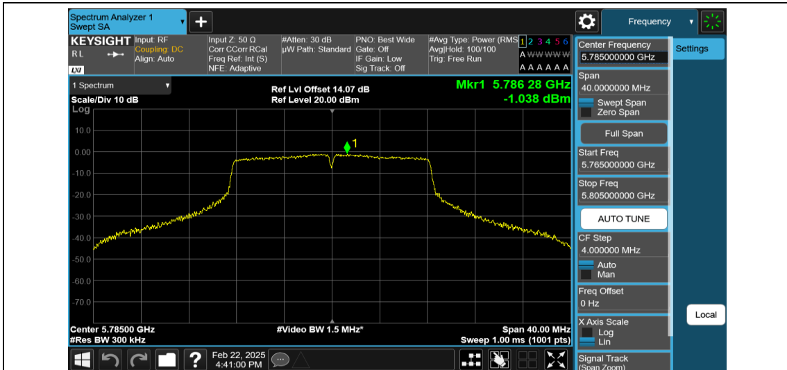
11A-Ant2-5785-PASS
