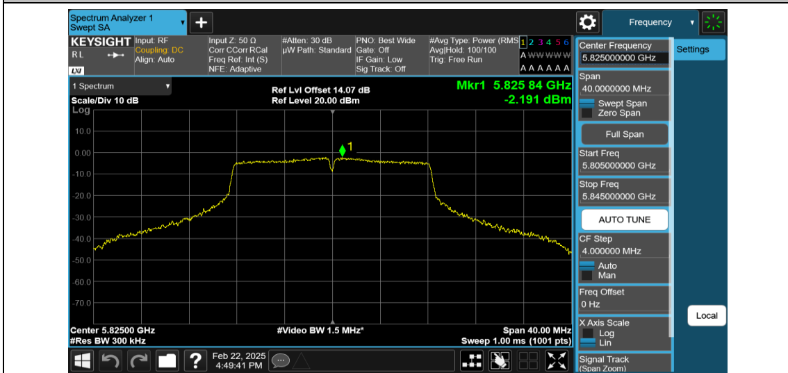
11A-Ant2-5825-PASS
