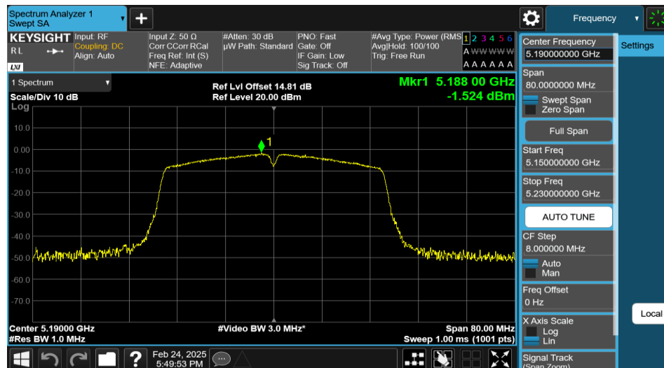
11N40MIMO-Ant1-5190-PASS
