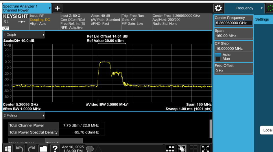
11AX80MIMO-Ant1-5290-106Tone-RU53-PASS
