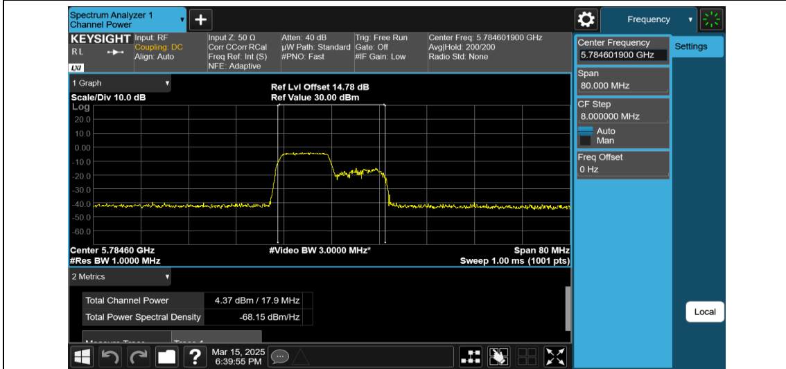
11AX40MIMO-Ant1-5795-106Tone-RU53-PASS
