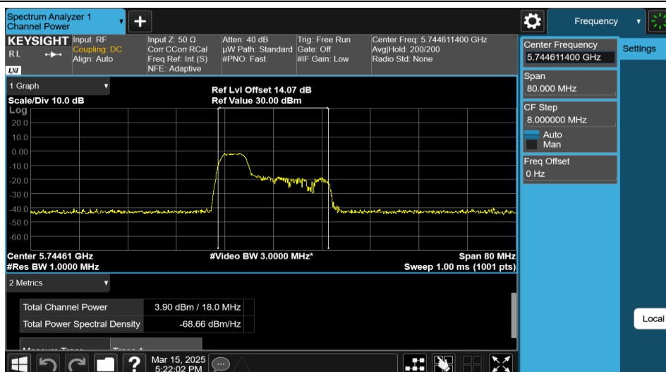
11AX40MIMO-Ant2-5755-52Tone-RU37-PASS
