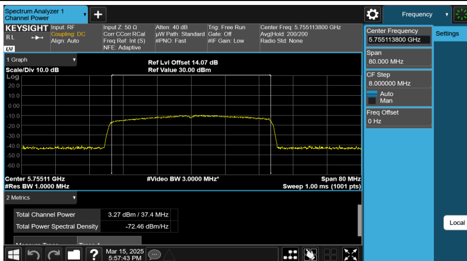
11AX40MIMO-Ant2-5755-484Tone-RU65-PASS
