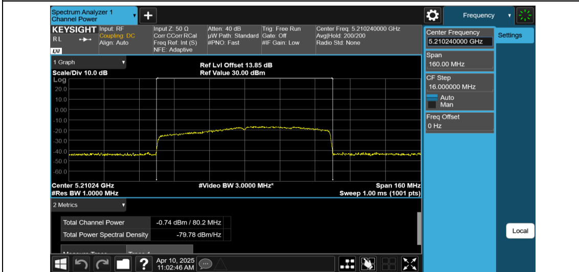
11AX80MIMO-Ant2-5210-996Tone-RU67-PASS
