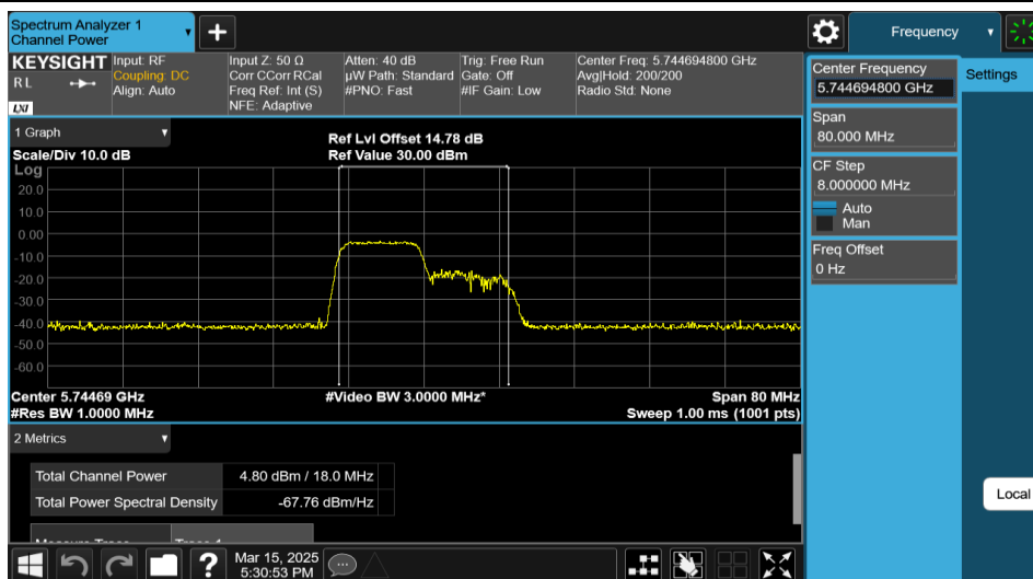
11AX40MIMO-Ant1-5755-106Tone-RU53-PASS
