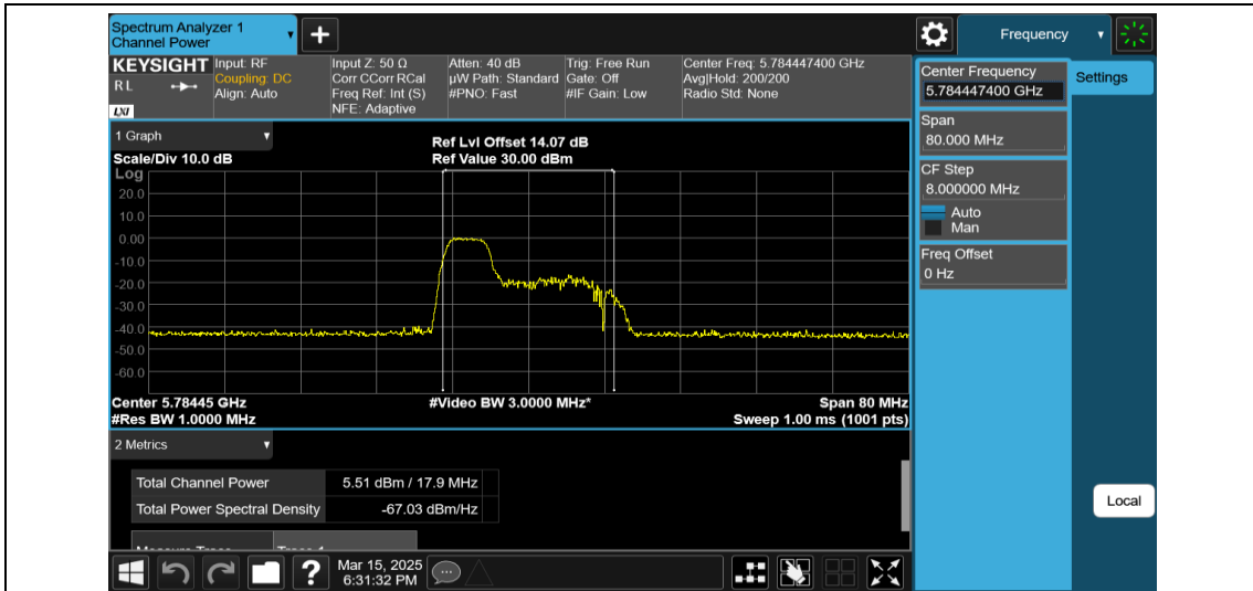
11AX40MIMO-Ant2-5795-52Tone-RU37-PASS
