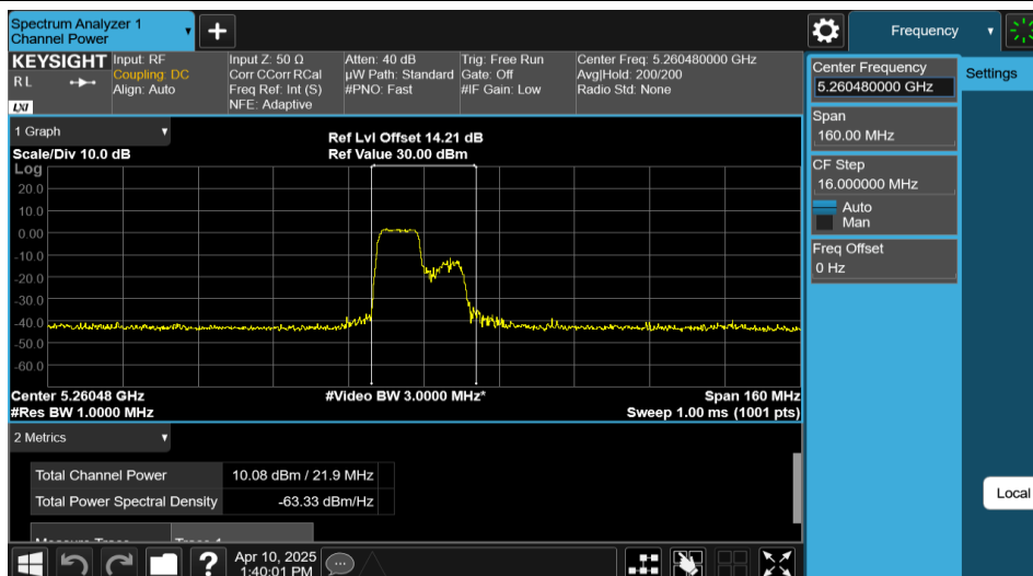
11AX80MIMO-Ant2-5290-106Tone-RU53-PASS
