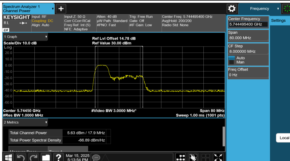
11AX40MIMO-Ant1-5755-52Tone-RU37-PASS
