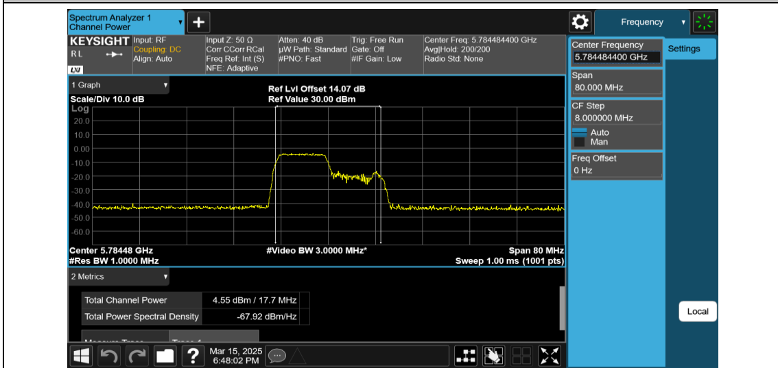
11AX40MIMO-Ant2-5795-106Tone-RU53-PASS
