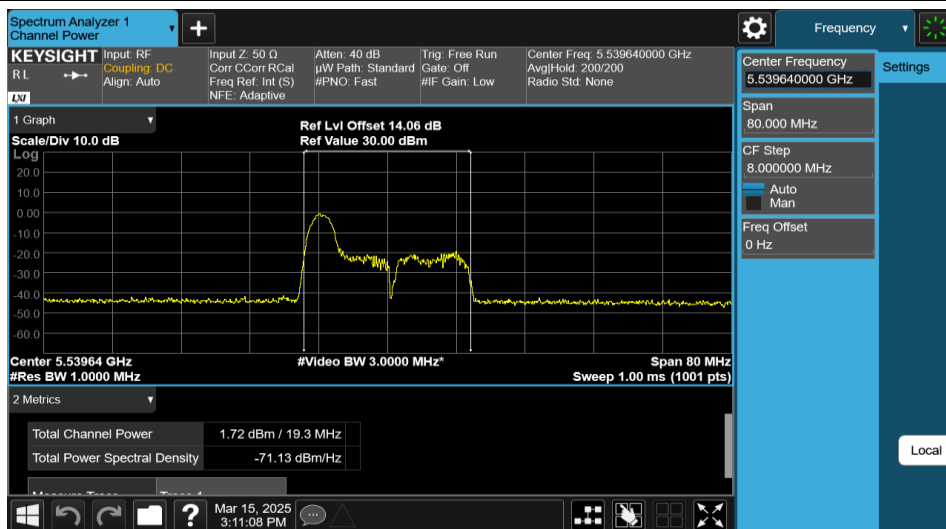
11AX40MIMO-Ant2-5550-26Tone-RU0-PASS
