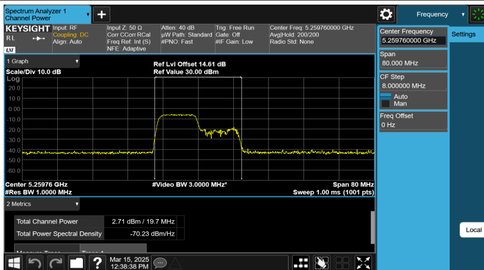
11AX40MIMO-Ant1-5270-106Tone-RU53-PASS
