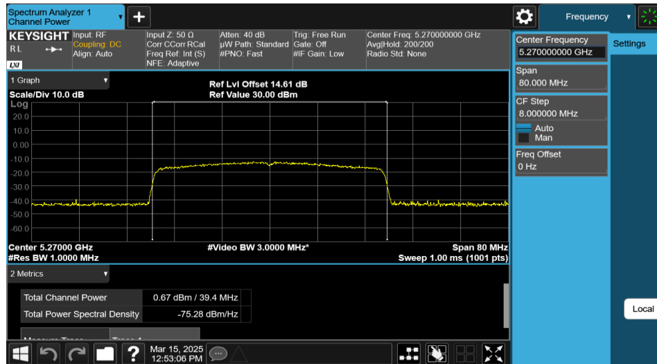
11AX40MIMO-Ant1-5270-484Tone-RU65-PASS
