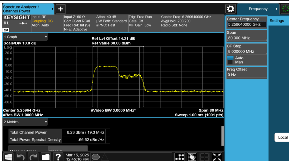
11AX40MIMO-Ant2-5270-106Tone-RU53-PASS
