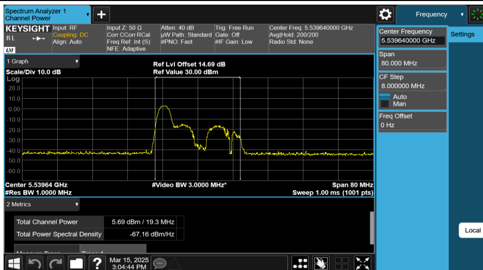
11AX40MIMO-Ant1-5550-26Tone-RU0-PASS
