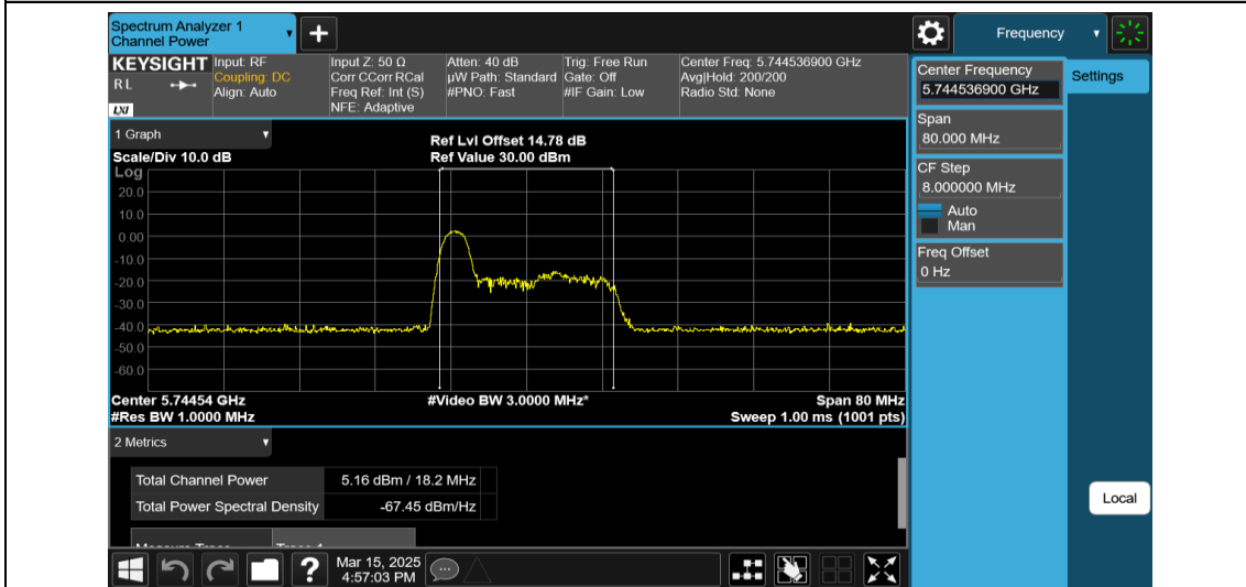
11AX40MIMO-Ant1-5755-26Tone-RU0-PASS
