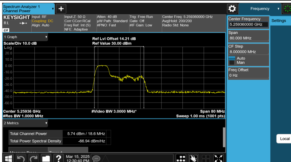
11AX40MIMO-Ant2-5270-52Tone-RU37-PASS
