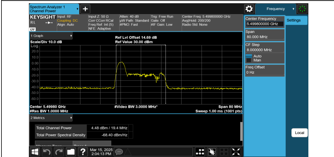
11AX40MIMO-Ant1-5510-26Tone-RU0-PASS
