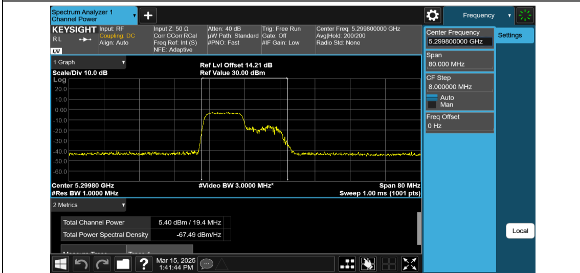
11AX40MIMO-Ant2-5310-106Tone-RU53-PASS
