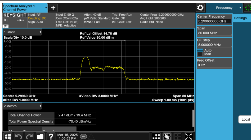
11AX40MIMO-Ant1-5310-26Tone-RU0-PASS
