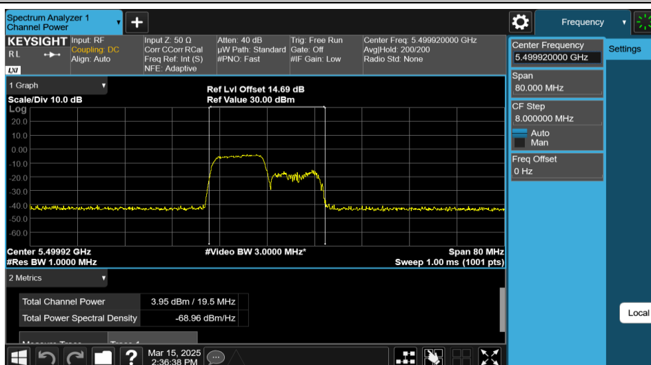
11AX40MIMO-Ant1-5510-106Tone-RU53-PASS
