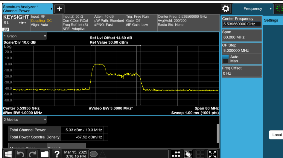
11AX40MIMO-Ant1-5550-52Tone-RU37-PASS
