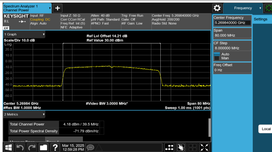
11AX40MIMO-Ant2-5270-484Tone-RU65-PASS
