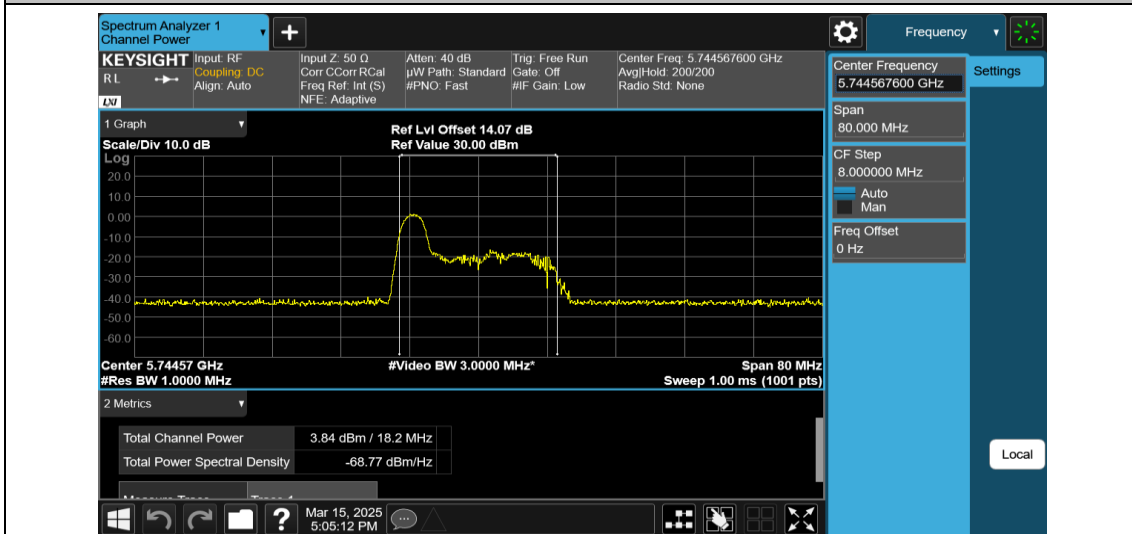
11AX40MIMO-Ant2-5755-26Tone-RU0-PASS
