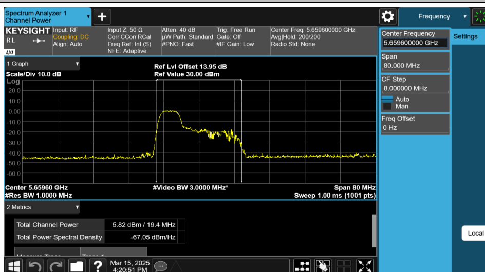
11AX40MIMO-Ant2-5670-52Tone-RU37-PASS
