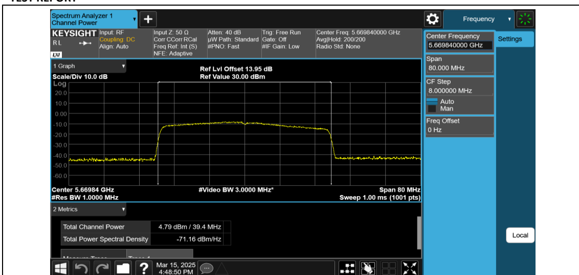
11AX40MIMO-Ant2-5670-484Tone-RU65-PASS
