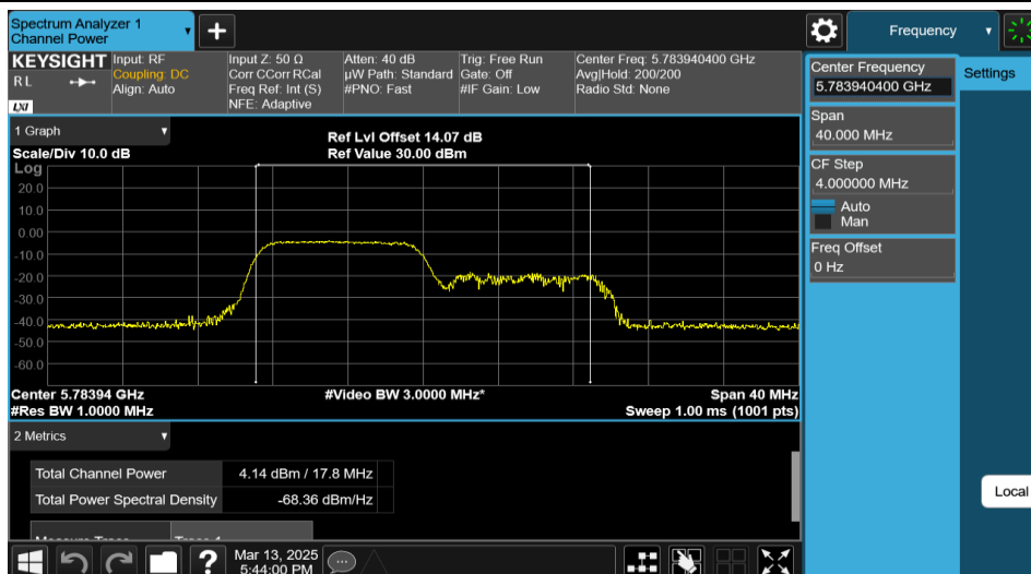
11AX20MIMO-Ant2-5785-106Tone-RU53-PASS
