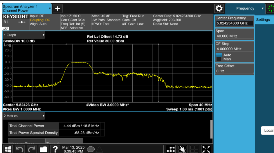
11AX20MIMO-Ant1-5825-52Tone-RU37-PASS
