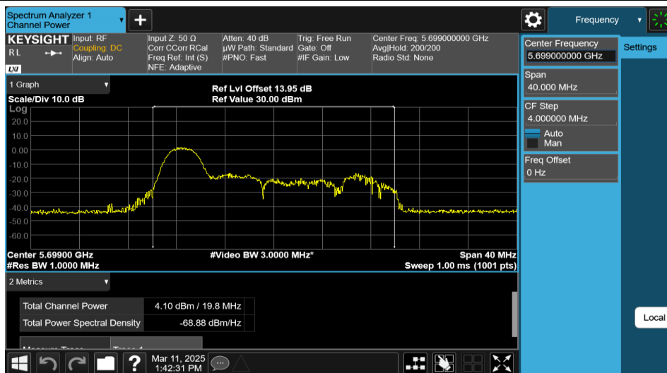
11AX20MIMO-Ant2-5700-26Tone-RU0-PASS
