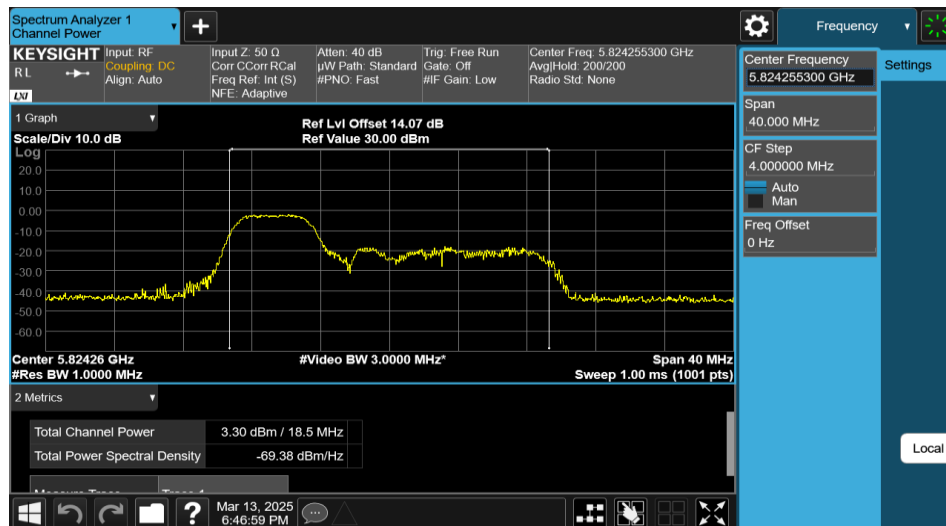
11AX20MIMO-Ant2-5825-52Tone-RU37-PASS
