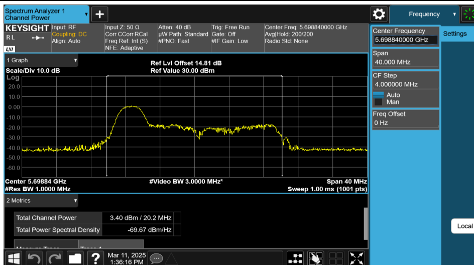
11AX20MIMO-Ant1-5700-26Tone-RU0-PASS
