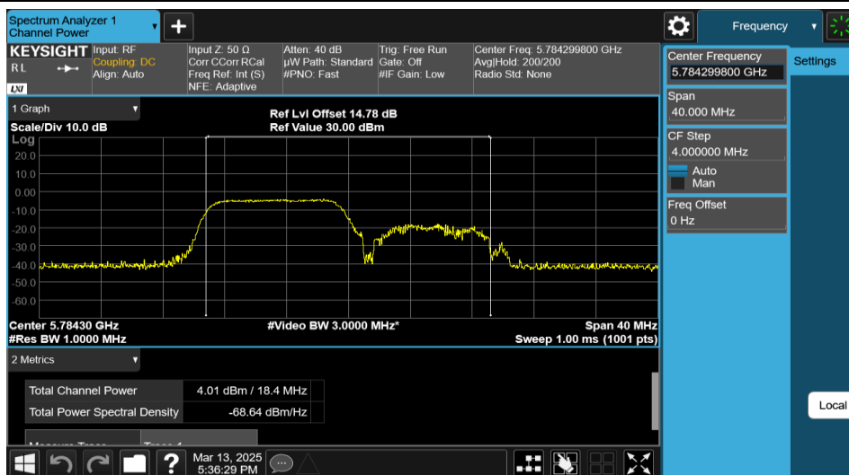
11AX20MIMO-Ant1-5785-106Tone-RU53-PASS
