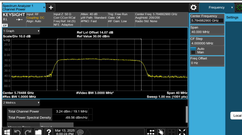
11AX20MIMO-Ant2-5785-242Tone-RU61-PASS
