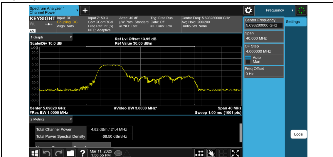
11AX20MIMO-Ant2-5700-52Tone-RU37-PASS
