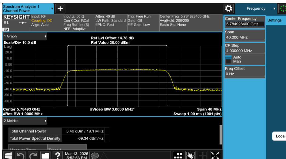
11AX20MIMO-Ant1-5785-242Tone-RU61-PASS
