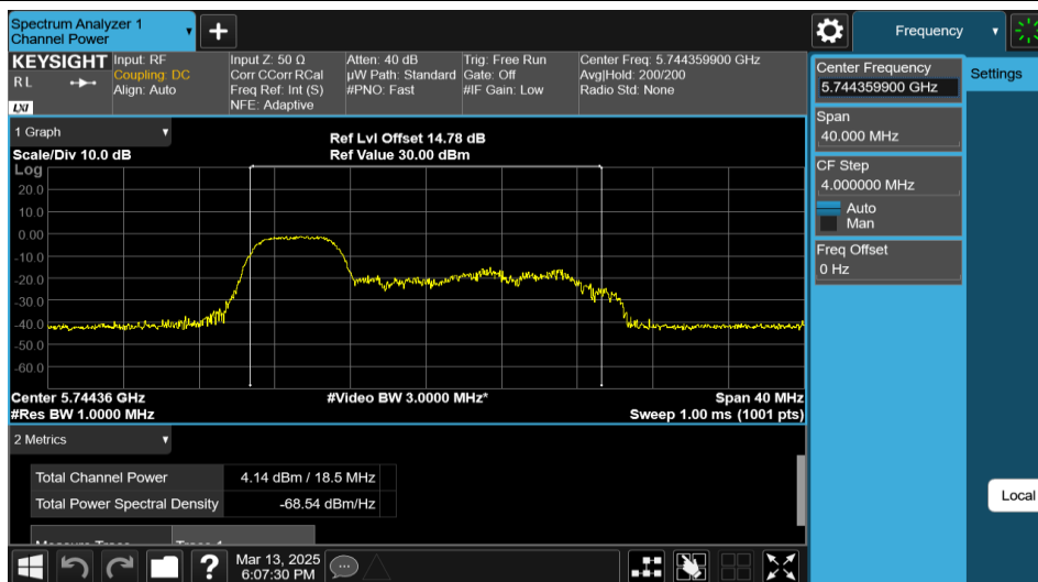
11AX20MIMO-Ant1-5745-52Tone-RU37-PASS
