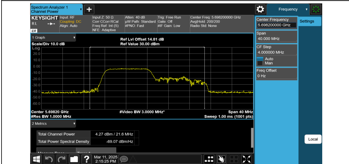
11AX20MIMO-Ant1-5700-106Tone-RU53-PASS
