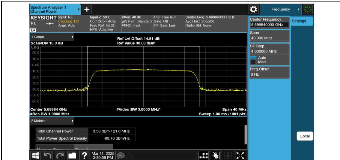
11AX20MIMO-Ant1-5700-242Tone-RU61-PASS
