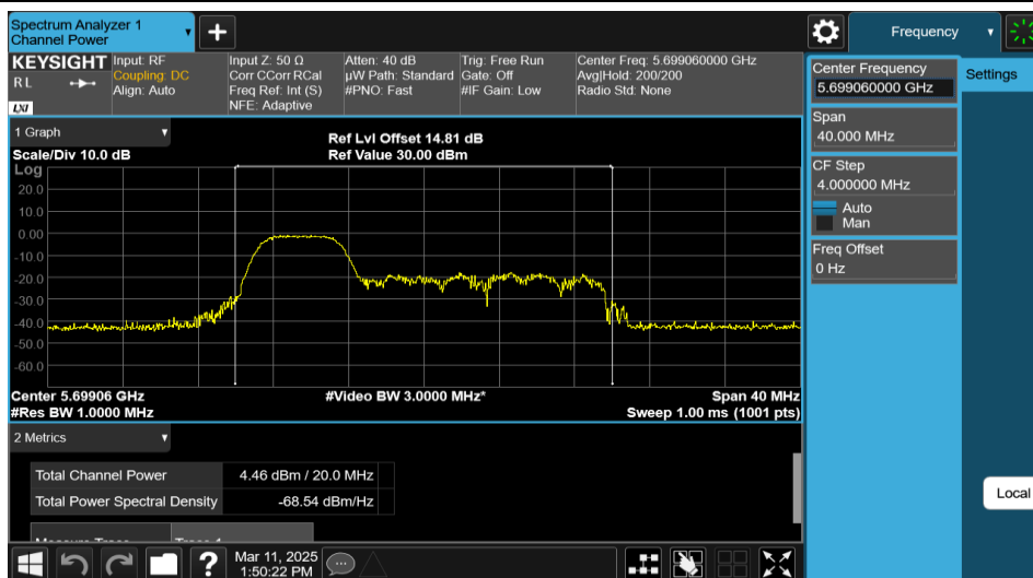
11AX20MIMO-Ant1-5700-52Tone-RU37-PASS
