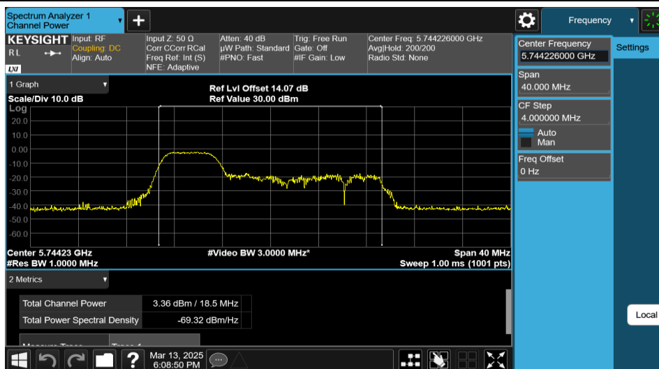
11AX20MIMO-Ant2-5745-52Tone-RU37-PASS
