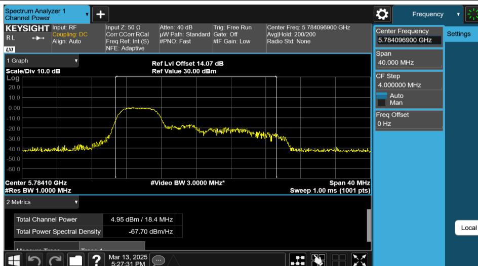
11AX20MIMO-Ant2-5785-52Tone-RU37-PASS
