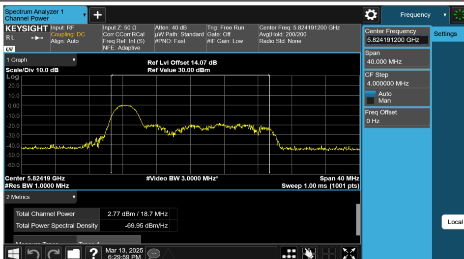
11AX20MIMO-Ant2-5825-26Tone-RU0-PASS
