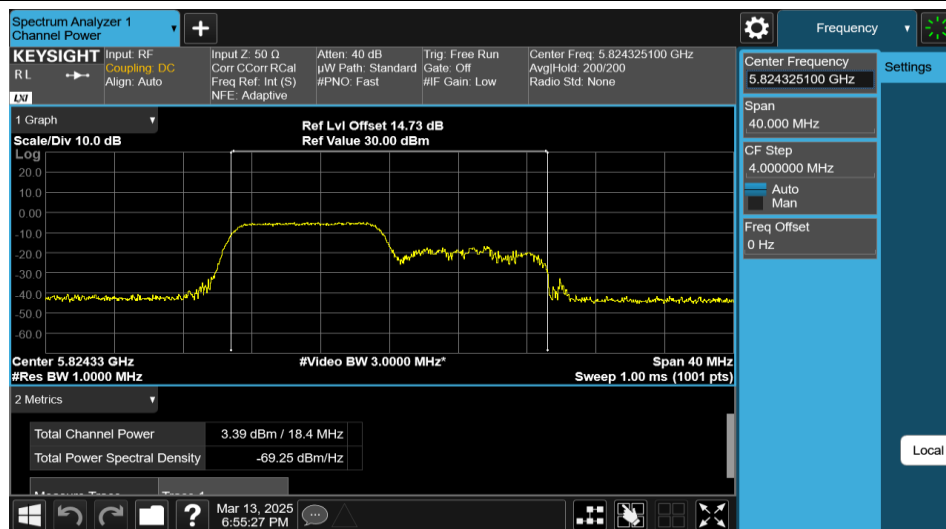
11AX20MIMO-Ant1-5825-106Tone-RU53-PASS
