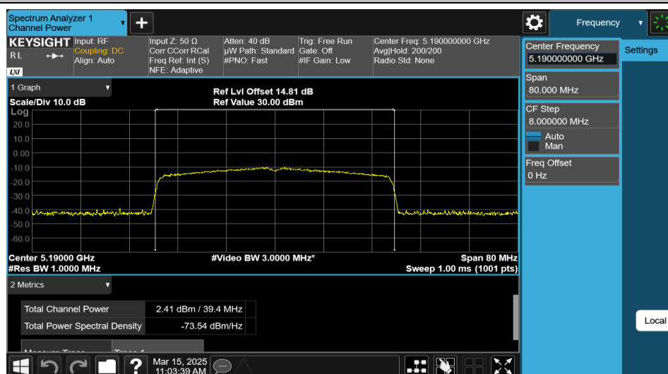
11AX40MIMO-Ant1-5190-484Tone-RU65-PASS
