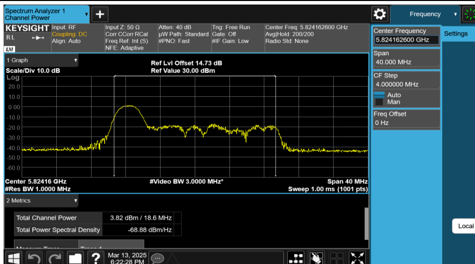
11AX20MIMO-Ant1-5825-26Tone-RU0-PASS
