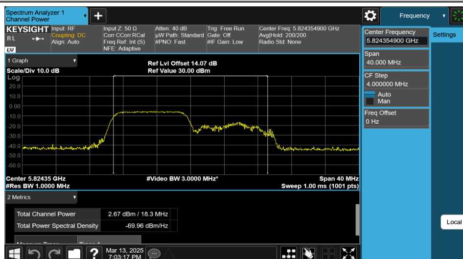
11AX20MIMO-Ant2-5825-106Tone-RU53-PASS
