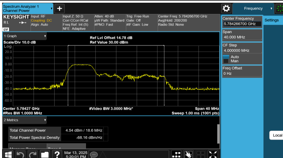
11AX20MIMO-Ant1-5785-52Tone-RU37-PASS
