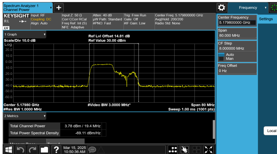
11AX40MIMO-Ant1-5190-106Tone-RU53-PASS
