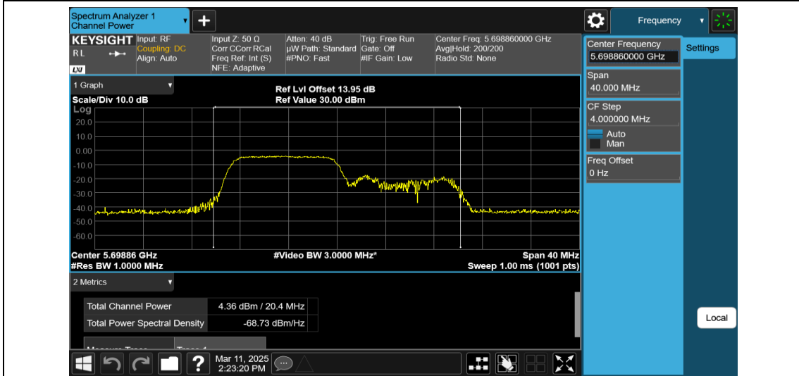
11AX20MIMO-Ant2-5700-106Tone-RU53-PASS
