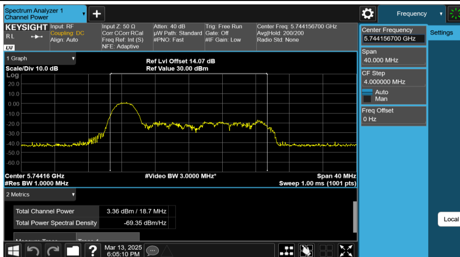
11AX20MIMO-Ant2-5745-26Tone-RU0-PASS
