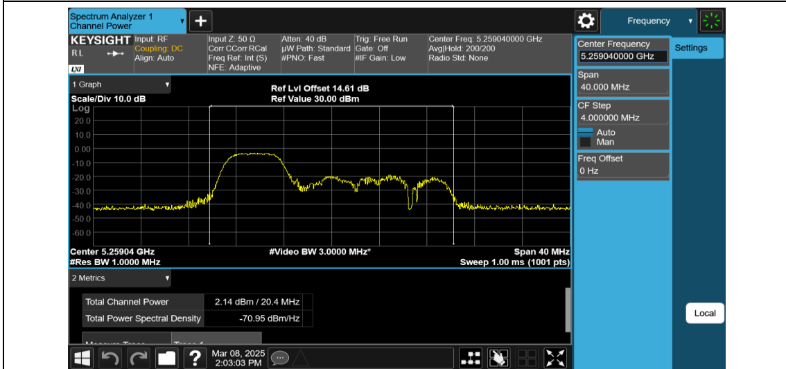
11AX20MIMO-Ant1-5260-52Tone-RU37-PASS
