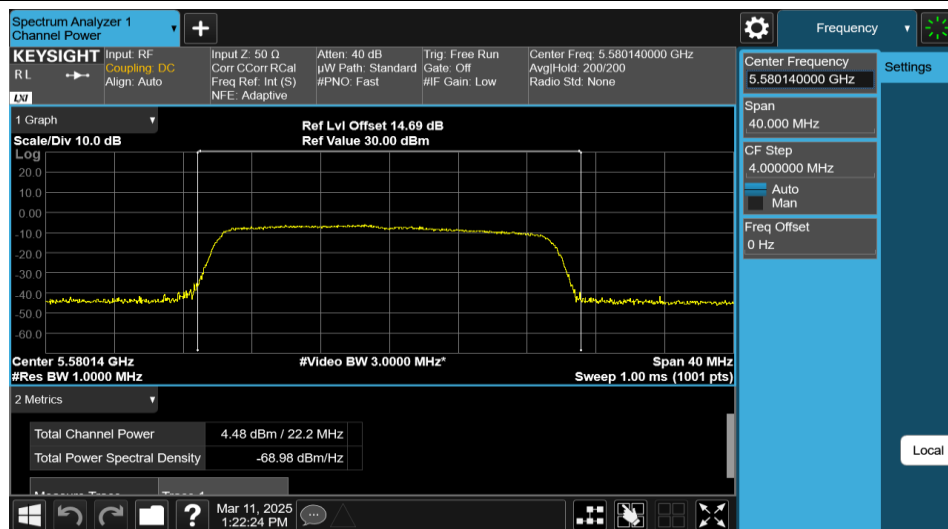
11AX20MIMO-Ant1-5580-242Tone-RU61-PASS
