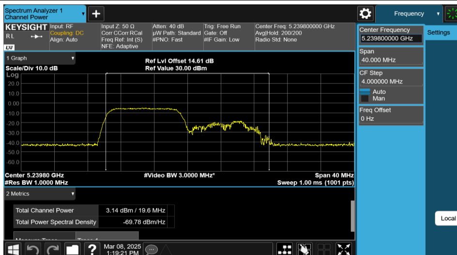
11AX20MIMO-Ant1-5240-106Tone-RU53-PASS
