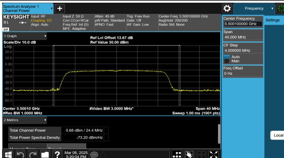
11AX20MIMO-Ant2-5500-242Tone-RU61-PASS
