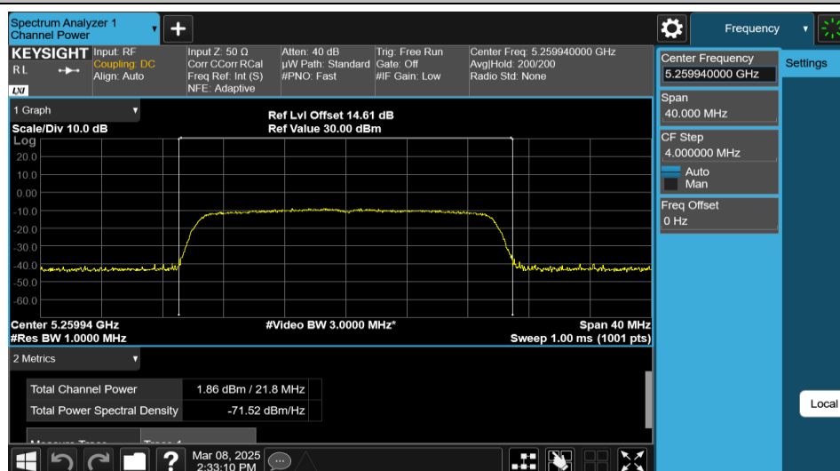
11AX20MIMO-Ant1-5260-242Tone-RU61-PASS
