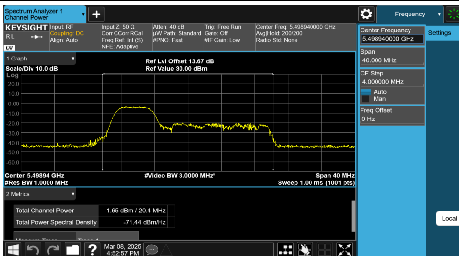
11AX20MIMO-Ant2-5500-52Tone-RU37-PASS
