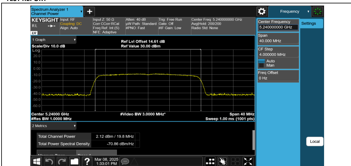
11AX20MIMO-Ant1-5240-242Tone-RU61-PASS
