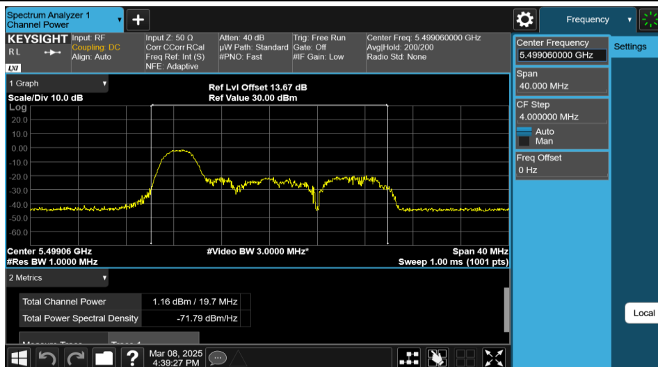
11AX20MIMO-Ant2-5500-26Tone-RU0-PASS
