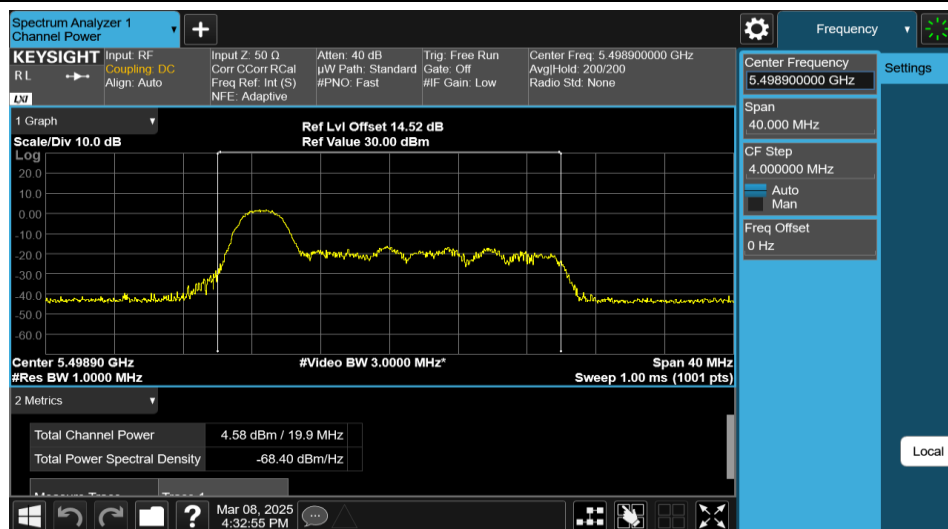
11AX20MIMO-Ant1-5500-26Tone-RU0-PASS
