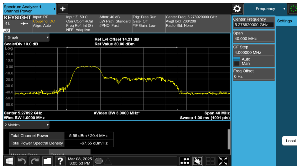
11AX20MIMO-Ant2-5280-52Tone-RU37-PASS
