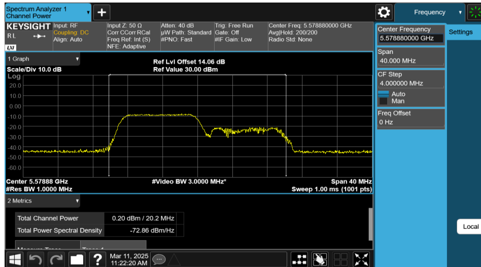
11AX20MIMO-Ant2-5580-106Tone-RU53-PASS
