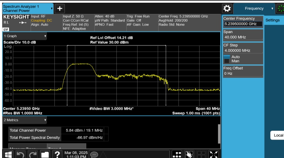
11AX20MIMO-Ant2-5240-52Tone-RU37-PASS
