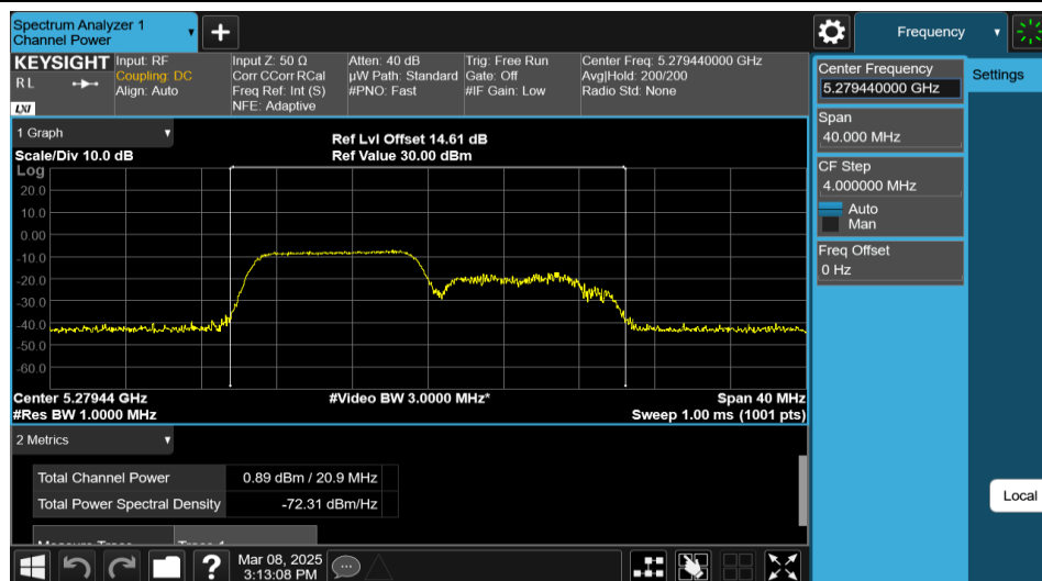
11AX20MIMO-Ant1-5280-106Tone-RU53-PASS
