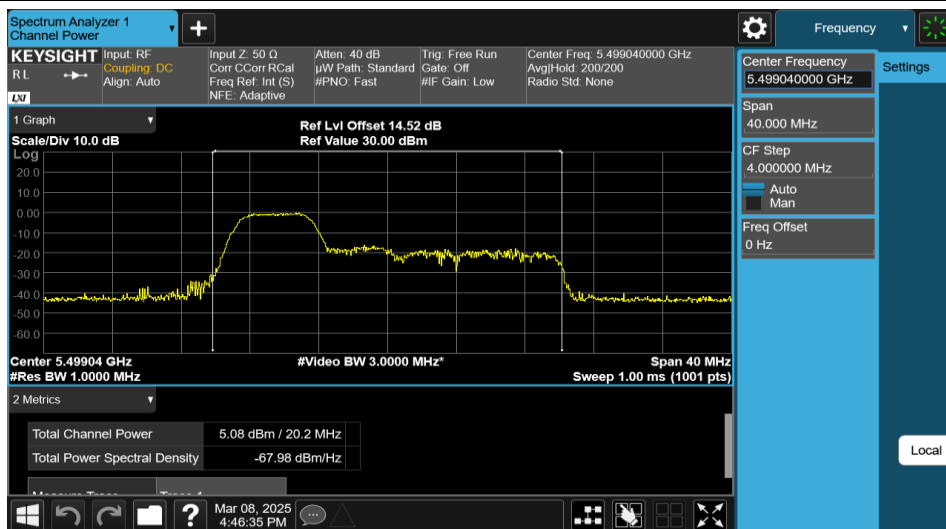
11AX20MIMO-Ant1-5500-52Tone-RU37-PASS
