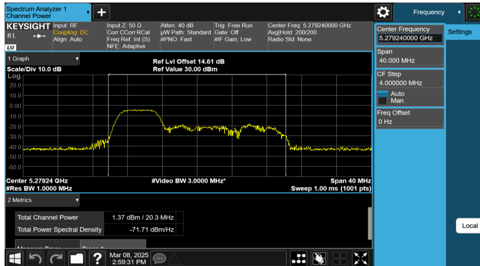
11AX20MIMO-Ant1-5280-52Tone-RU37-PASS
