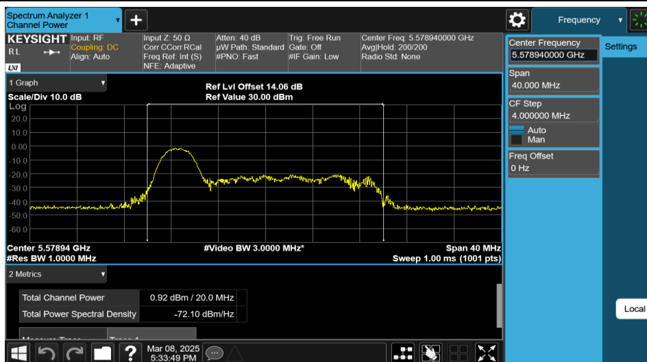
11AX20MIMO-Ant2-5580-26Tone-RU0-PASS
