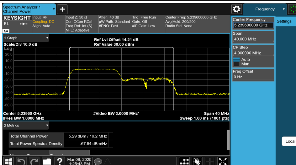
11AX20MIMO-Ant2-5240-106Tone-RU53-PASS
