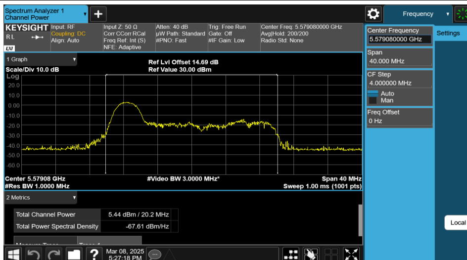
11AX20MIMO-Ant1-5580-26Tone-RU0-PASS
