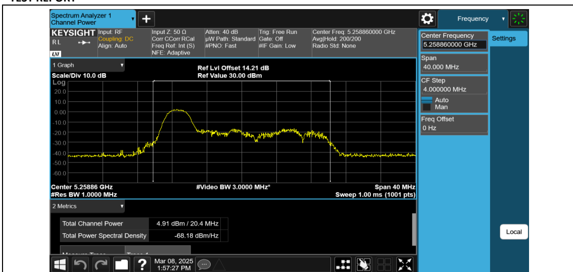
11AX20MIMO-Ant2-5260-26Tone-RU0-PASS
