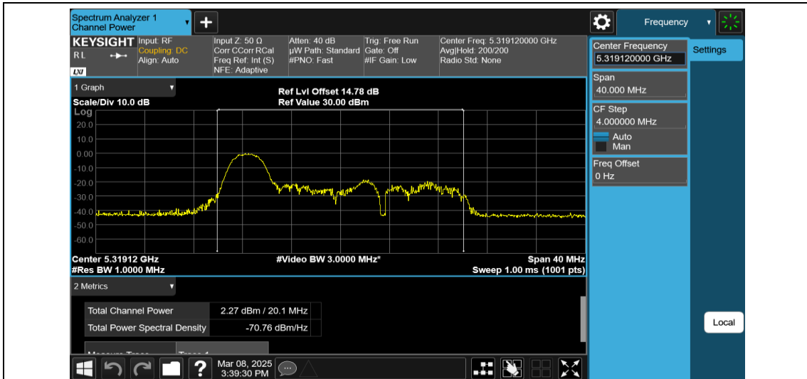
11AX20MIMO-Ant1-5320-26Tone-RU0-PASS
