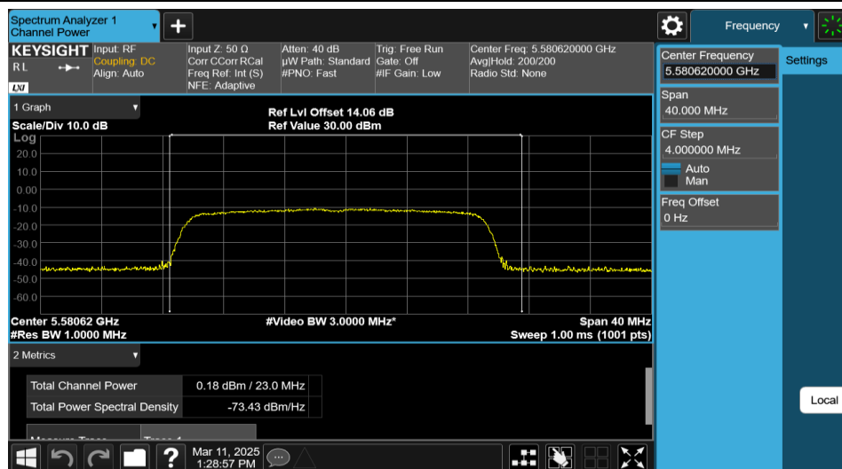
11AX20MIMO-Ant2-5580-242Tone-RU61-PASS
