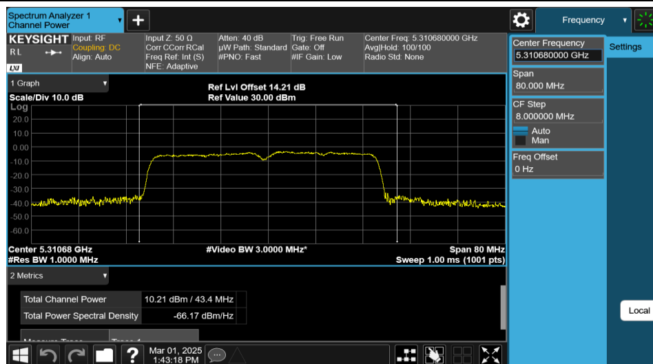
11AX40MIMO-Ant2-5310-PASS
