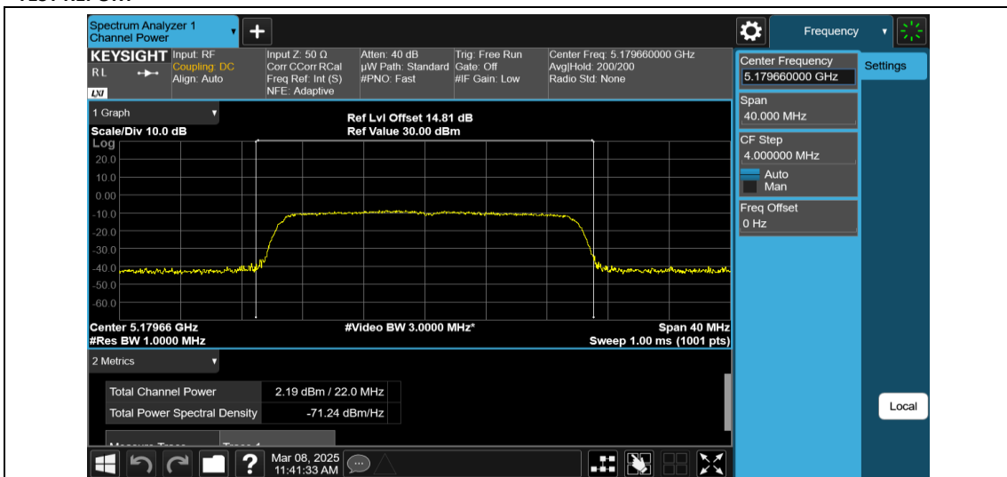
11AX20MIMO-Ant1-5180-242Tone-RU61-PASS
