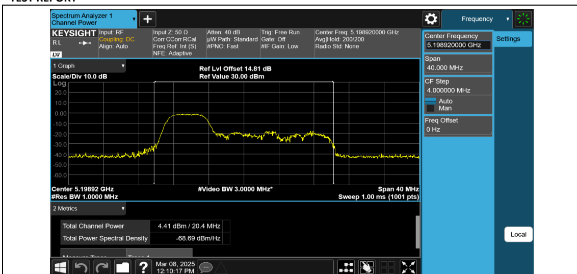
11AX20MIMO-Ant1-5200-52Tone-RU37-PASS
