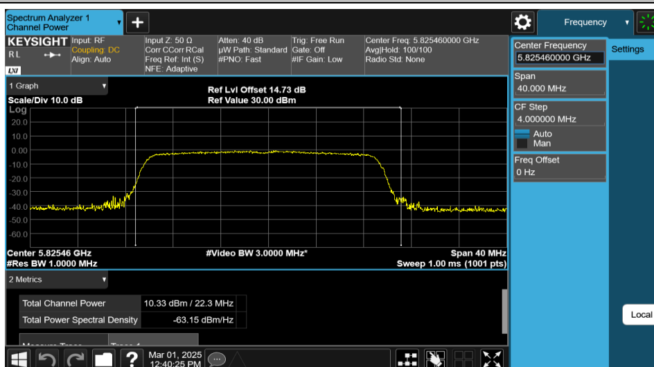
11AX20MIMO-Ant1-5825-PASS
