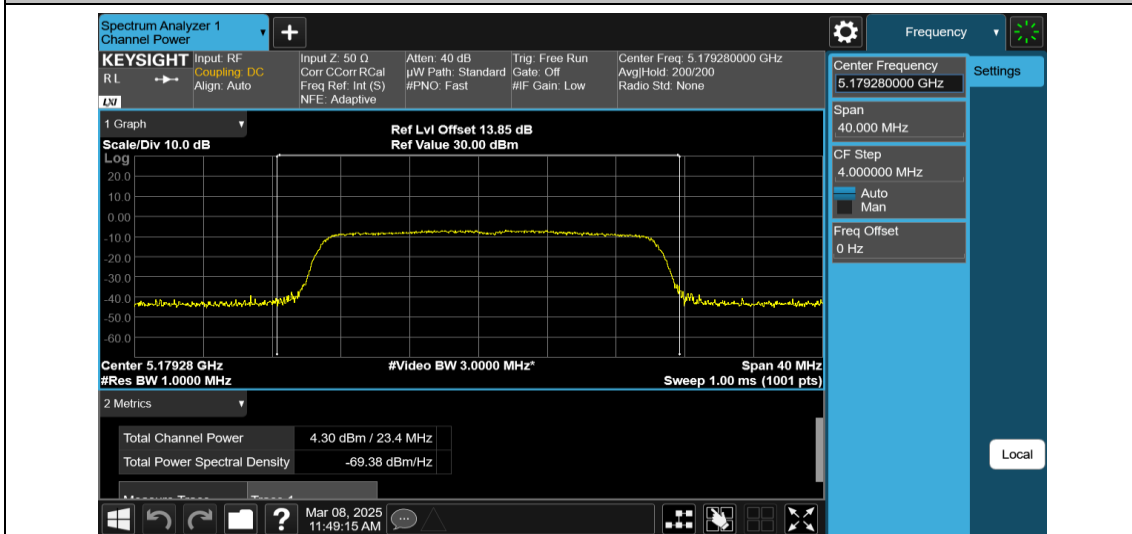
11AX20MIMO-Ant2-5180-242Tone-RU61-PASS
