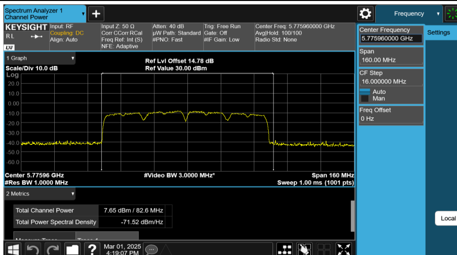
11AX80MIMO-Ant1-5775-PASS
