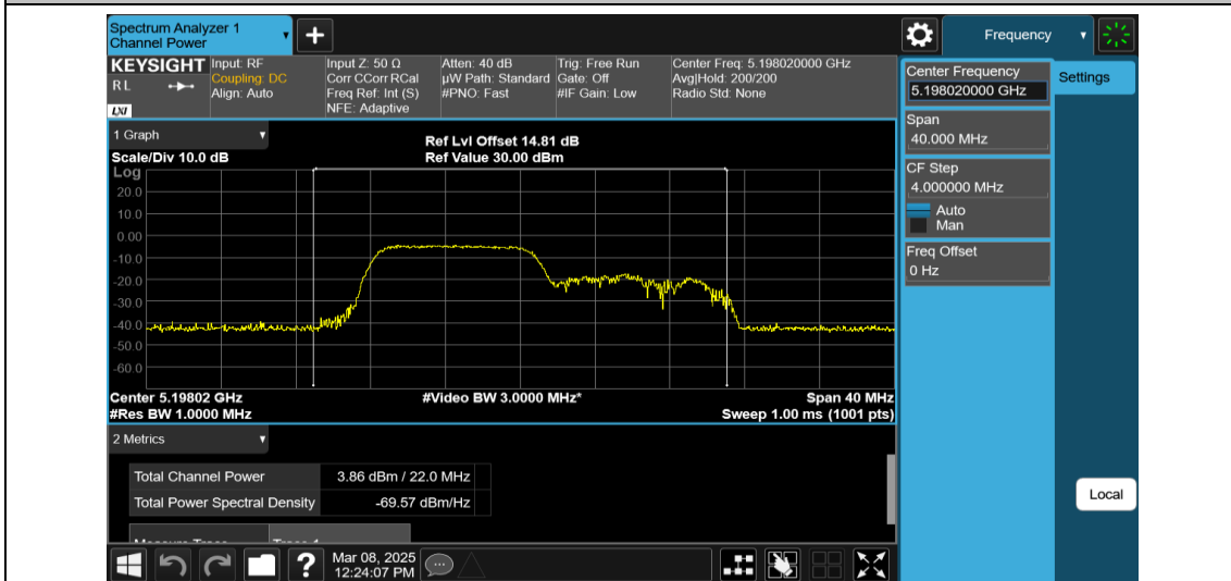
11AX20MIMO-Ant1-5200-106Tone-RU53-PASS
