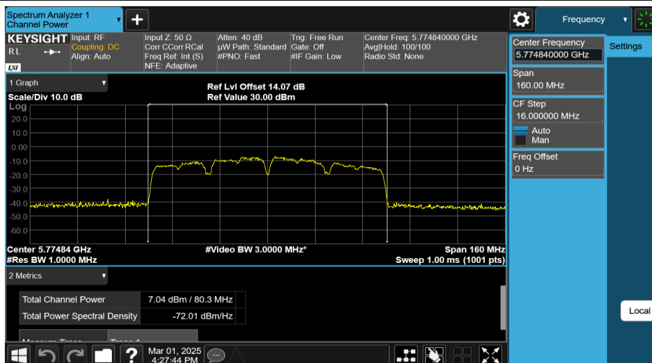
11AX80MIMO-Ant2-5775-PASS
