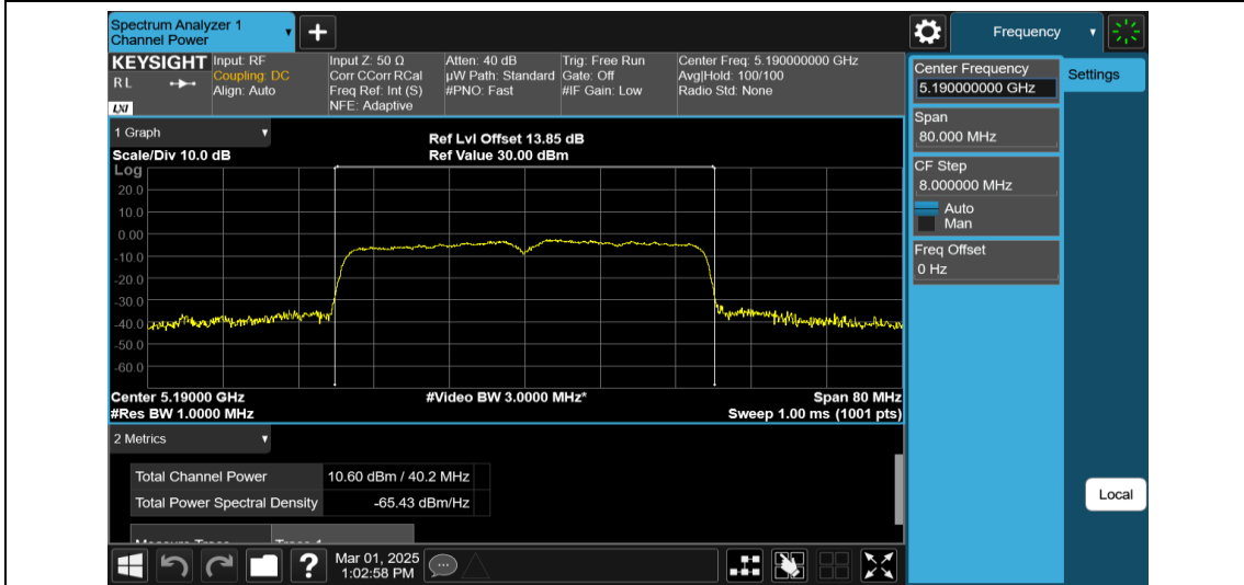
11AX40MIMO-Ant2-5190-PASS
