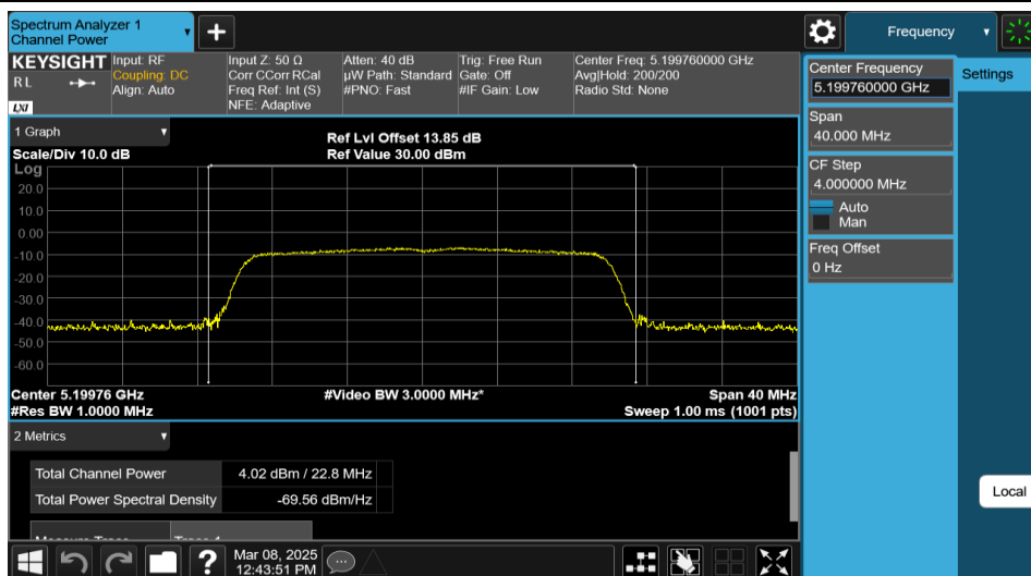
11AX20MIMO-Ant2-5200-242Tone-RU61-PASS
