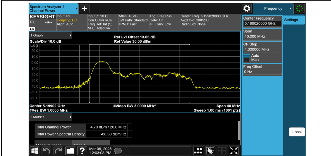
11AX20MIMO-Ant2-5200-26Tone-RU0-PASS
