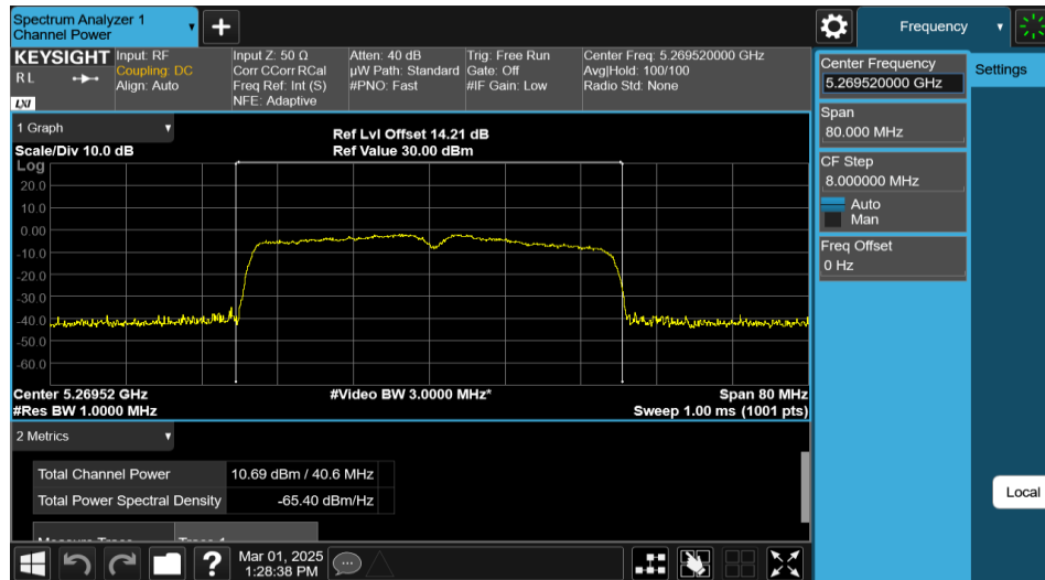
11AX40MIMO-Ant2-5270-PASS
