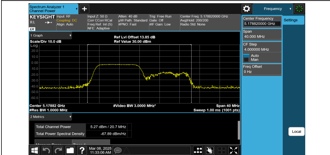
11AX20MIMO-Ant2-5180-106Tone-RU53-PASS
