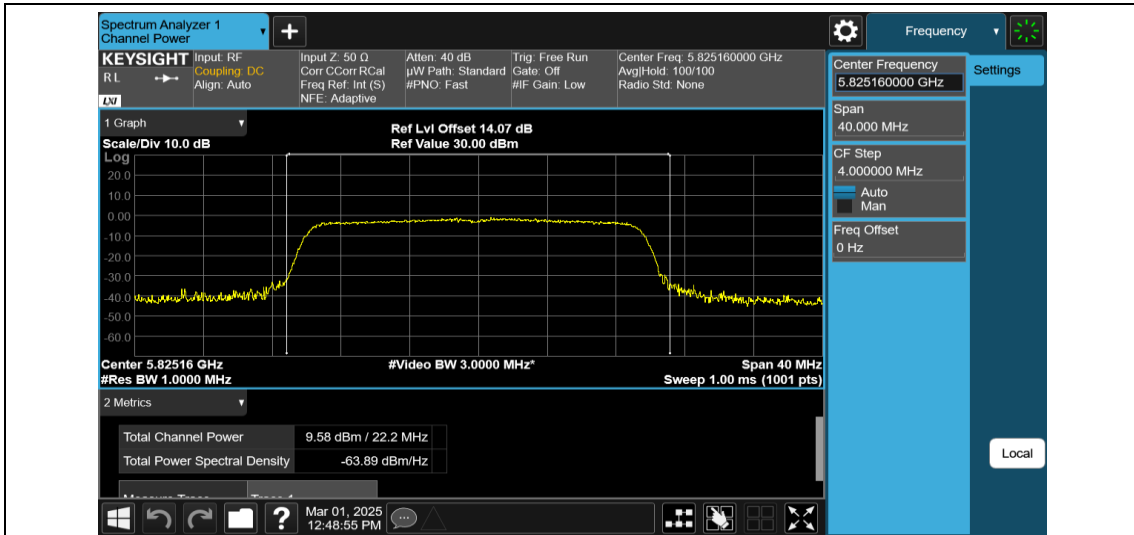
11AX20MIMO-Ant2-5825-PASS
