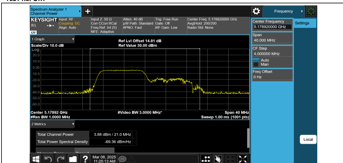
11AX20MIMO-Ant1-5180-106Tone-RU53-PASS
