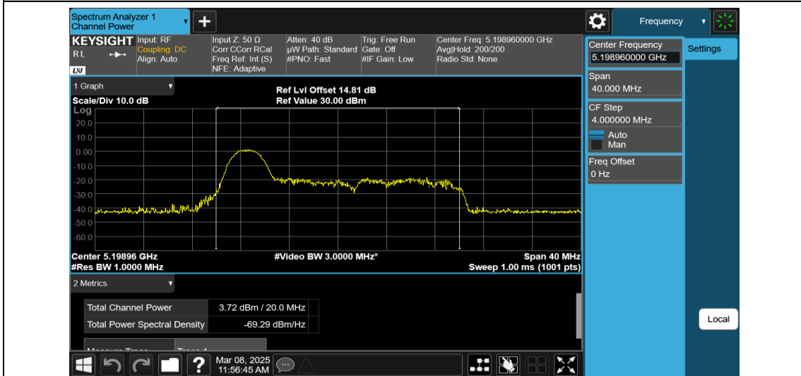
11AX20MIMO-Ant1-5200-26Tone-RU0-PASS
