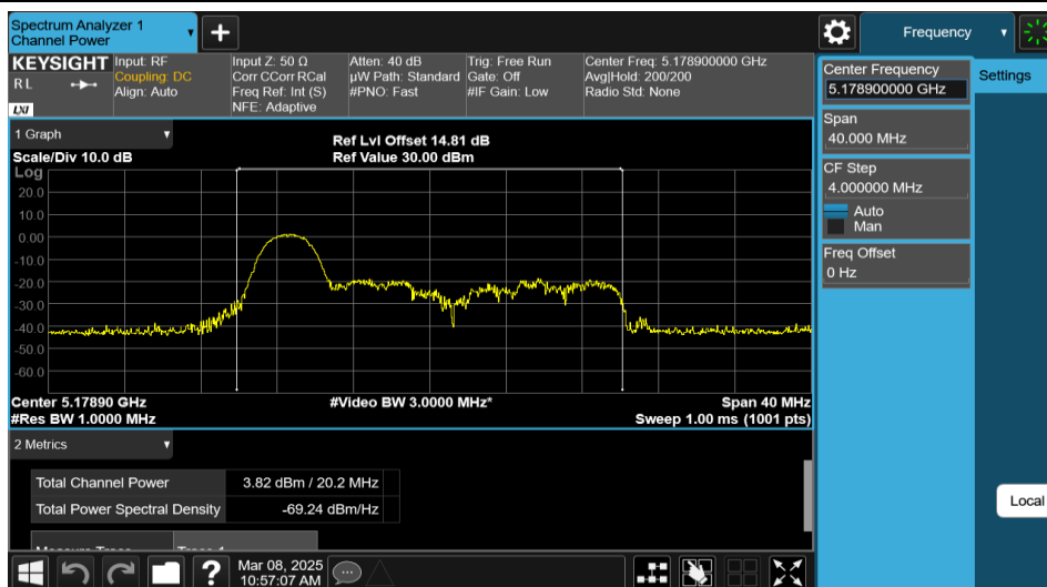
11AX20MIMO-Ant1-5180-26Tone-RU0-PASS
