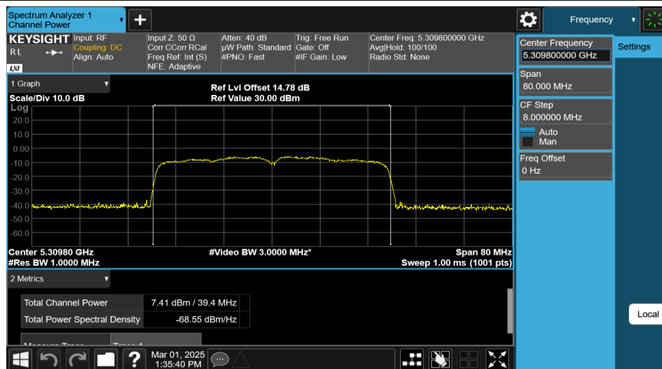
11AX40MIMO-Ant1-5310-PASS
