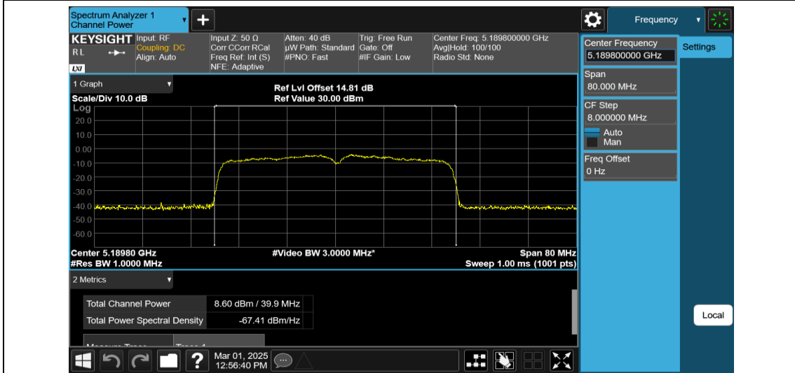
11AX40MIMO-Ant1-5190-PASS
