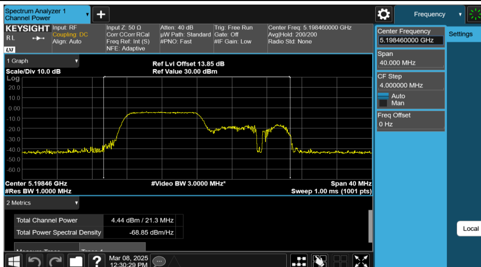
11AX20MIMO-Ant2-5200-106Tone-RU53-PASS
