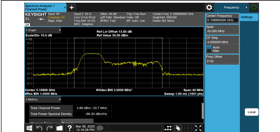
11AX20MIMO-Ant2-5200-52Tone-RU37-PASS
