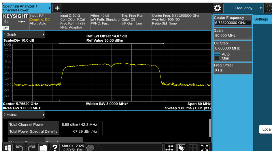
11AX40MIMO-Ant2-5755-PASS
