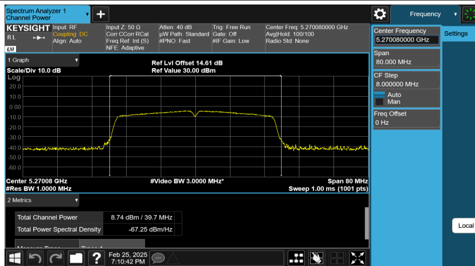
11AC40MIMO-Ant1-5270-PASS
