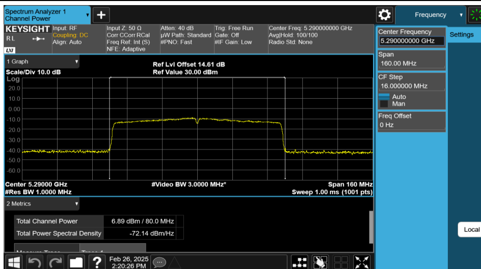
11AC80MIMO-Ant1-5290-PASS
