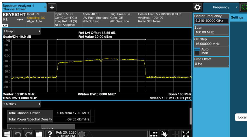
11AC80MIMO-Ant2-5210-PASS
