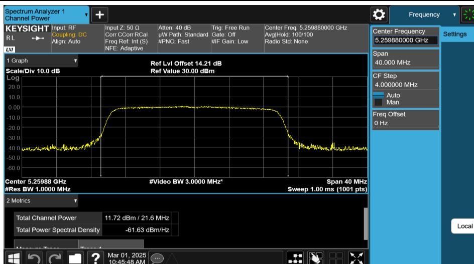
11AX20MIMO-Ant2-5260-PASS
