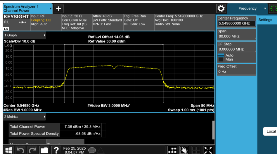
11AC40MIMO-Ant2-5550-PASS
