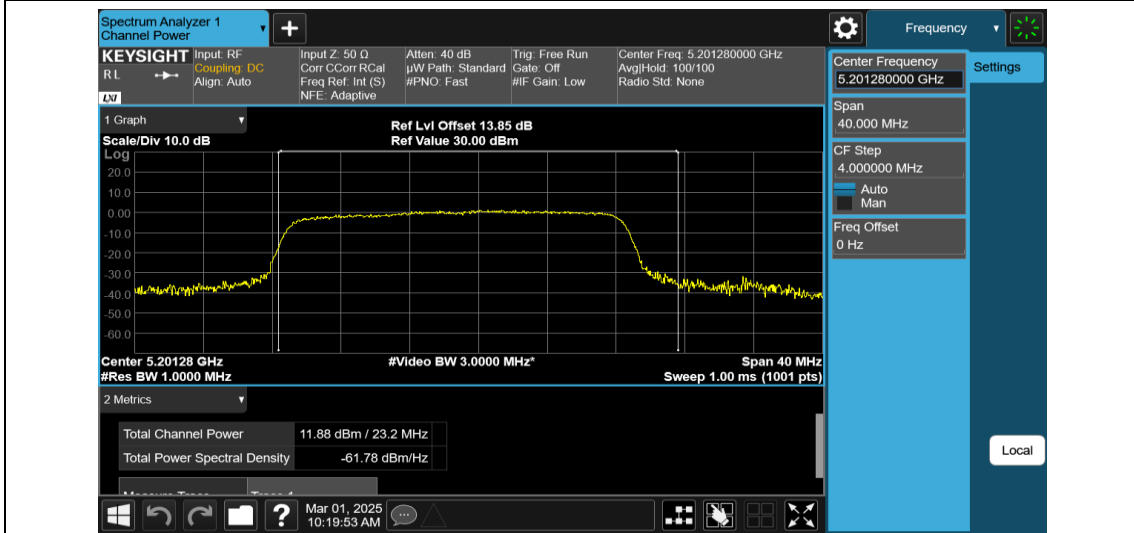
11AX20MIMO-Ant2-5200-PASS
