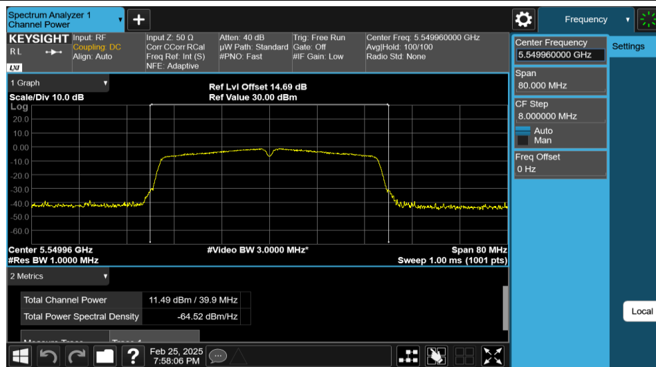
11AC40MIMO-Ant1-5550-PASS
