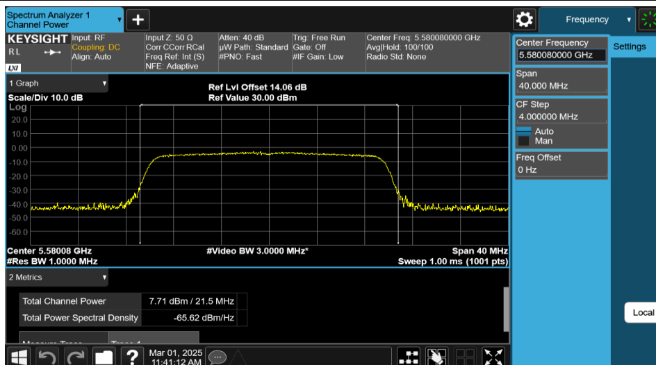
11AX20MIMO-Ant2-5580-PASS
