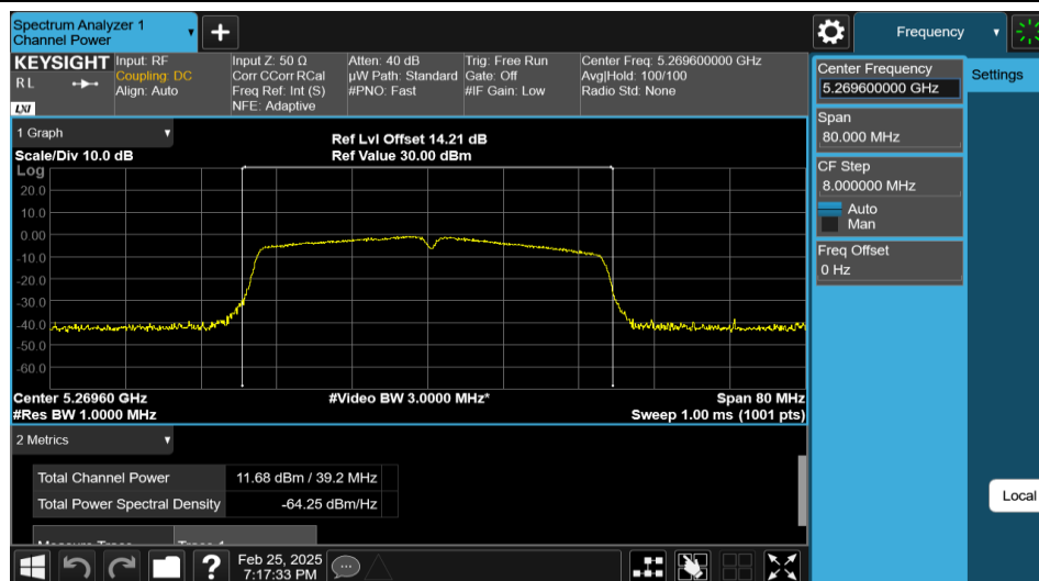
11AC40MIMO-Ant2-5270-PASS
