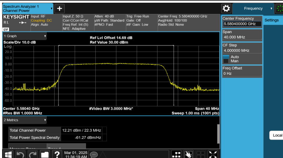
11AX20MIMO-Ant1-5580-PASS
