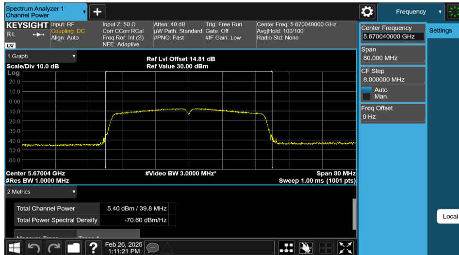
11AC40MIMO-Ant1-5670-PASS
