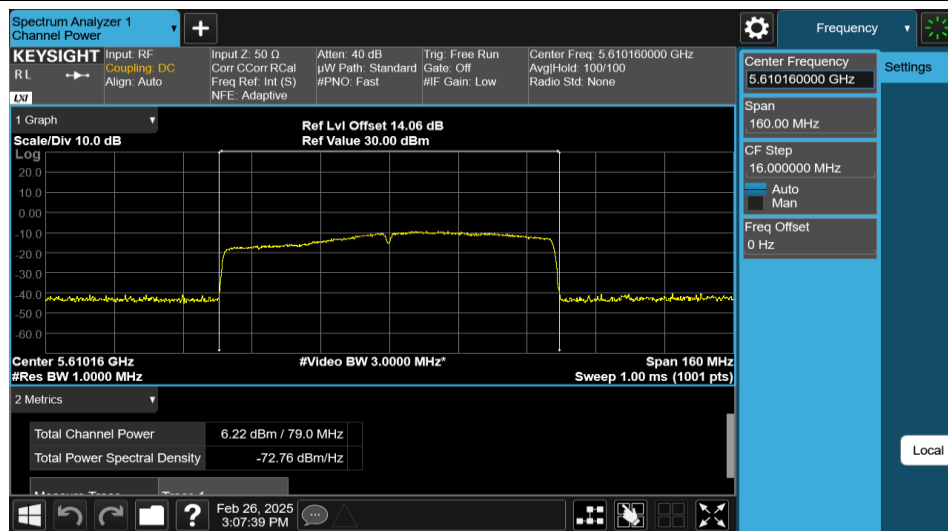
11AC80MIMO-Ant2-5610-PASS
