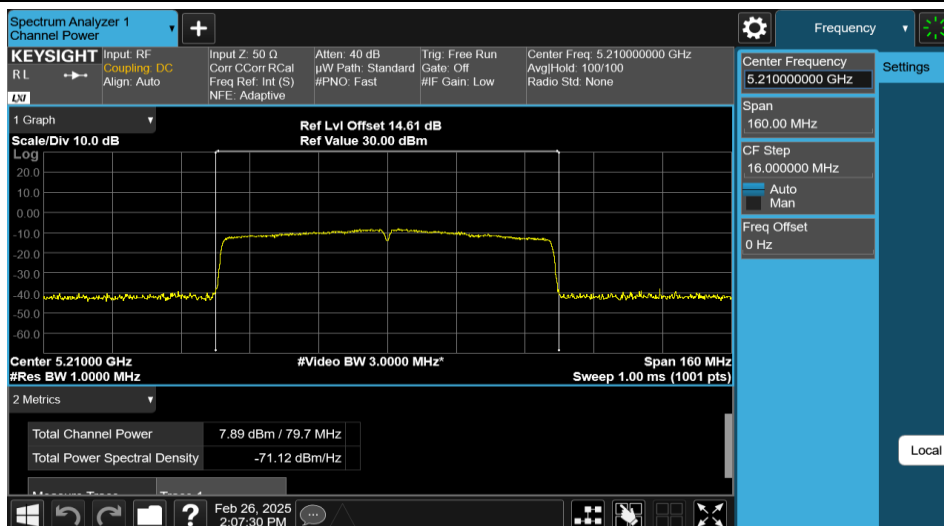
11AC80MIMO-Ant1-5210-PASS
