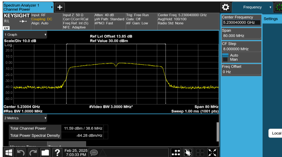
11AC40MIMO-Ant2-5230-PASS
