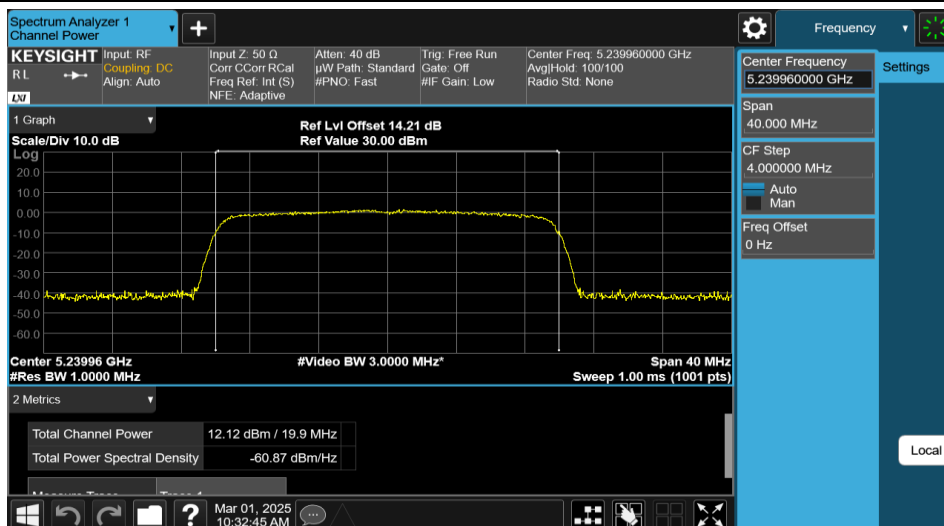
11AX20MIMO-Ant2-5240-PASS
