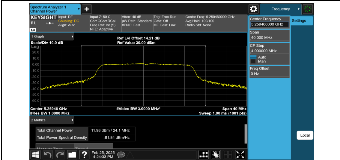
11AC20MIMO-Ant2-5260-PASS
