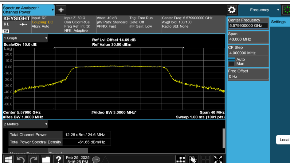
11AC20MIMO-Ant1-5580-PASS
