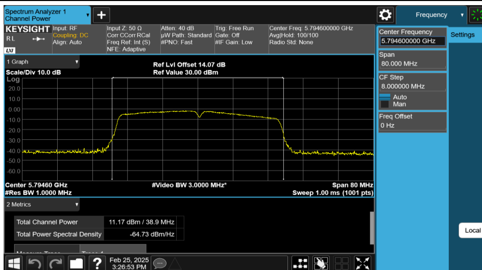
11N40MIMO-Ant2-5795-PASS
