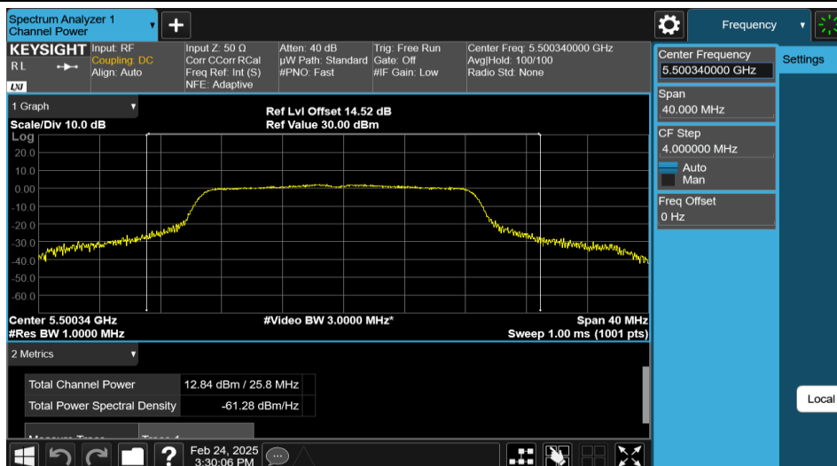
11N20MIMO-Ant1-5500-PASS
