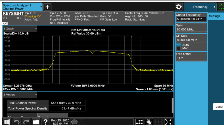
11N40MIMO-Ant2-5270-PASS
