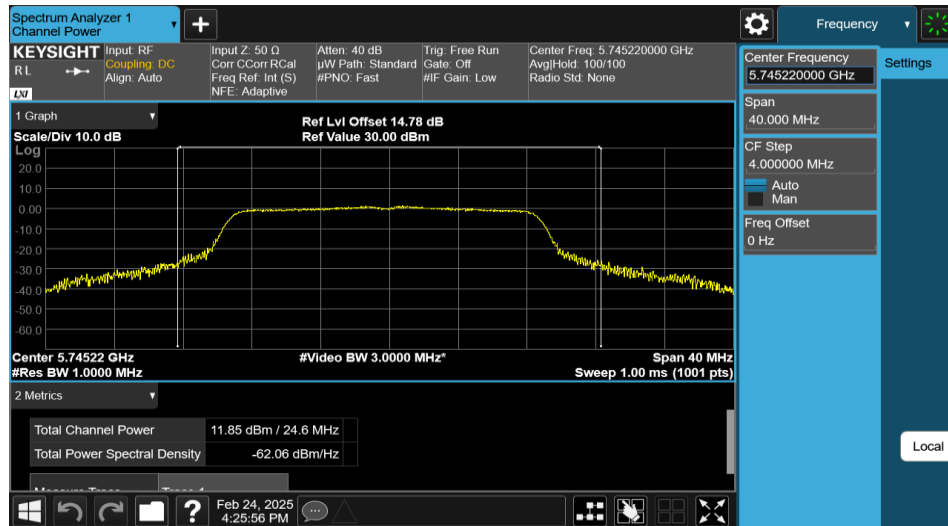
11N20MIMO-Ant1-5745-PASS
