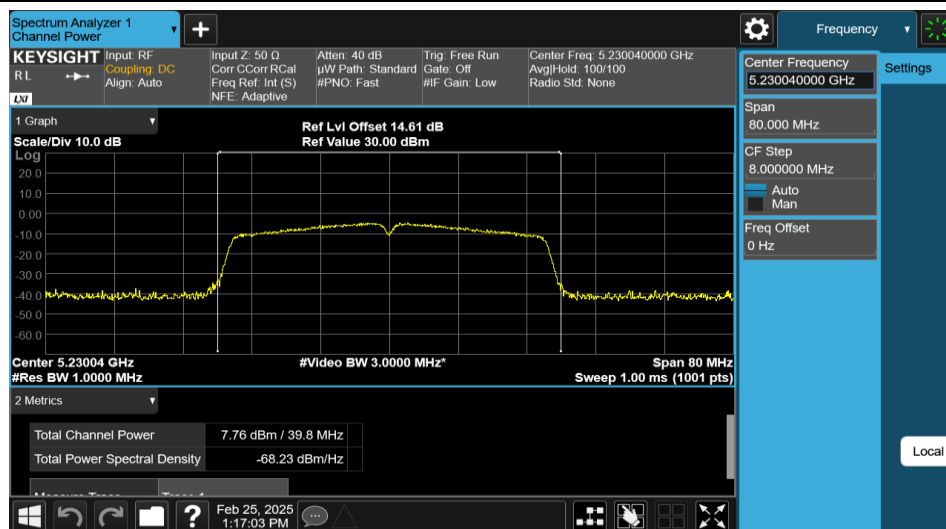
11N40MIMO-Ant1-5230-PASS
