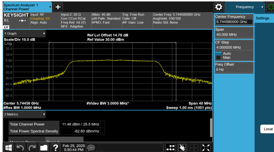
11AC20MIMO-Ant1-5745-PASS
