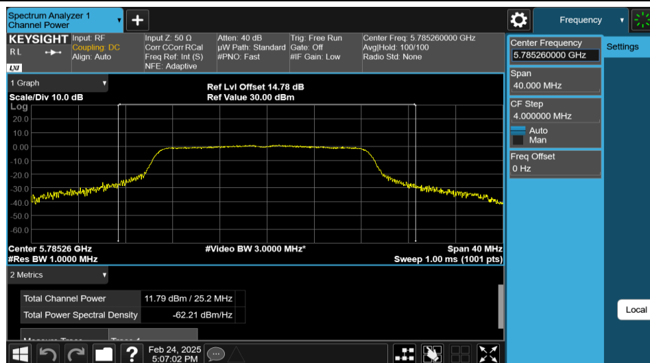
11N20MIMO-Ant1-5785-PASS
