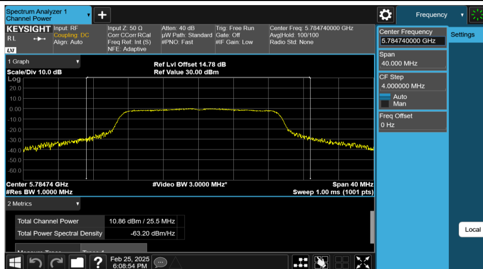
11AC20MIMO-Ant1-5785-PASS
