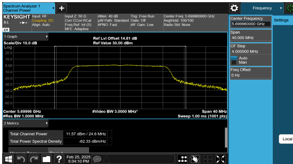
11AC20MIMO-Ant1-5700-PASS
