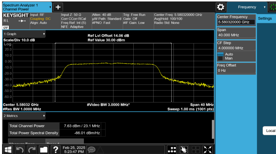
11AC20MIMO-Ant2-5580-PASS
