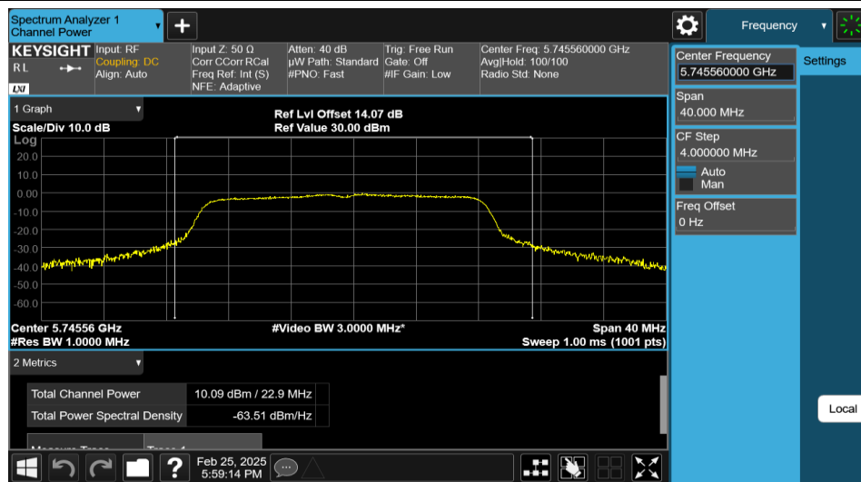
11AC20MIMO-Ant2-5745-PASS
