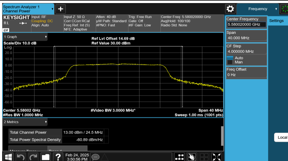
11N20MIMO-Ant1-5580-PASS
