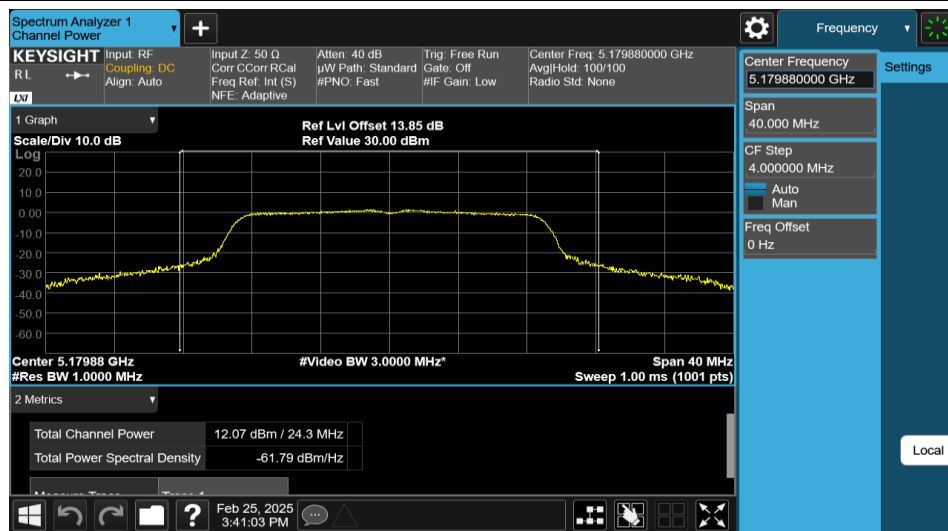
11AC20MIMO-Ant2-5180-PASS
