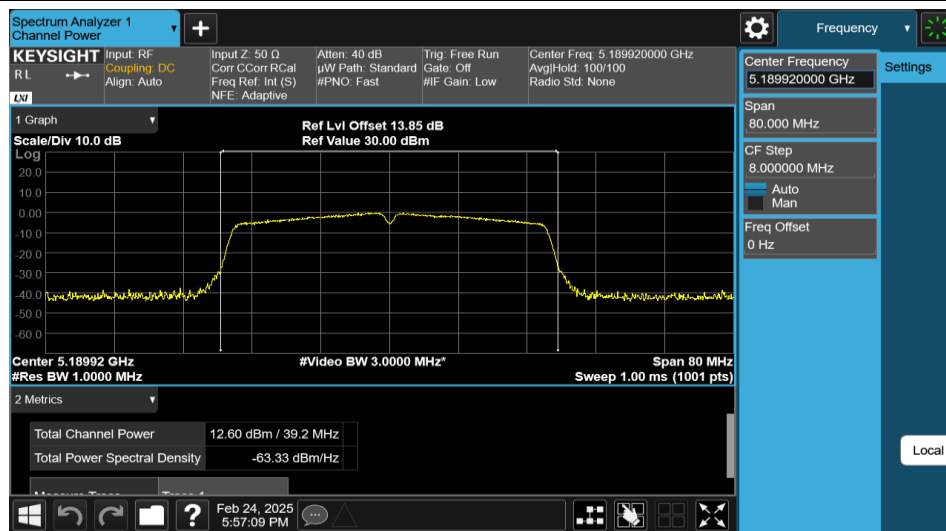
11N40MIMO-Ant2-5190-PASS
