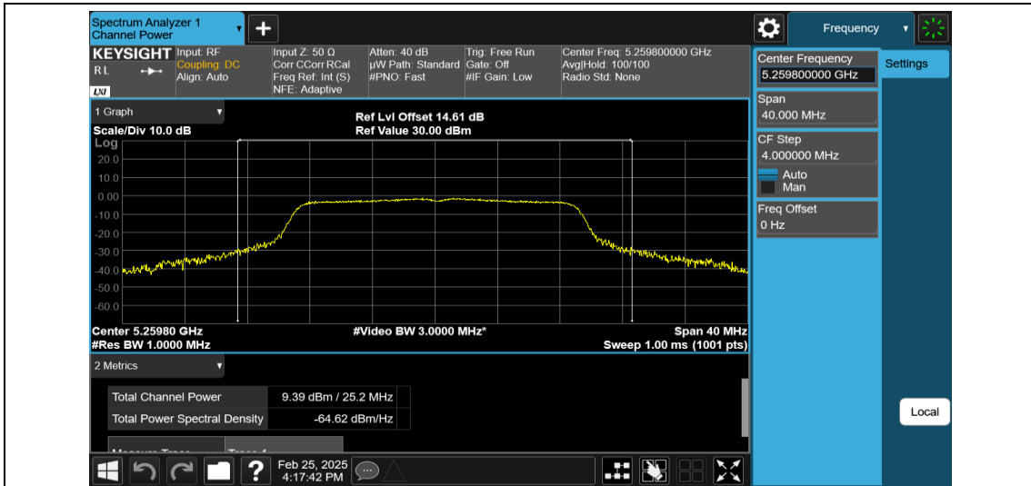
11AC20MIMO-Ant1-5260-PASS
