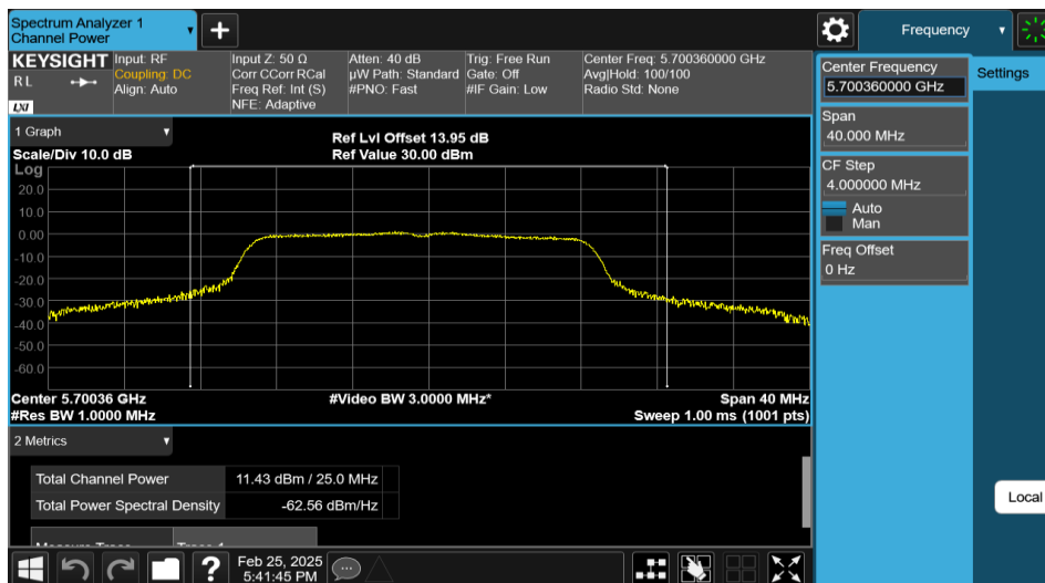
11AC20MIMO-Ant2-5700-PASS
