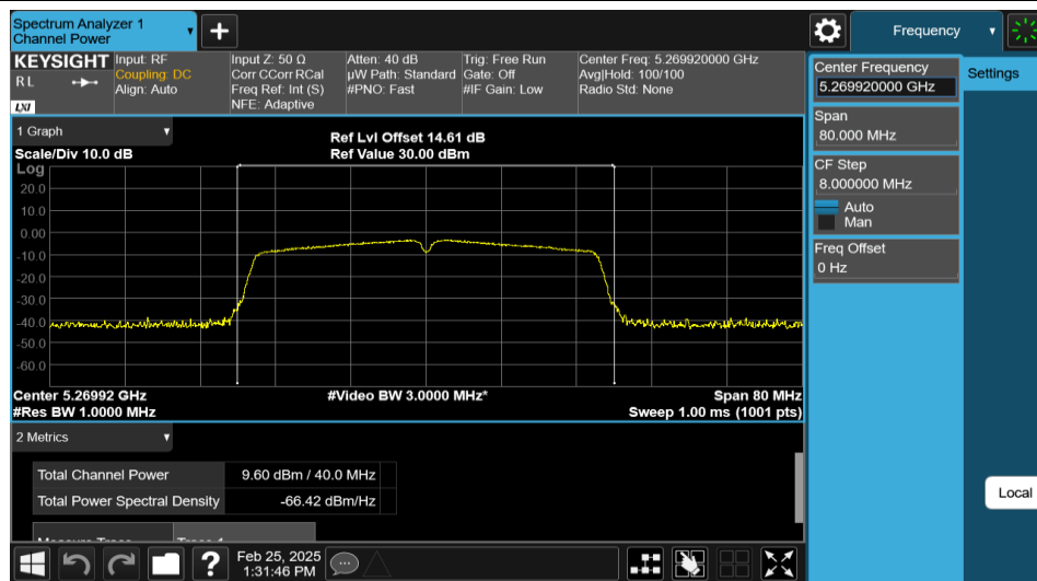
11N40MIMO-Ant1-5270-PASS
