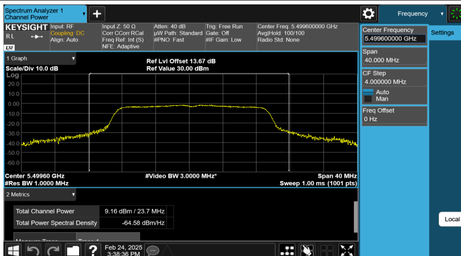
11N20MIMO-Ant2-5500-PASS
