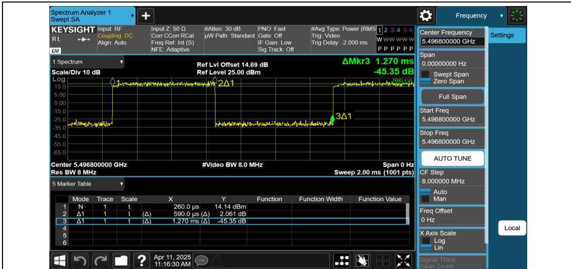
NTNV-11AX80MIMO-Ant1-5530-106Tone-RU53
