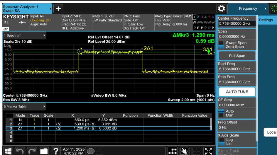
NTNV-11AX80MIMO-Ant2-5775-52Tone-RU37
