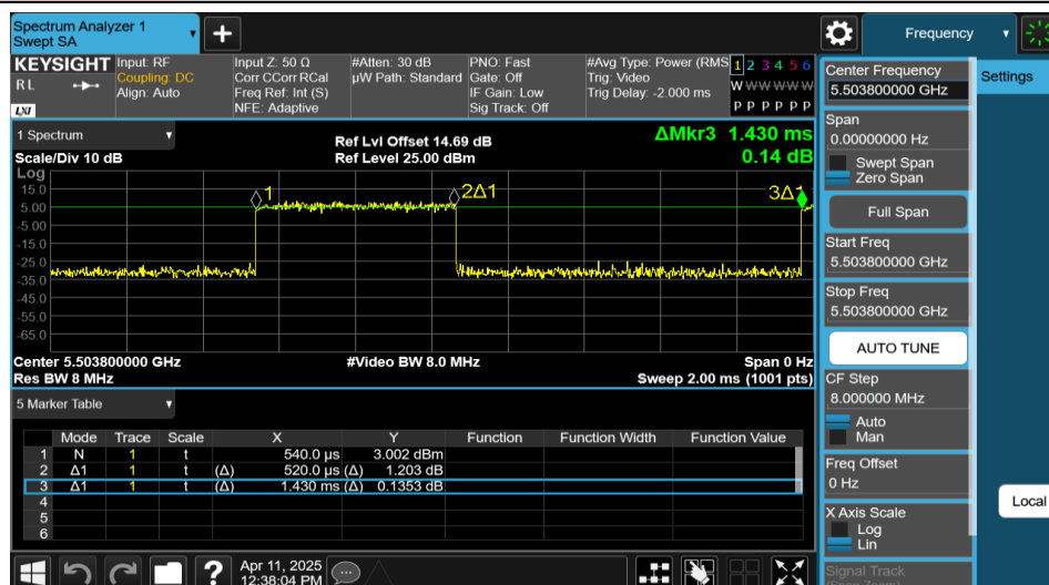
NTNV-11AX80MIMO-Ant1-5530-484Tone-RU65
