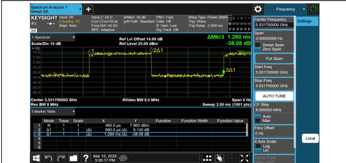
NTNV-11AX40MIMO-Ant1-5550-106Tone-RU53
