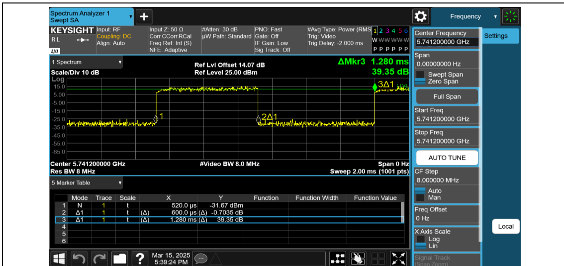
NTVN-11AX40MIMO-Ant2-5755-106Tone-RU53
