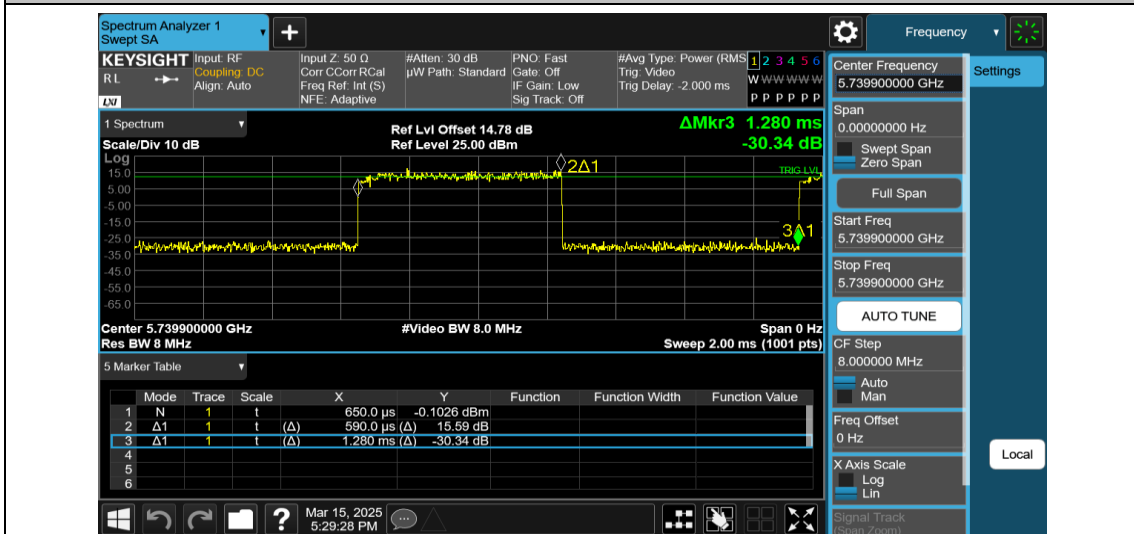
NTNV-11AX40MIMO-Ant1-5755-106Tone-RU53
