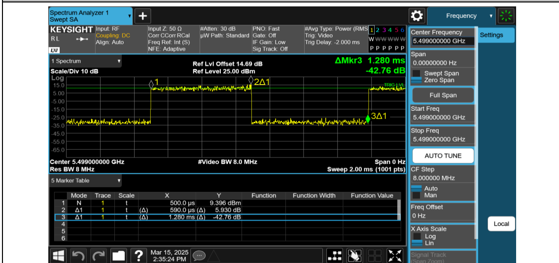
NTNV-11AX40MIMO-Ant1-5510-106Tone-RU53
