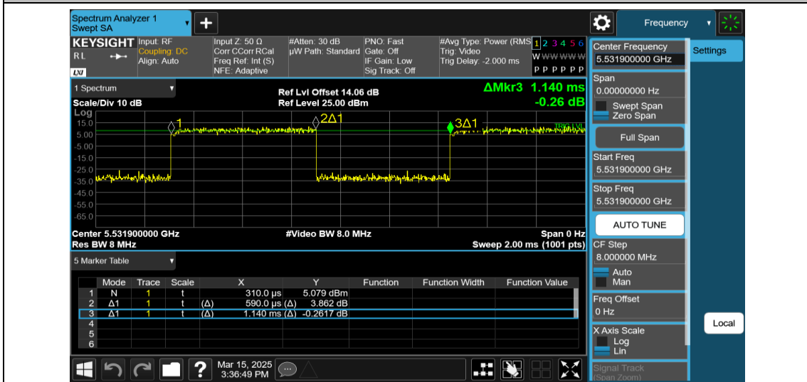
NTNV-11AX40MIMO-Ant2-5550-106Tone-RU53
