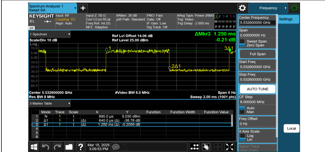
NTNV-11AX40MIMO-Ant2-5550-26Tone-RU0
