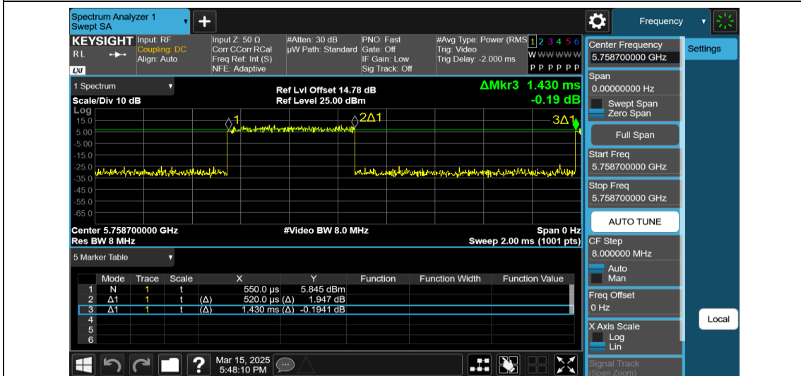
NTNV-11AX40MIMO-Ant1-5755-484Tone-RU65
