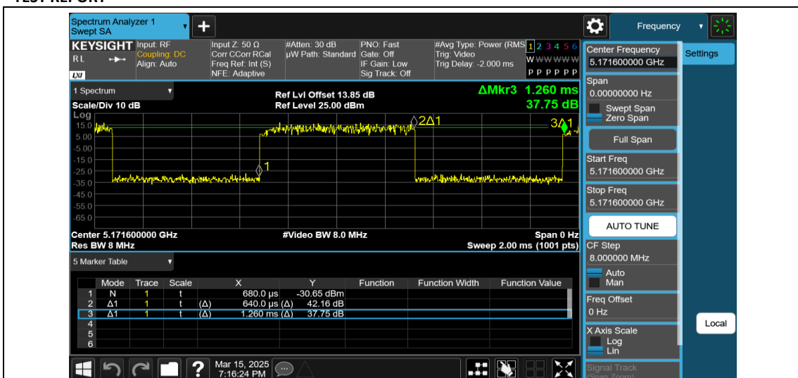
NTNV-11AX80MIMO-Ant2-5210-26Tone-RU0
