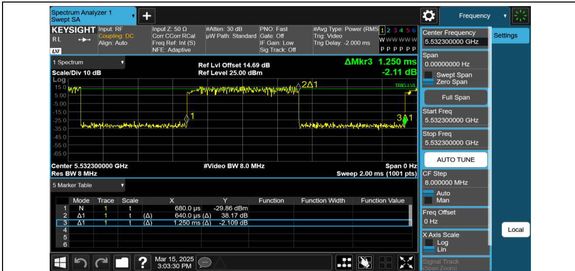
NTNV-11AX40MIMO-Ant1-5550-26Tone-RU0
