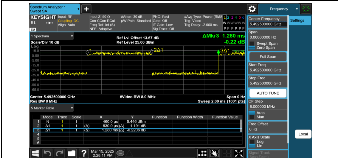
NTNV-11AX40MIMO-Ant2-5510-52Tone-RU37
