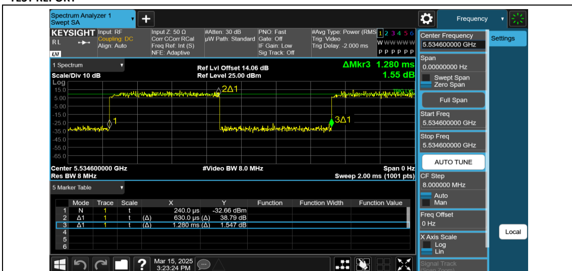
NTNV-11AX40MIMO-Ant2-5550-52Tone-RU37
