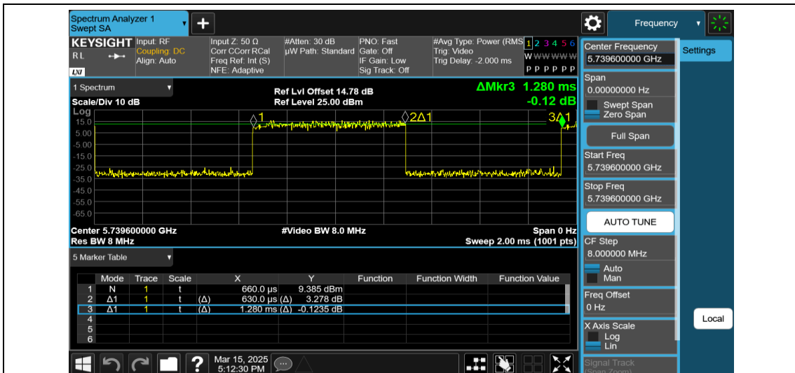
NTNV-11AX40MIMO-Ant1-5755-52Tone-RU37
