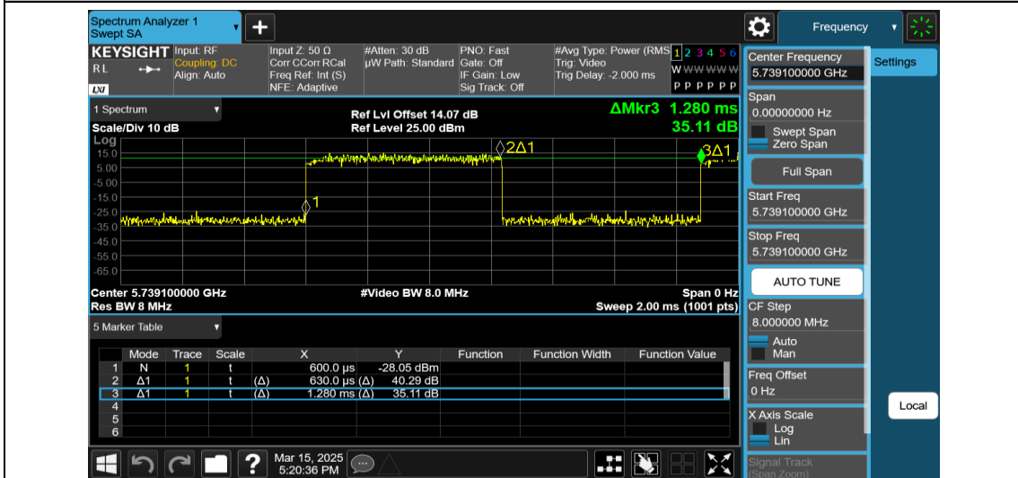
NTNV-11AX40MIMO-Ant2-5755-52Tone-RU37
