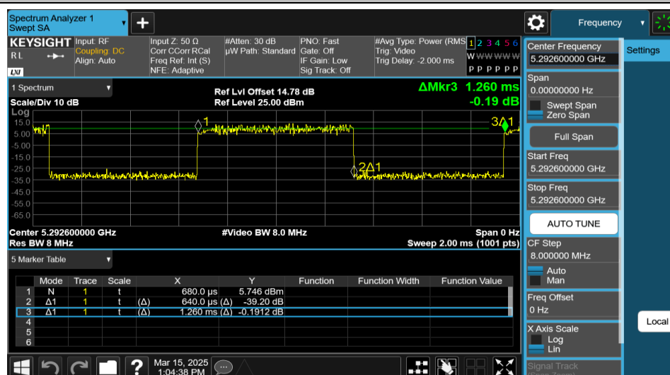
NTNV-11AX40MIMO-Ant1-5310-26Tone-RU0
