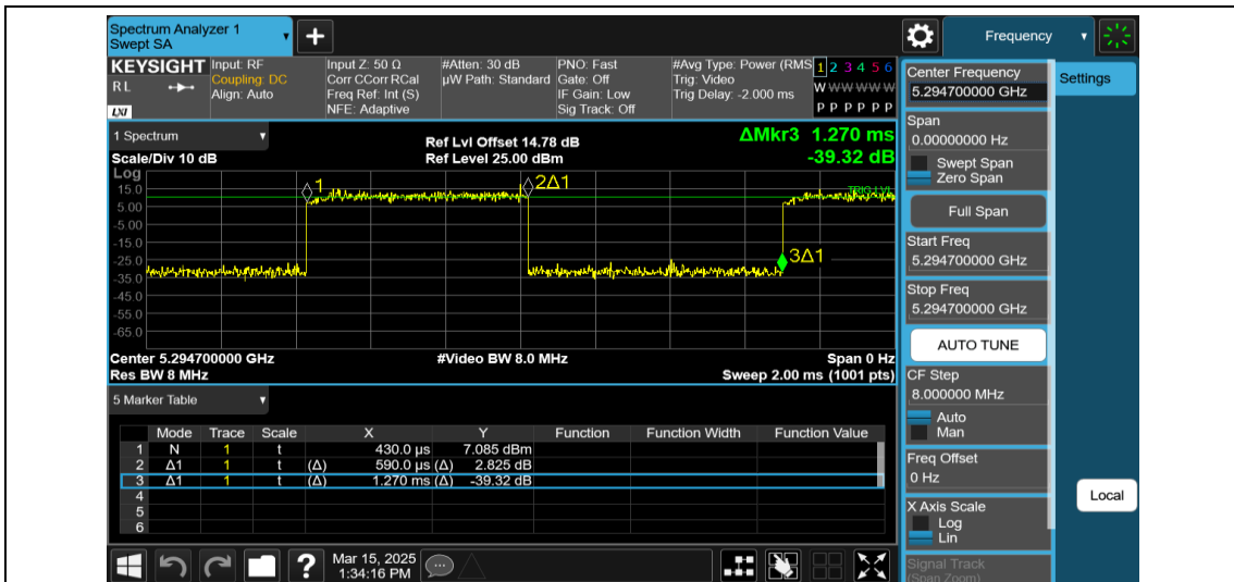
NTNV-11AX40MIMO-Ant1-5310-106Tone-RU53
