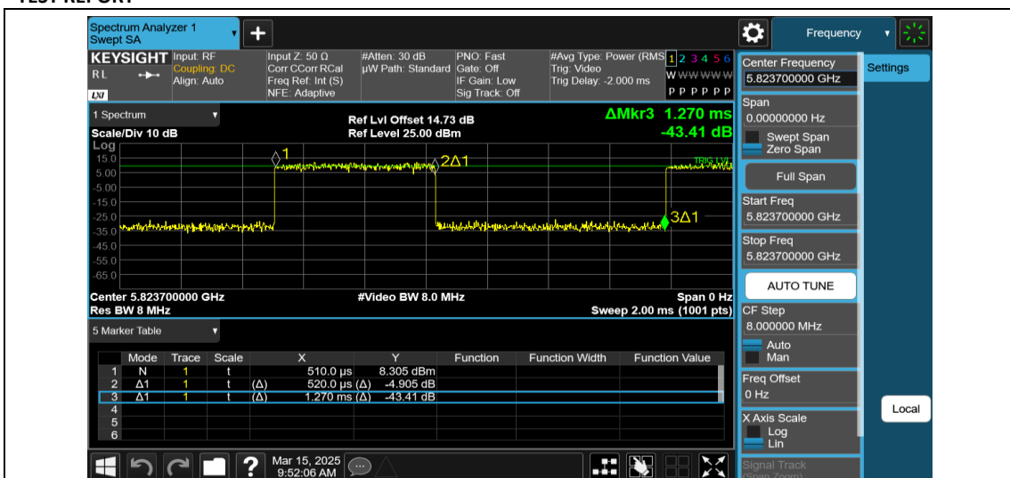
NTNV-11AX20MIMO-Ant1-5825-242Tone-RU61
