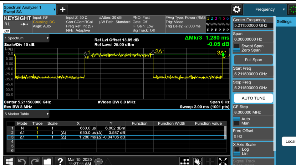
NTNV-11AX40MIMO-Ant2-5230-52Tone-RU37
