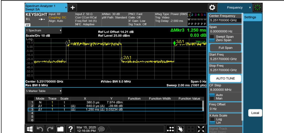
NTNV-11AX40MIMO-Ant2-5270-26Tone-RU0
