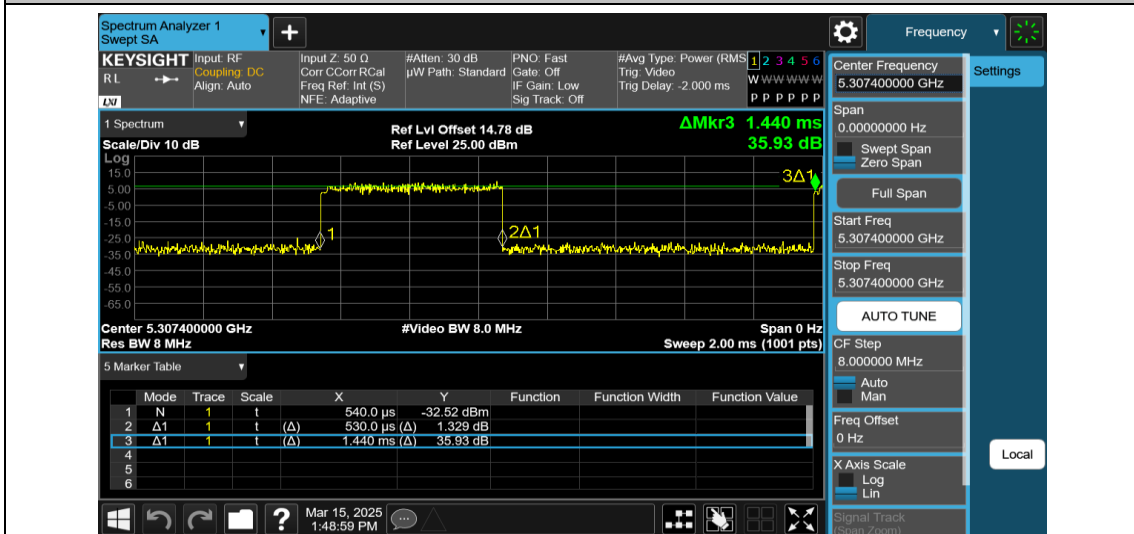
NTNV-11AX40MIMO-Ant1-5310-484Tone-RU65
