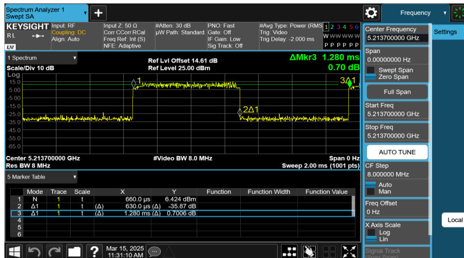
NTNV-11AX40MIMO-Ant1-5230-52Tone-RU37
