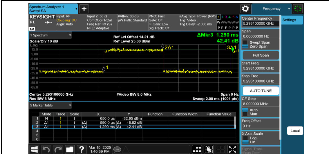
NTNV-11AX40MIMO-Ant2-5310-106Tone-RU53
