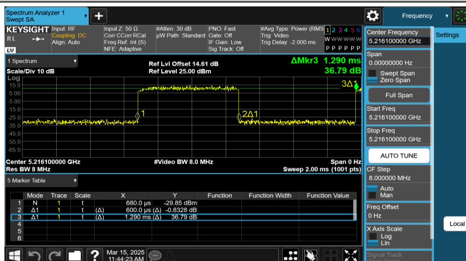
NTNV-11AX40MIMO-Ant1-5230-106Tone-RU53
