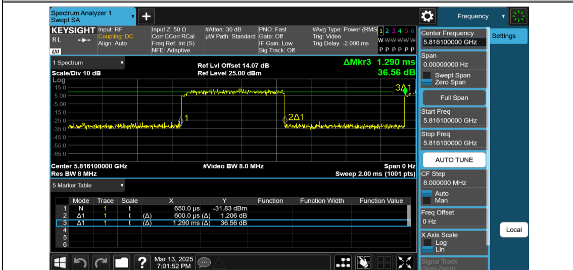
NTNV-11AX20MIMO-Ant2-5825-106Tone-RU53
