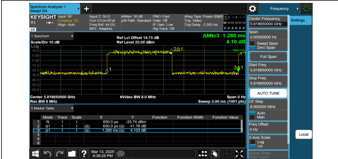
NTNV-11AX20MIMO-Ant1-5825-52Tone-RU37
