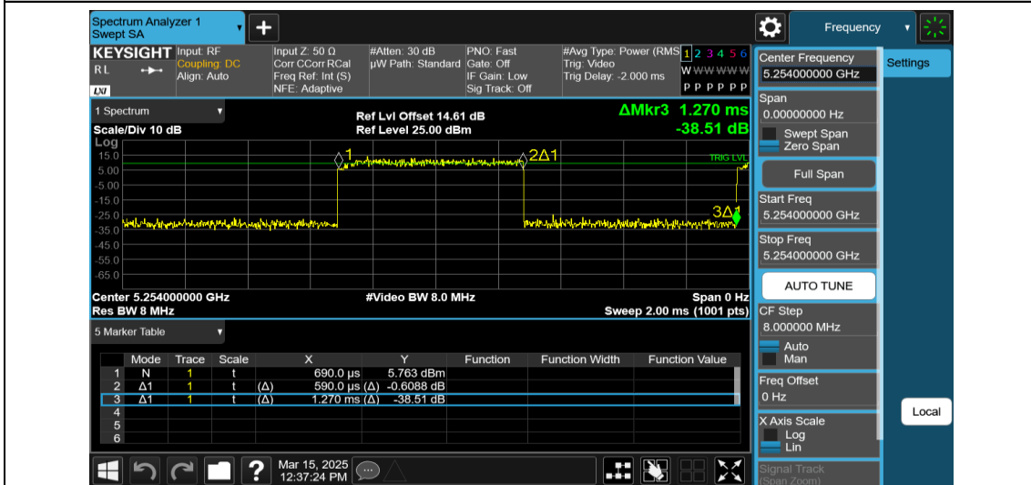
NTNV-11AX40MIMO-Ant1-5270-106Tone-RU53
