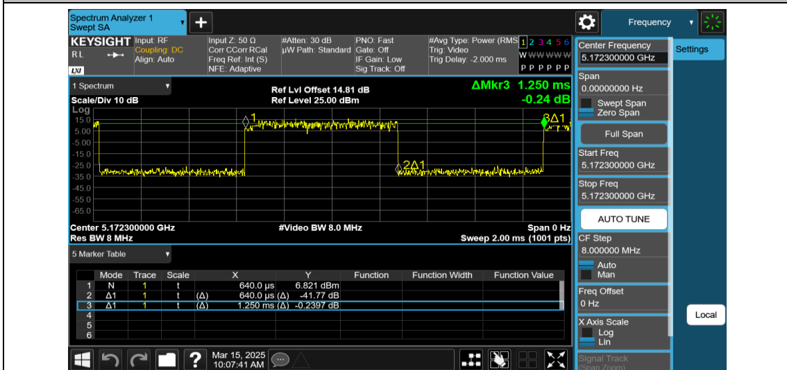
NTNV-11AX40MIMO-Ant1-5190-26Tone-RU0
