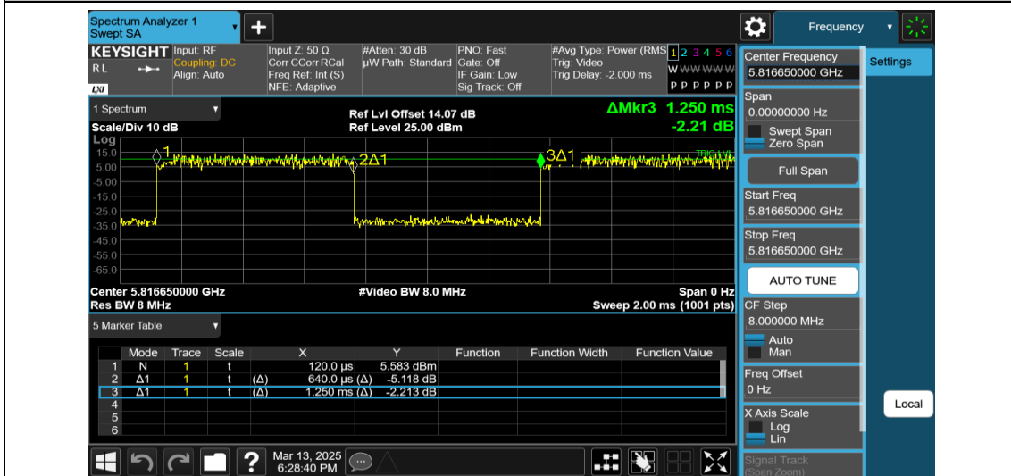
NTNV-11AX20MIMO-Ant2-5825-26Tone-RU0
