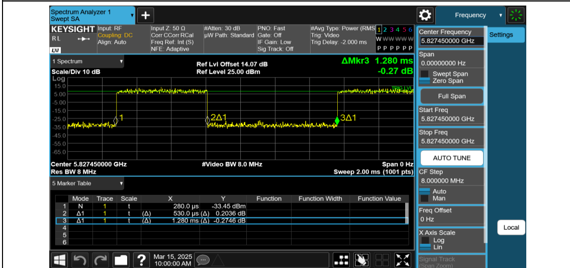
NTNV-11AX20MIMO-Ant2-5825-242Tone-RU61
