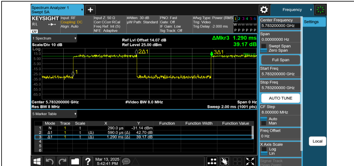
NTNV-11AX20MIMO-Ant2-5785-106Tone-RU53
