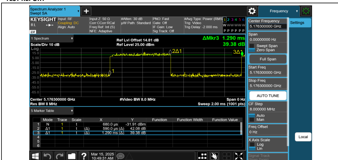
NTVN-11AX40MIMO-Ant1-5190-106Tone-RU53
