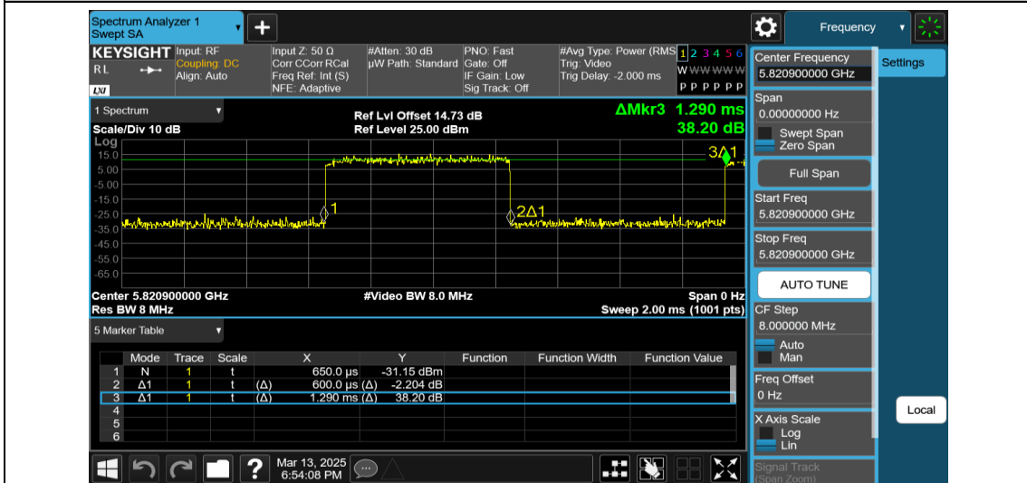
NTNV-11AX20MIMO-Ant1-5825-106Tone-RU53
