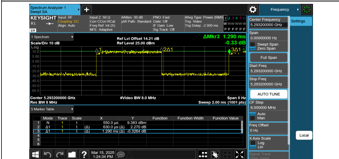
NTNV-11AX40MIMO-Ant2-5310-52Tone-RU37
