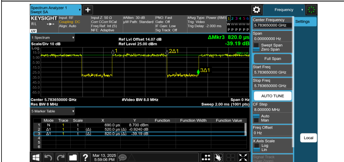
NTNV-11AX20MIMO-Ant2-5785-242Tone-RU61
