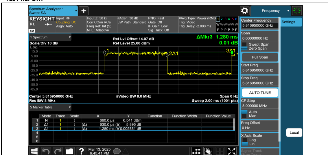
NTNV-11AX20MIMO-Ant2-5825-52Tone-RU37
