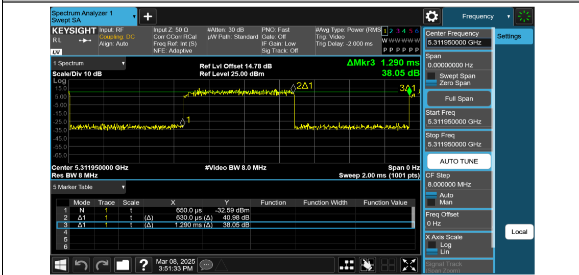
NTNV-11AX20MIMO-Ant1-5320-52Tone-RU37
