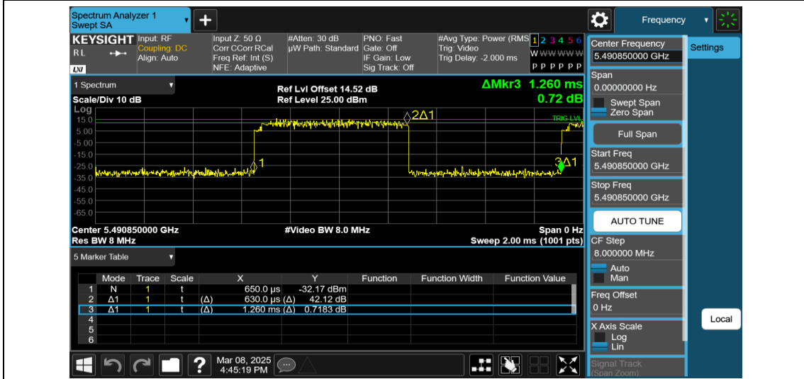
NTNV-11AX20MIMO-Ant1-5500-52Tone-RU37
