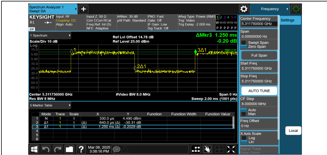
NTNV-11AX20MIMO-Ant1-5320-26Tone-RU0
