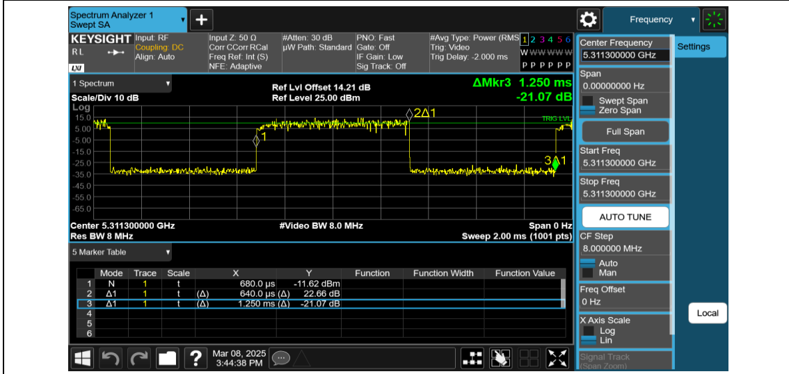
NTNV-11AX20MIMO-Ant2-5320-26Tone-RU0
