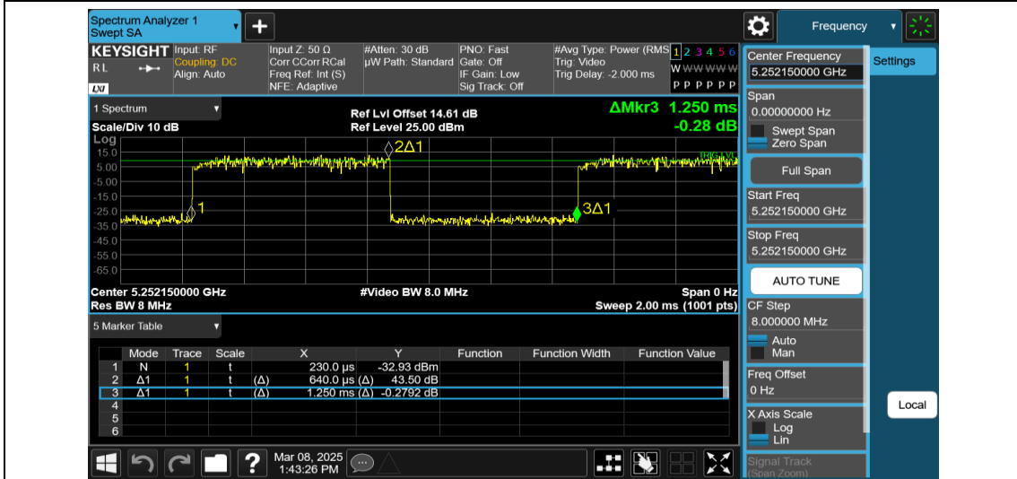
NTNV-11AX20MIMO-Ant1-5260-26Tone-RU0
