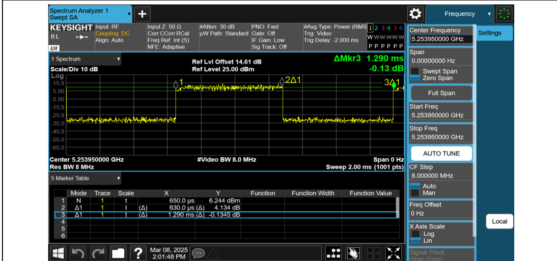
NTNV-11AX20MIMO-Ant1-5260-52Tone-RU37
