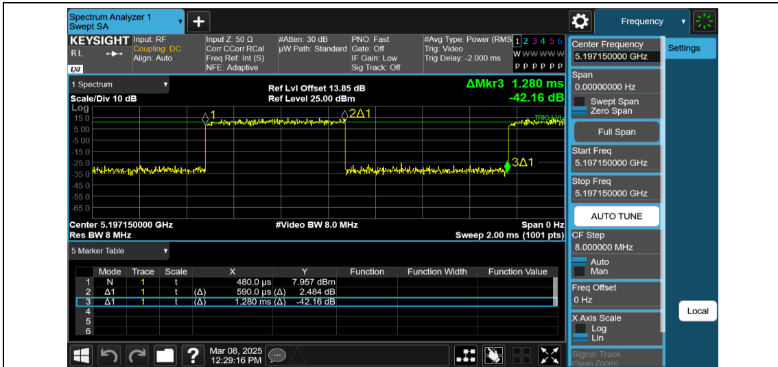
NTNV-11AX20MIMO-Ant2-5200-106Tone-RU53
