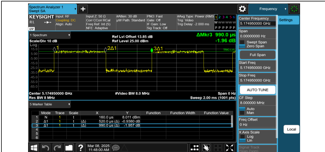
NTNV-11AX20MIMO-Ant2-5180-242Tone-RU61
