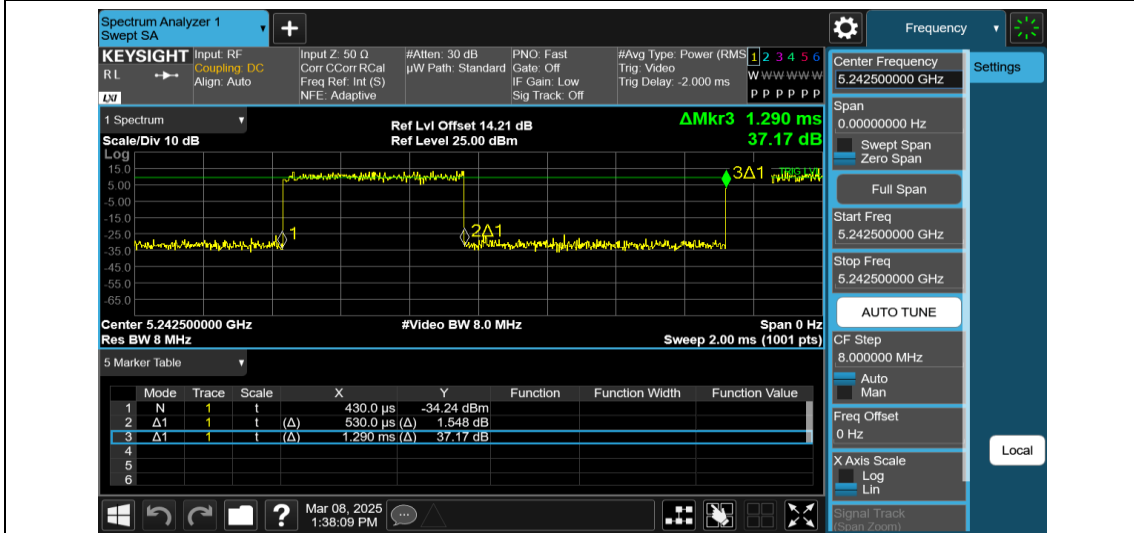
NTNV-11AX20MIMO-Ant2-5240-242Tone-RU61
