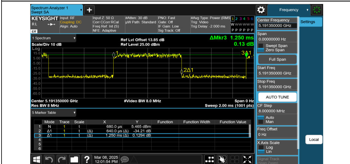
NTNV-11AX20MIMO-Ant2-5200-26Tone-RU0
