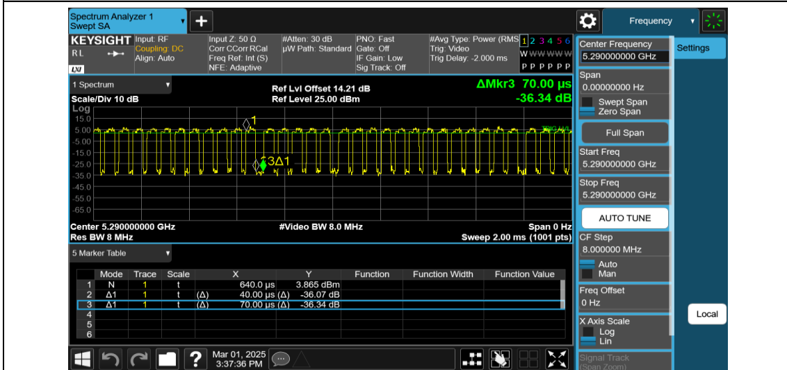
NTNV-11AX80MIMO-Ant2-5290
