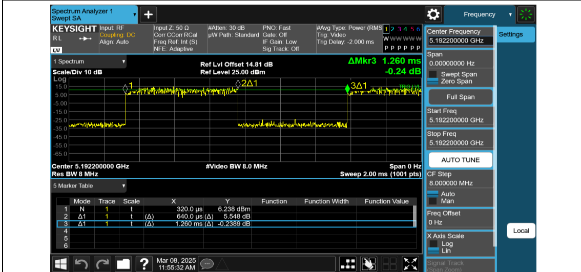
NTNV-11AX20MIMO-Ant1-5200-26Tone-RU0
