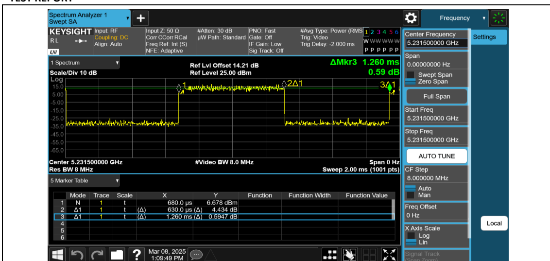
NTNV-11AX20MIMO-Ant2-5240-52Tone-RU37
