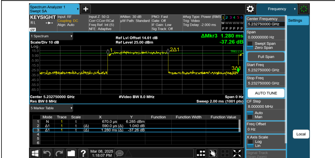
NTNV-11AX20MIMO-Ant1-5240-106Tone-RU53
