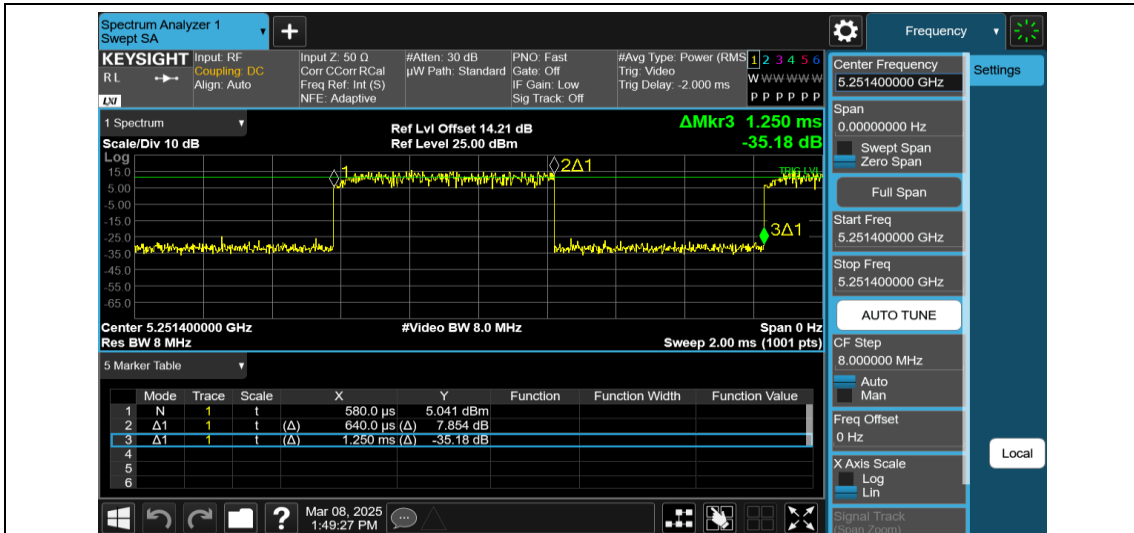
NTNV-11AX20MIMO-Ant2-5260-26Tone-RU0
