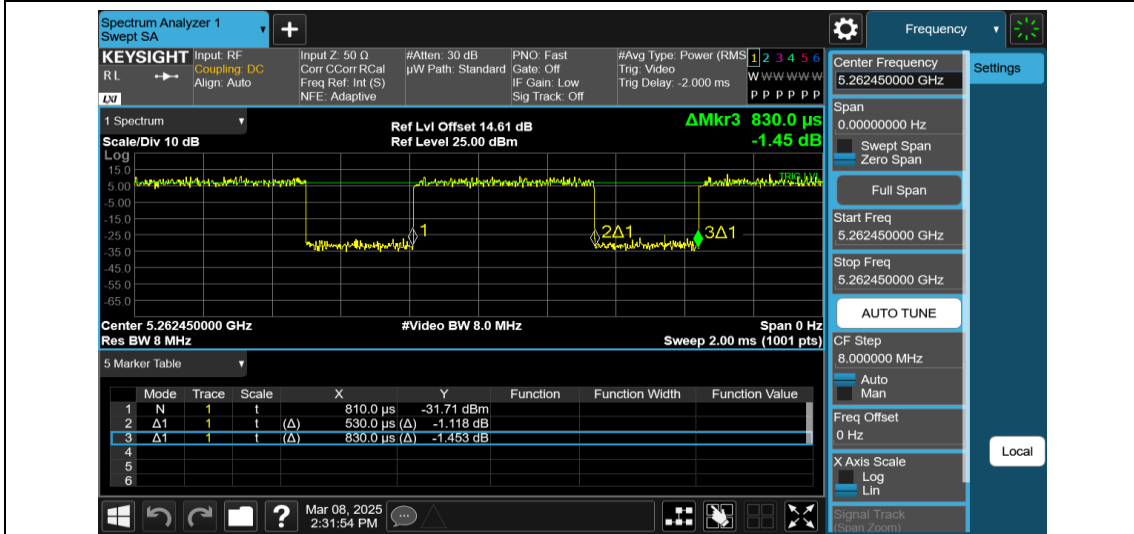
NTNV-11AX20MIMO-Ant1-5260-242Tone-RU61
