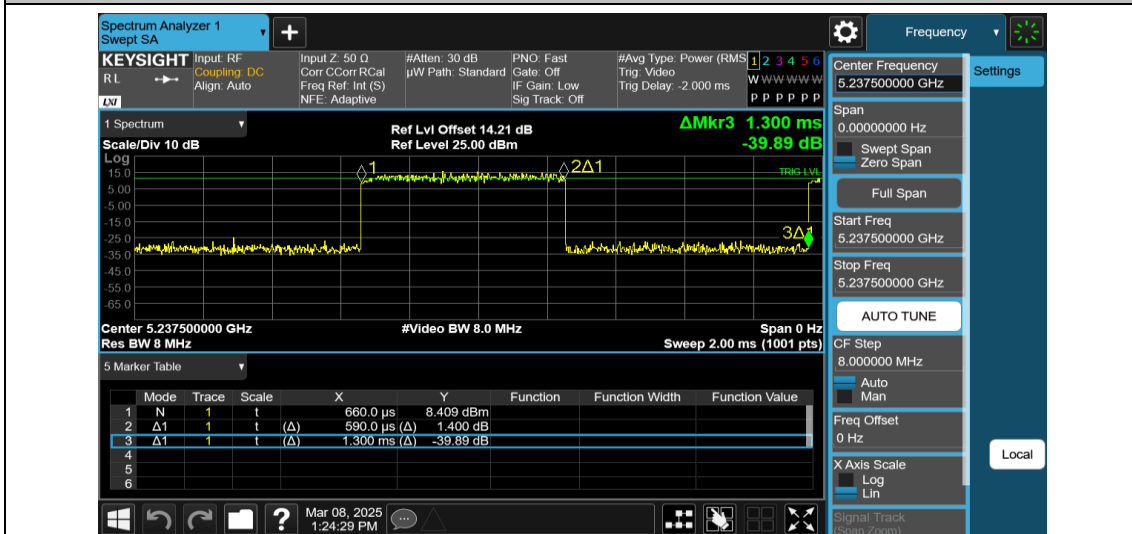
NTNV-11AX20MIMO-Ant2-5240-106Tone-RU53
