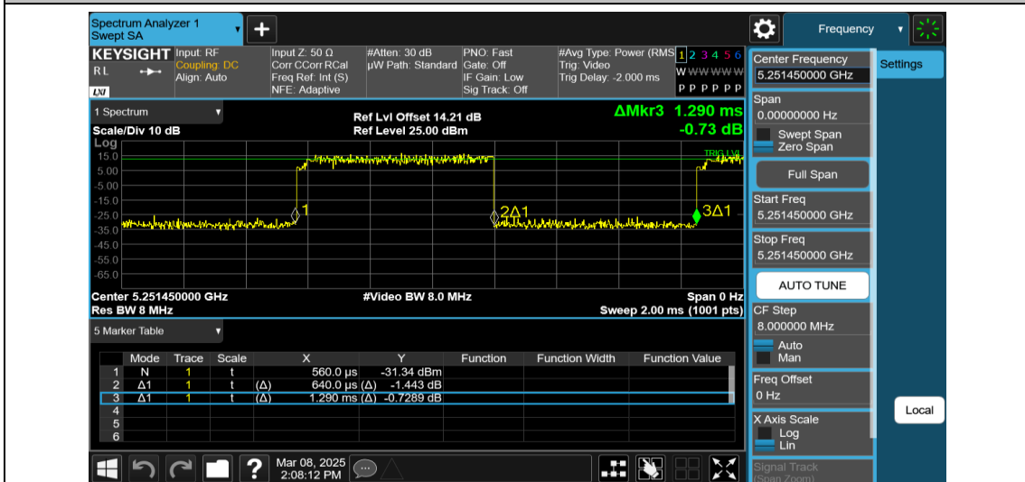
NTNV-11AX20MIMO-Ant2-5260-52Tone-RU37
