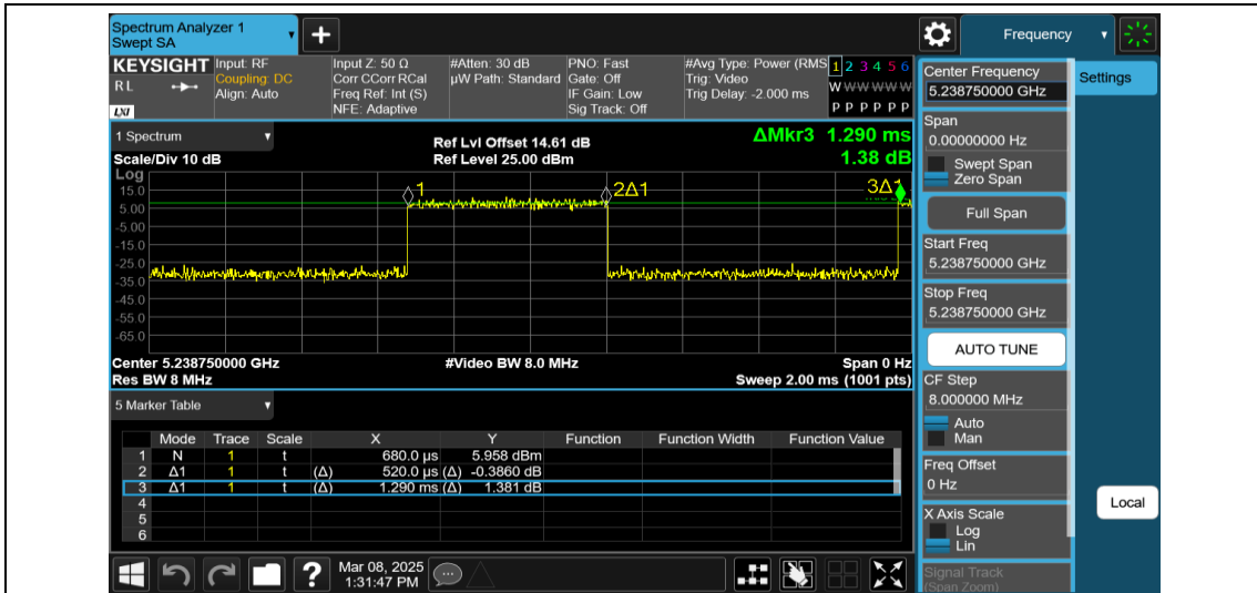
NTNV-11AX20MIMO-Ant1-5240-242Tone-RU61
