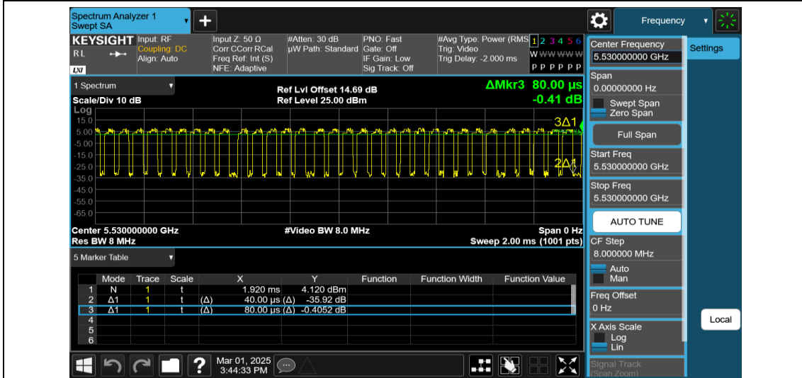
NTNV-11AX80MIMO-Ant1-5530
