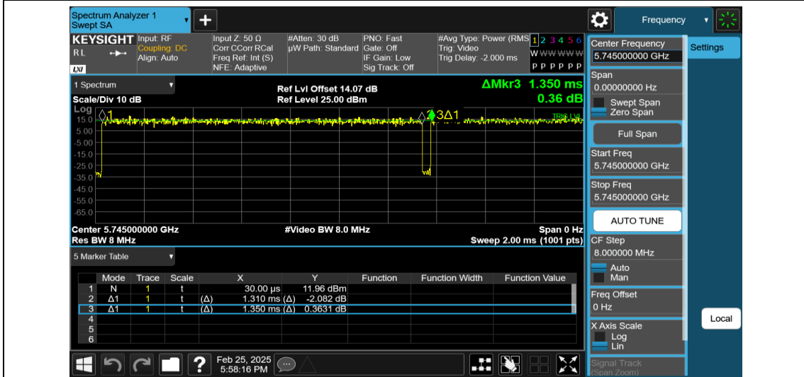
NTNV-11AC20MIMO-Ant2-5745
