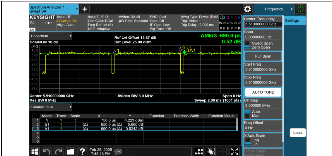
NTNV-11AC40MIMO-Ant2-5510
