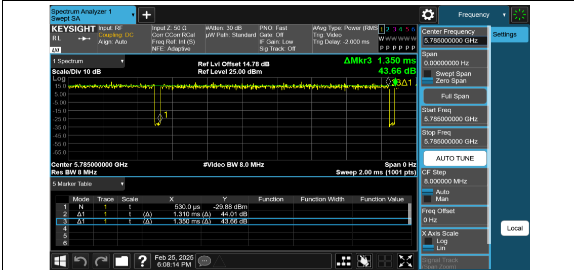
NTNV-11AC20MIMO-Ant1-5785
