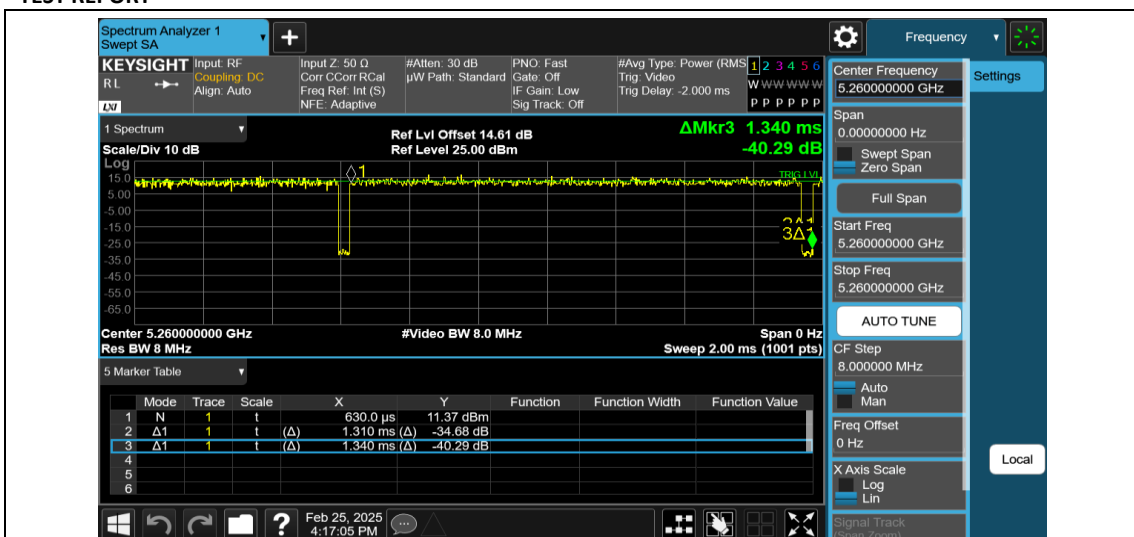
NTNV-11AC20MIMO-Ant1-5260
