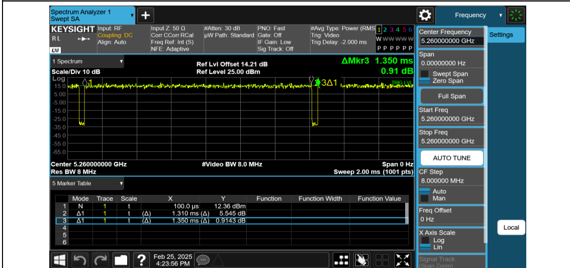
NTNV-11AC20MIMO-Ant2-5260
