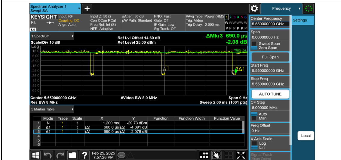
NTNV-11AC40MIMO-Ant1-5550
