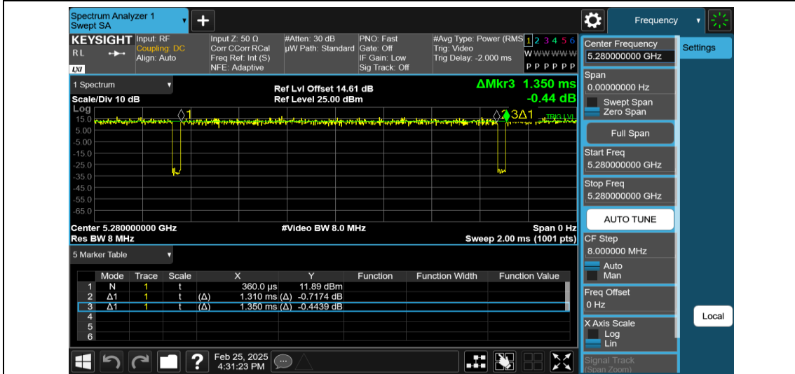
NTNV-11AC20MIMO-Ant1-5280
