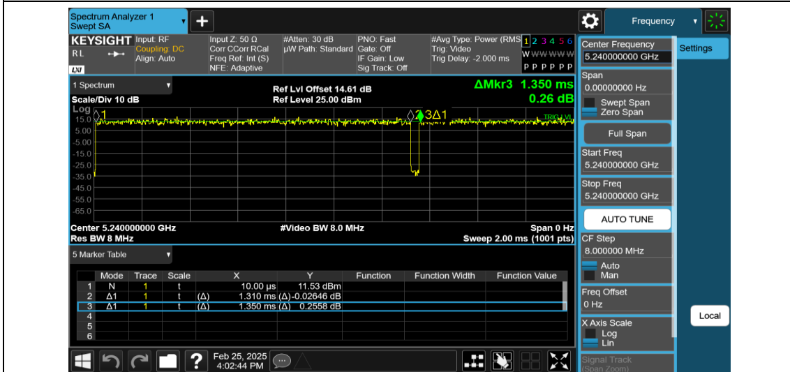
NTNV-11AC20MIMO-Ant1-5240
