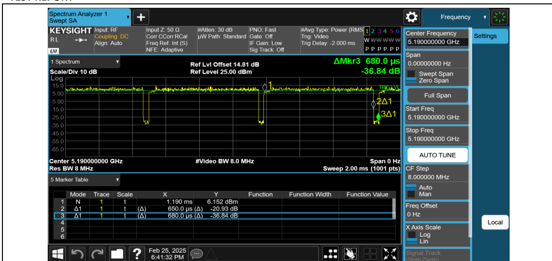
NTNV-11AC40MIMO-Ant1-5190
