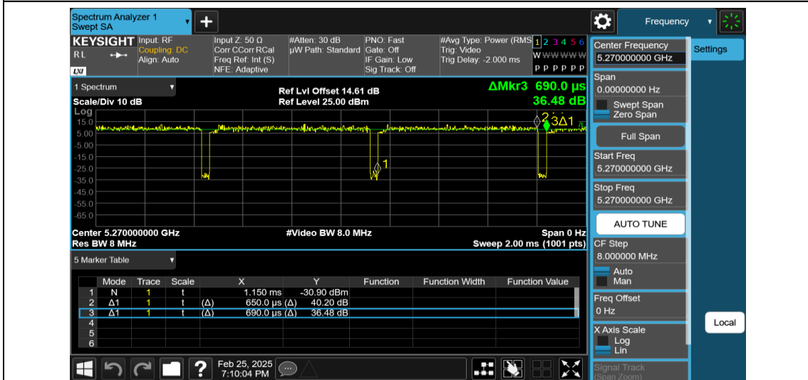
NTNV-11AC40MIMO-Ant1-5270
