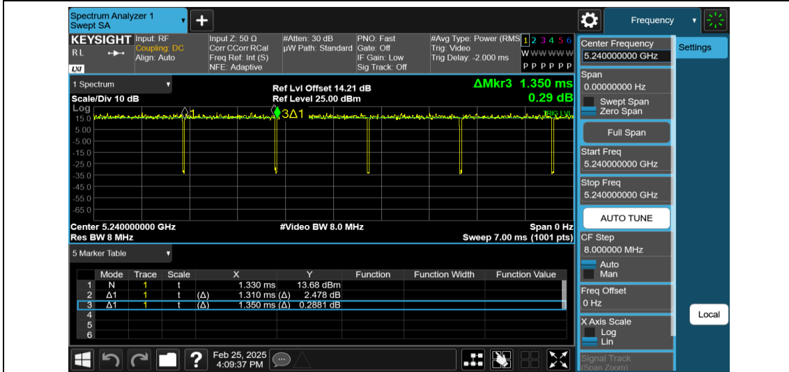
NTNV-11AC20MIMO-Ant2-5240
