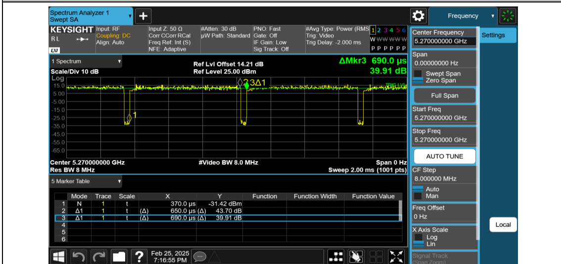
NTNV-11AC40MIMO-Ant2-5270
