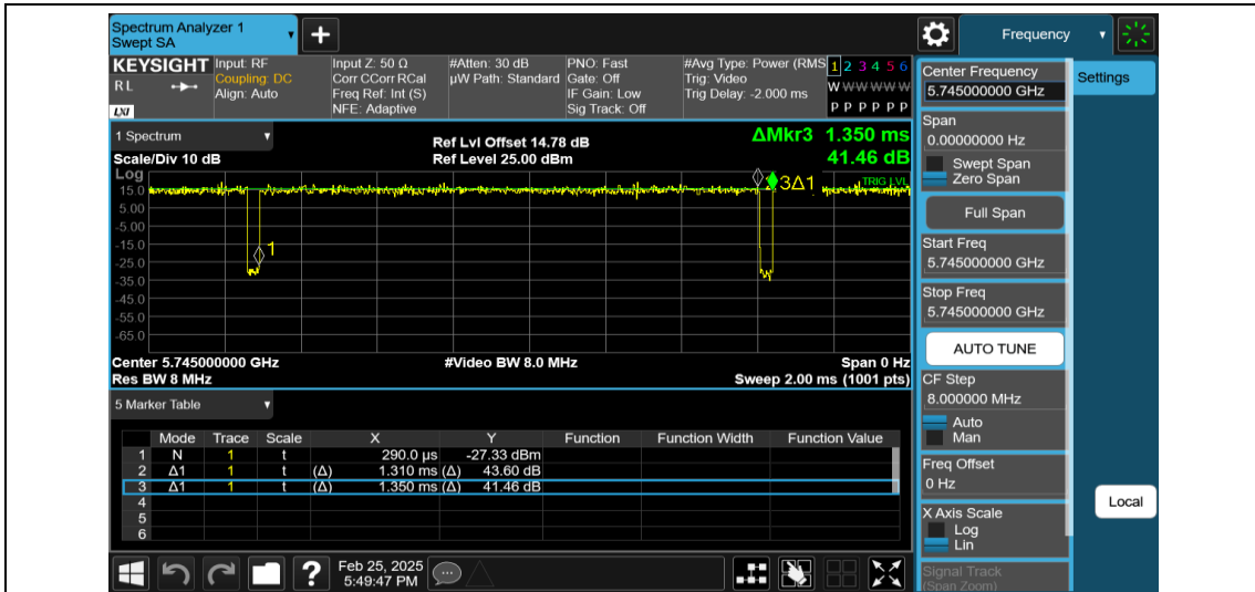
NTNV-11AC20MIMO-Ant1-5745
