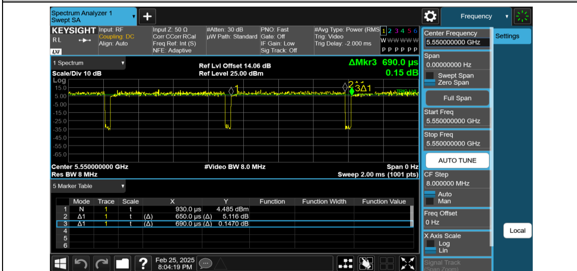
NTNV-11AC40MIMO-Ant2-5550
