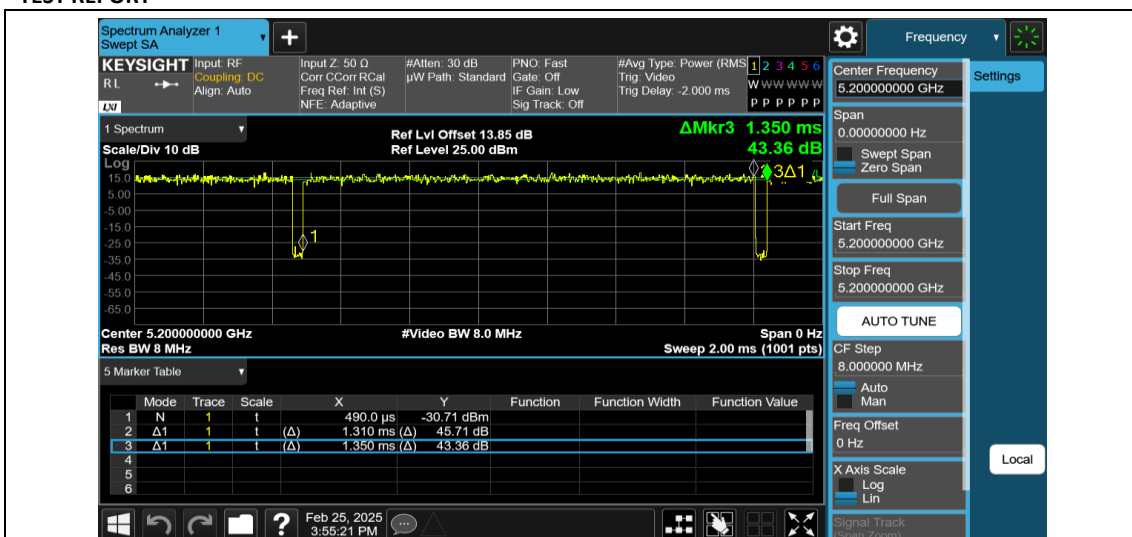
NTNV-11AC20MIMO-Ant2-5200
