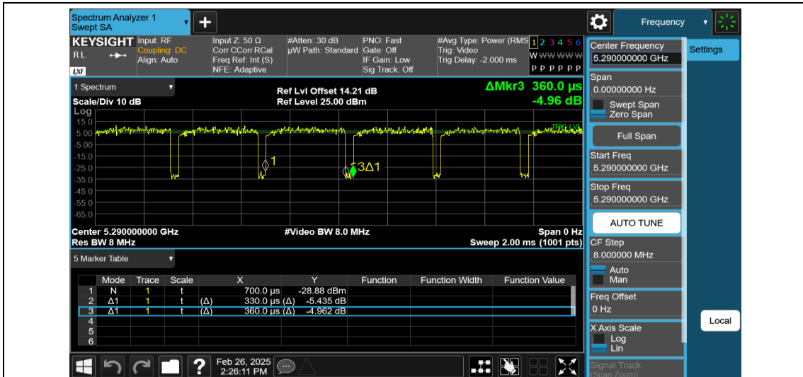
NTNV-11AC80MIMO-Ant2-5290
