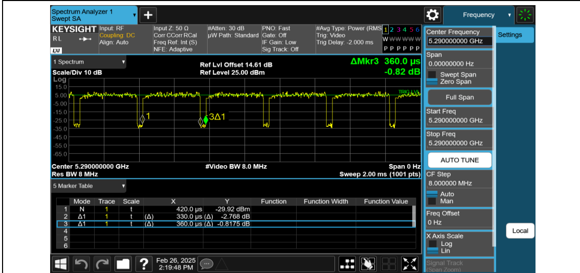
NTNV-11AC80MIMO-Ant1-5290
