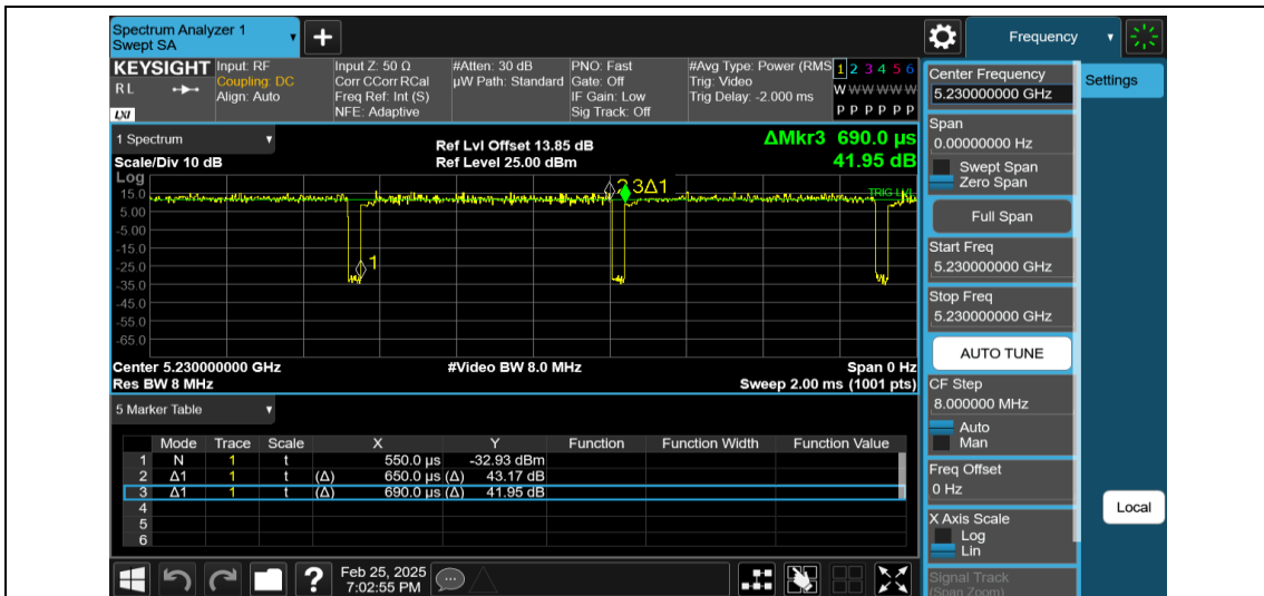
NTNV-11AC40MIMO-Ant2-5230
