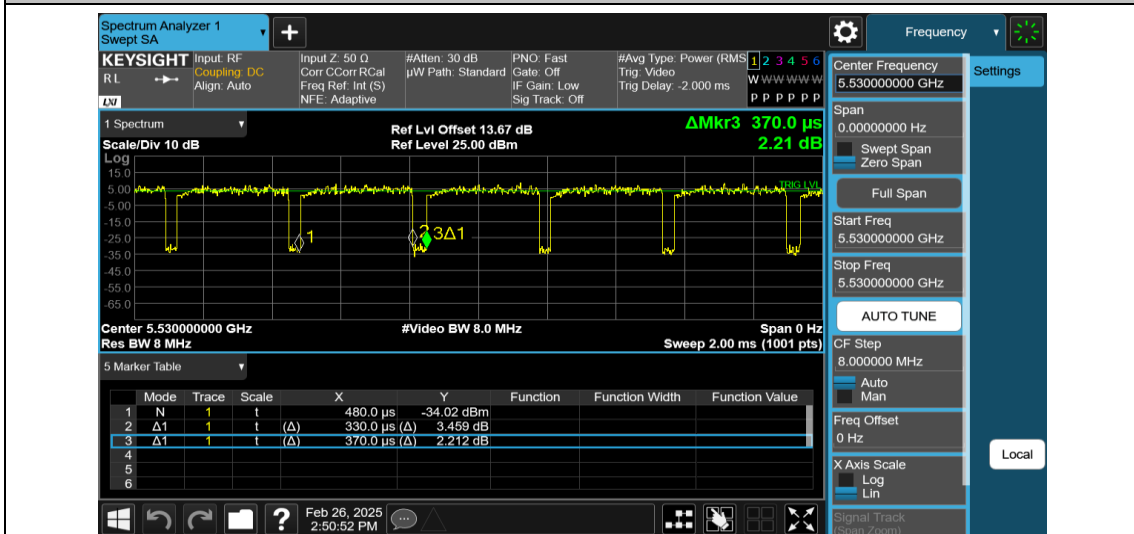
NTNV-11AC80MIMO-Ant2-5530
