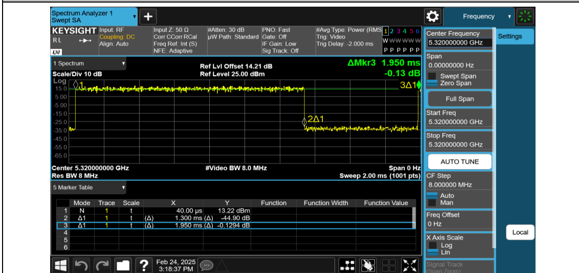
NTNV-11N20MIMO-Ant2-5320
