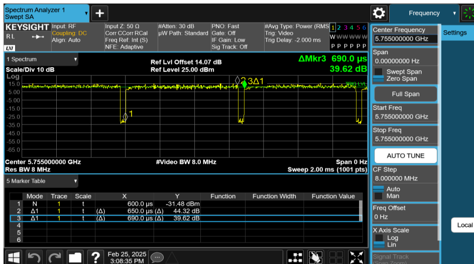
NTNV-11N40MIMO-Ant2-5755
