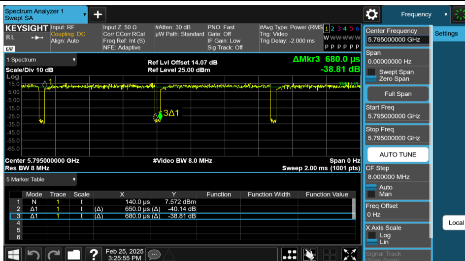
NTNV-11N40MIMO-Ant2-5795
