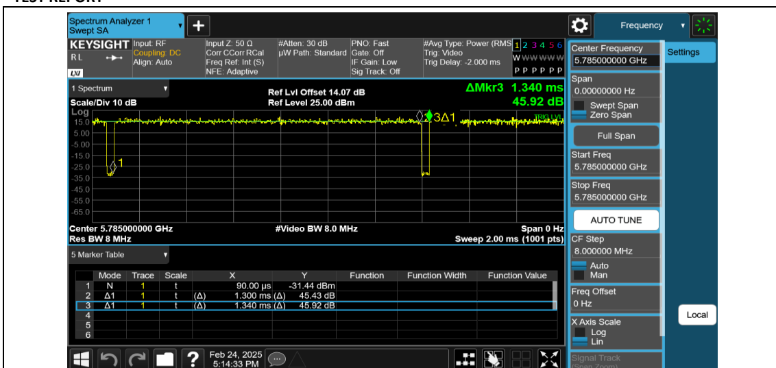
NTNV-11N20MIMO-Ant2-5785
