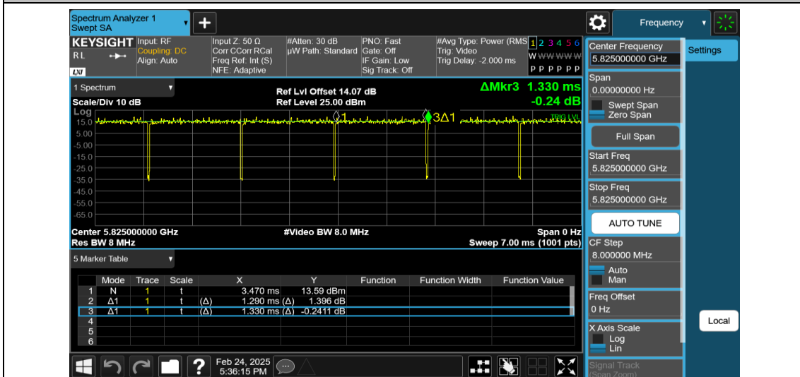
NTNV-11N20MIMO-Ant2-5825
