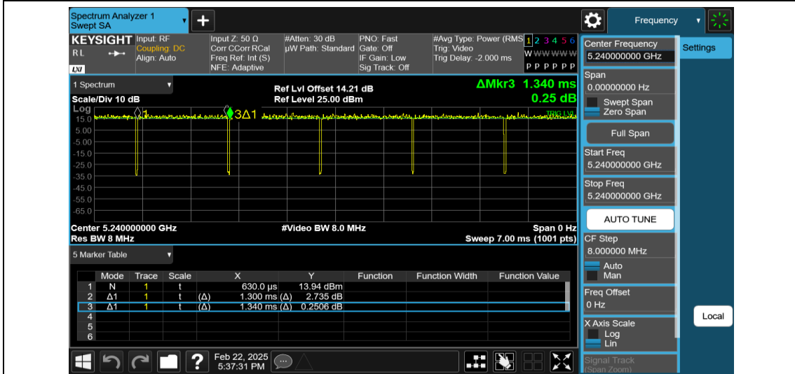
NTNV-11N20MIMO-Ant2-5240
