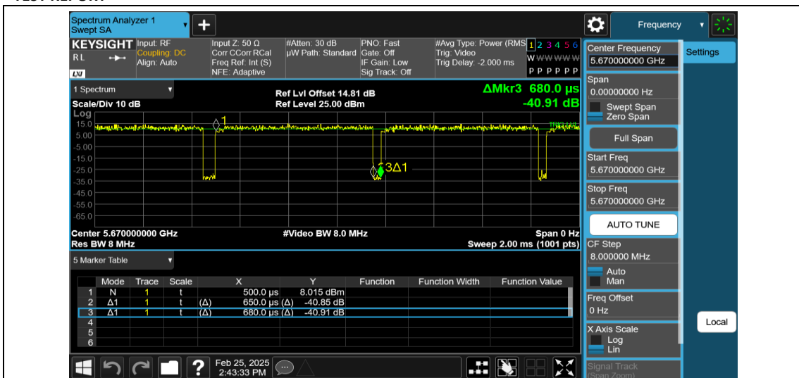
NTNV-11N40MIMO-Ant1-5670
