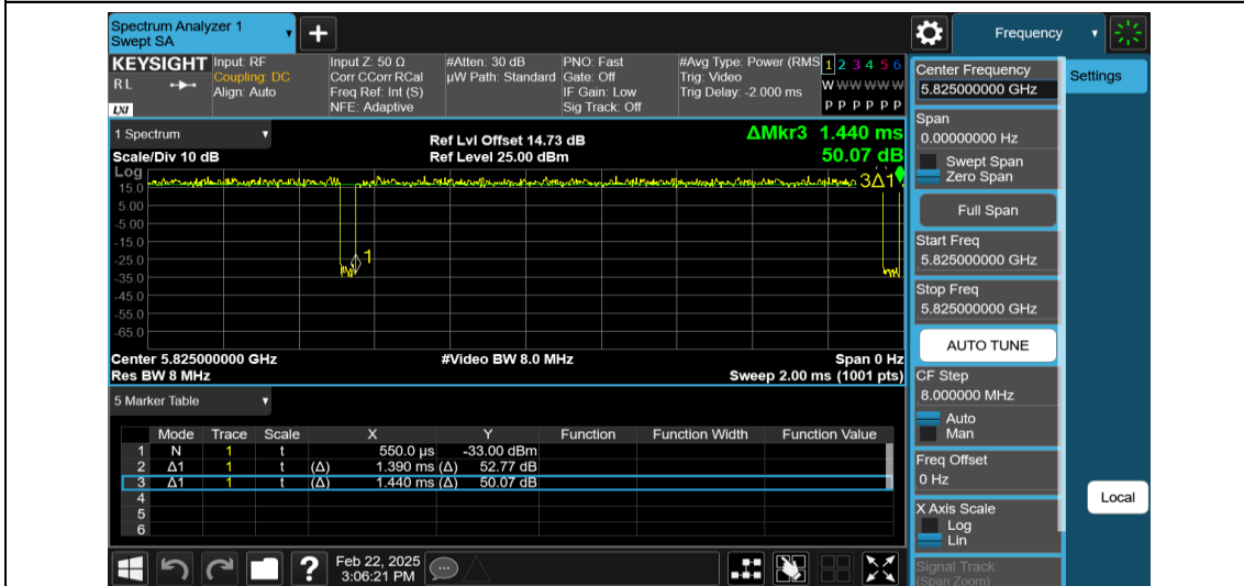
NTNV-11A-Ant1-5825
