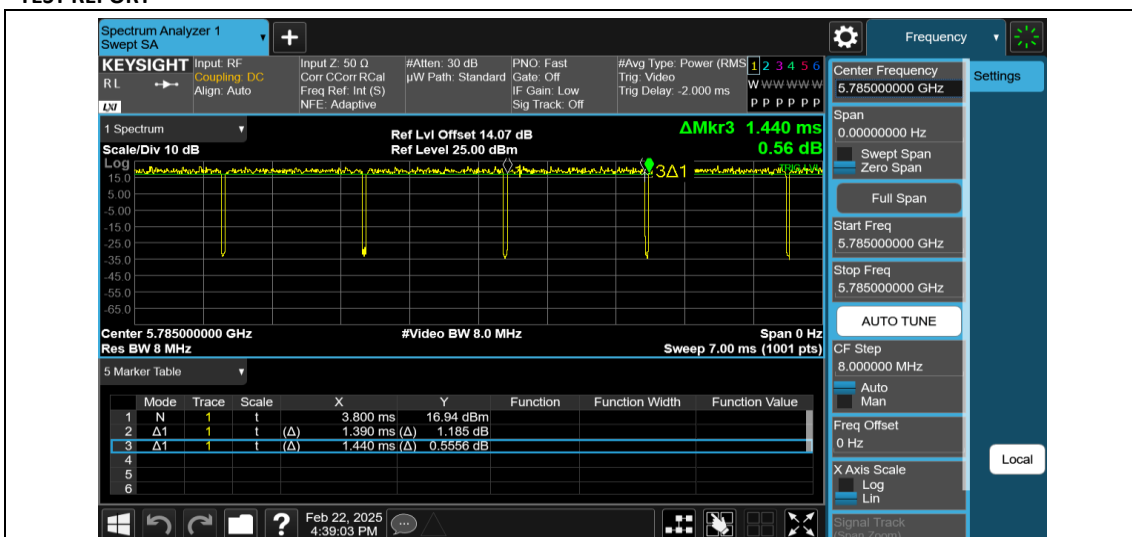
NTNV-11A-Ant2-5785
