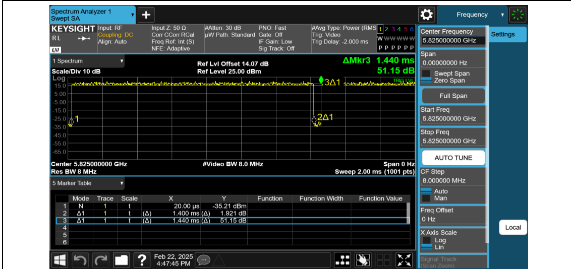
NTNV-11A-Ant2-5825
