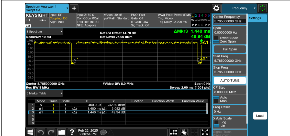
NTNV-11A-Ant1-5785
