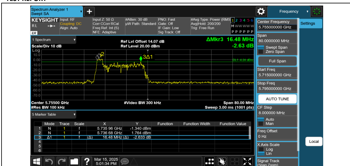
11AX40MIMO-Ant2-5755-26Tone-RU0-PASS
