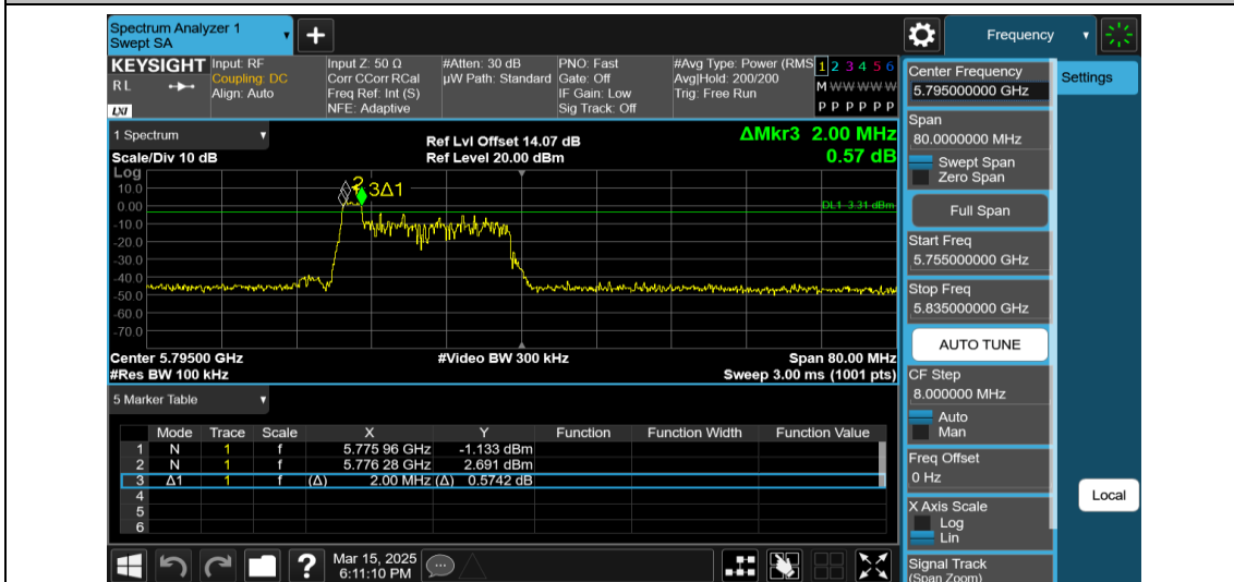
11AX40MIMO-Ant2-5795-26Tone-RU0-PASS
