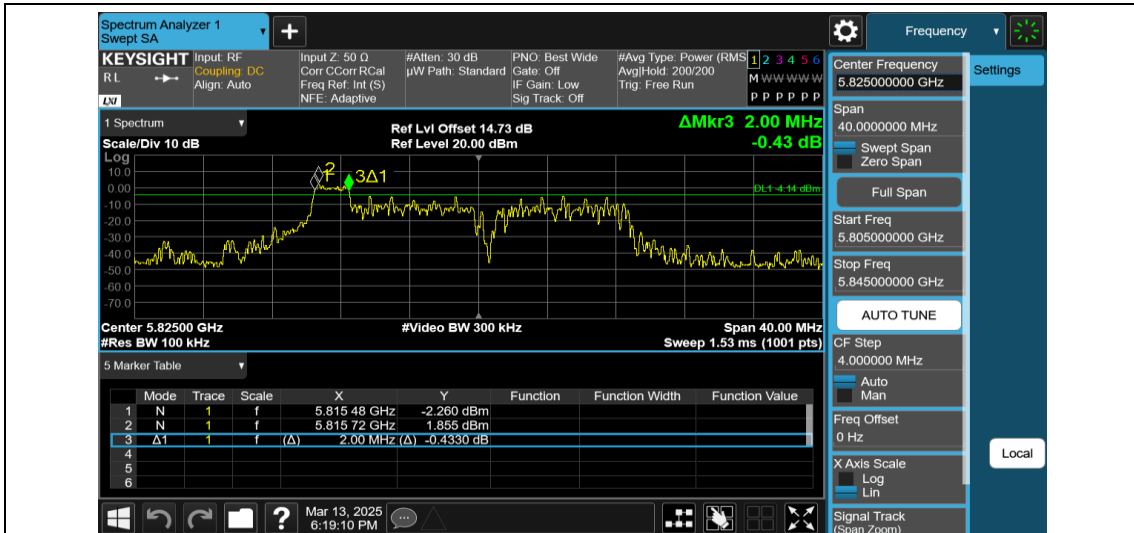
11AX20MIMO-Ant1-5825-26Tone-RU0-PASS
