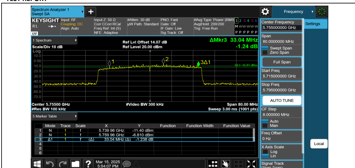
11AX40MIMO-Ant2-5755-484Tone-RU65-PASS
