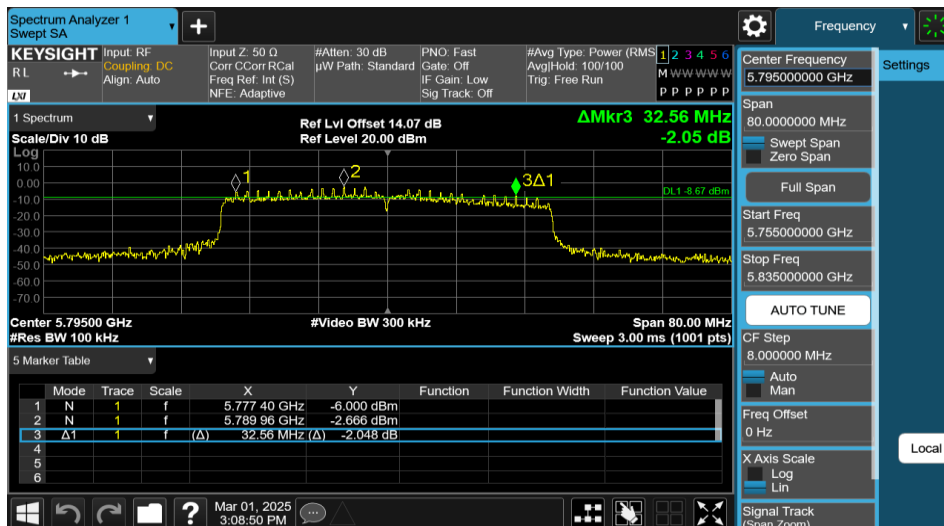
11AX40MIMO-Ant2-5795-PASS
