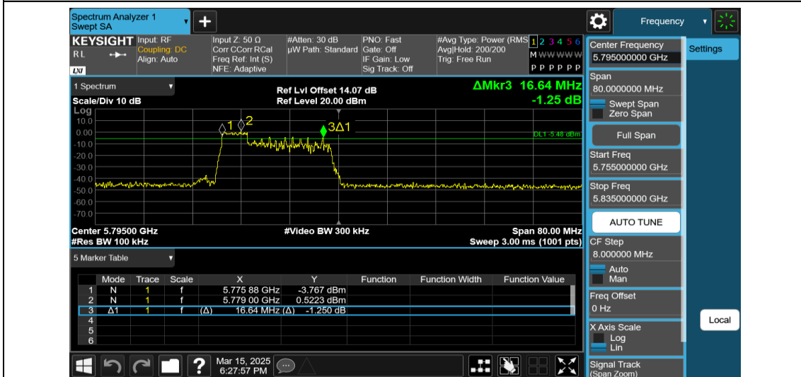
11AX40MIMO-Ant2-5795-52Tone-RU37-PASS
