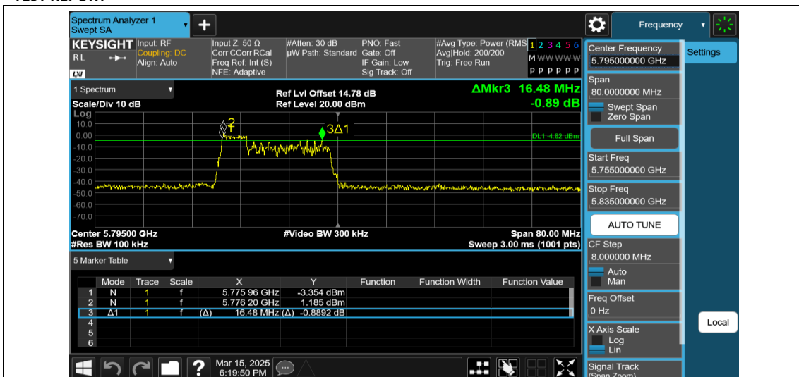
11AX40MIMO-Ant1-5795-52Tone-RU37-PASS
