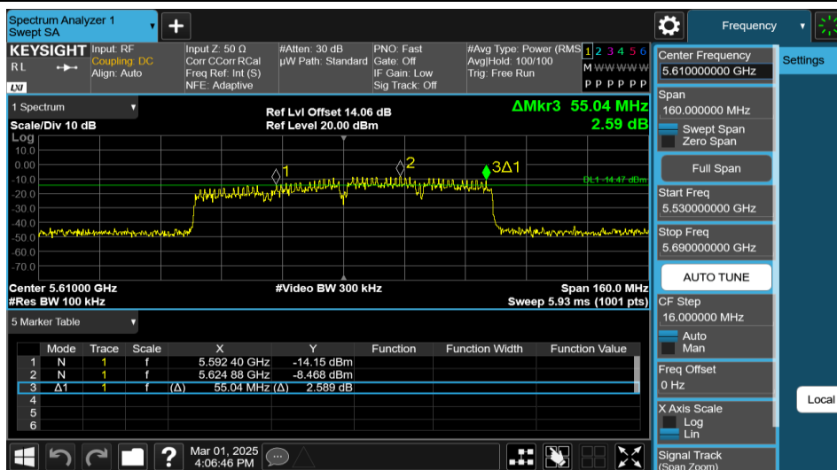
11AX80MIMO-Ant2-5610-PASS
