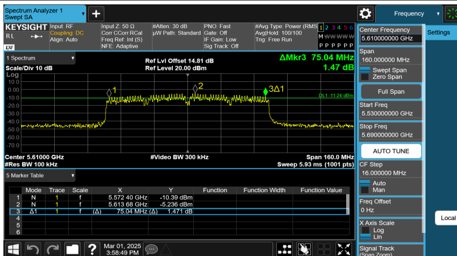
11AX80MIMO-Ant1-5610-PASS
