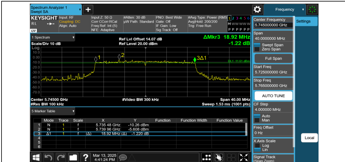
11AX20MIMO-Ant2-5745-242Tone-RU61-PASS
