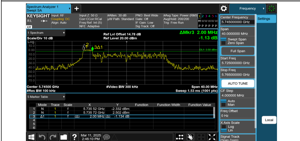
11AX20MIMO-Ant1-5745-26Tone-RU0-PASS
