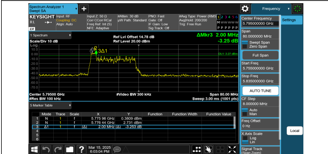
11AX40MIMO-Ant1-5795-26Tone-RU0-PASS
