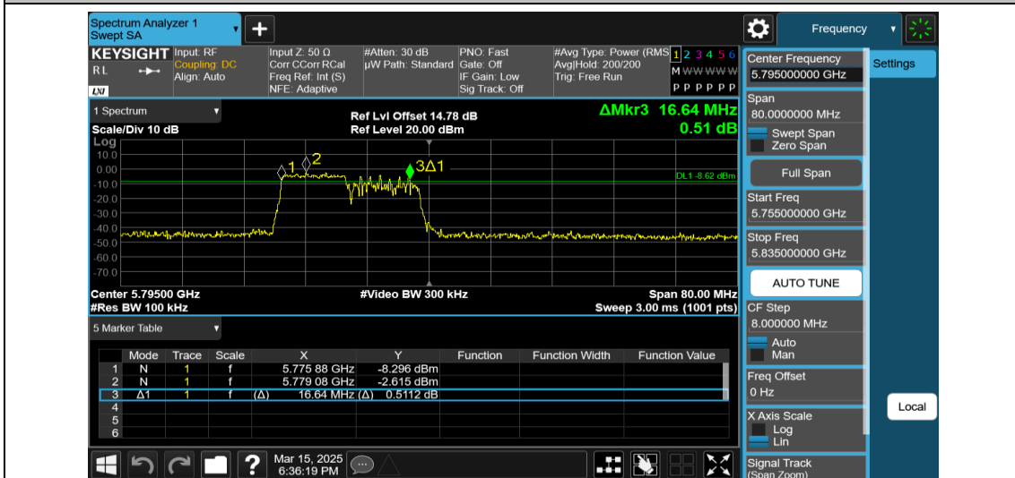
11AX40MIMO-Ant1-5795-106Tone-RU53-PASS
