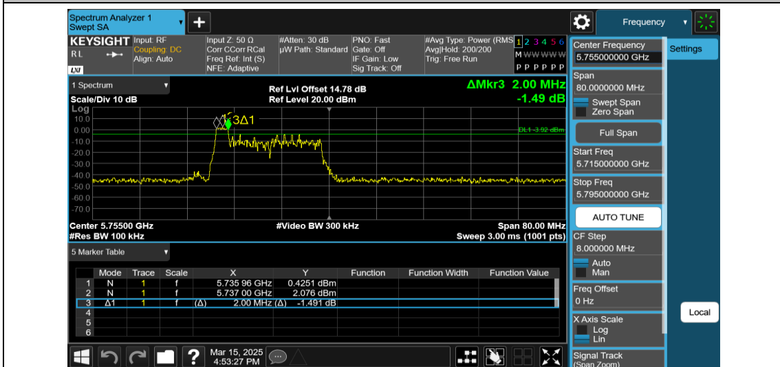
11AX40MIMO-Ant1-5755-26Tone-RU0-PASS
