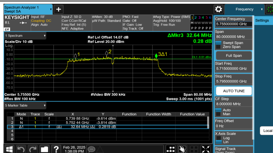
11AC40MIMO-Ant2-5755-PASS
