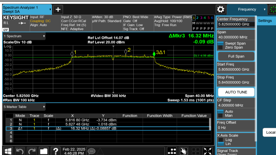
11A-Ant2-5825-PASS
