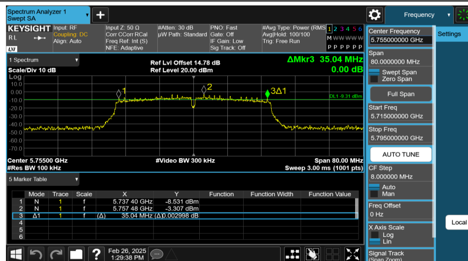
11AC40MIMO-Ant1-5755-PASS
