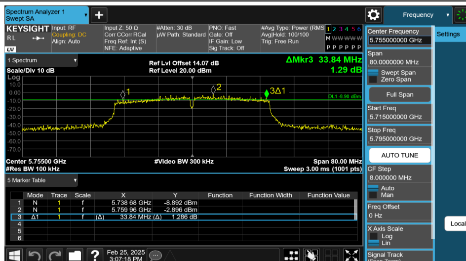
11N40MIMO-Ant2-5755-PASS
