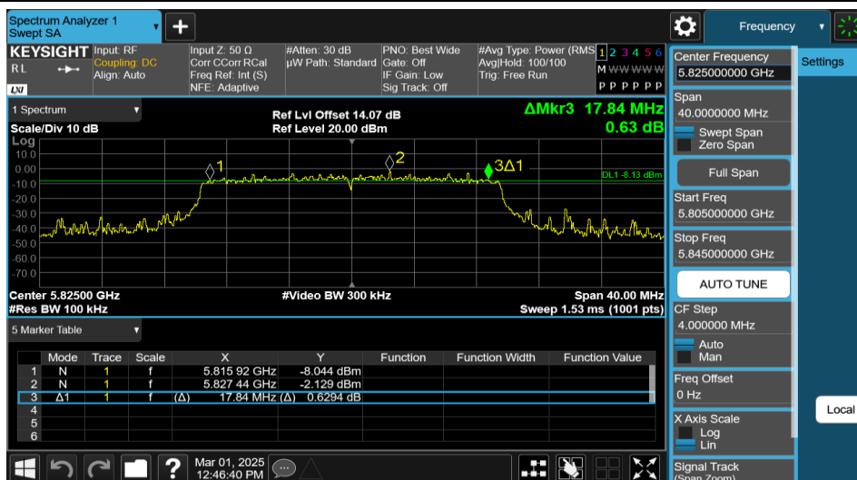
11AX20MIMO-Ant2-5825-PASS
