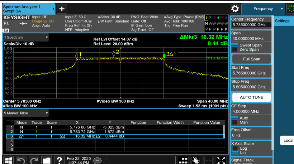
11A-Ant2-5785-PASS
