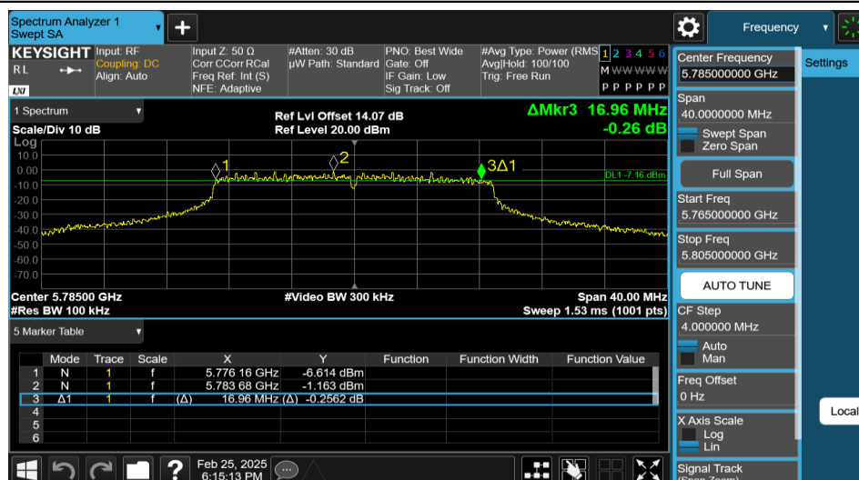
11AC20MIMO-Ant2-5785-PASS
