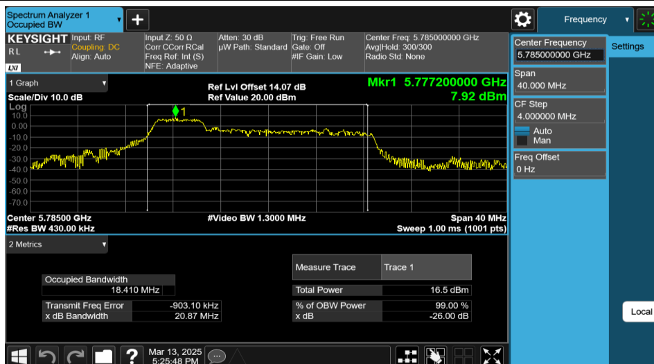
11AX20MIMO-Ant2-5785-52Tone-RU37
