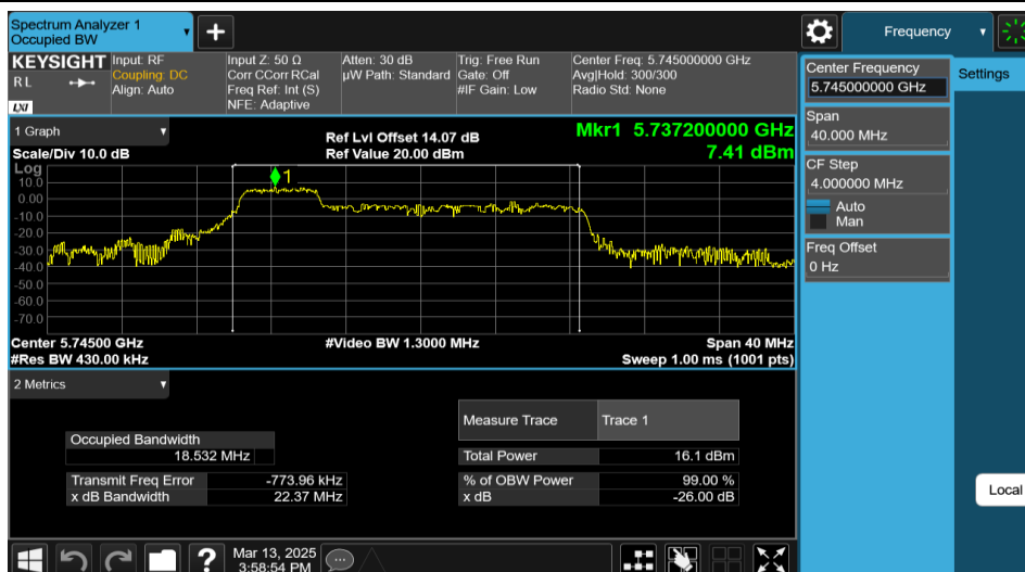
11AX20MIMO-Ant2-5745-52Tone-RU37
