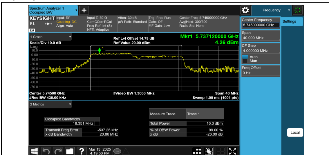
11AX20MIMO-Ant1-5745-106Tone-RU53
