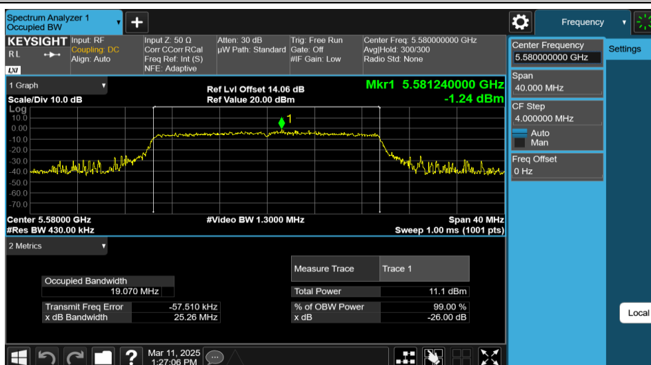
11AX20MIMO-Ant2-5580-242Tone-RU61
