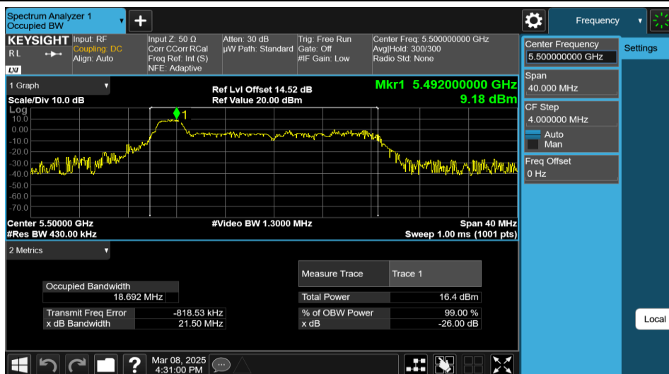
11AX20MIMO-Ant1-5500-26Tone-RU0
