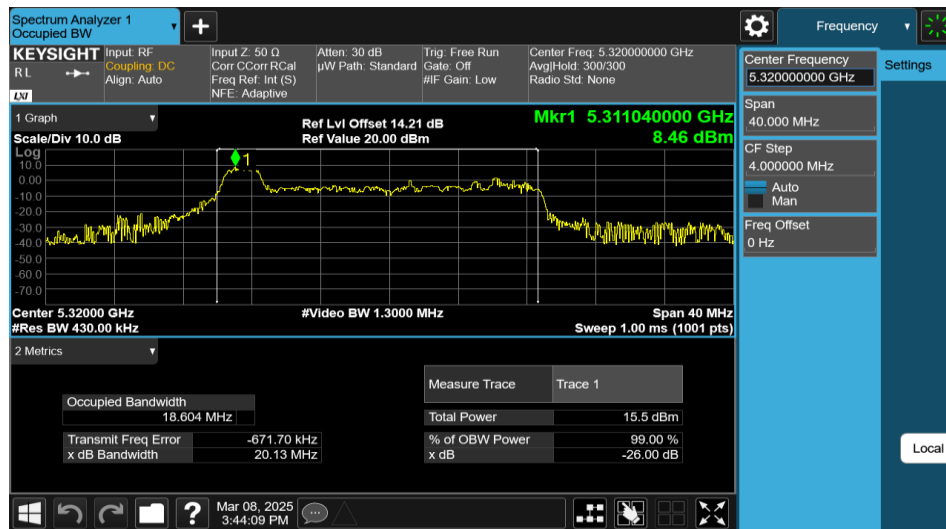
11AX20MIMO-Ant2-5320-26Tone-RU0
