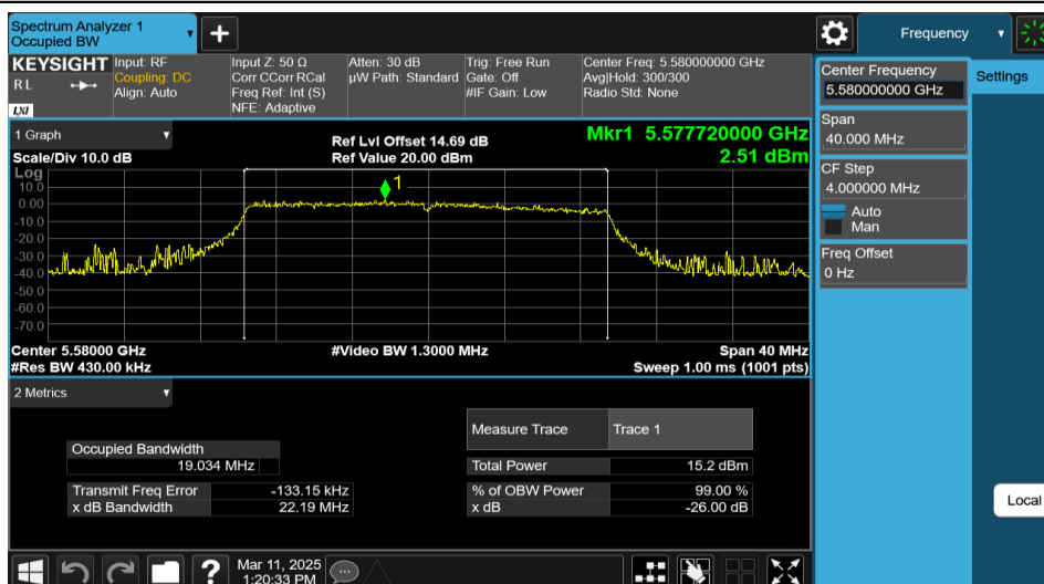
11AX20MIMO-Ant1-5580-242Tone-RU61
