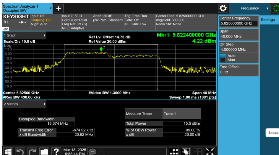
11AX20MIMO-Ant1-5825-106Tone-RU53
