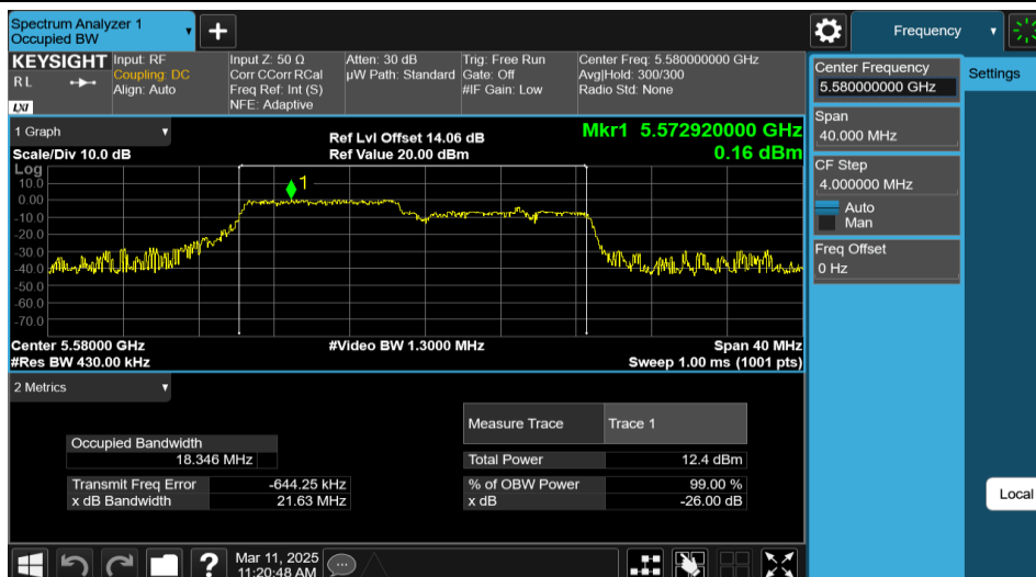
11AX20MIMO-Ant2-5580-106Tone-RU53
