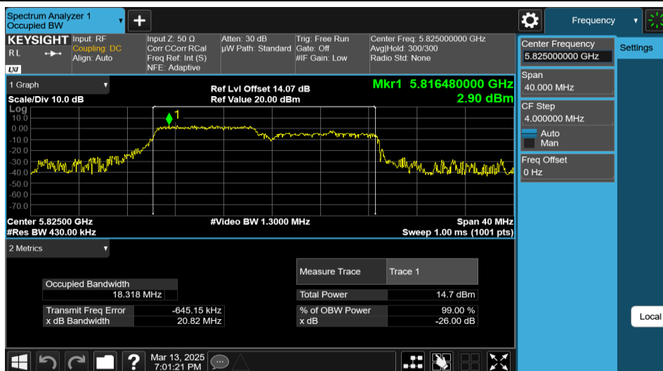
11AX20MIMO-Ant2-5825-106Tone-RU53
