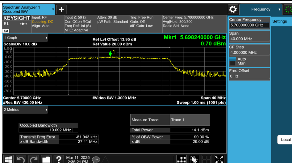
11AX20MIMO-Ant2-5700-242Tone-RU61
