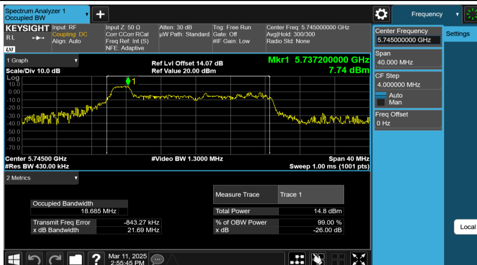
11AX20MIMO-Ant2-5745-26Tone-RU0
