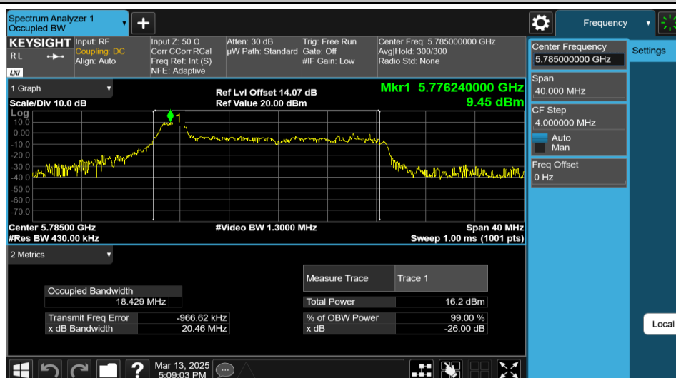
11AX20MIMO-Ant2-5785-26Tone-RU0
