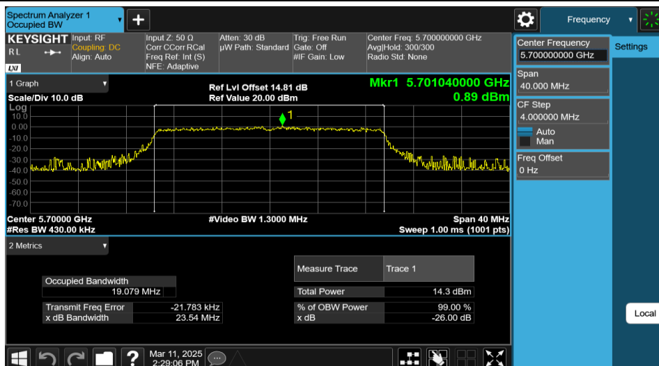
11AX20MIMO-Ant1-5700-242Tone-RU61
