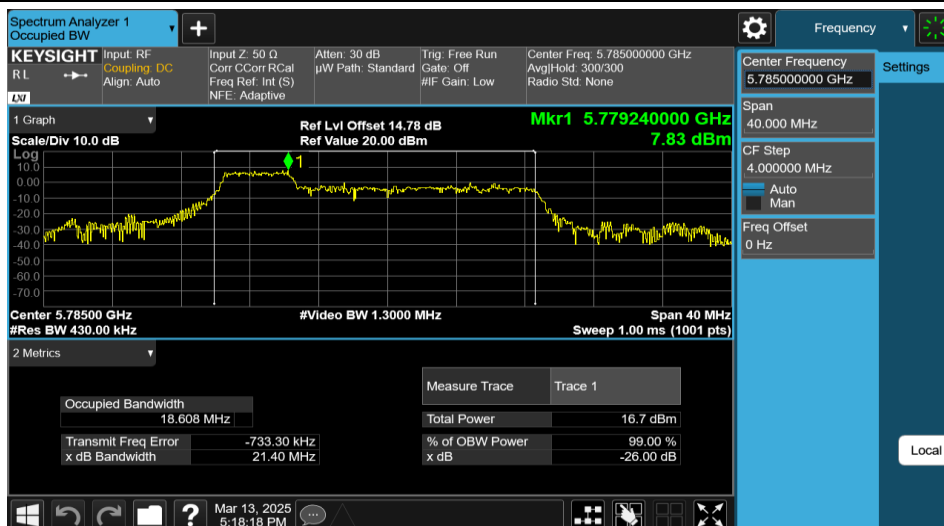
11AX20MIMO-Ant1-5785-52Tone-RU37
