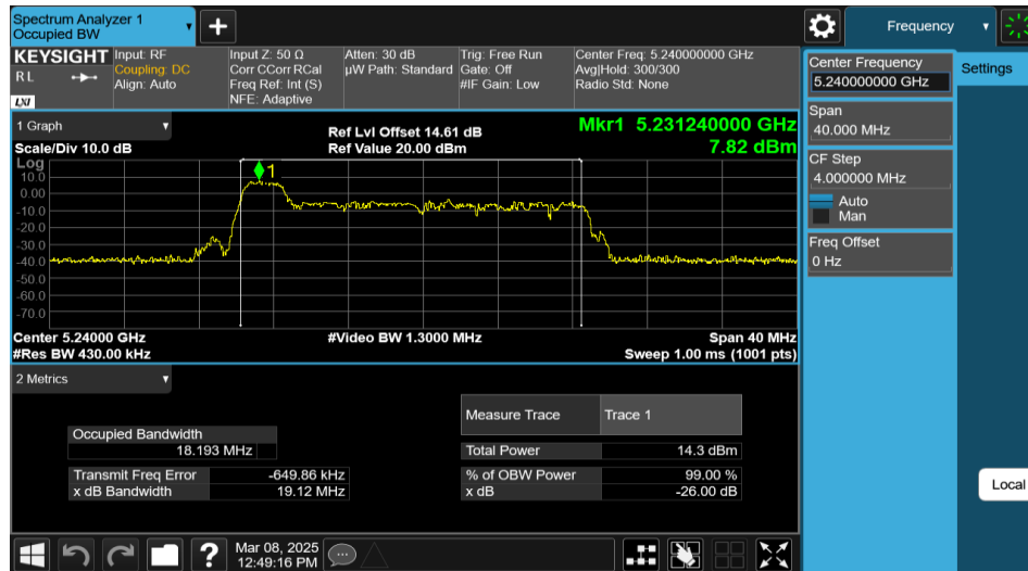
11AX20MIMO-Ant1-5240-26Tone-RU0
