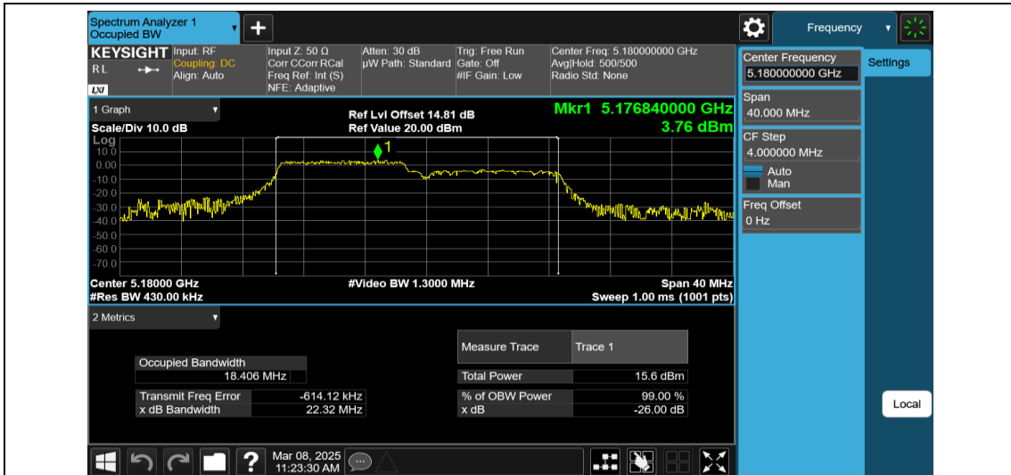
11AX20MIMO-Ant1-5180-106Tone-RU53
