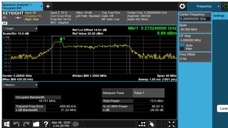
11AX20MIMO-Ant1-5280-26Tone-RU0
