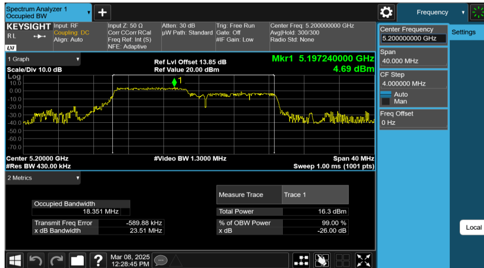
11AX20MIMO-Ant2-5200-106Tone-RU53
