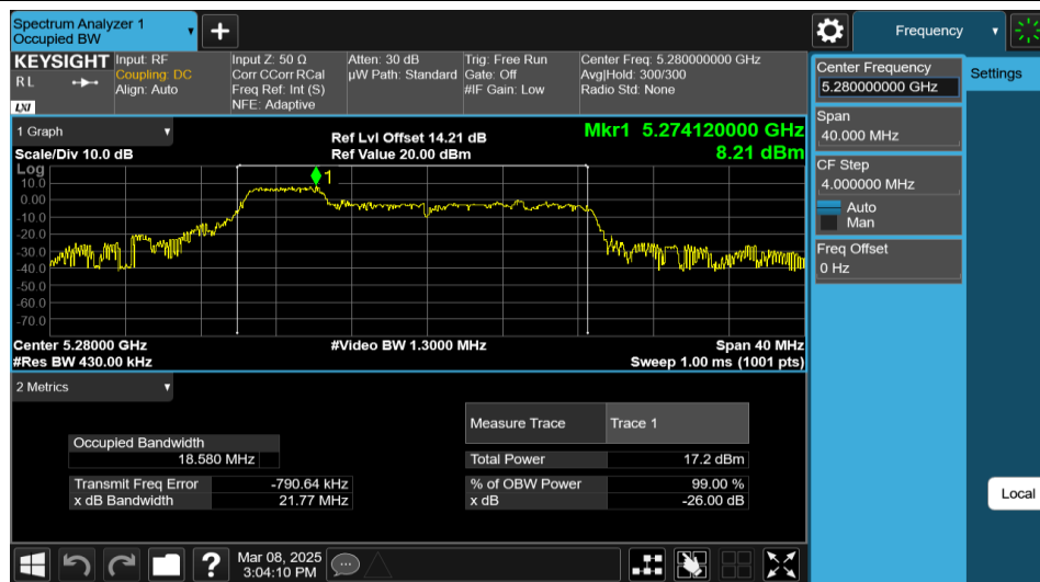
11AX20MIMO-Ant2-5280-52Tone-RU37
