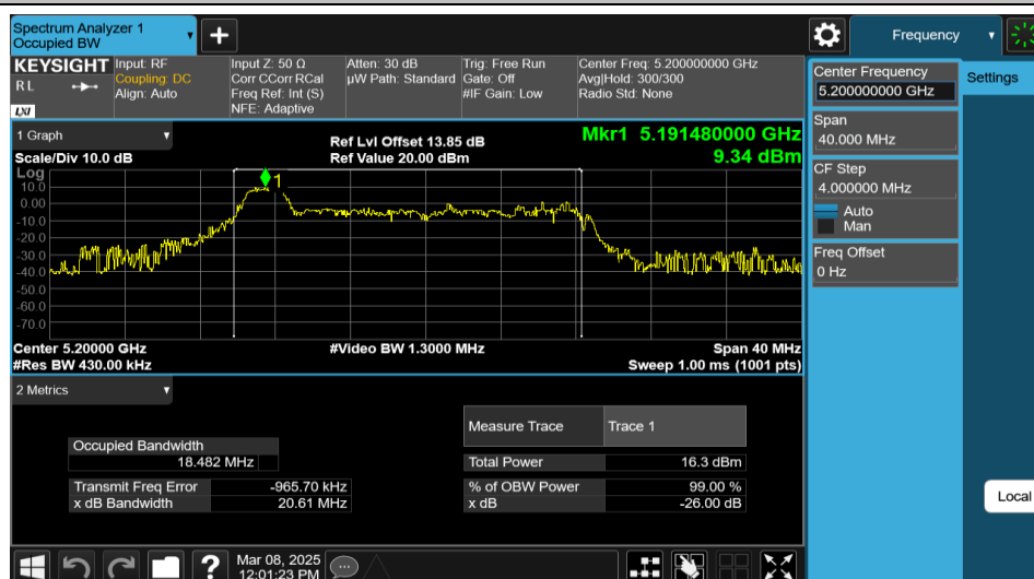
11AX20MIMO-Ant2-5200-26Tone-RU0
