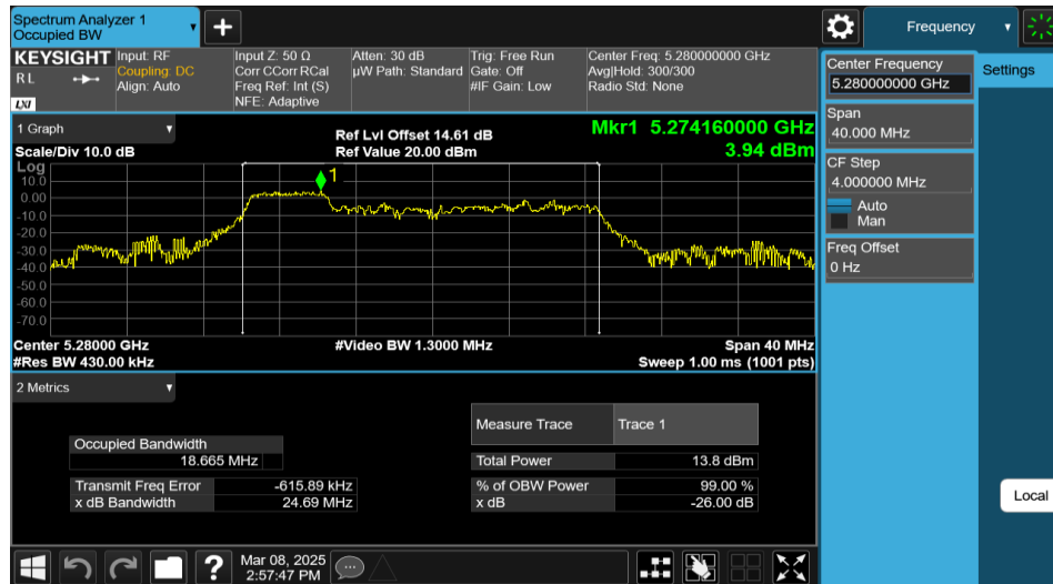
11AX20MIMO-Ant1-5280-52Tone-RU37
