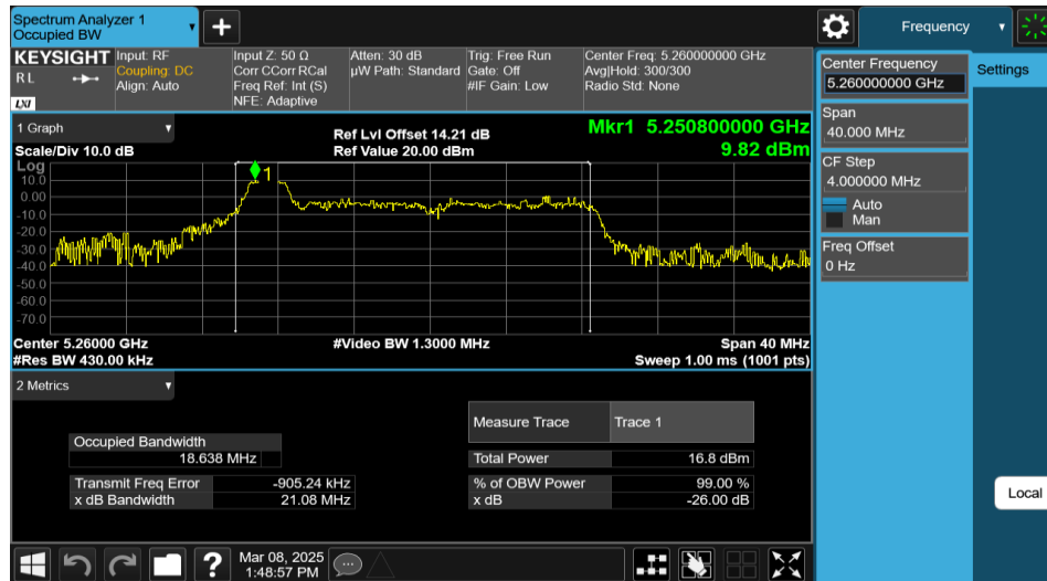
11AX20MIMO-Ant2-5260-26Tone-RU0
