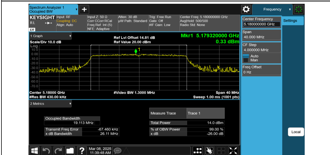
11AX20MIMO-Ant1-5180-242Tone-RU61
