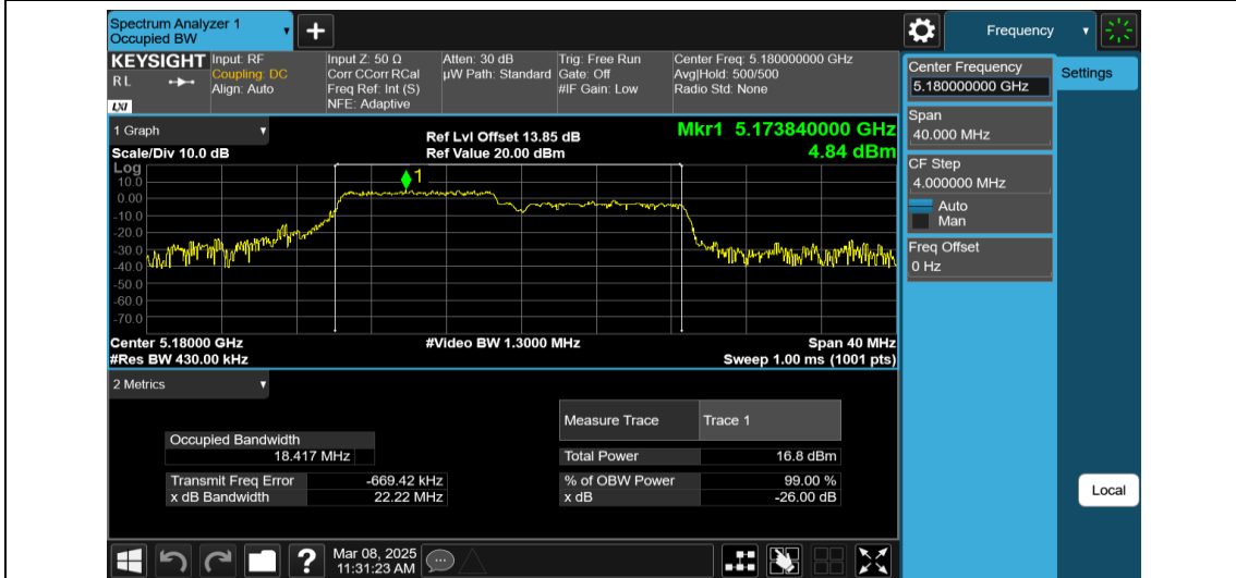
11AX20MIMO-Ant2-5180-106Tone-RU53
