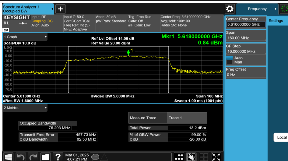
11AX80MIMO-Ant2-5610
