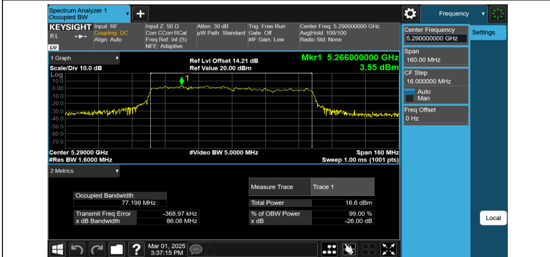
11AX80MIMO-Ant2-5290
