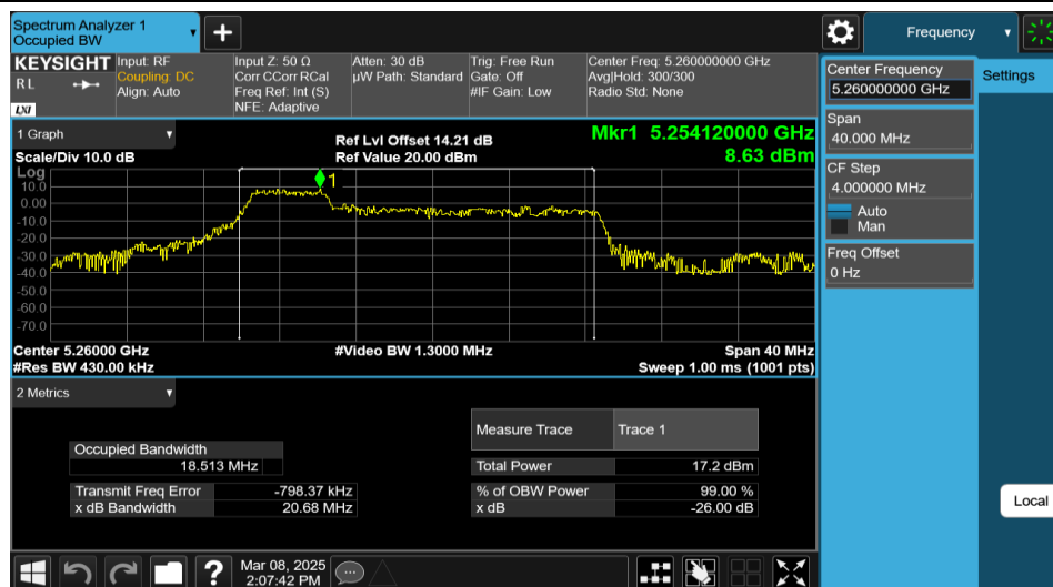
11AX20MIMO-Ant2-5260-52Tone-RU37
