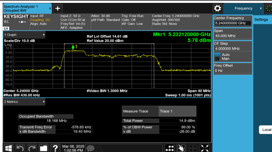
11AX20MIMO-Ant1-5240-52Tone-RU37
