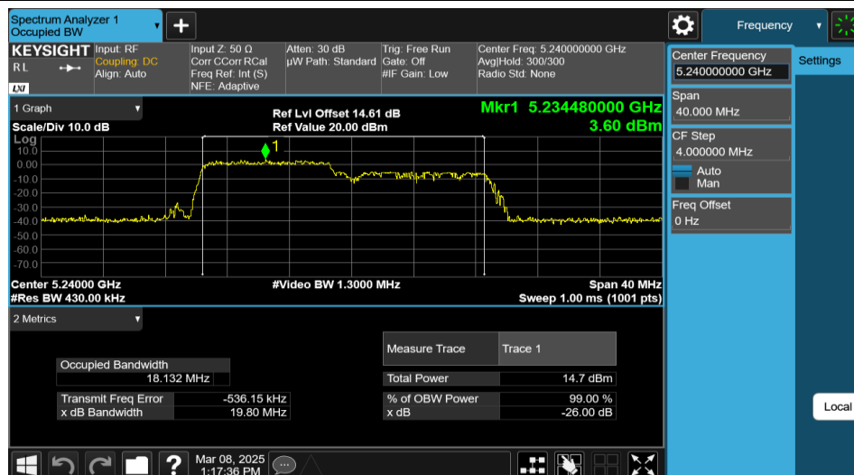
11AX20MIMO-Ant1-5240-106Tone-RU53
