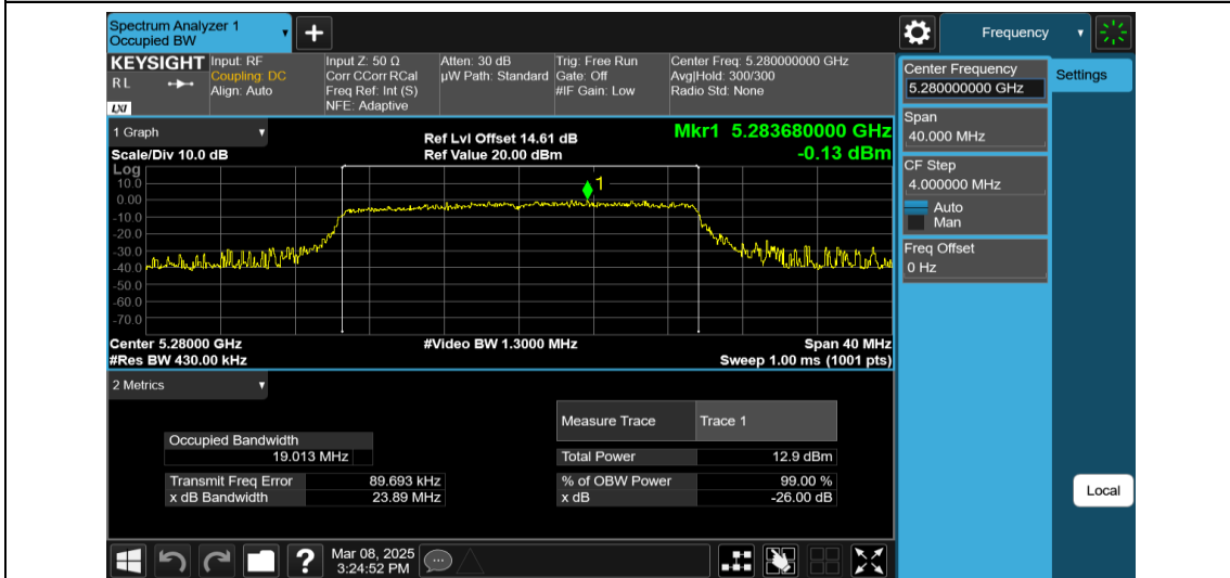
11AX20MIMO-Ant1-5280-242Tone-RU61
