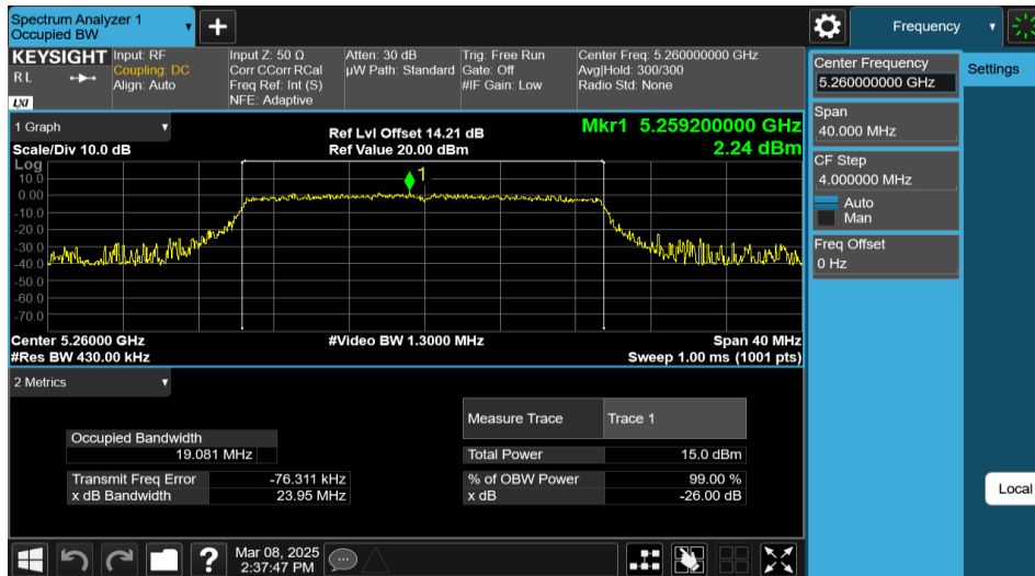
11AX20MIMO-Ant2-5260-242Tone-RU61
