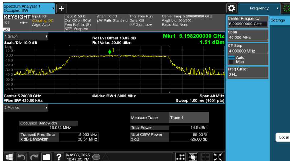
11AX20MIMO-Ant2-5200-242Tone-RU61
