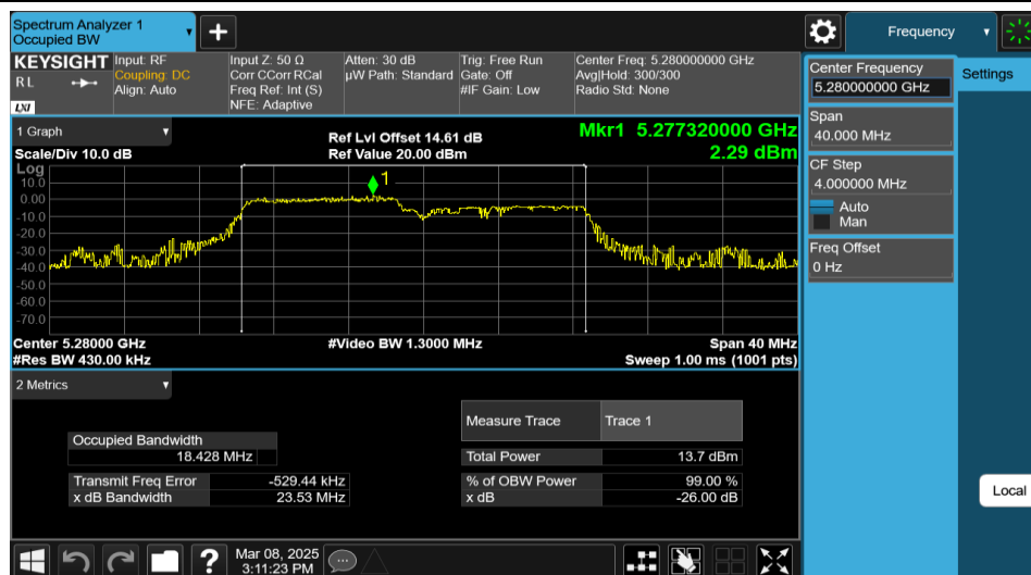
11AX20MIMO-Ant1-5280-106Tone-RU53
