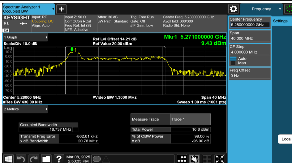
11AX20MIMO-Ant2-5280-26Tone-RU0
