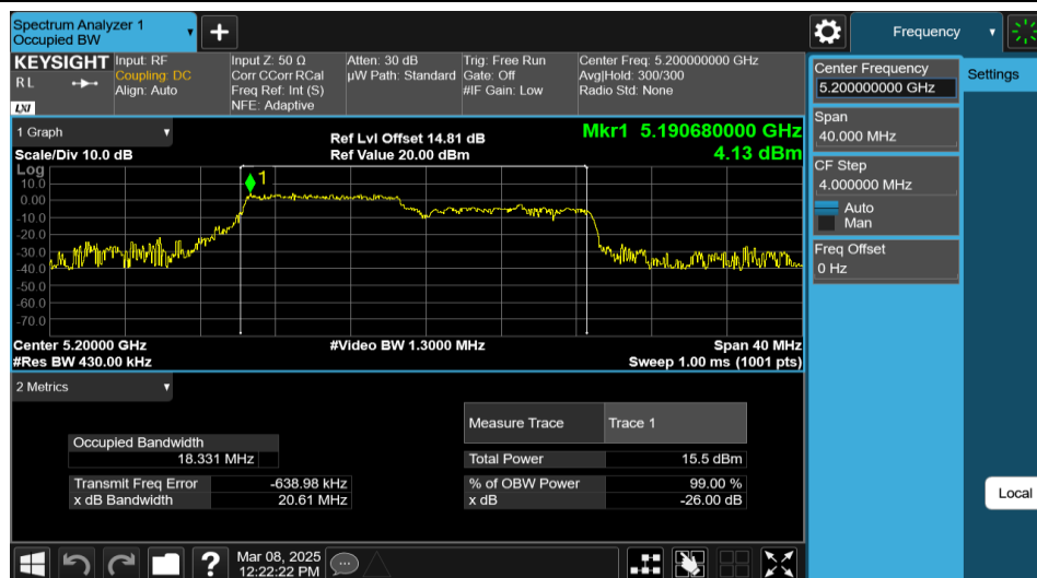
11AX20MIMO-Ant1-5200-106Tone-RU53
