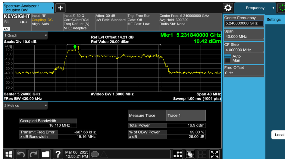
11AX20MIMO-Ant2-5240-26Tone-RU0
