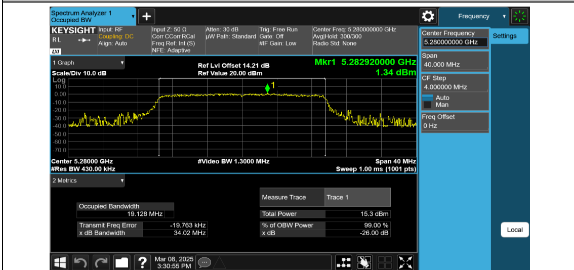
11AX20MIMO-Ant2-5280-242Tone-RU61
