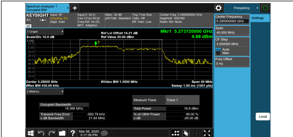
11AX20MIMO-Ant2-5280-106Tone-RU53
