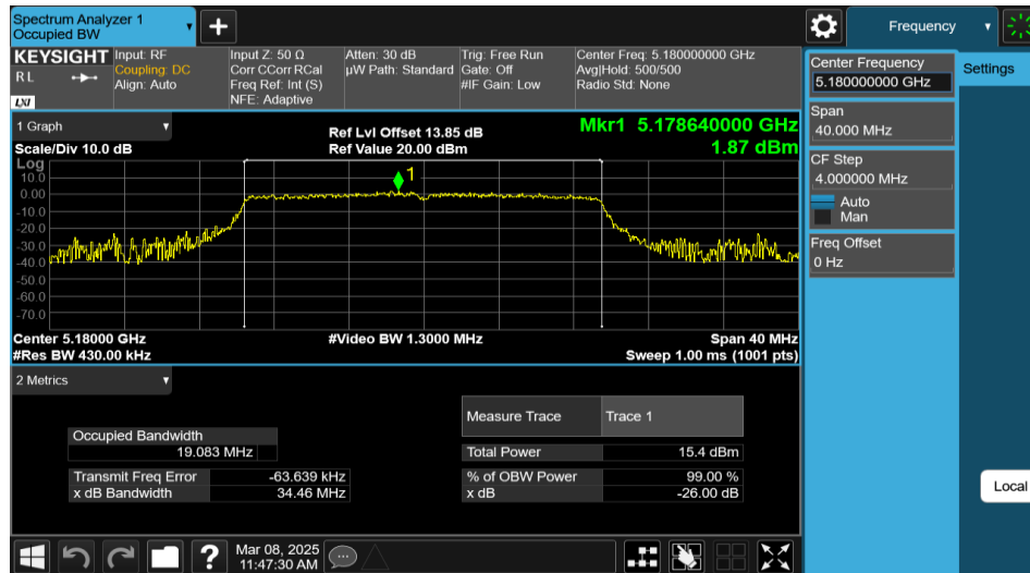
11AX20MIMO-Ant2-5180-242Tone-RU61
