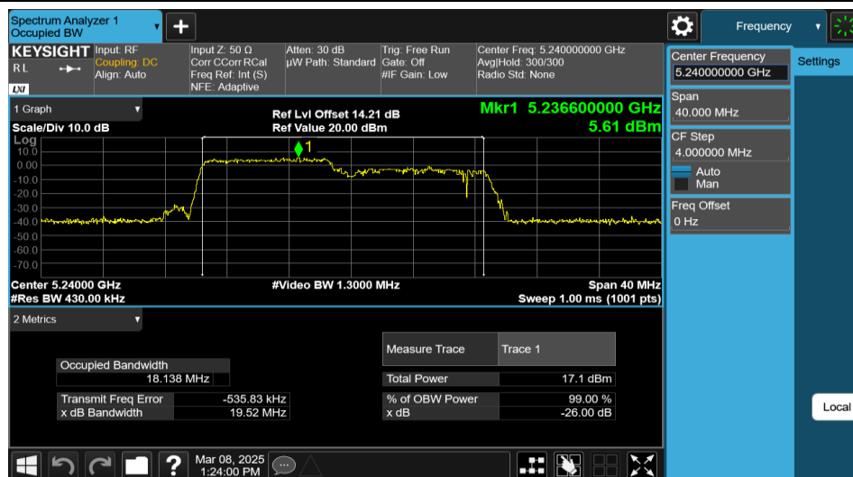
11AX20MIMO-Ant2-5240-106Tone-RU53
