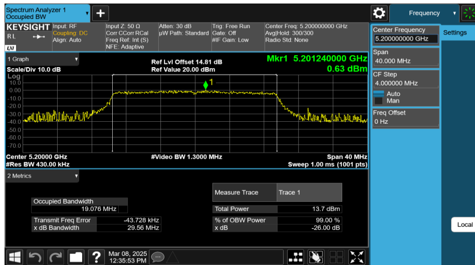
11AX20MIMO-Ant1-5200-242Tone-RU61
