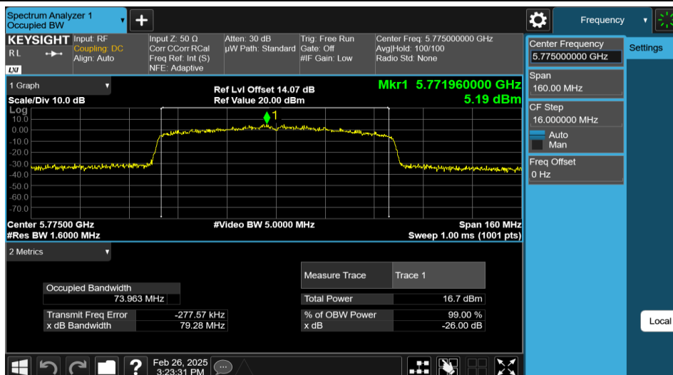
11AC80MIMO-Ant2-5775
