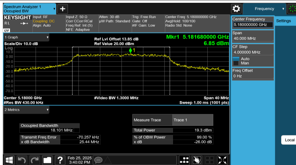
11AC20MIMO-Ant2-5180
