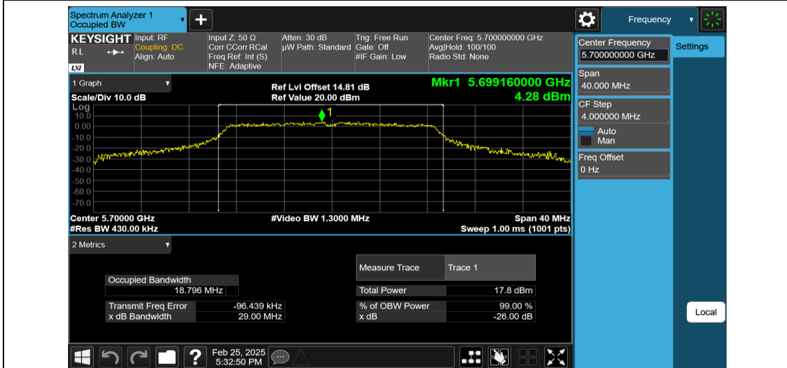
11AC20MIMO-Ant1-5700
