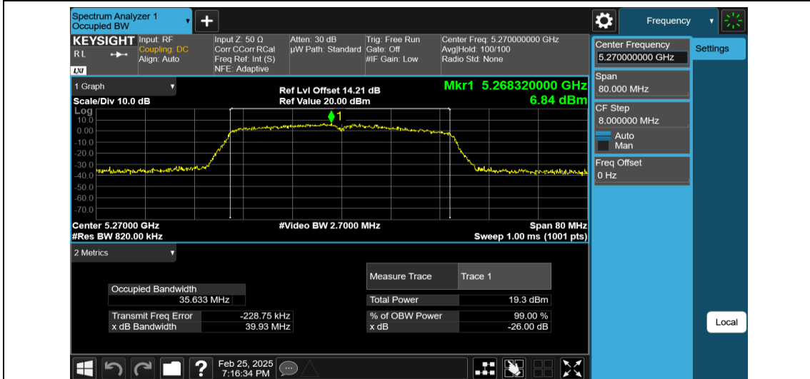
11AC40MIMO-Ant2-5270
