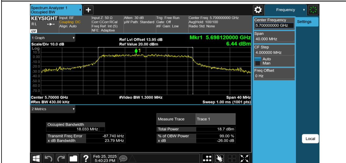
11AC20MIMO-Ant2-5700
