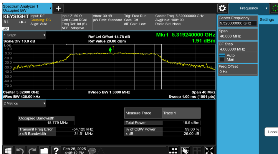
11AC20MIMO-Ant1-5320
