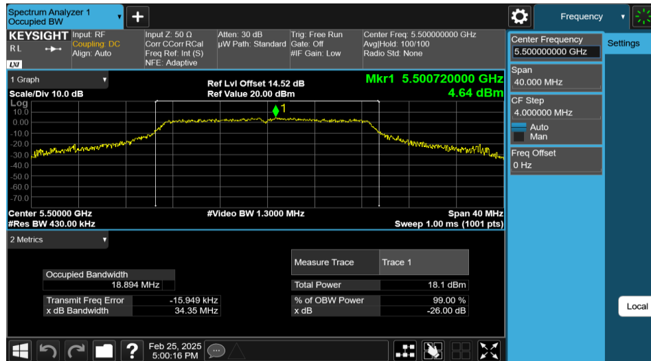
11AC20MIMO-Ant1-5500
