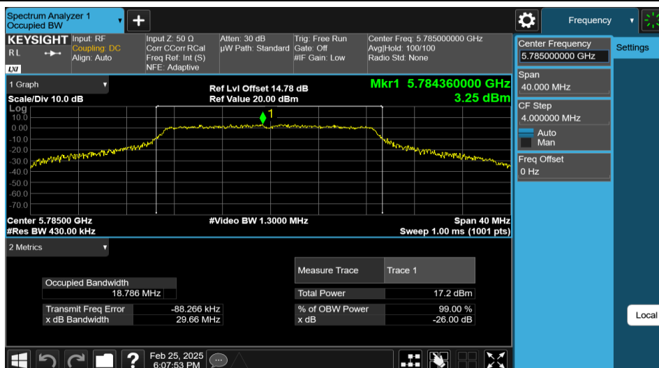
11AC20MIMO-Ant1-5785
