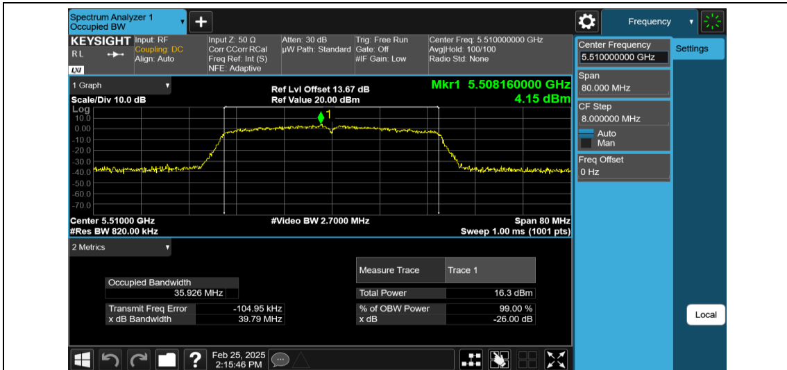
11N40MIMO-Ant2-5510
