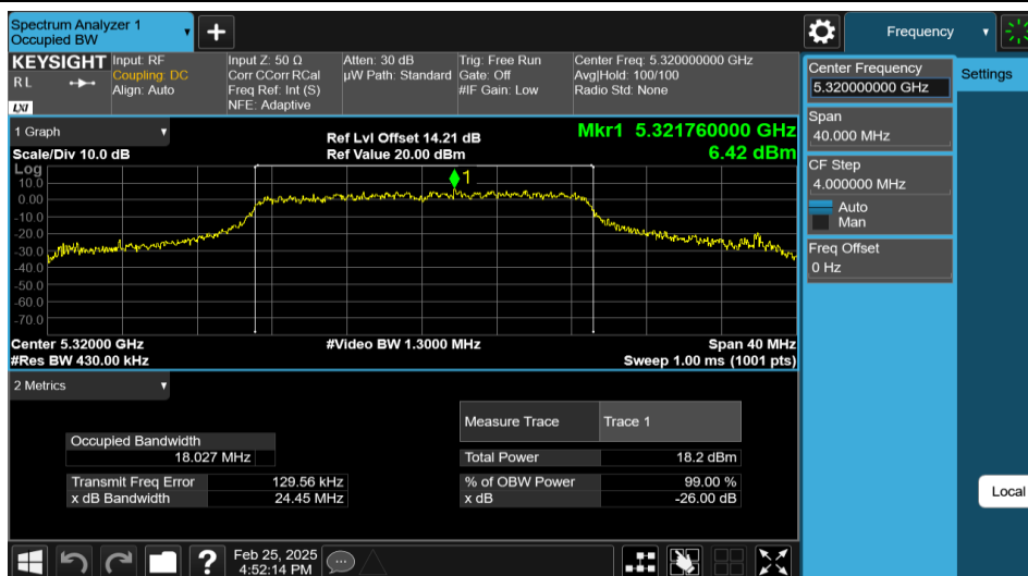
11AC20MIMO-Ant2-5320
