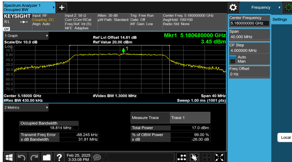
11AC20MIMO-Ant1-5180
