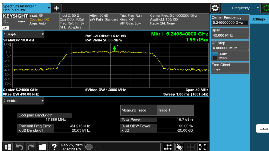
11AC20MIMO-Ant1-5240
