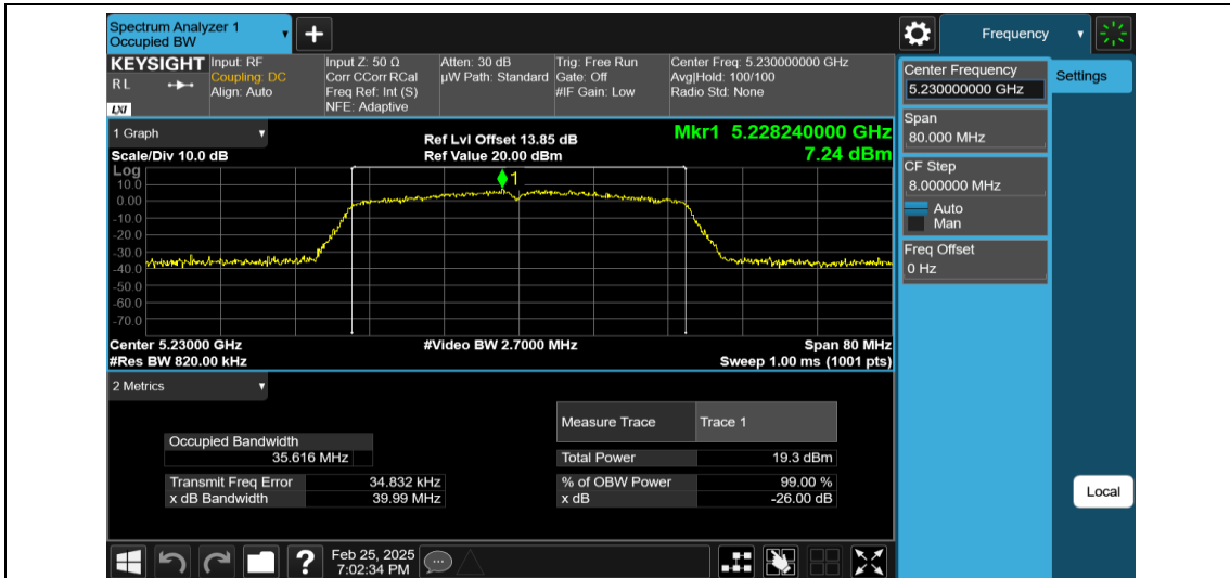
11AC40MIMO-Ant2-5230
