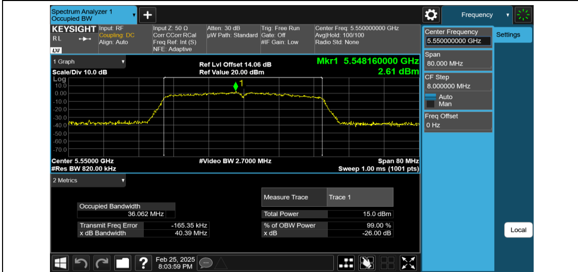
11AC40MIMO-Ant2-5550
