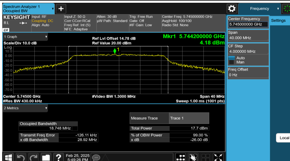
11AC20MIMO-Ant1-5745
