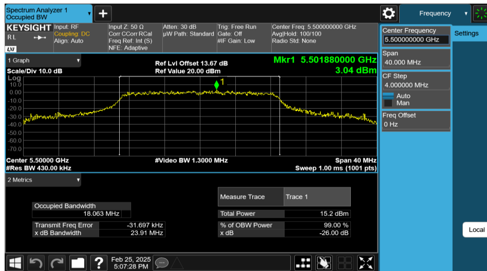
11AC20MIMO-Ant2-5500
