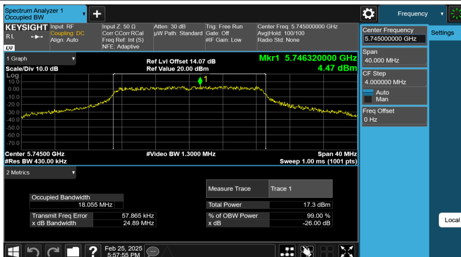
11AC20MIMO-Ant2-5745
