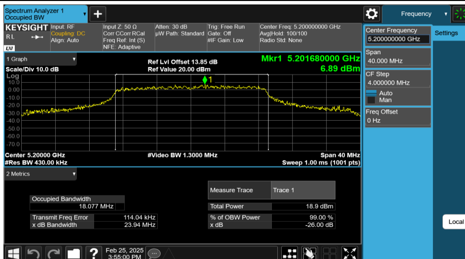
11AC20MIMO-Ant2-5200
