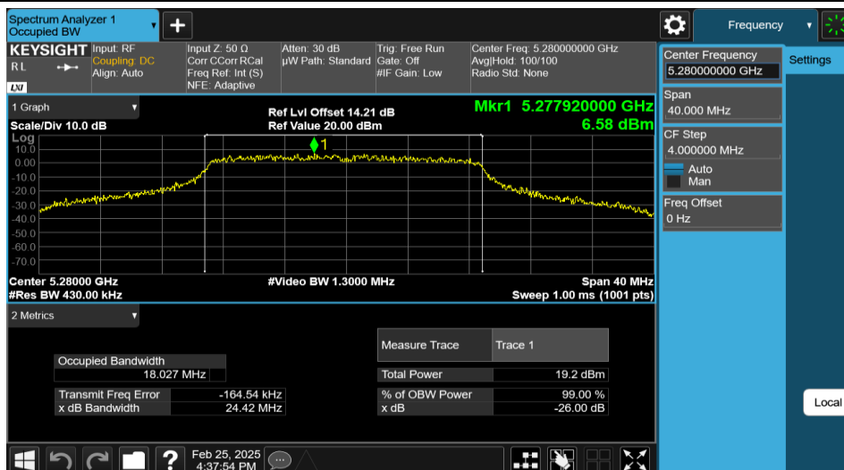
11AC20MIMO-Ant2-5280
