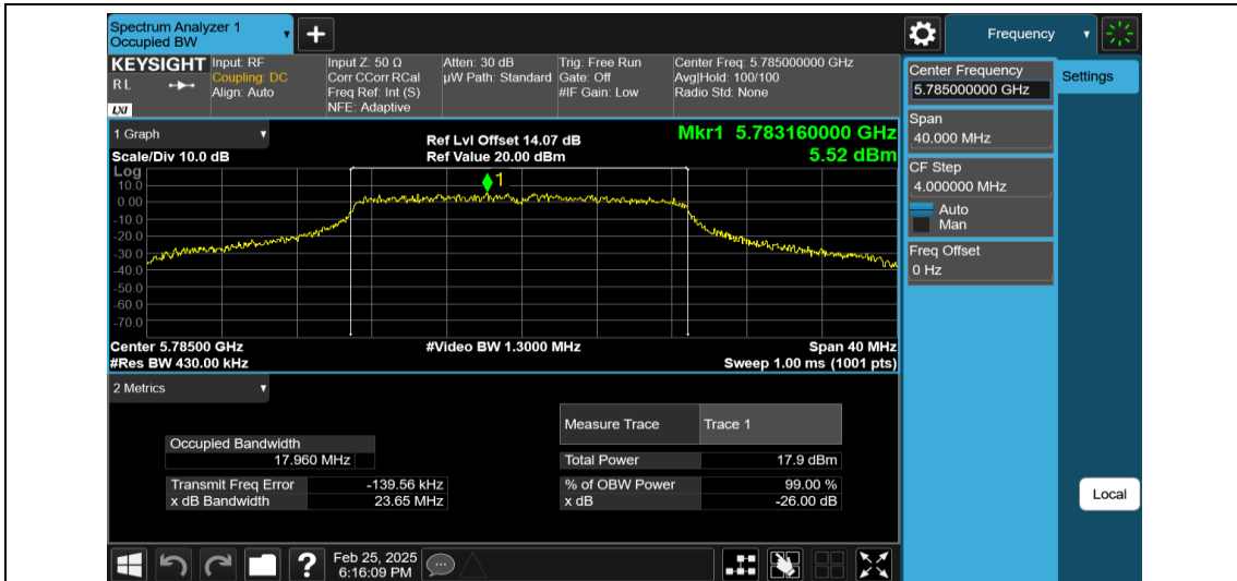
11AC20MIMO-Ant2-5785
