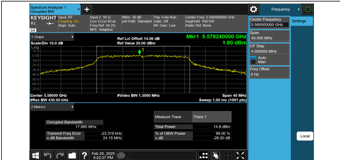
11AC20MIMO-Ant2-5580
