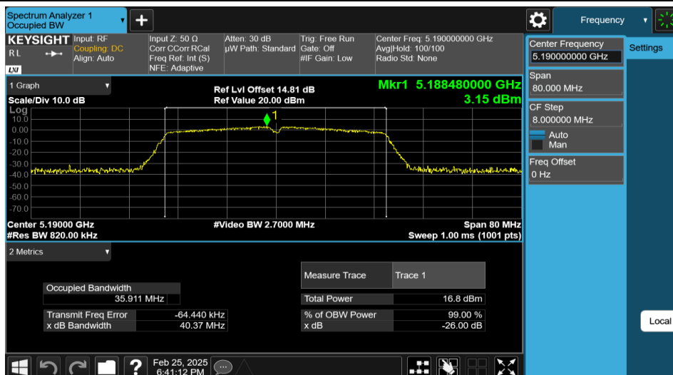
11AC40MIMO-Ant1-5190
