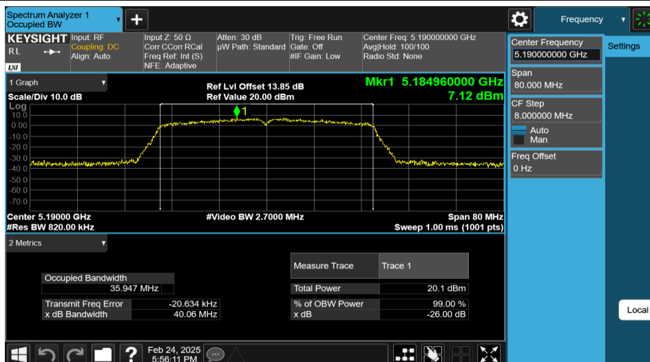
11N40MIMO-Ant2-5190
