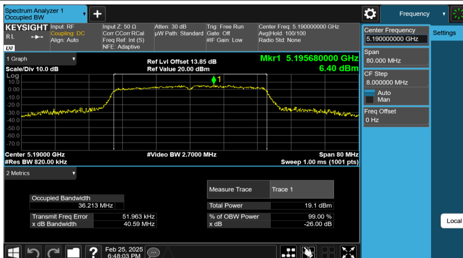
11AC40MIMO-Ant2-5190
