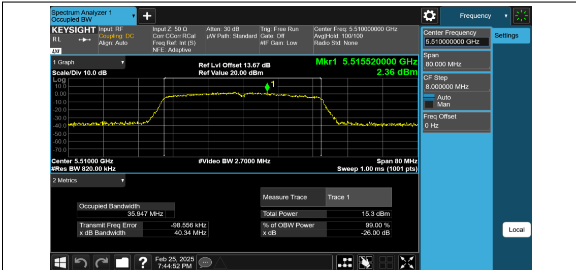
11AC40MIMO-Ant2-5510
