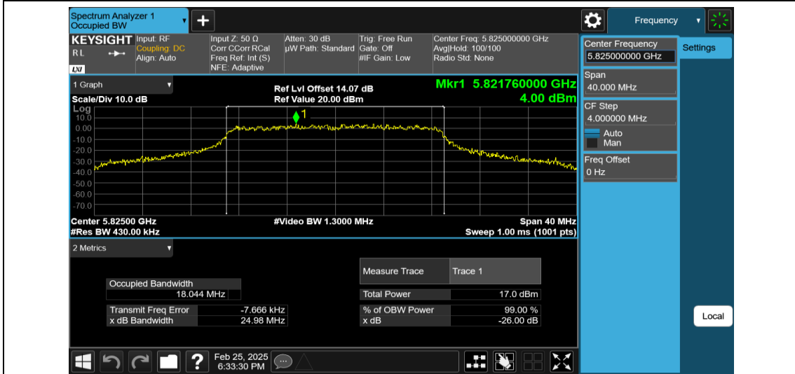
11AC20MIMO-Ant2-5825
