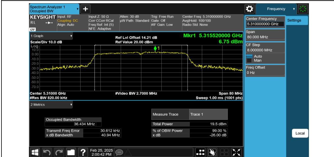
11N40MIMO-Ant2-5310
