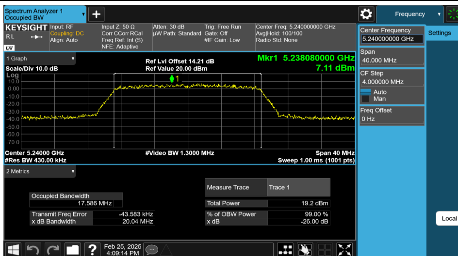
11AC20MIMO-Ant2-5240
