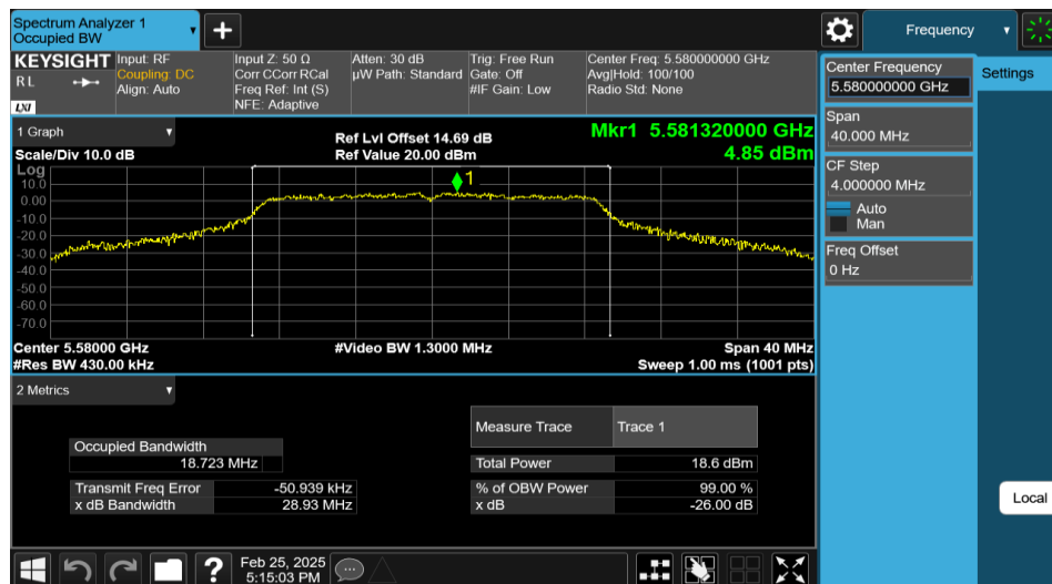
11AC20MIMO-Ant1-5580
