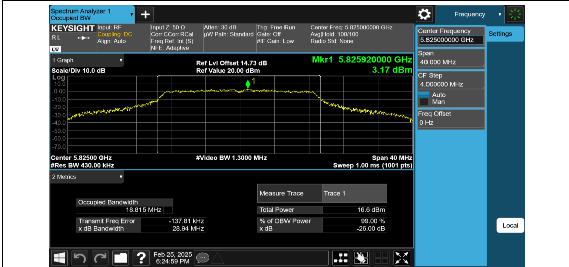
11AC20MIMO-Ant1-5825
