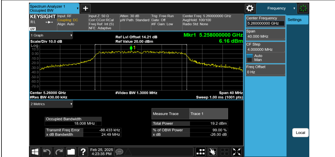
11AC20MIMO-Ant2-5260
