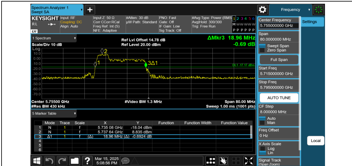
11AX40MIMO-Ant1-5755-52Tone-RU37
