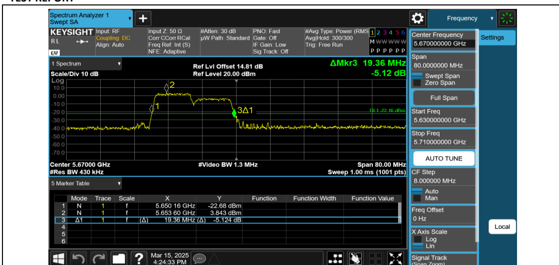
11AX40MIMO-Ant1-5670-106Tone-RU53
