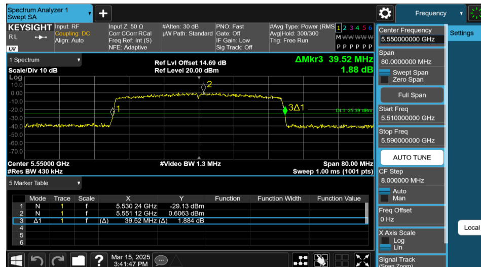
11AX40MIMO-Ant1-5550-484Tone-RU65
