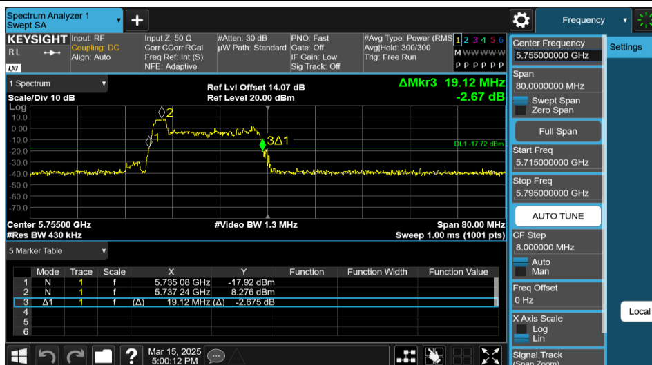
11AX40MIMO-Ant2-5755-26Tone-RU0
