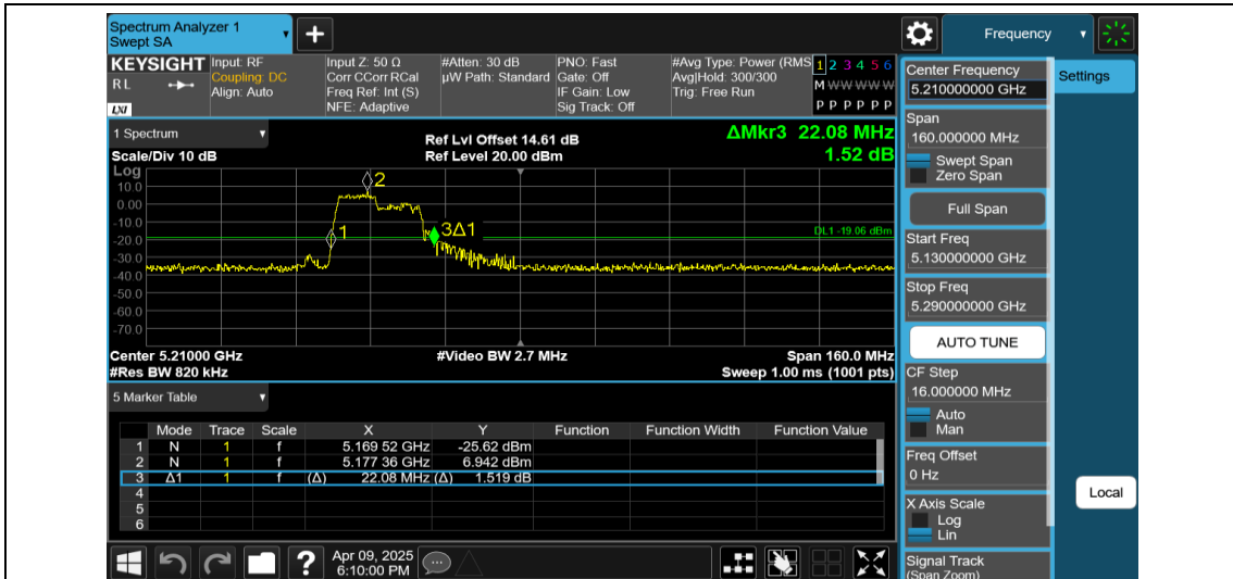
11AX80MIMO-Ant1-5210-106Tone-RU53
