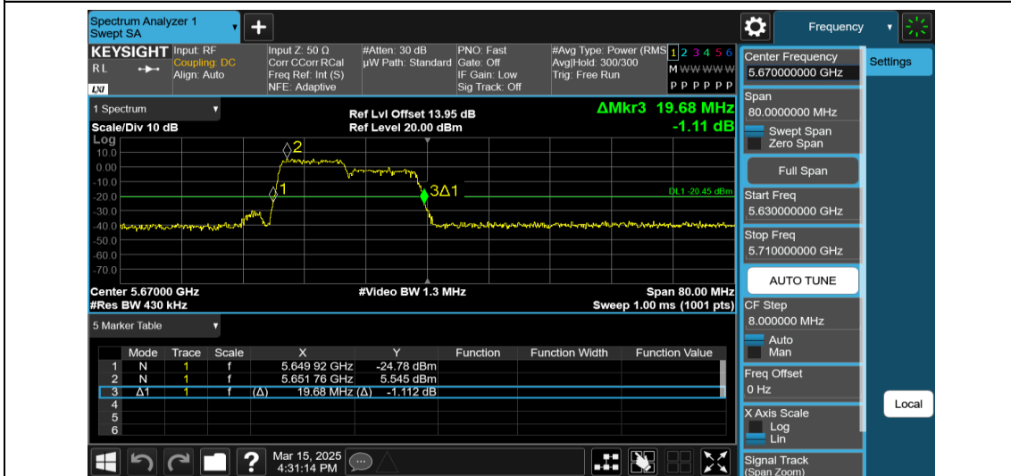
11AX40MIMO-Ant2-5670-106Tone-RU53
