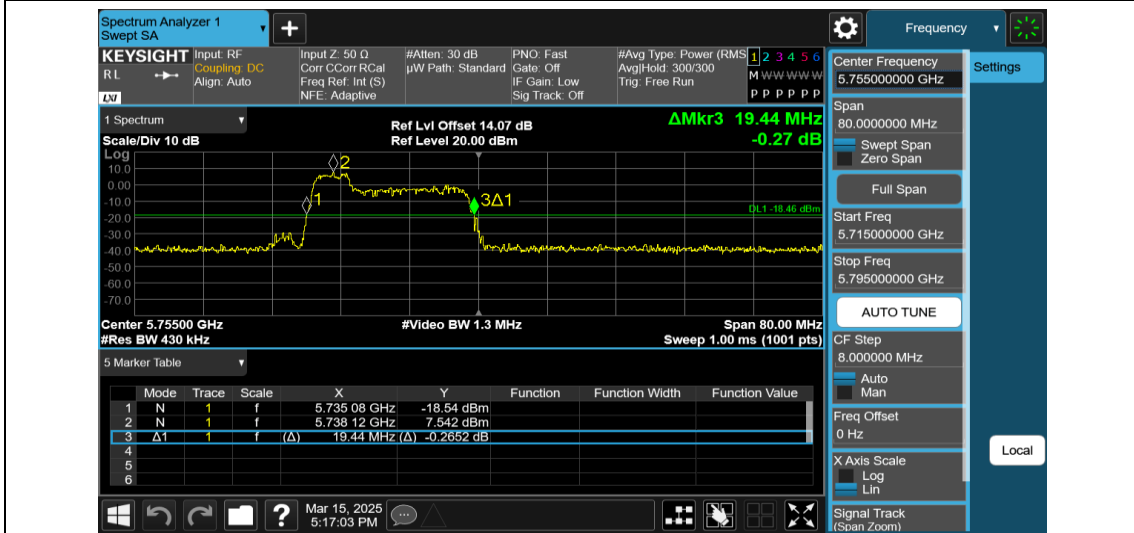
11AX40MIMO-Ant2-5755-52Tone-RU37
