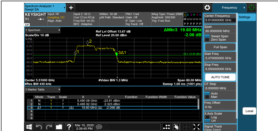
11AX40MIMO-Ant2-5510-106Tone-RU53
