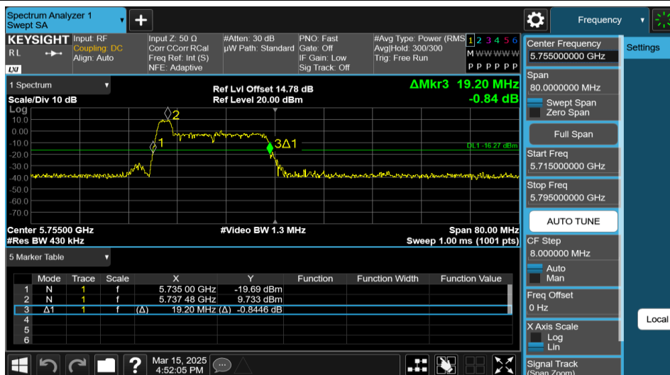
11AX40MIMO-Ant1-5755-26Tone-RU0
