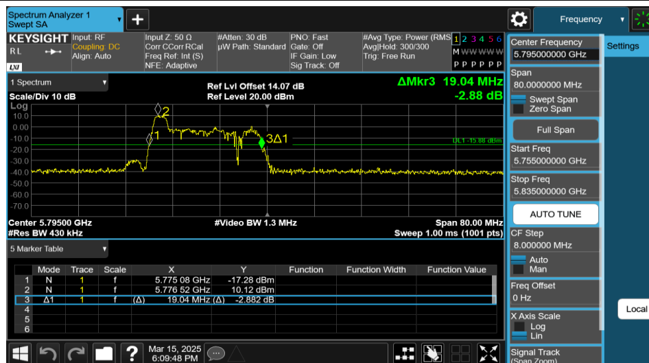
11AX40MIMO-Ant2-5795-26Tone-RU0
