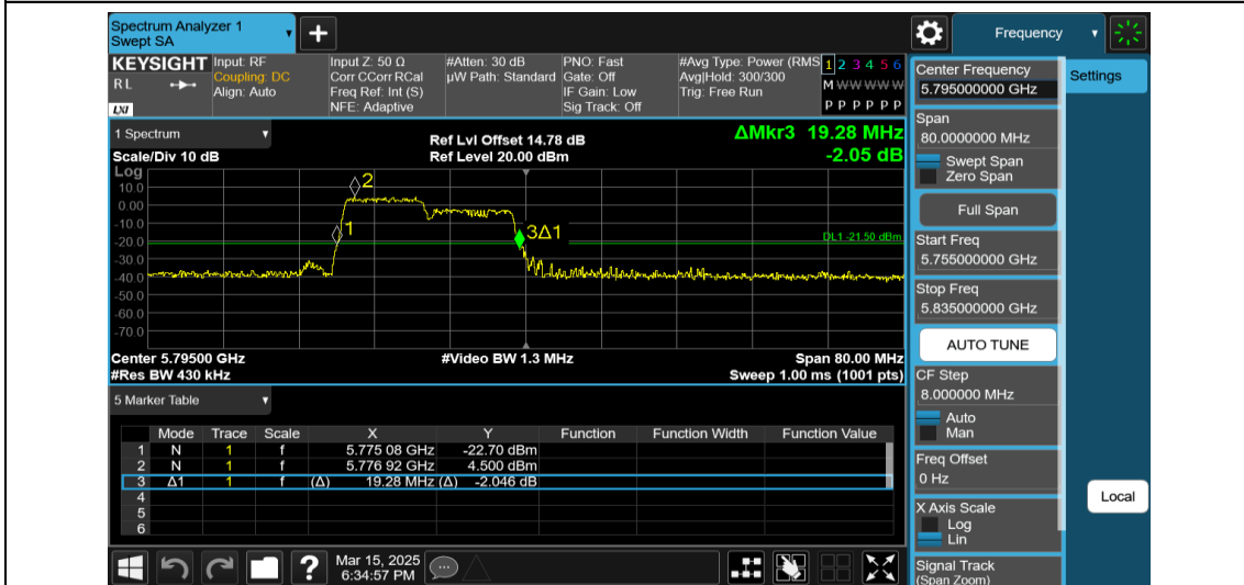
11AX40MIMO-Ant1-5795-106Tone-RU53
