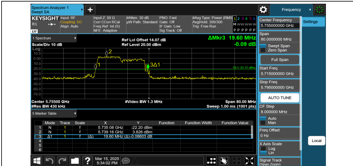
11AX40MIMO-Ant2-5755-106Tone-RU53
