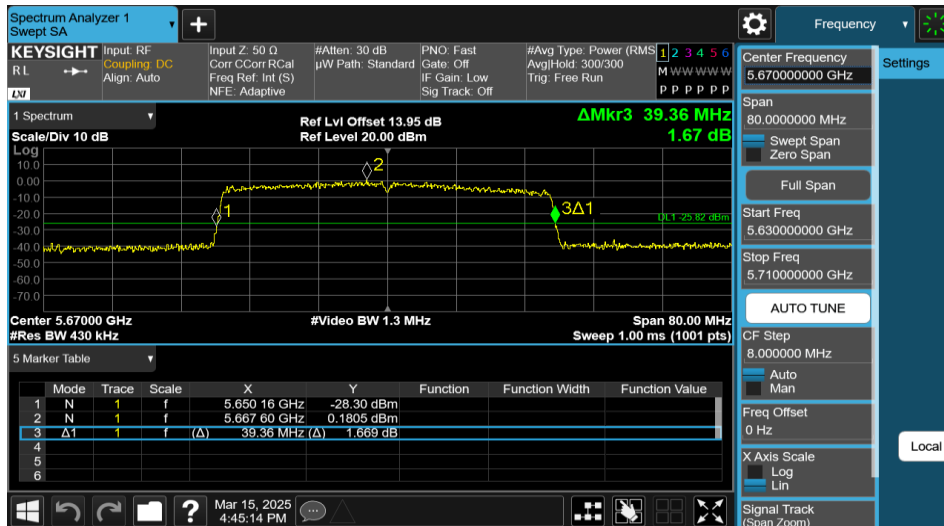
11AX40MIMO-Ant2-5670-484Tone-RU65
