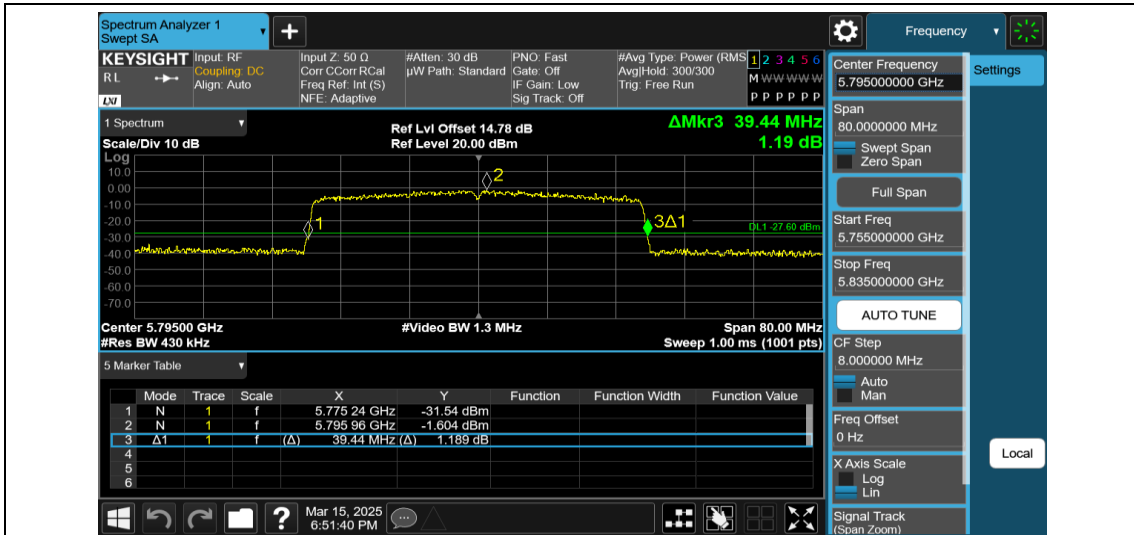
11AX40MIMO-Ant1-5795-484Tone-RU65
