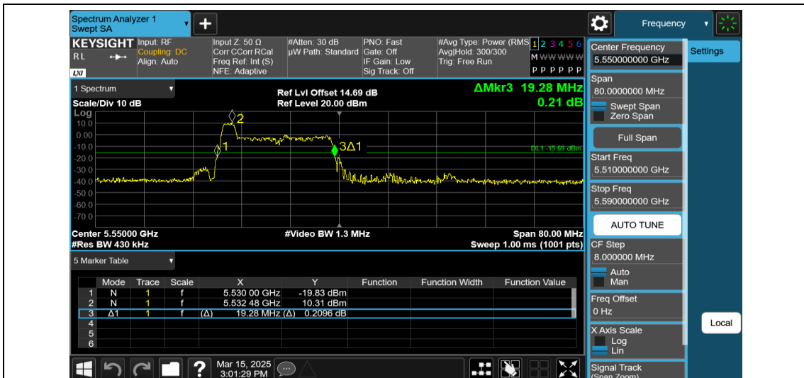
11AX40MIMO-Ant1-5550-26Tone-RU0
