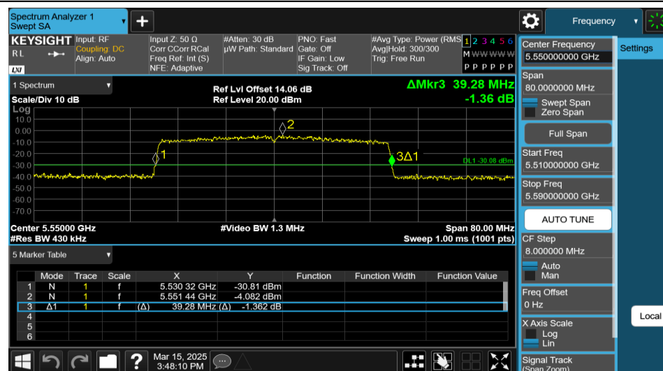
11AX40MIMO-Ant2-5550-484Tone-RU65
