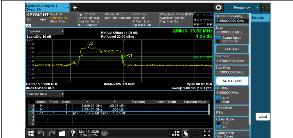
11AX40MIMO-Ant2-5550-106Tone-RU53
