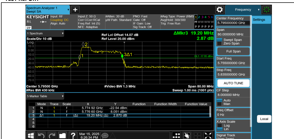
11AX40MIMO-Ant2-5795-52Tone-RU37
