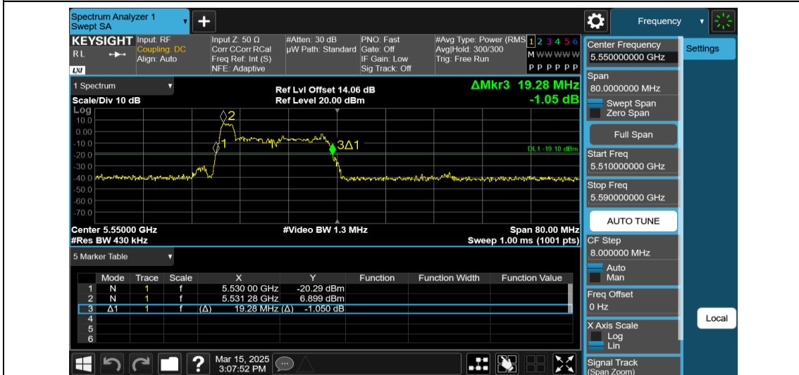
11AX40MIMO-Ant2-5550-26Tone-RU0
