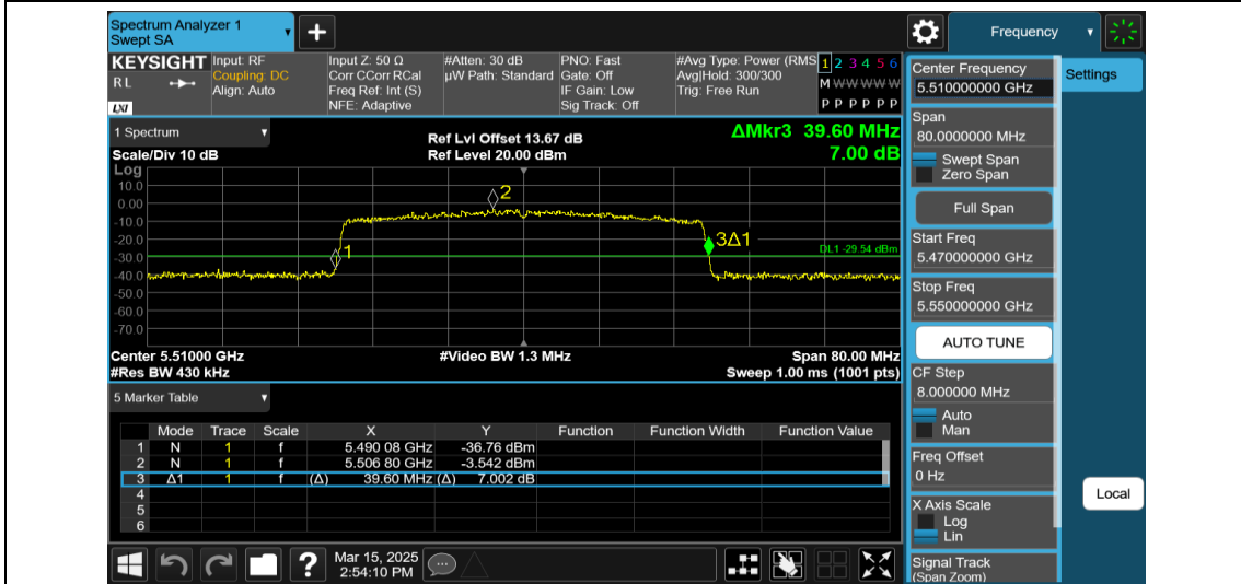
11AX40MIMO-Ant2-5510-484Tone-RU65
