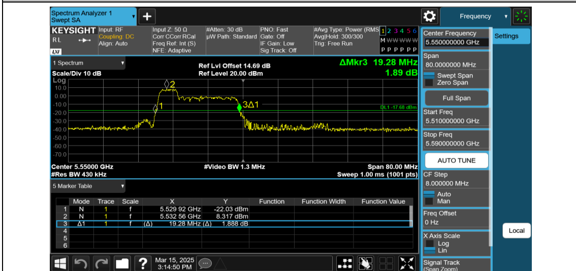
11AX40MIMO-Ant1-5550-52Tone-RU37
