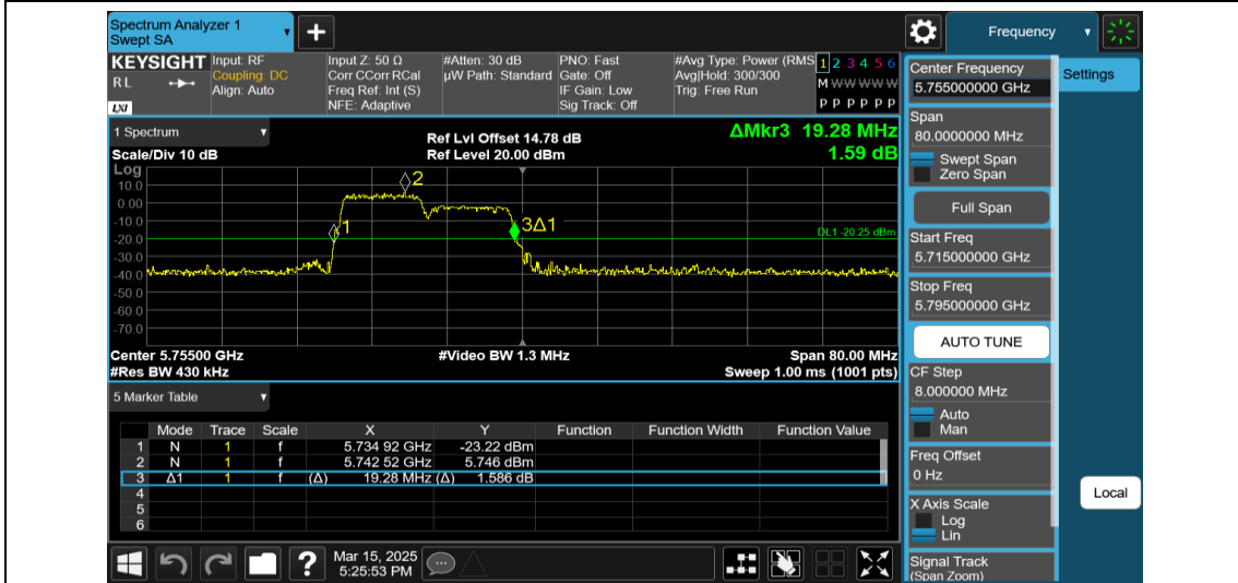
11AX40MIMO-Ant1-5755-106Tone-RU53
