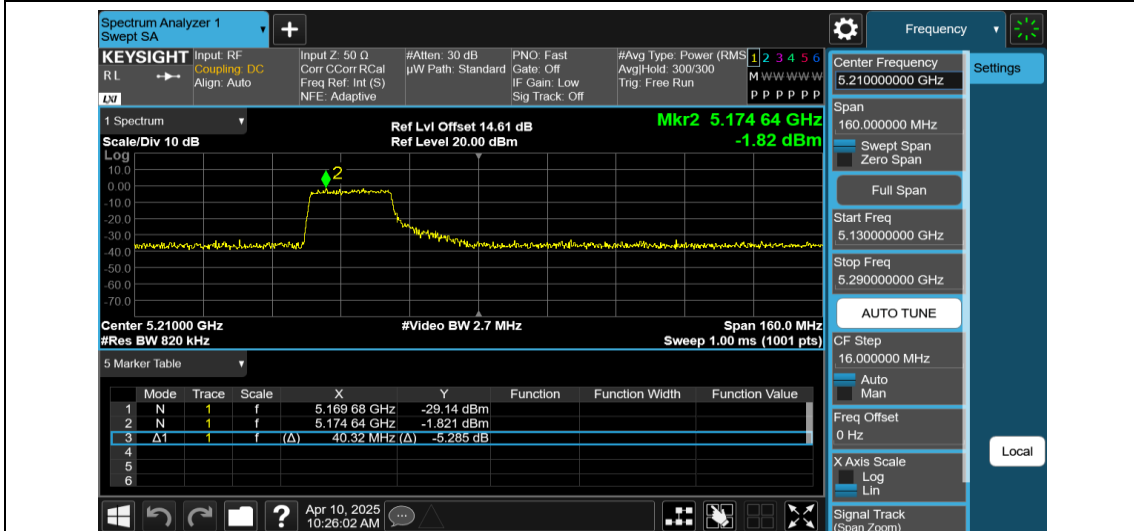
11AX80MIMO-Ant1-5210-242Tone-RU61
