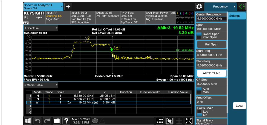
11AX40MIMO-Ant1-5550-106Tone-RU53
