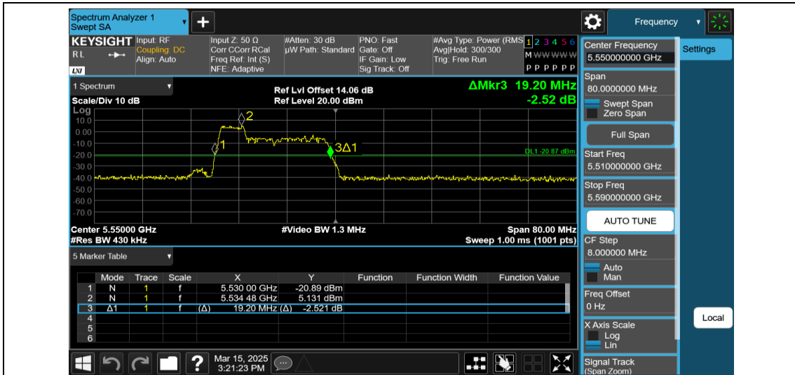
11AX40MIMO-Ant2-5550-52Tone-RU37
