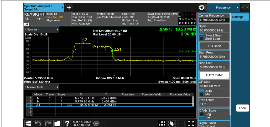
11AX40MIMO-Ant2-5795-106Tone-RU53
