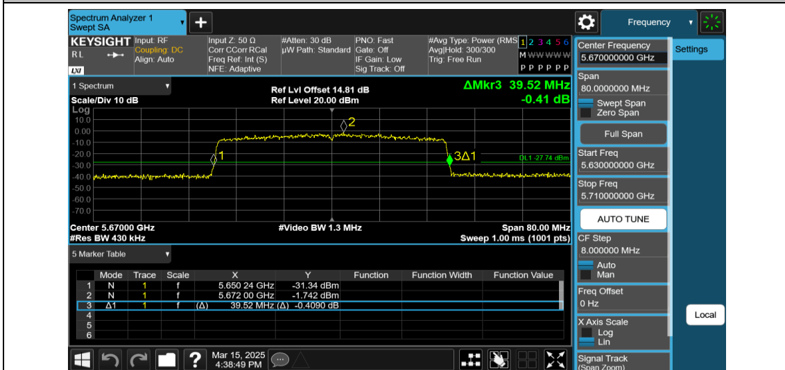
11AX40MIMO-Ant1-5670-484Tone-RU65
