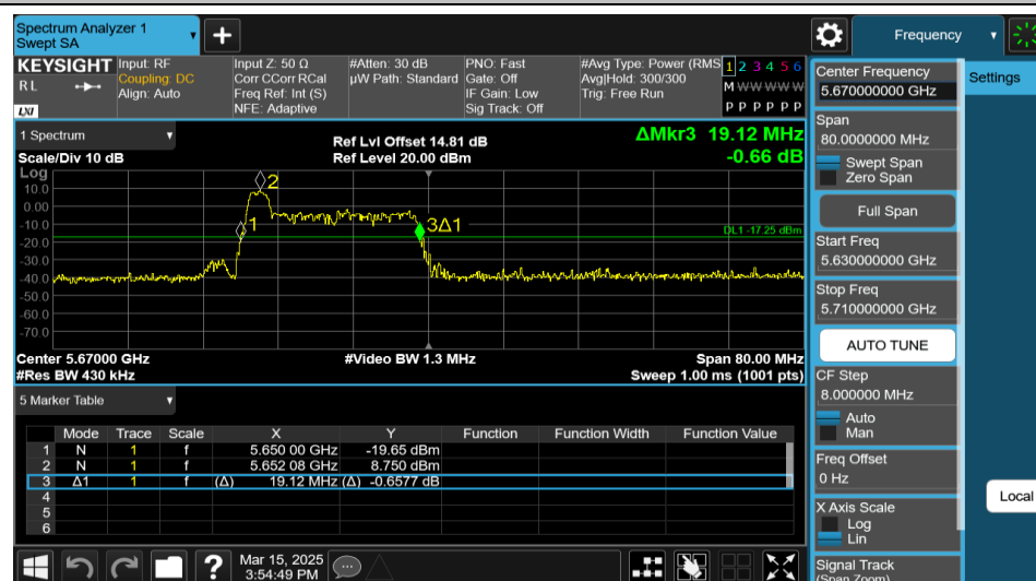
11AX40MIMO-Ant1-5670-26Tone-RU0
