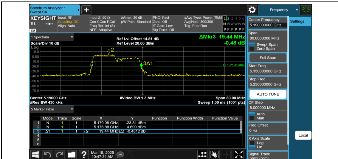
11AX40MIMO-Ant1-5190-106Tone-RU53
