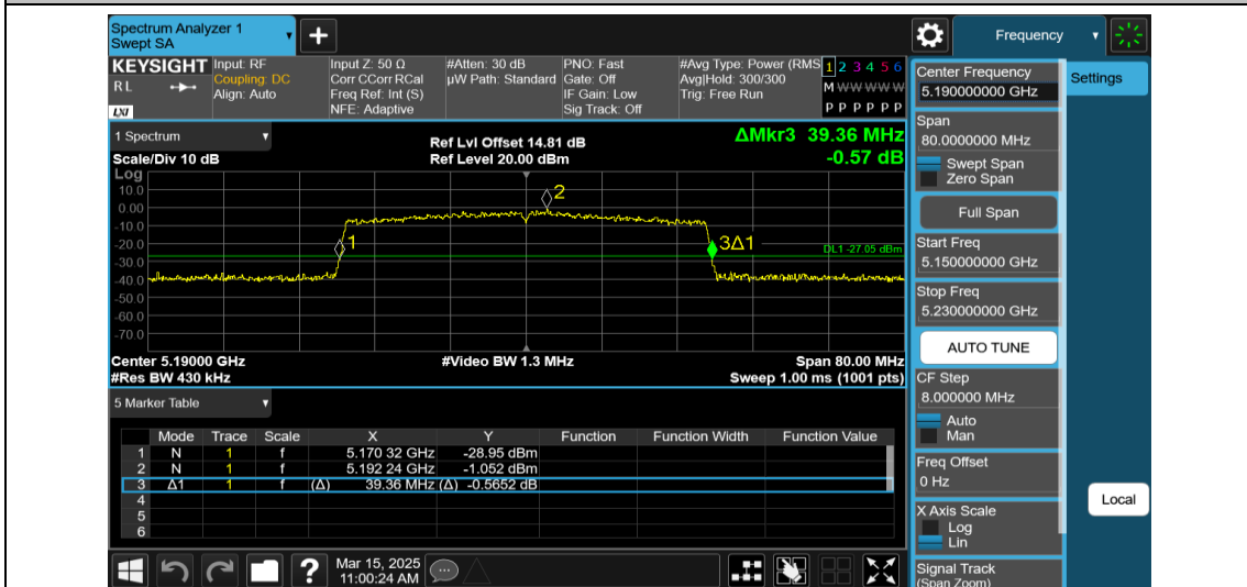
11AX40MIMO-Ant1-5190-484Tone-RU65
