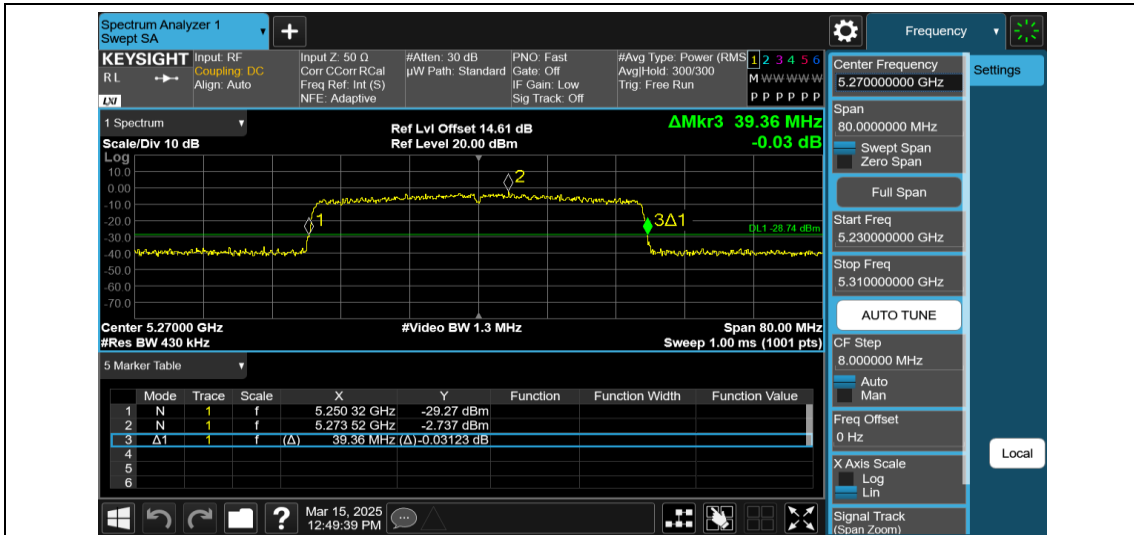
11AX40MIMO-Ant1-5270-484Tone-RU65
