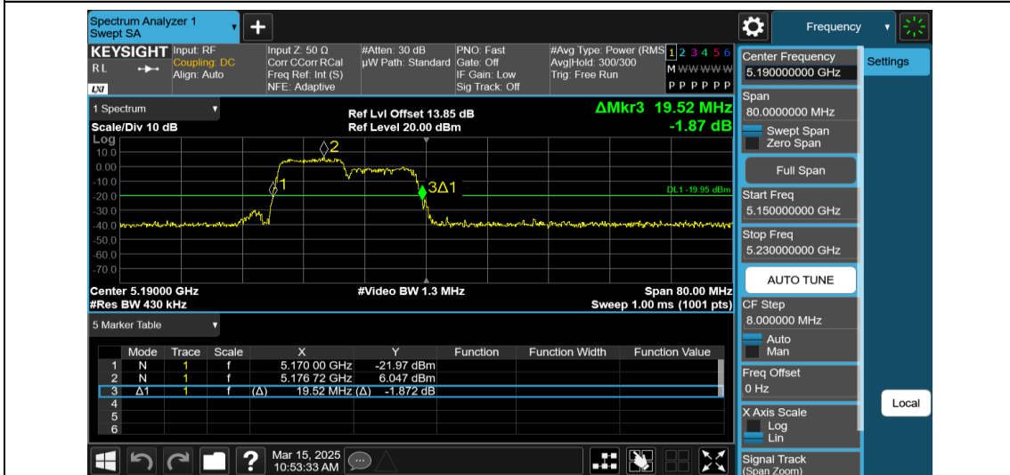
11AX40MIMO-Ant2-5190-106Tone-RU53
