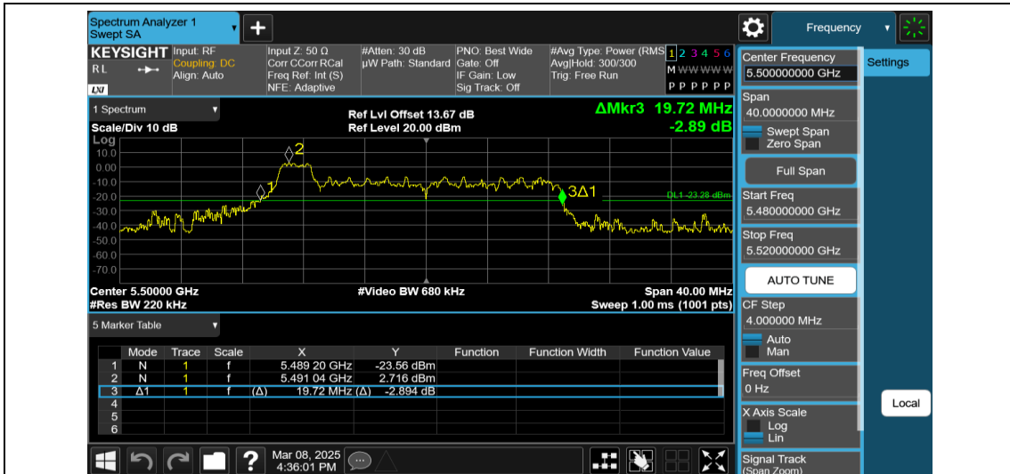
11AX20MIMO-Ant2-5500-26Tone-RU0
