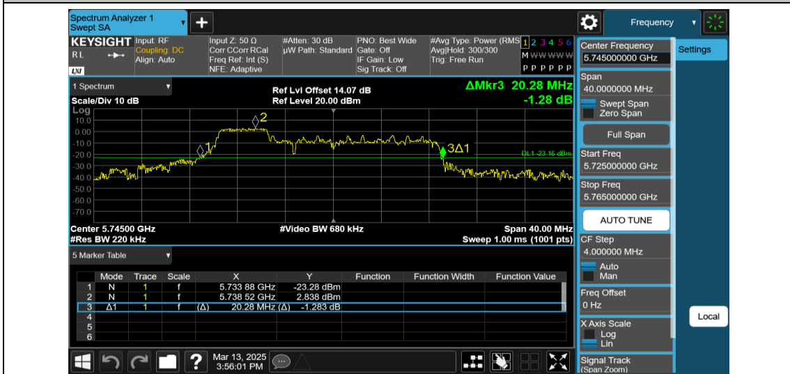
11AX20MIMO-Ant2-5745-52Tone-RU37
