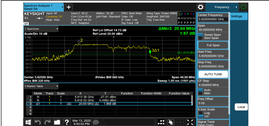
11AX20MIMO-Ant1-5825-106Tone-RU53
