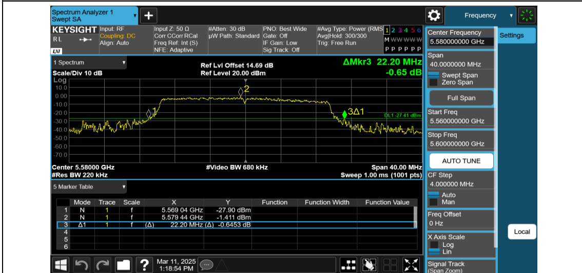
11AX20MIMO-Ant1-5580-242Tone-RU61
