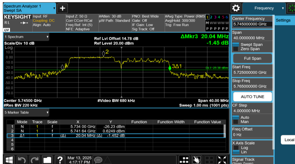
11AX20MIMO-Ant1-5745-106Tone-RU53
