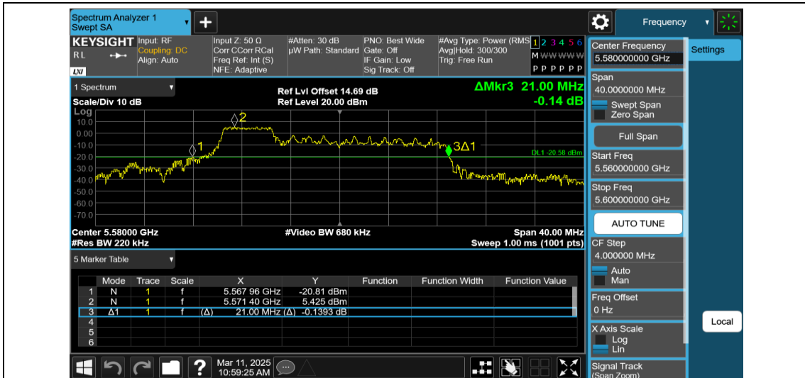
11AX20MIMO-Ant1-5580-52Tone-RU37
