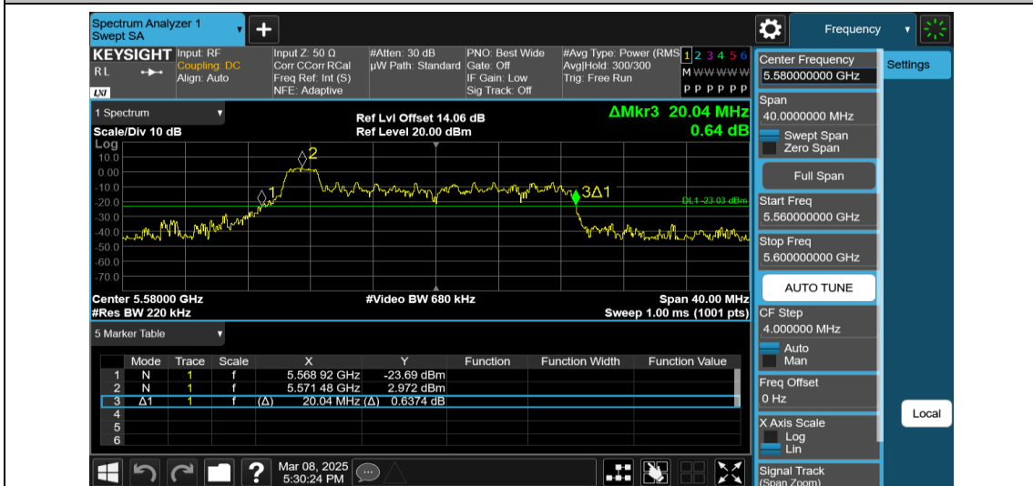
11AX20MIMO-Ant2-5580-26Tone-RU0
