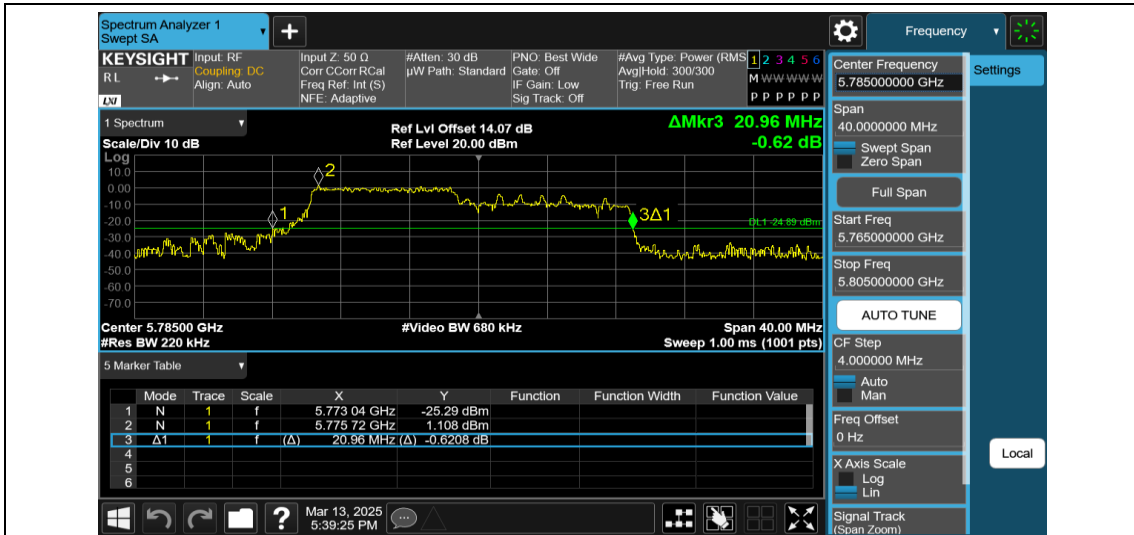
11AX20MIMO-Ant2-5785-106Tone-RU53
