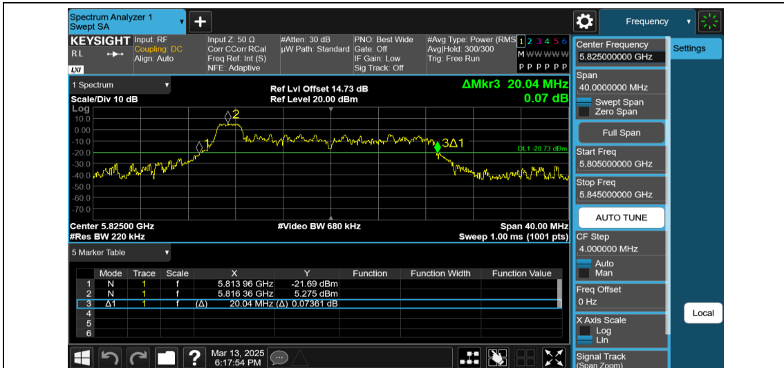
11AX20MIMO-Ant1-5825-26Tone-RU0
