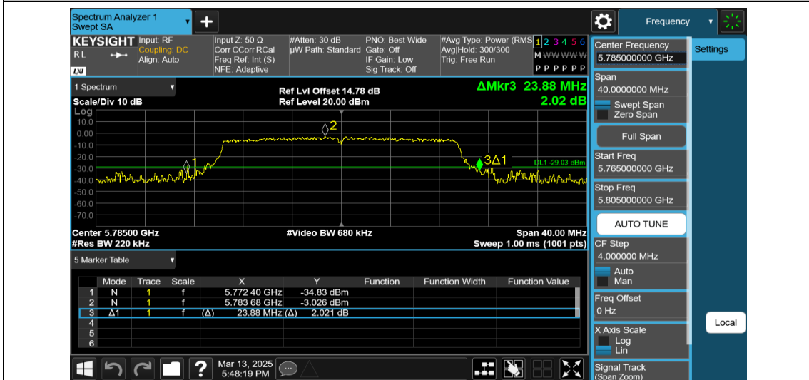
11AX20MIMO-Ant1-5785-242Tone-RU61
