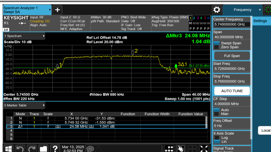
11AX20MIMO-Ant1-5745-242Tone-RU61
