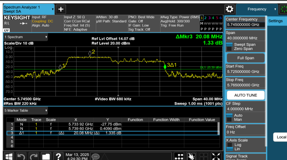
11AX20MIMO-Ant2-5745-106Tone-RU53
