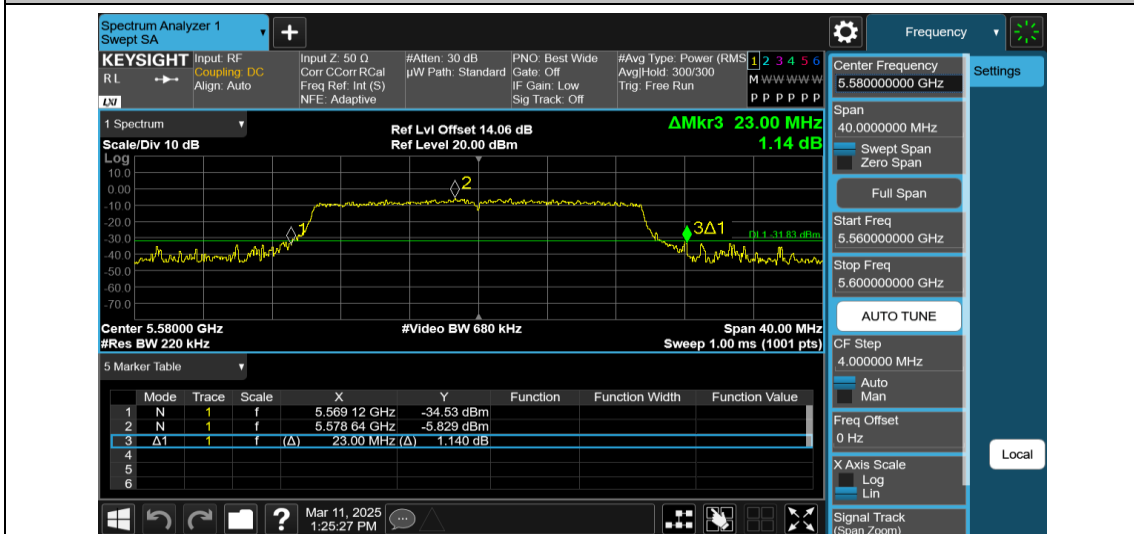
11AX20MIMO-Ant2-5580-242Tone-RU61
