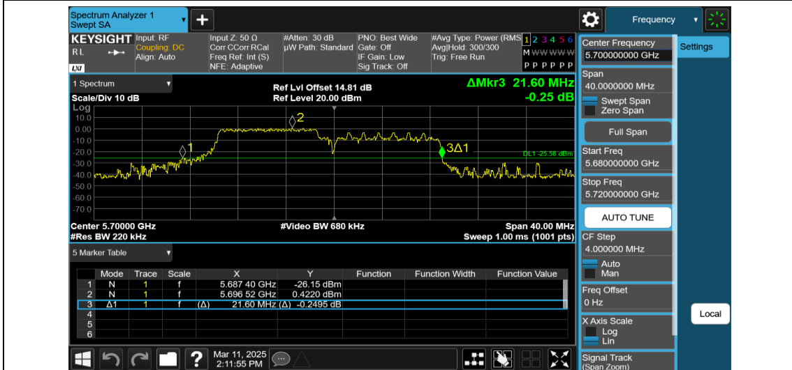
11AX20MIMO-Ant1-5700-106Tone-RU53
