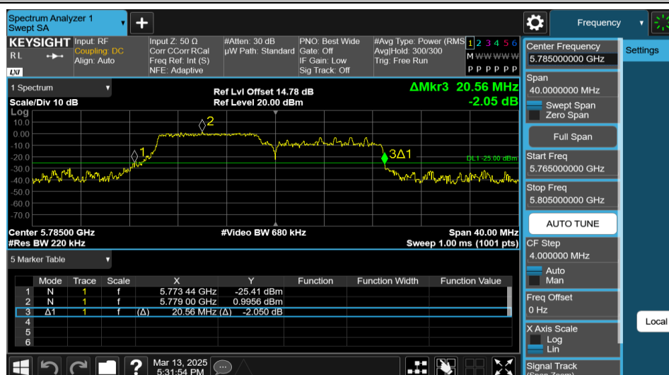
11AX20MIMO-Ant1-5785-106Tone-RU53
