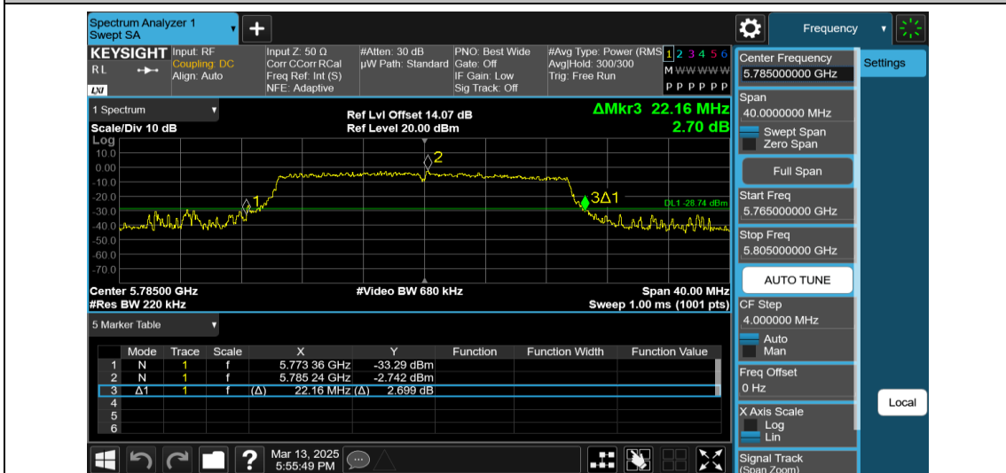
11AX20MIMO-Ant2-5785-242Tone-RU61
