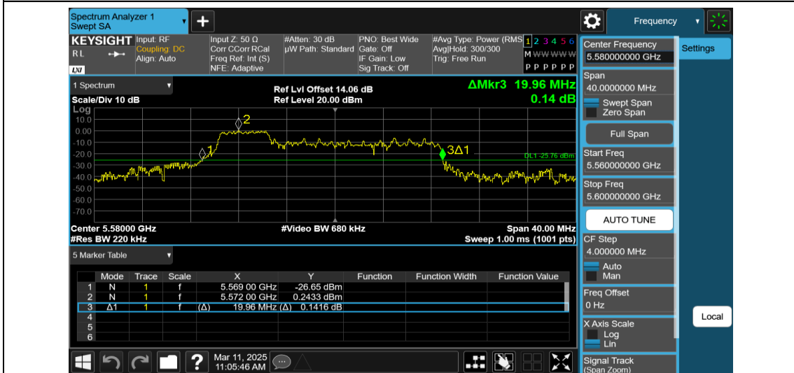
11AX20MIMO-Ant2-5580-52Tone-RU37
