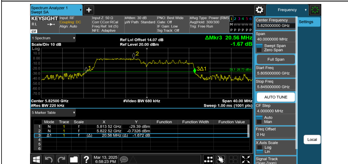
11AX20MIMO-Ant2-5825-106Tone-RU53
