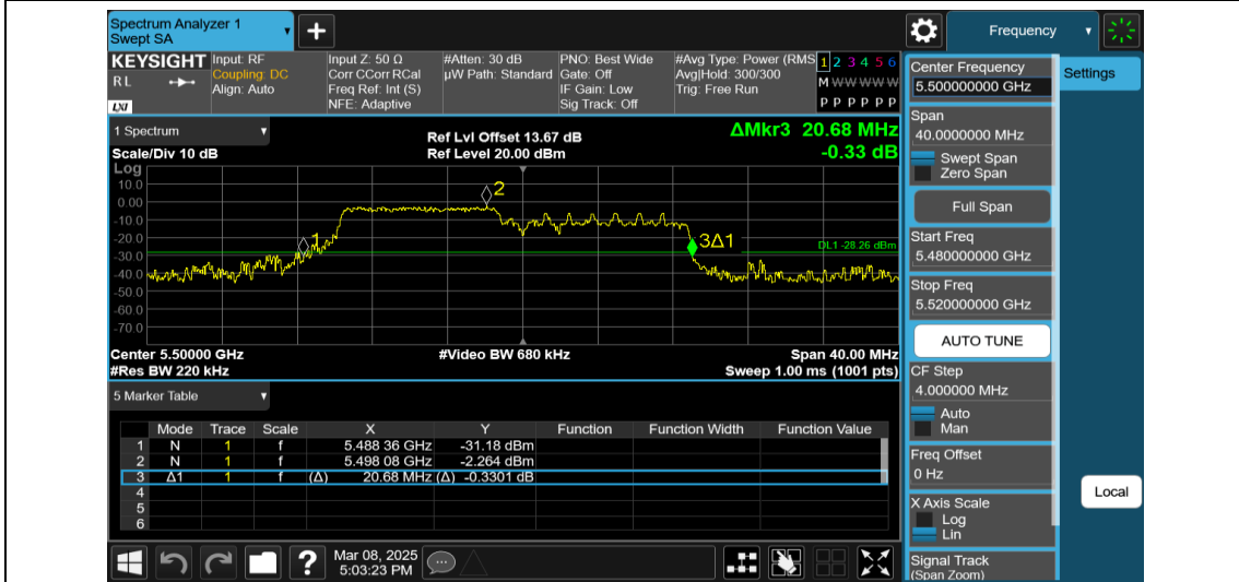
11AX20MIMO-Ant2-5500-106Tone-RU53
