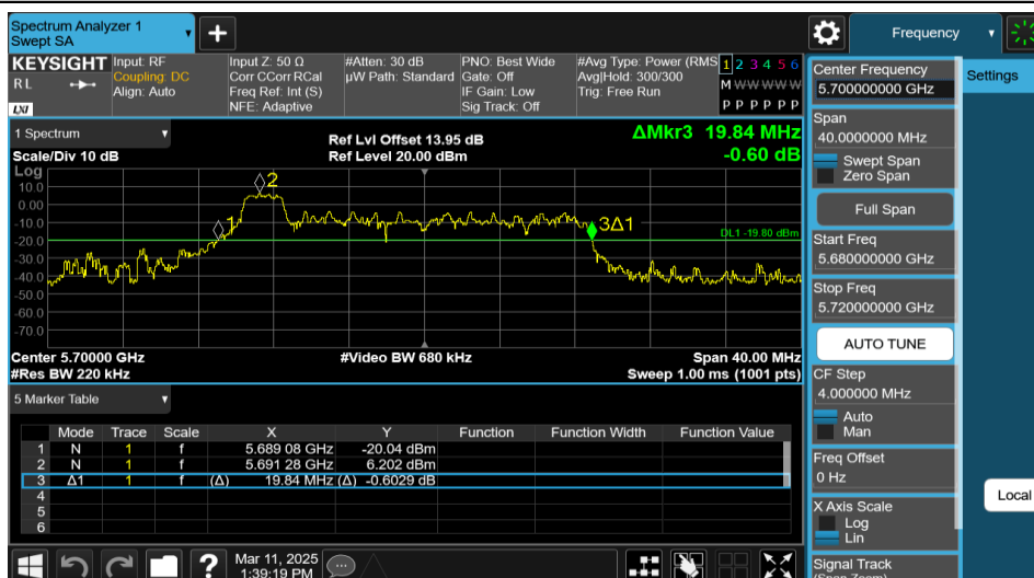
11AX20MIMO-Ant2-5700-26Tone-RU0
