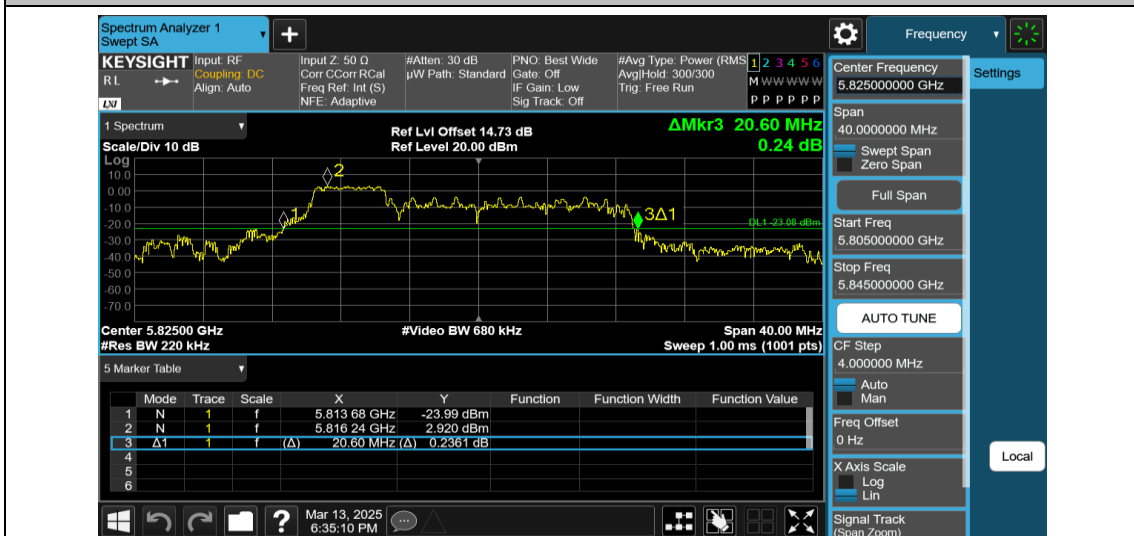
11AX20MIMO-Ant1-5825-52Tone-RU37
