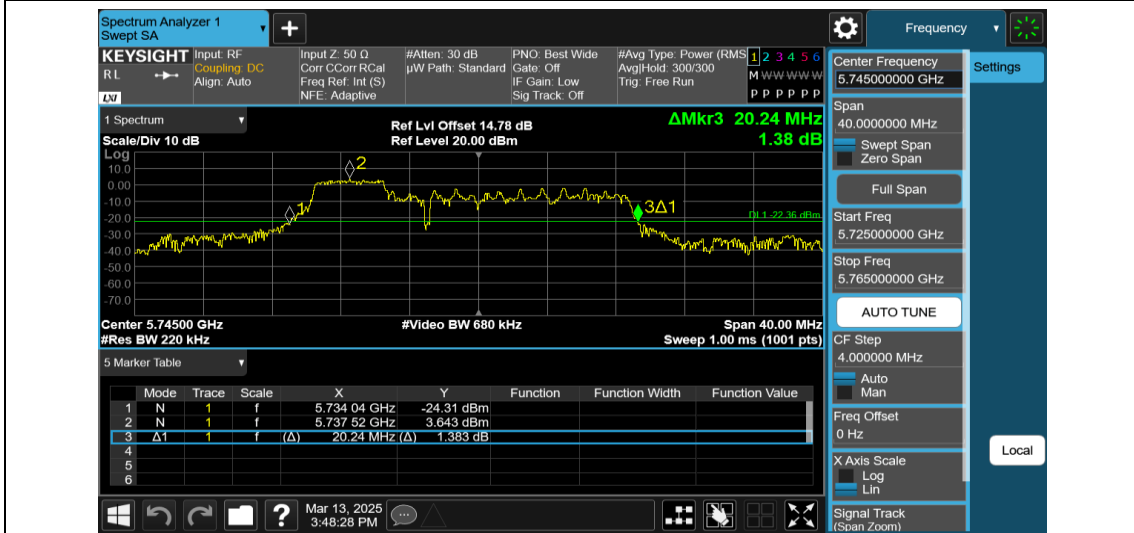
11AX20MIMO-Ant1-5745-52Tone-RU37
