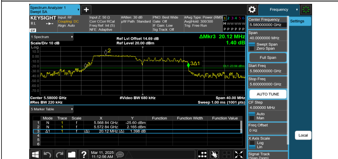
11AX20MIMO-Ant1-5580-106Tone-RU53
