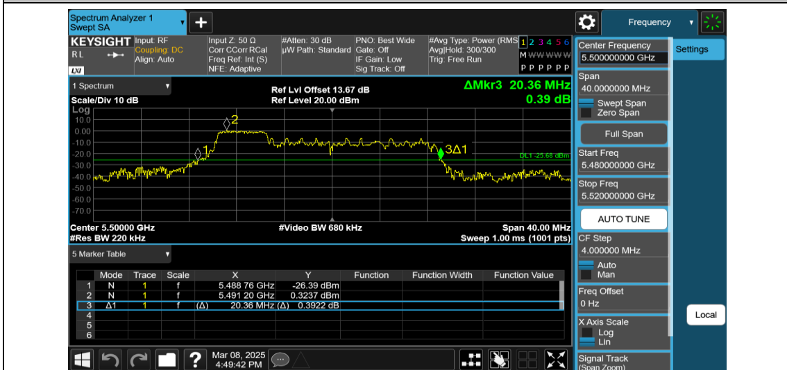
11AX20MIMO-Ant2-5500-52Tone-RU37
