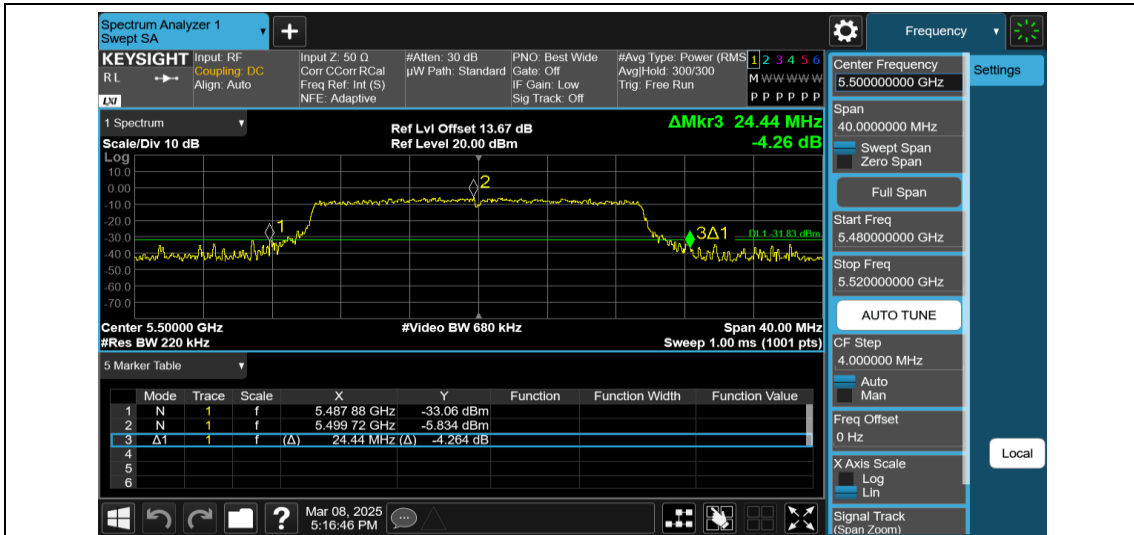
11AX20MIMO-Ant2-5500-242Tone-RU61
