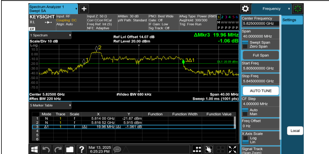
11AX20MIMO-Ant2-5825-26Tone-RU0
