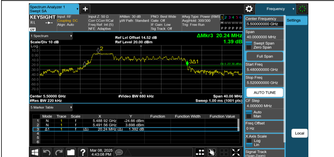
11AX20MIMO-Ant1-5500-52Tone-RU37
