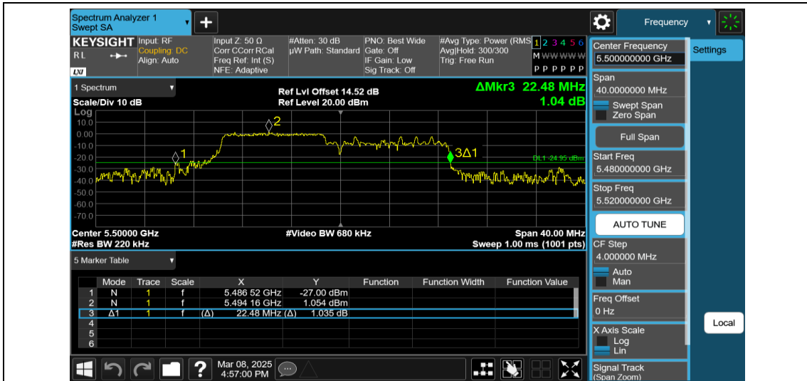
11AX20MIMO-Ant1-5500-106Tone-RU53
