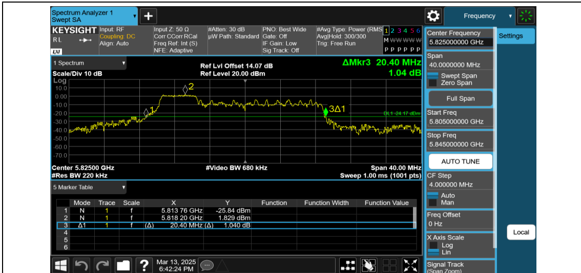
11AX20MIMO-Ant2-5825-52Tone-RU37
