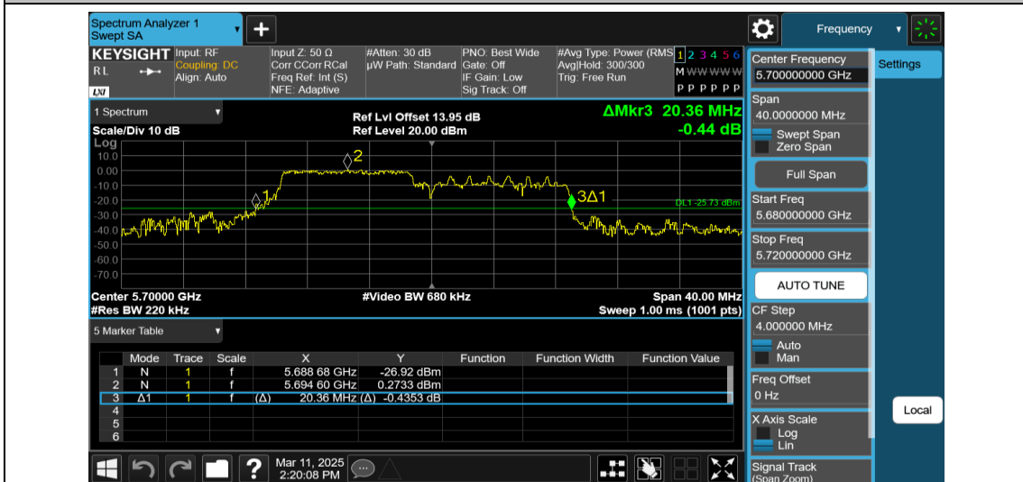
11AX20MIMO-Ant2-5700-106Tone-RU53
