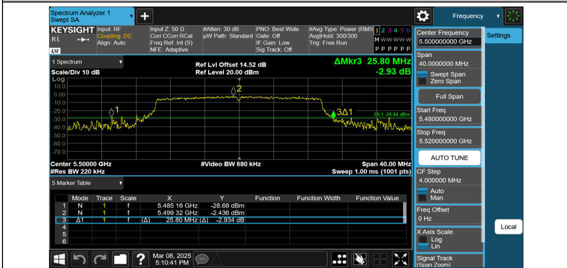
11AX20MIMO-Ant1-5500-242Tone-RU61
