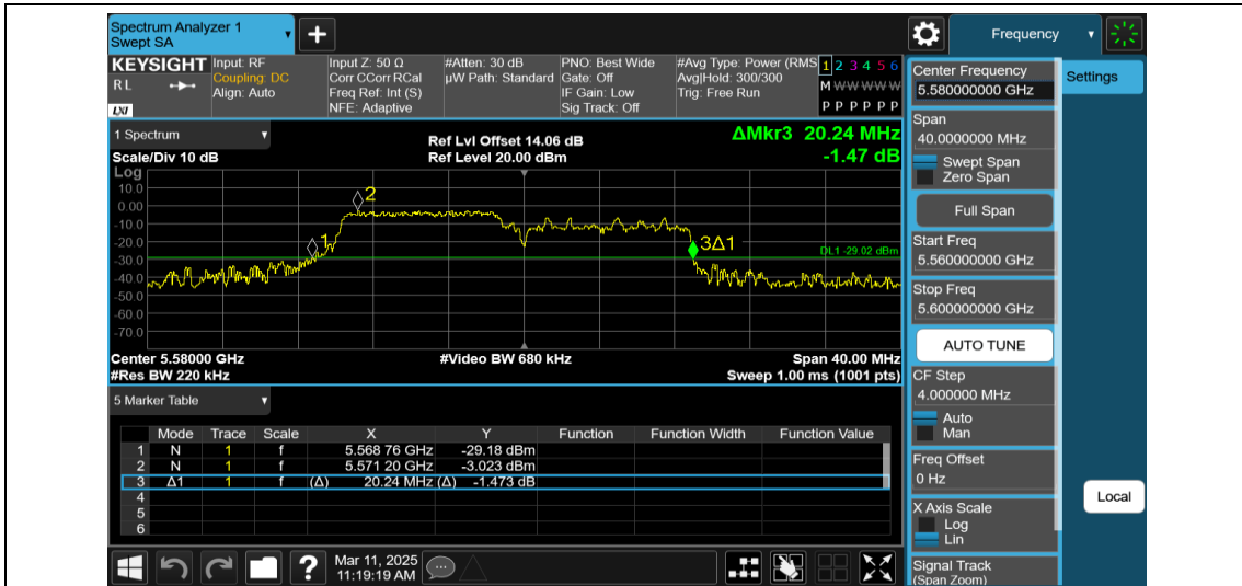
11AX20MIMO-Ant2-5580-106Tone-RU53
