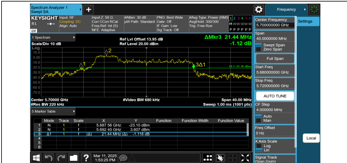
11AX20MIMO-Ant2-5700-52Tone-RU37
