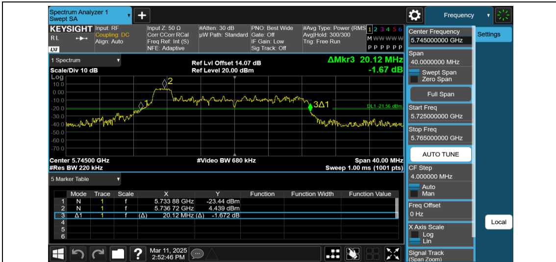
11AX20MIMO-Ant2-5745-26Tone-RU0
