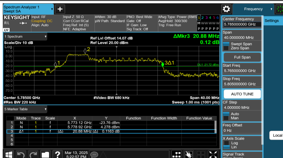
11AX20MIMO-Ant2-5785-52Tone-RU37
