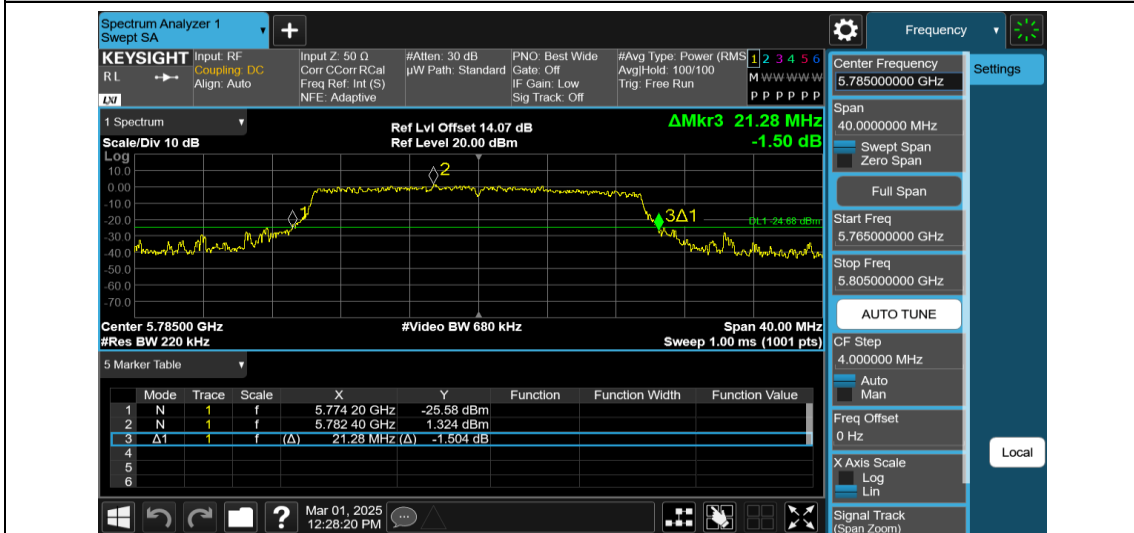
11AX20MIMO-Ant2-5785
