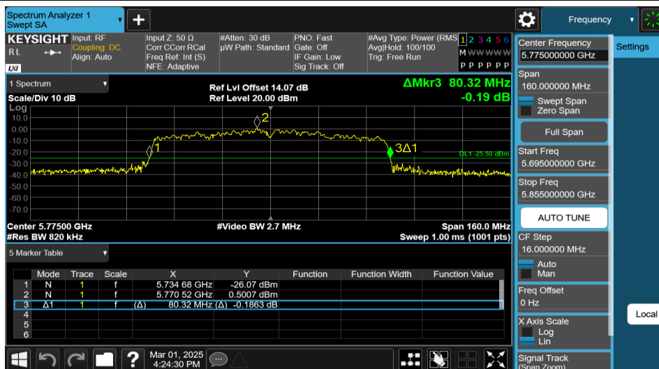
11AX80MIMO-Ant2-5775
