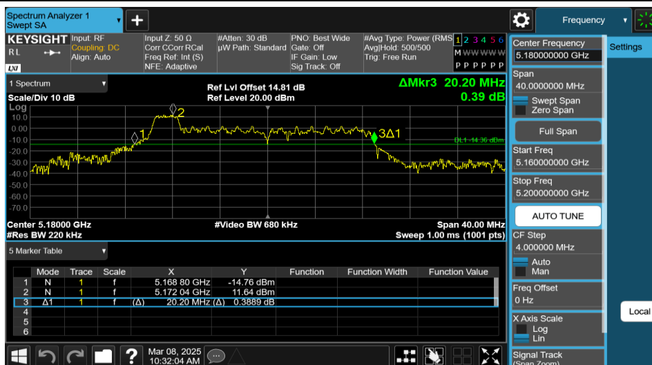
11AX20MIMO-Ant1-5180-26Tone-RU0
