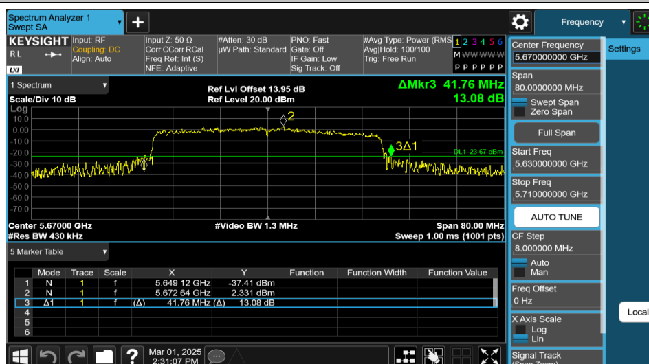
11AX40MIMO-Ant2-5670
