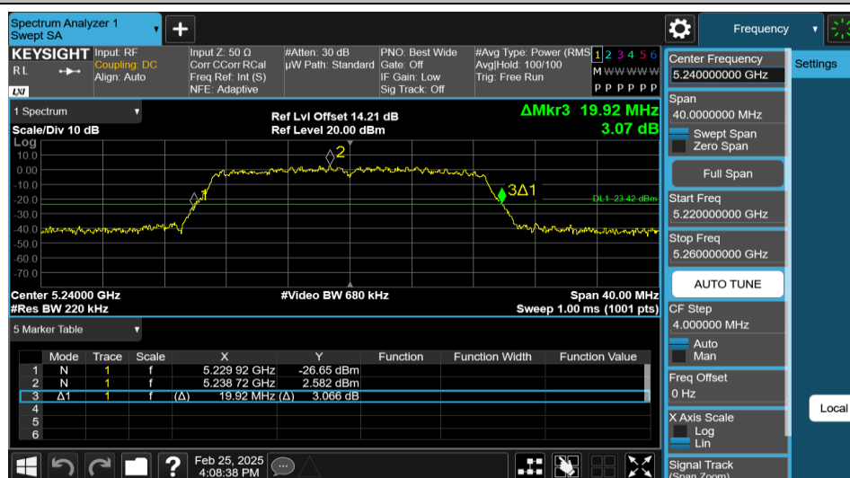
11AC20MIMO-Ant2-5240
