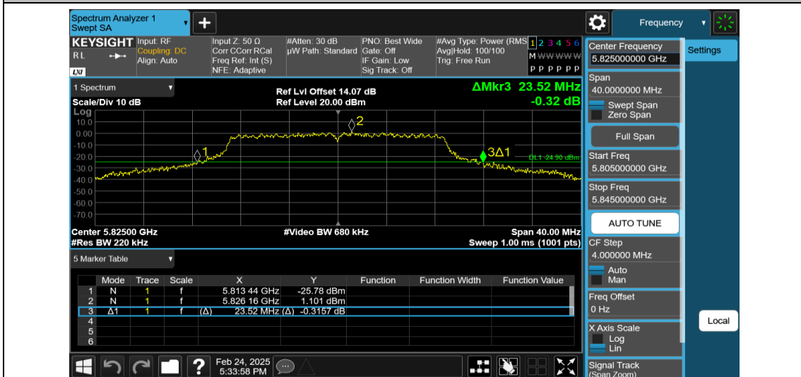
11N20MIMO-Ant2-5825
