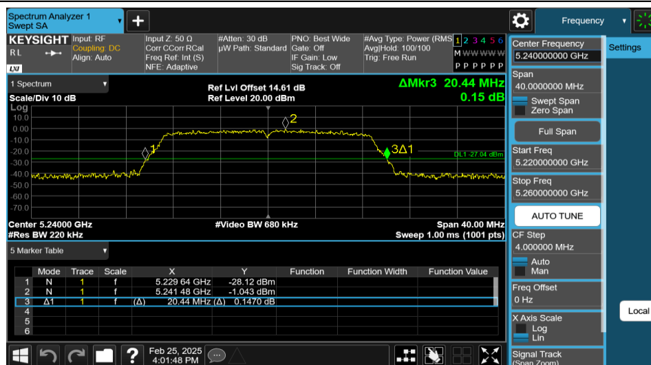
11AC20MIMO-Ant1-5240
