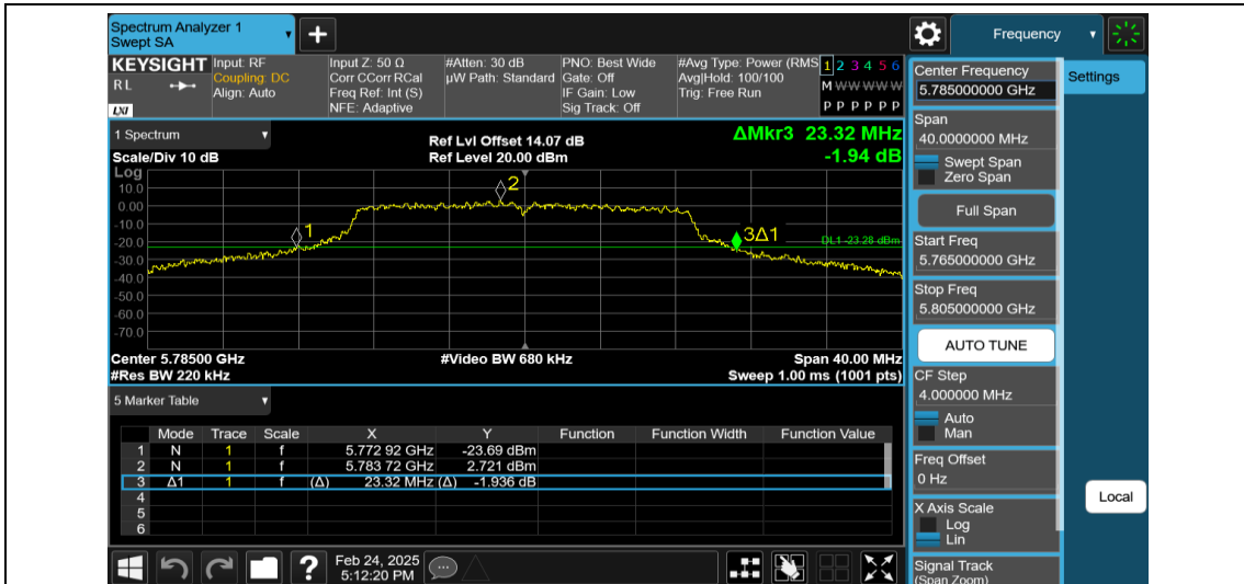
11N20MIMO-Ant2-5785
