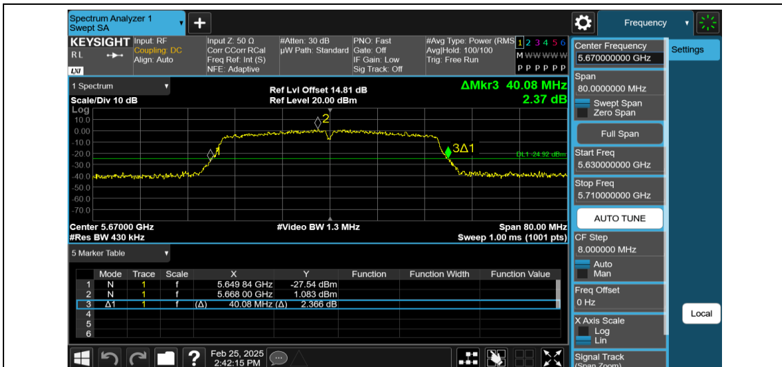
11N40MIMO-Ant1-5670
