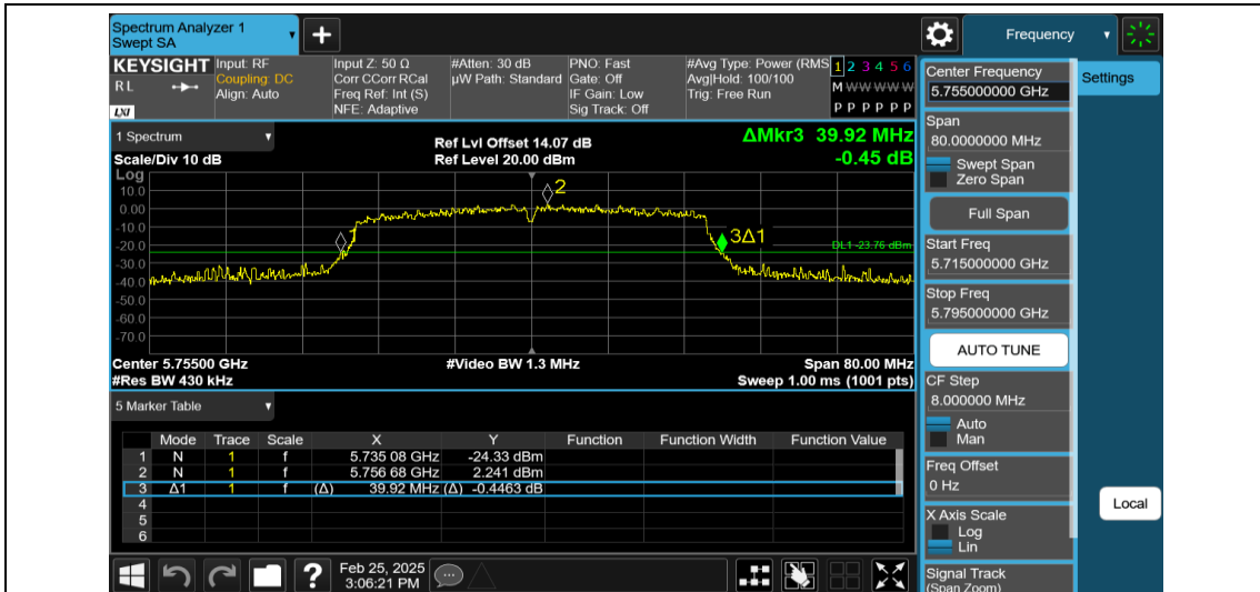
11N40MIMO-Ant2-5755
