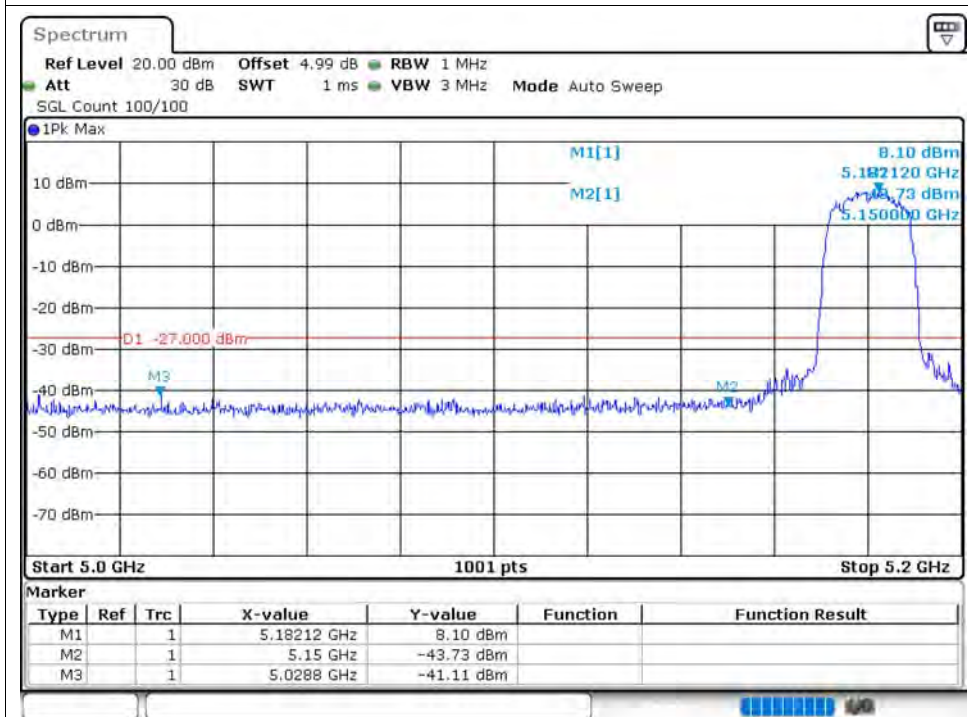
Band Edge NVNT n20 5180MHz Low Ant2
